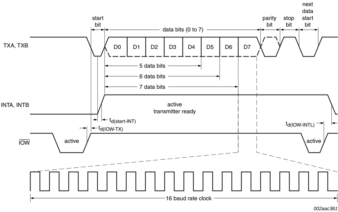
Fig 17. Transmit timing
