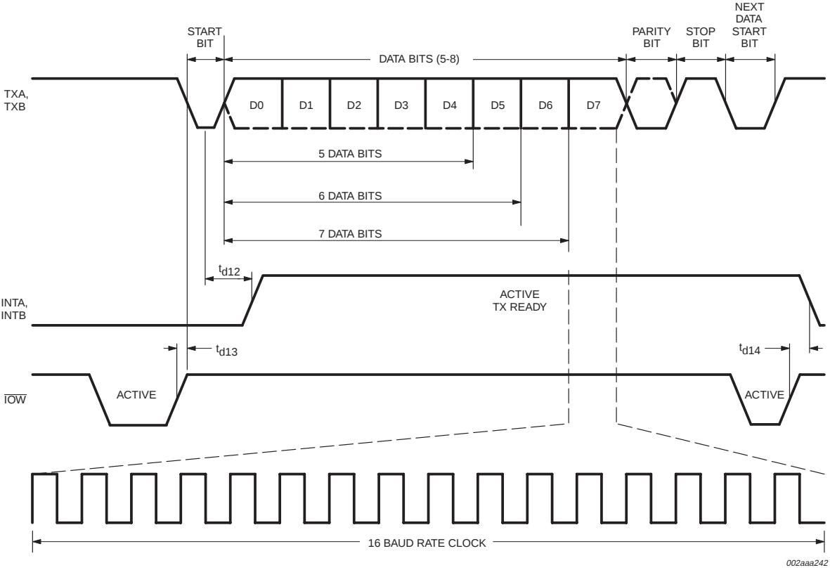
Fig 20. Transmit timing.
