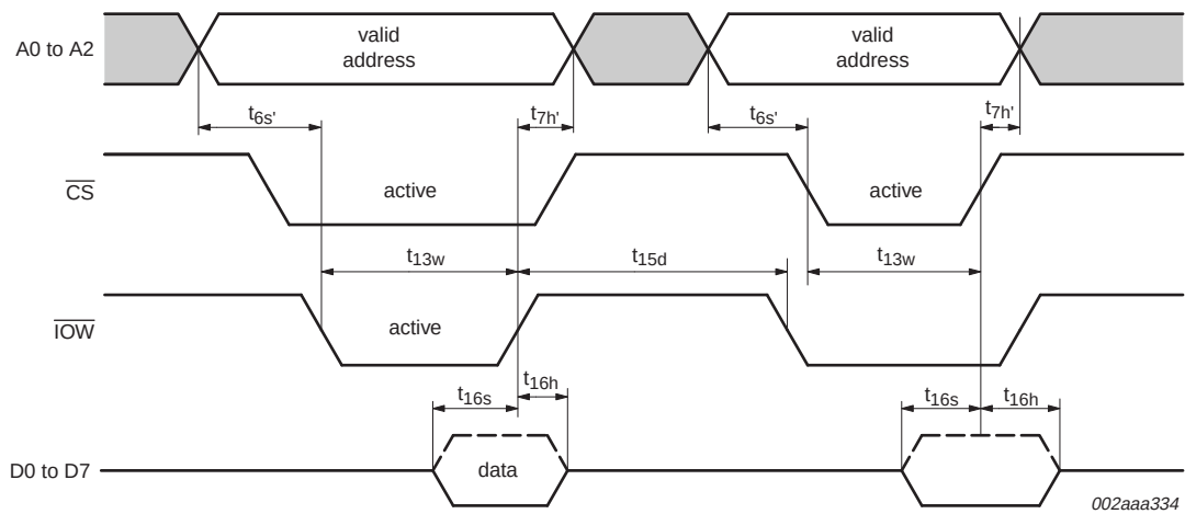
Fig 10. General write timing when \overline{AS} is tied to GND
