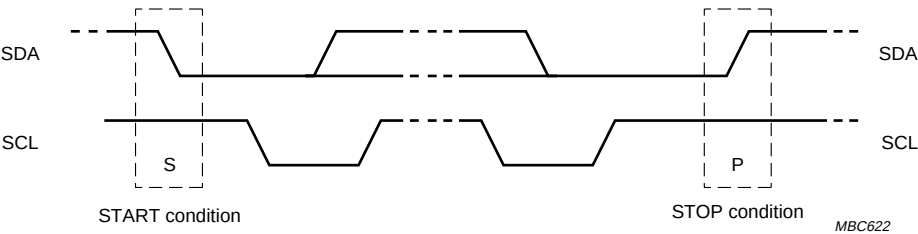
Fig.4 Definition of START and STOP conditions.
