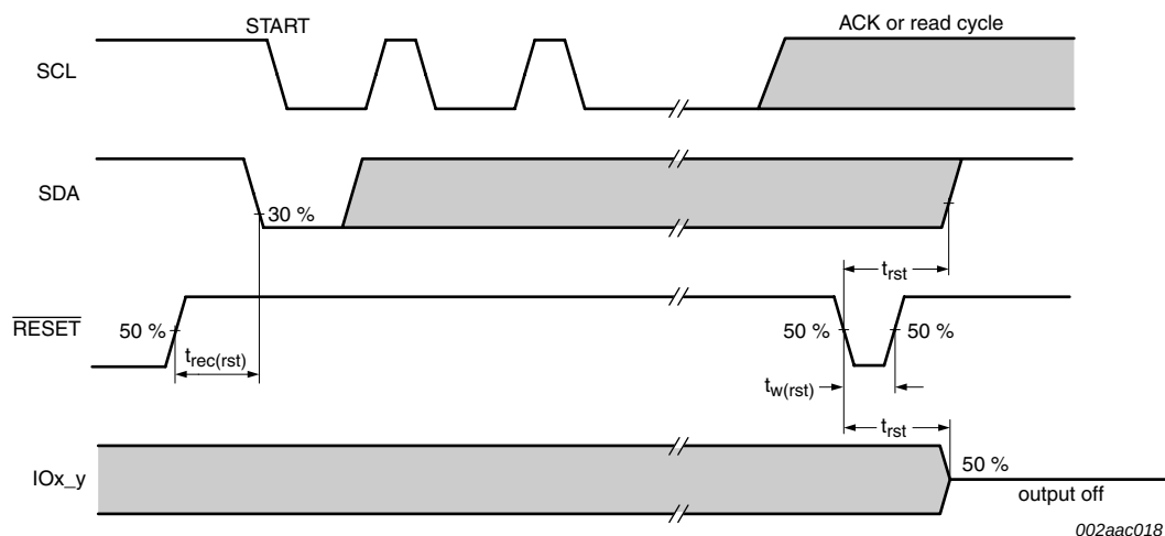
Fig 39. Reset timing
