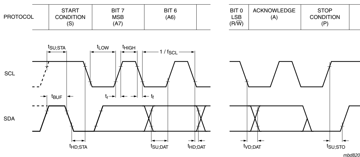
Fig 23. I 2 C-bus timing diagram
