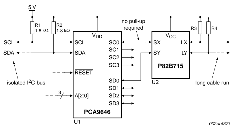
Fig 15. PCA9646 isolating the standard I 2 C-bus from a P82B715 used as a line driver
