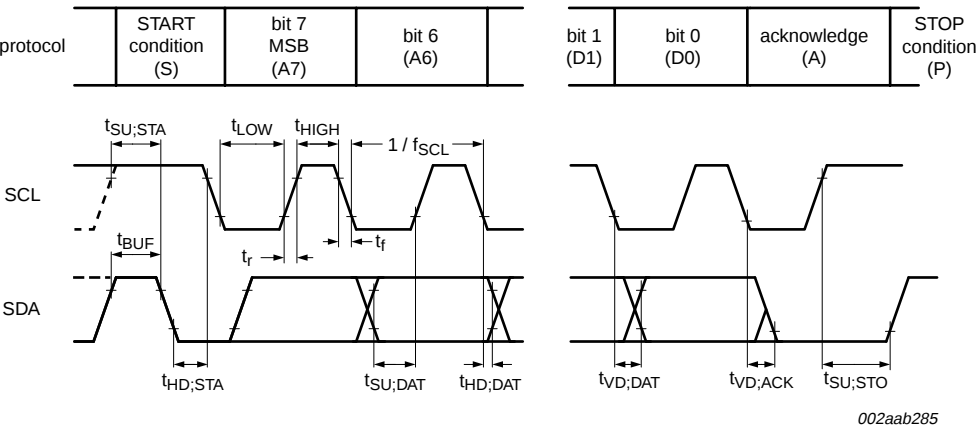
Fig 13. I 2 C-bus timing diagram
