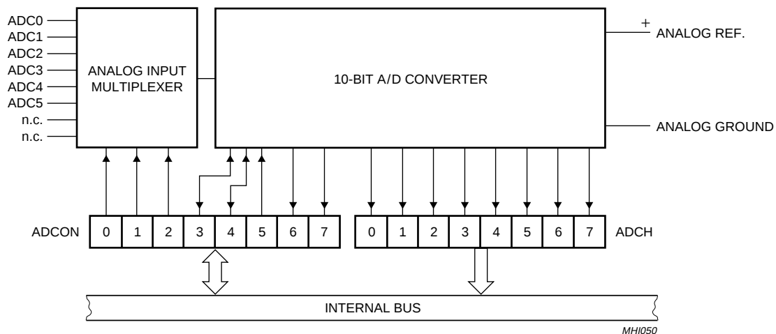
Fig.48 Functional diagram of Analog Input Circuitry.
