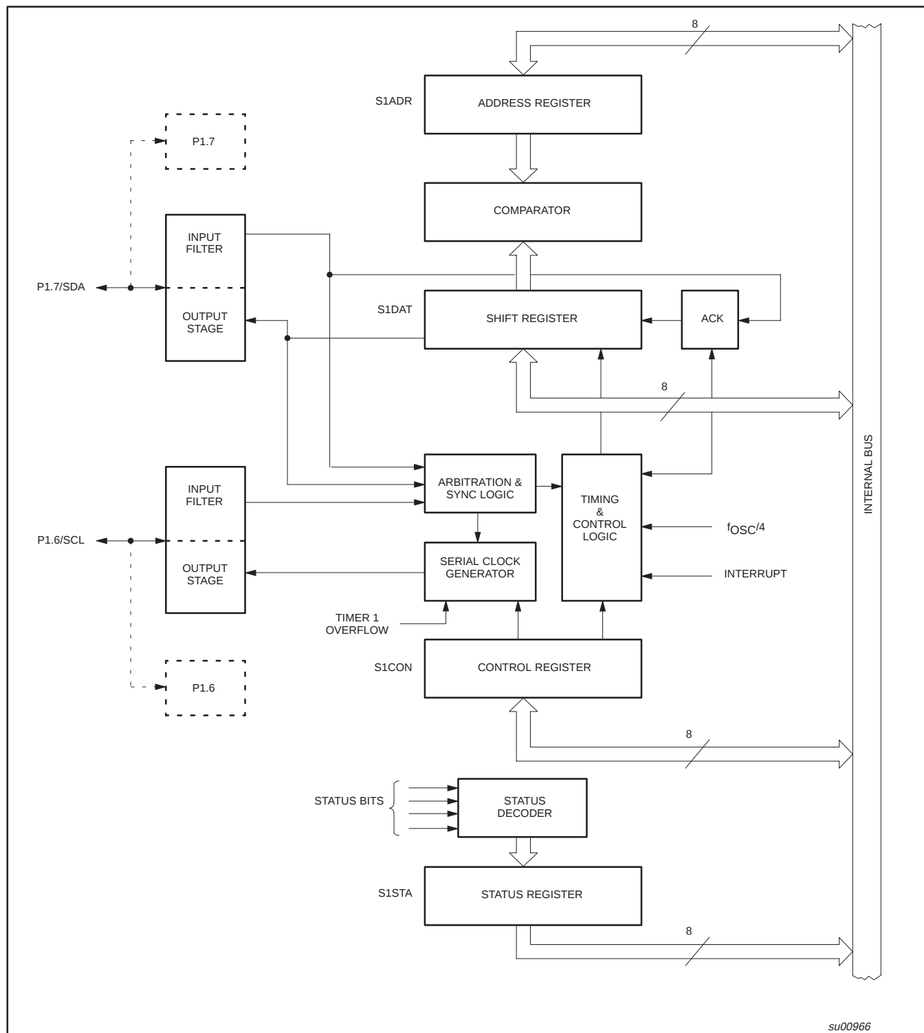
Figure 34. I²C Bus Serial Interface Block Diagram
