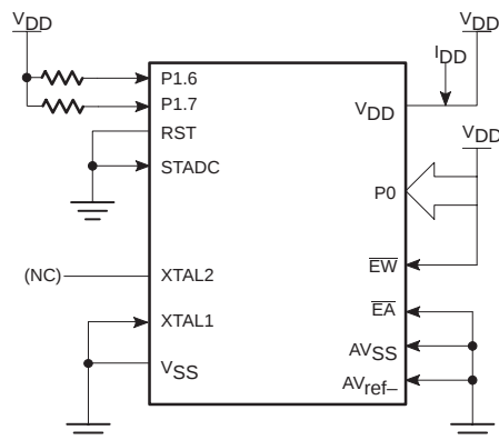
Figure 60. I DD Test Condition, Power Down Mode All other pins are disconnected. V DD = 2V to 5.5V 3
