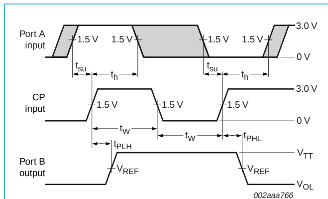
Fig 4. CP to B timing.
