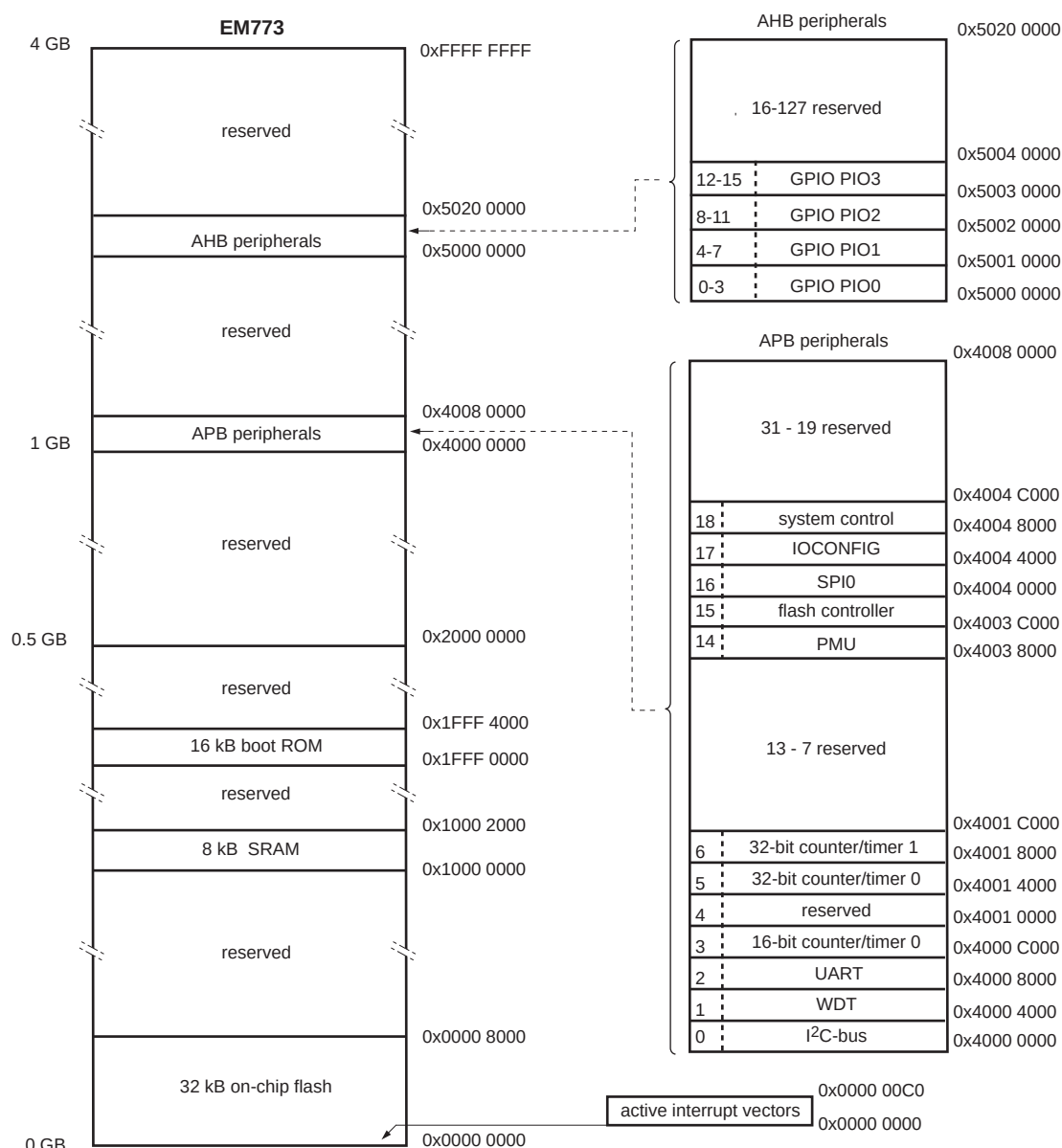
Fig 3. EM773 memory map
