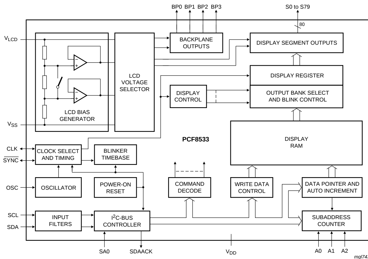
Fig 1. Block diagram of PCF8533
