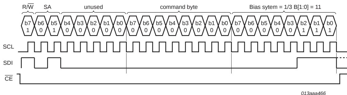
Fig 40. SPI-bus example
