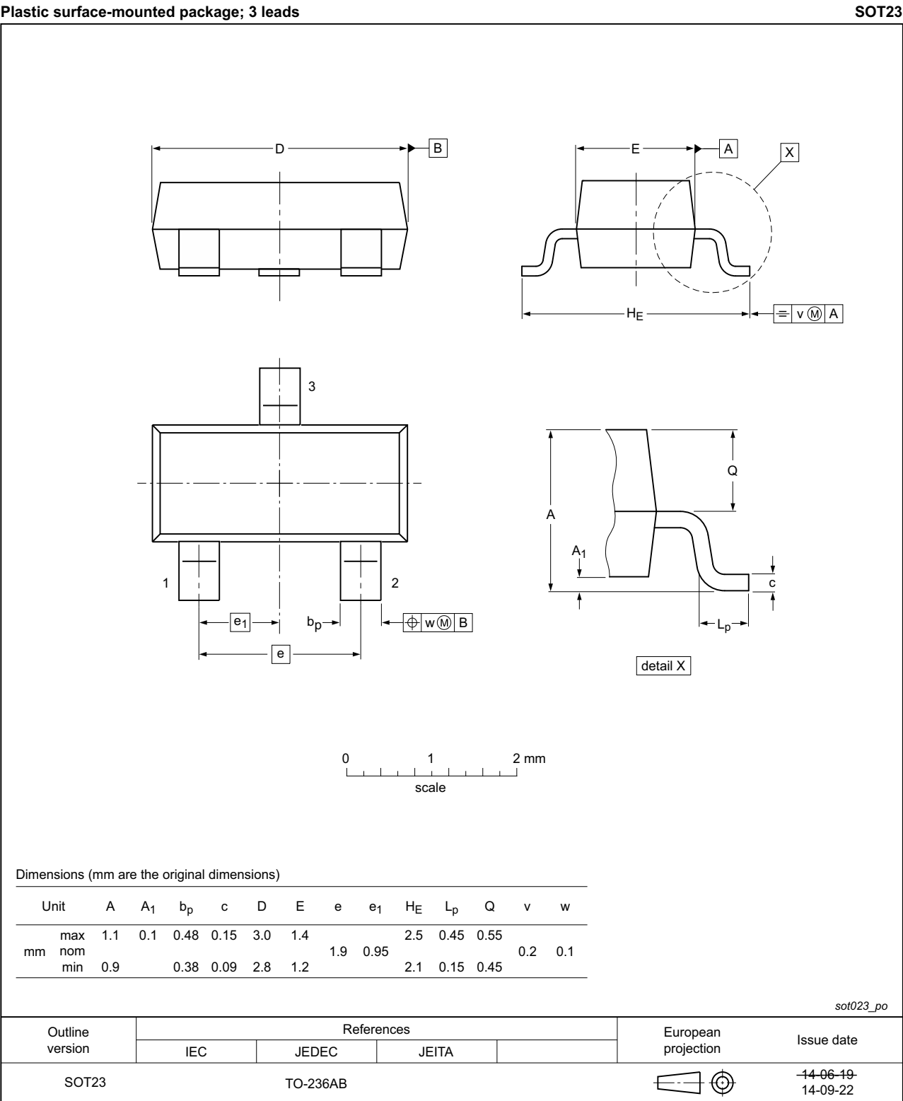
Fig 5. Package outline SOT23
