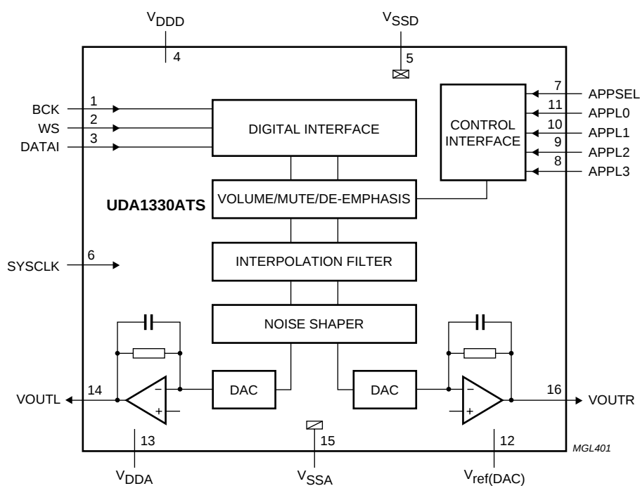
Fig.1 Block diagram.
