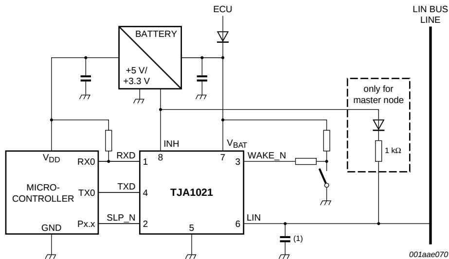
Fig 7. Typical application of the TJA1021
