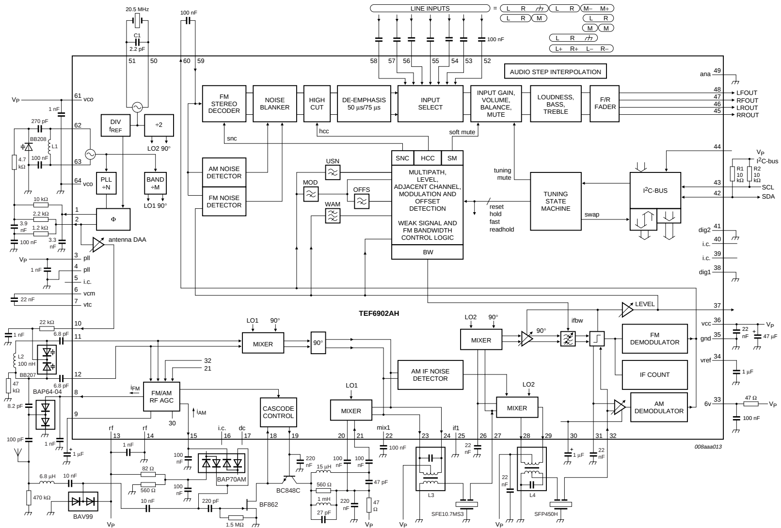
Fig 41. Application diagram of TEF6902AH
