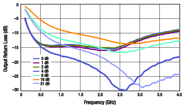
Figure 5. Output Return Loss vs Frequency
