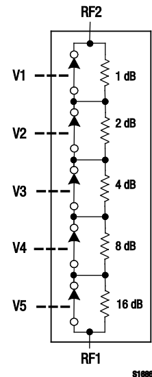
Figure 1. SKY12339-350LF Block Diagram
