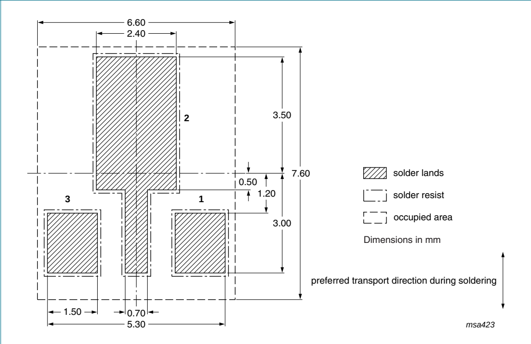
Not recommended for wave soldering Fig 17. Wave soldering footprint SOT89 (SC-62)
