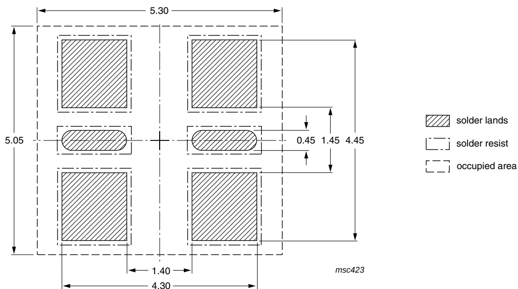
Fig 16. Reflow soldering footprint
