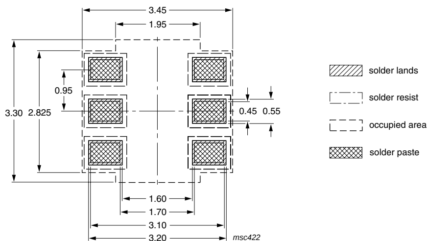
Fig 16. Reflow soldering footprint
