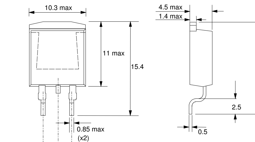
Fig.16. SOT404 : centre pin connected to mounting base.
