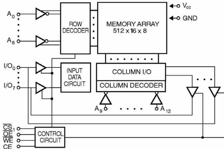
FIGURE 6 - Block diagram
