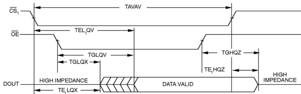
Figure 4c - Read Cycle 3
