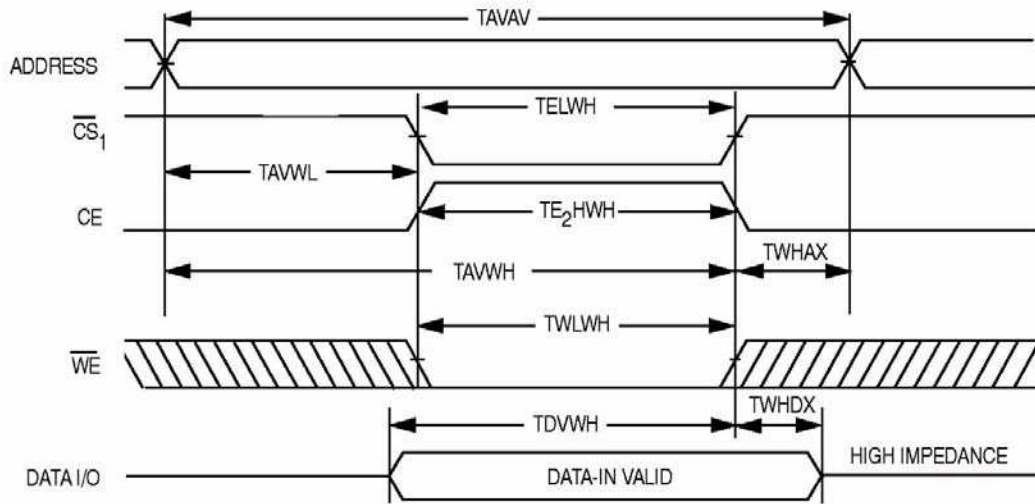
Figure 3c - Write Cycle 3 CS1 or CE controlled
