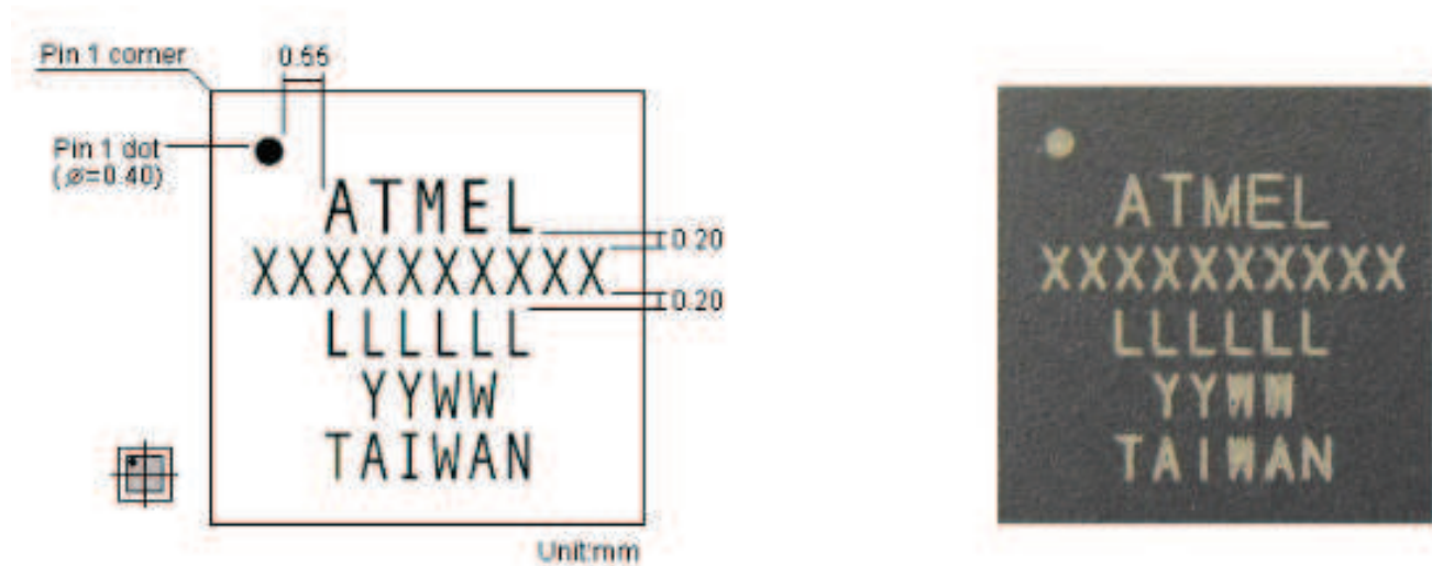
Figure 2. 40-pin TQFN Package Dimensions
