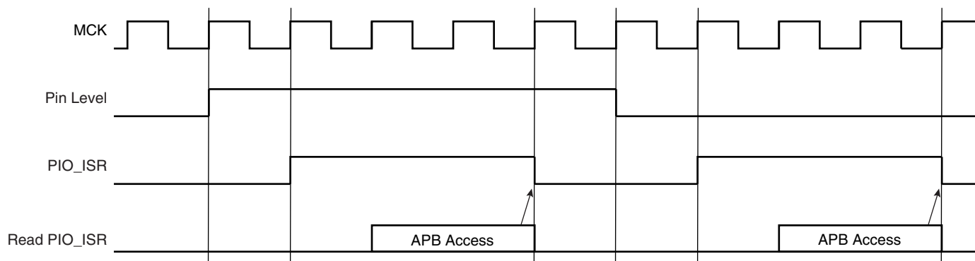
Figure 30-8. Input Change Interrupt Timings if there are no Additional Interrupt Modes
