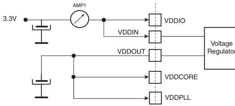
Figure 43-4. Measurement Setup
