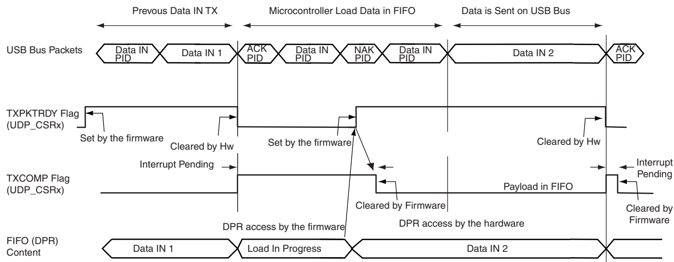
Figure 39-6. Data IN Transfer for Non Ping-pong Endpoint
