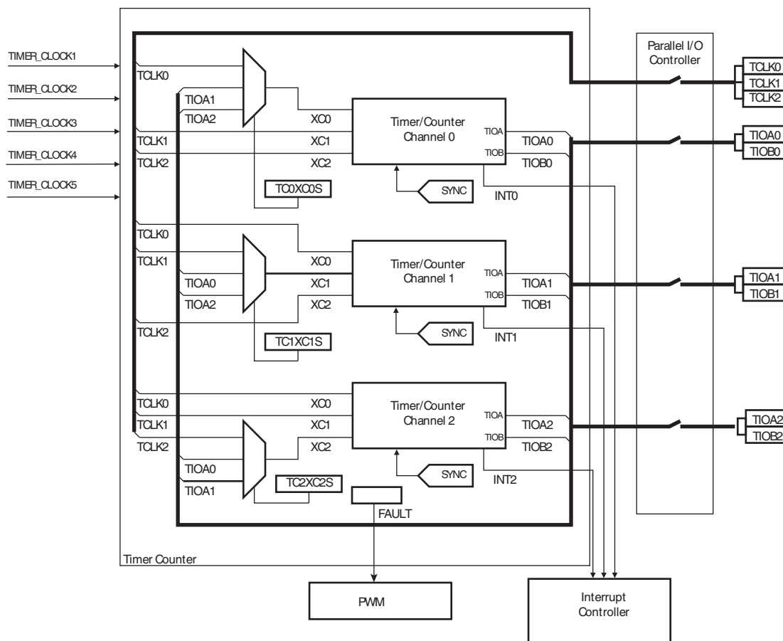
Figure 36-2. Timer Counter Block Diagram
