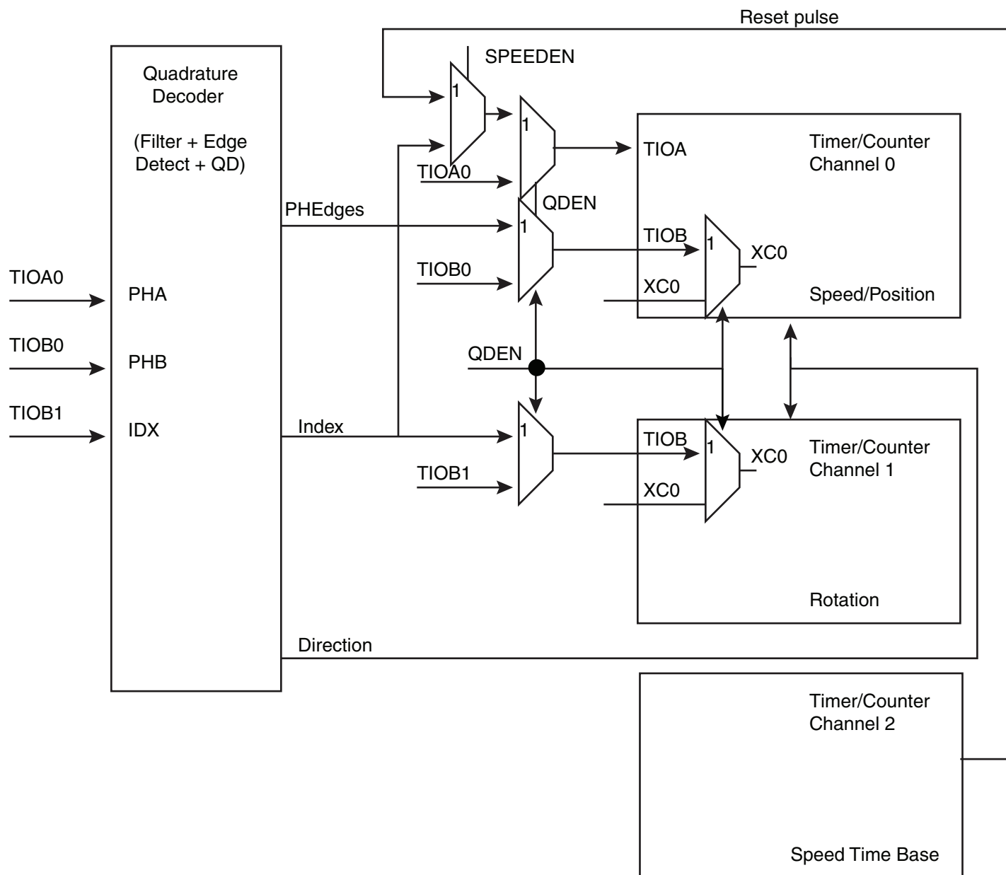
Figure 36-16. Predefined Connection of the Quadrature Decoder with Timer Counters
