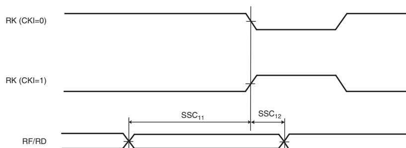
Figure 43-24. SSC Receiver, RK as output and RF as input
