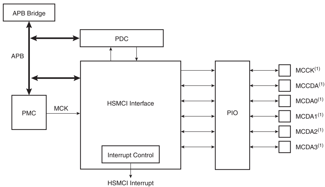
Figure 37-1. Block Diagram
