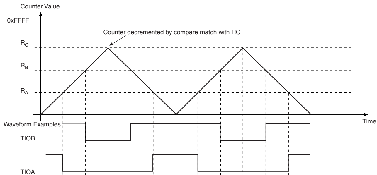
Figure 36-14. WAVSEL = 11 Without Trigger
