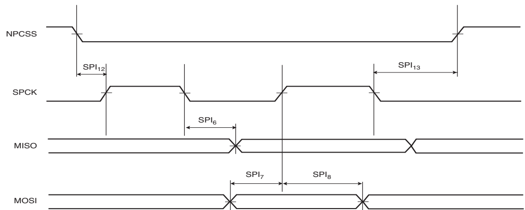
Figure 43-15. SPI Slave Mode with (CPOL=0 and NCPHA=1) or (CPOL=1 and NCPHA=0)
