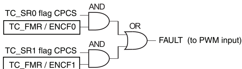
Figure 36-22. Fault Output Generation
