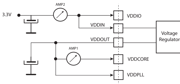
Figure 43-8. Active Mode Measurement Setup
