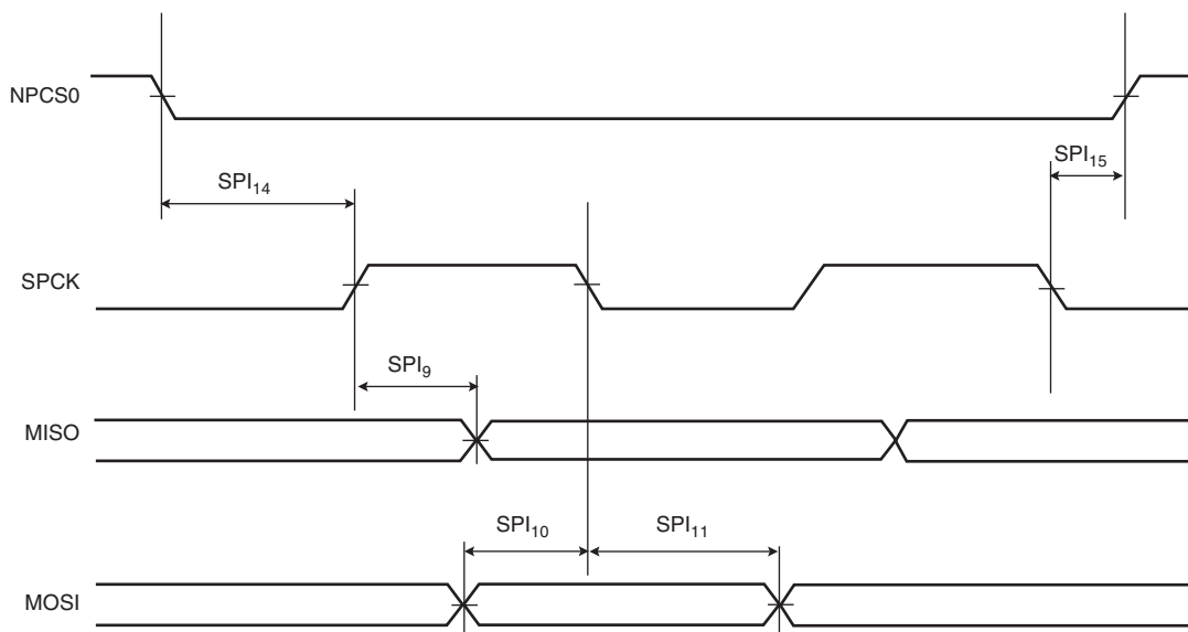
Figure 43-16. SPI Slave Mode with (CPOL = NCPHA = 0) or (CPOL= NCPHA= 1)
