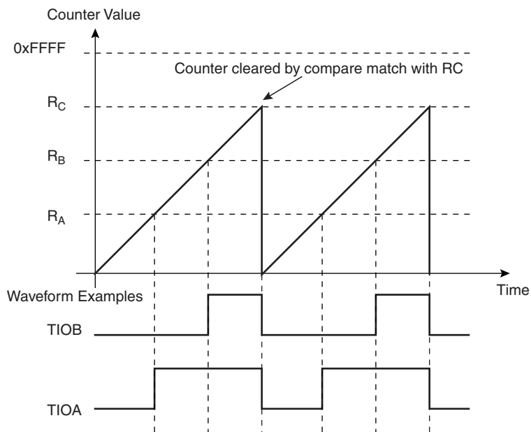
Figure 36-10. WAVSEL = 10 Without Trigger
