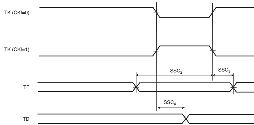
Figure 43-19. SSC Transmitter, TK as output and TF as input
