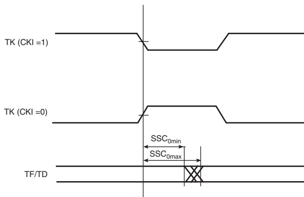
Figure 43-25. Min and Max Access Time of Output Signals
