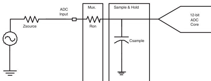
Figure 43-12. Simplified Acquisition Path
