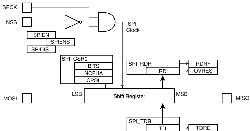
Figure 32-12. Slave Mode Functional Bloc Diagram
