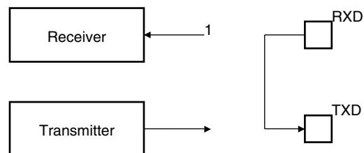
Figure 35-43. Remote Loopback Mode Configuration
