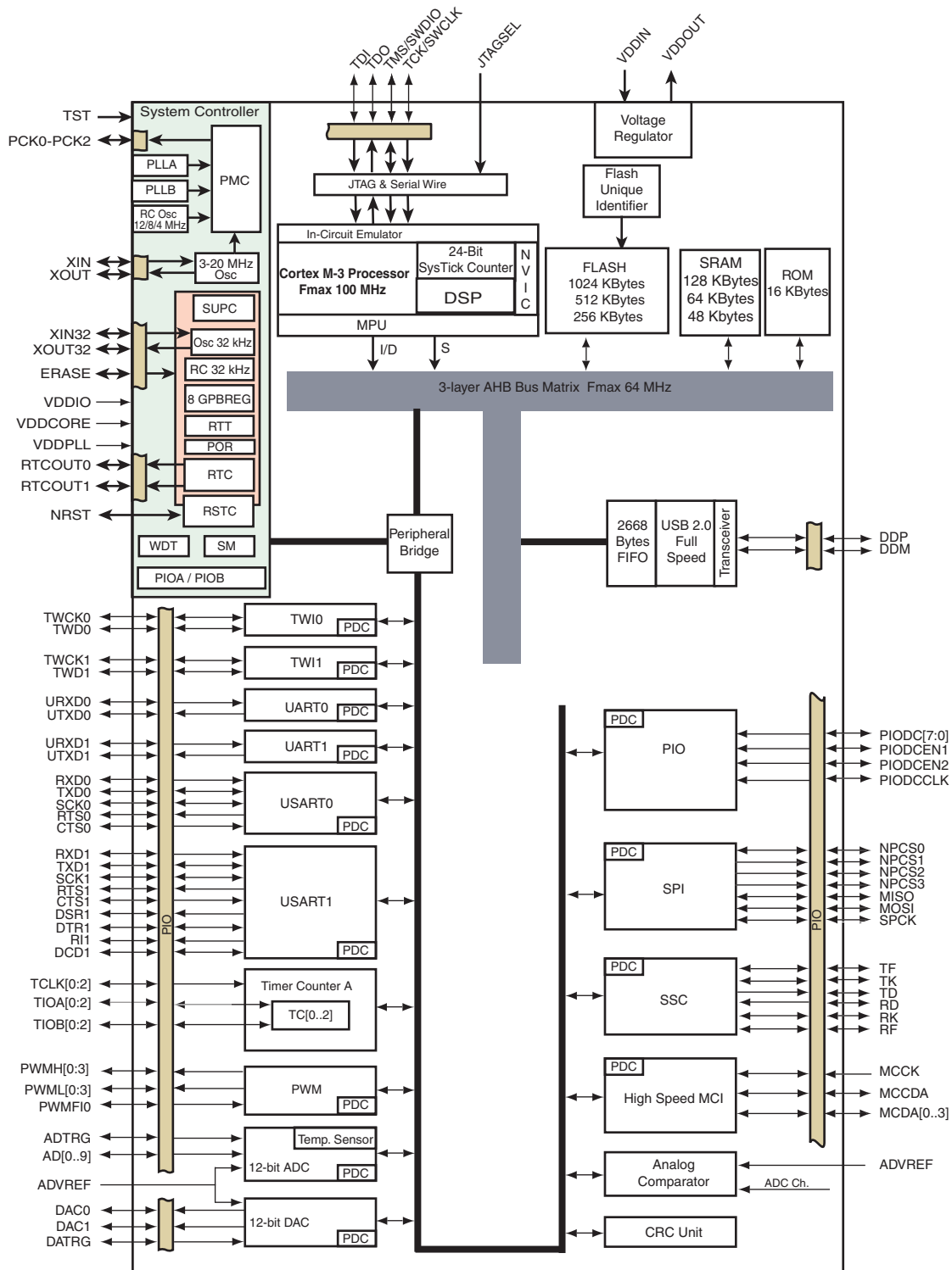
Figure 2-2. SAM3S16 64-pin Version Block Diagram
