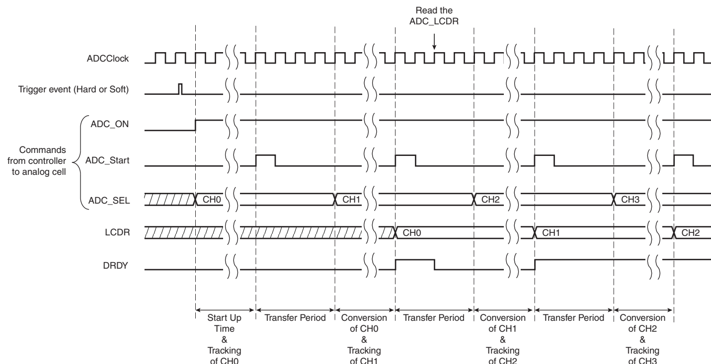
Figure 41-3. Sequence of ADC conversions when Tracking time < Conversion time
