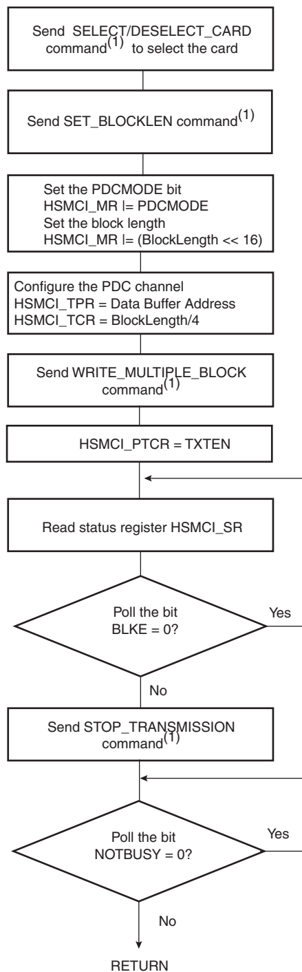
Figure 37-10. Multiple Write Functional Flow Diagram
