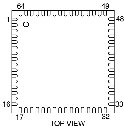
Figure 4-2. Orientation of the 64-pad QFN Package
