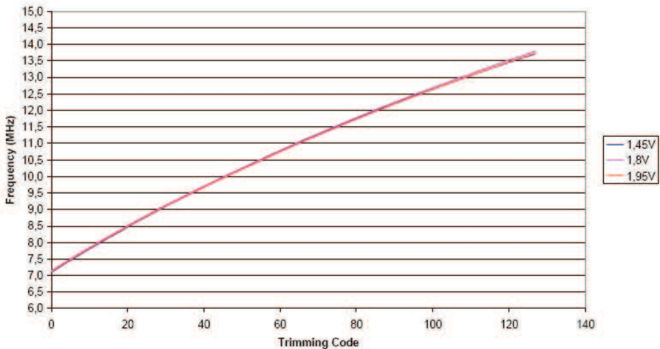
Figure 43-10. RC 12 MHz trimming
