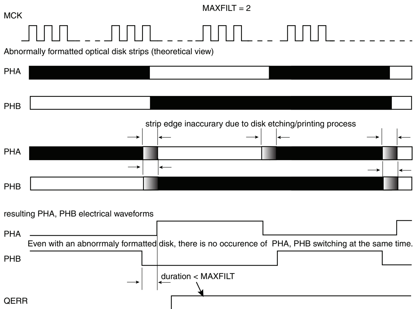
Figure 36-20. Quadrature Error Detection
