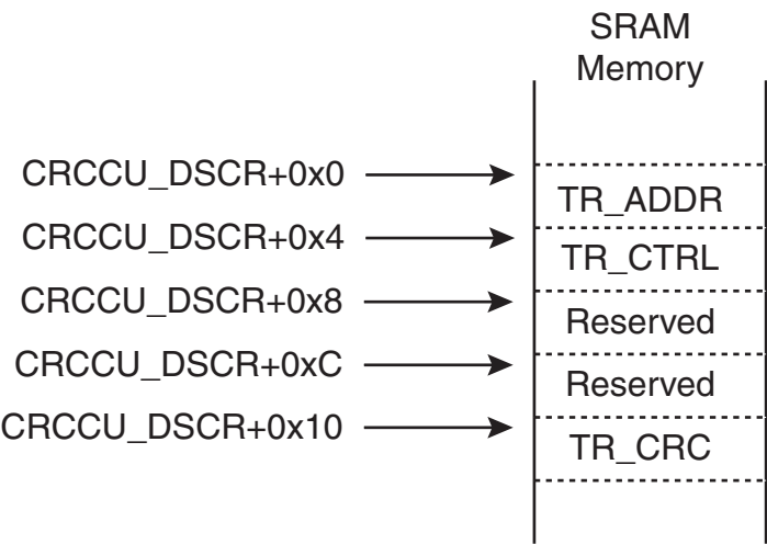
Figure 22-2. CRCCU Descriptor Memory Mapping
