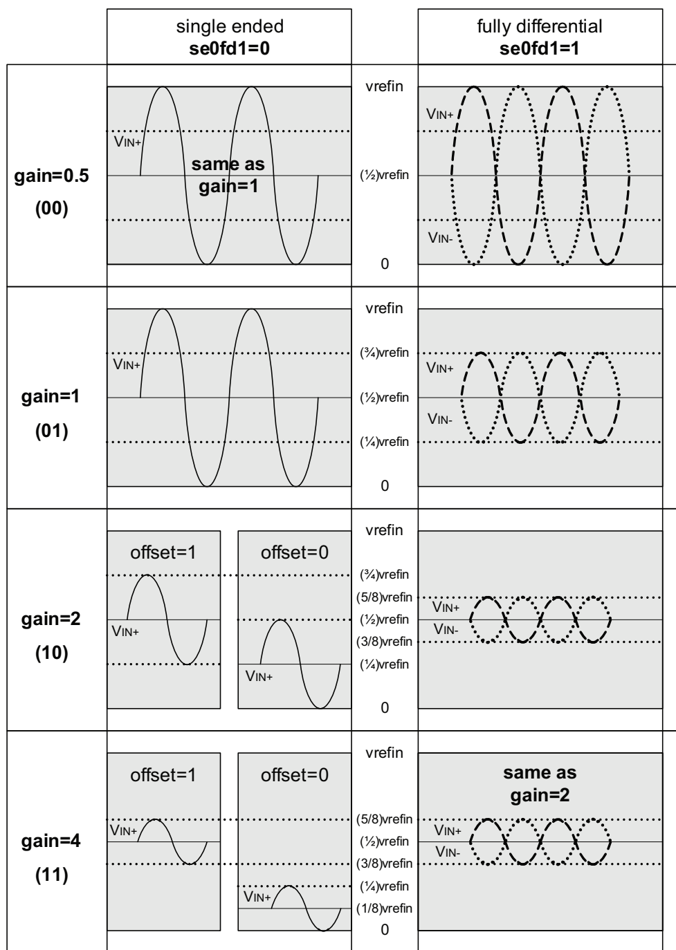
Figure 41-6. Analog Full Scale Ranges in Single Ended/Differential Applications Versus Gain and Offset
