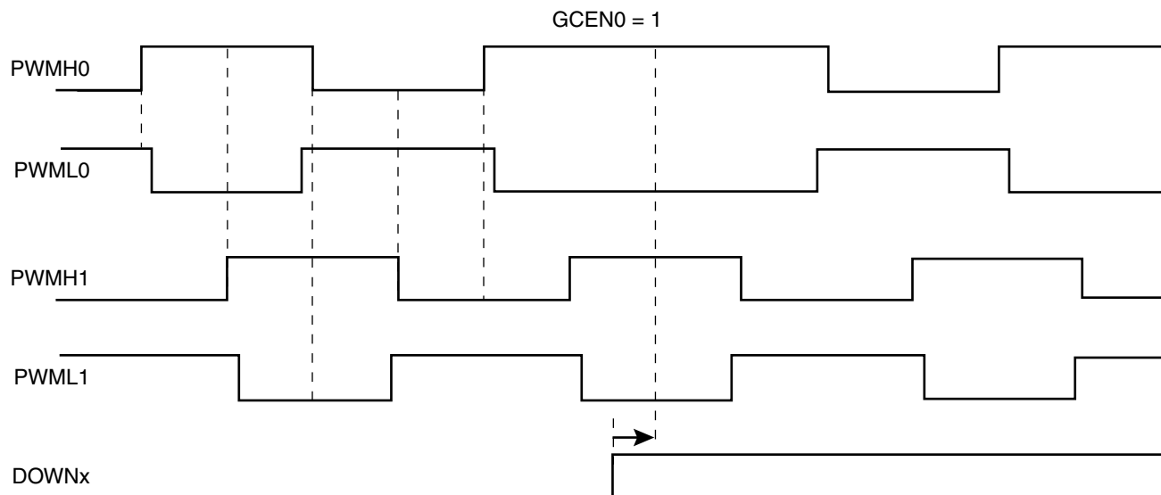
Figure 38-6. 2-bit Gray Up/Down Counter
