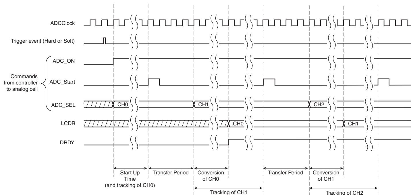
Figure 41-2. Sequence of ADC conversions when Tracking time > Conversion time
