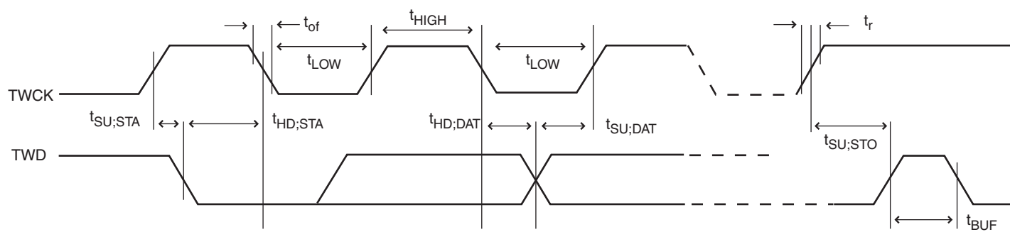
Figure 43-31. Two-wire Serial Bus Timing
