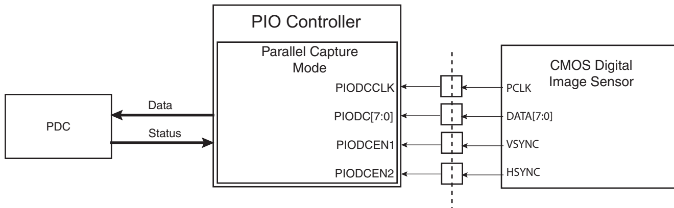
Figure 30-9. PIO controller connection with CMOS digital image sensor
