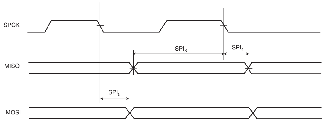
Figure 43-14. SPI Master Mode with (CPOL = 0 and NCPHA=1) or (CPOL=1 and NCPHA= 0)
