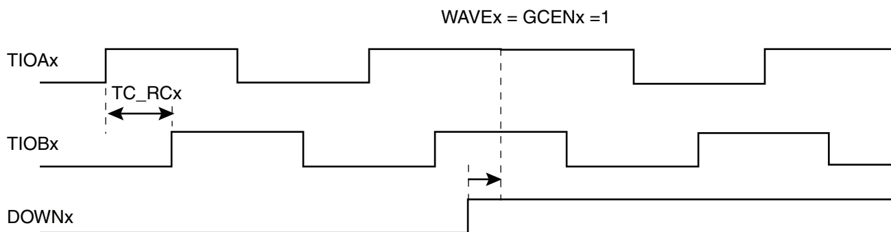
Figure 36-21. 2-bit Gray Up/Down Counter.
