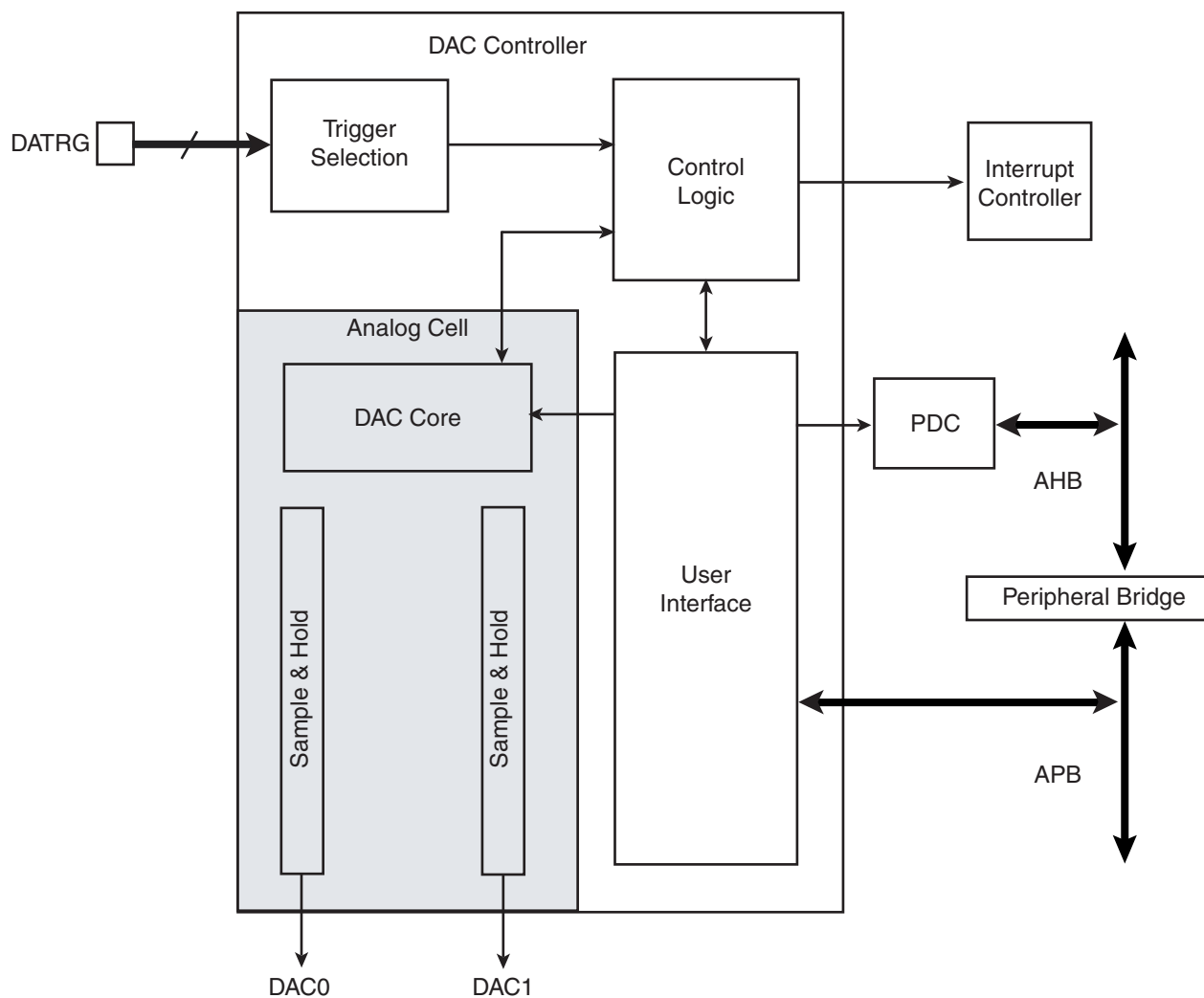
Figure 42-1. Digital-to-Analog Converter Controller Block Diagram
