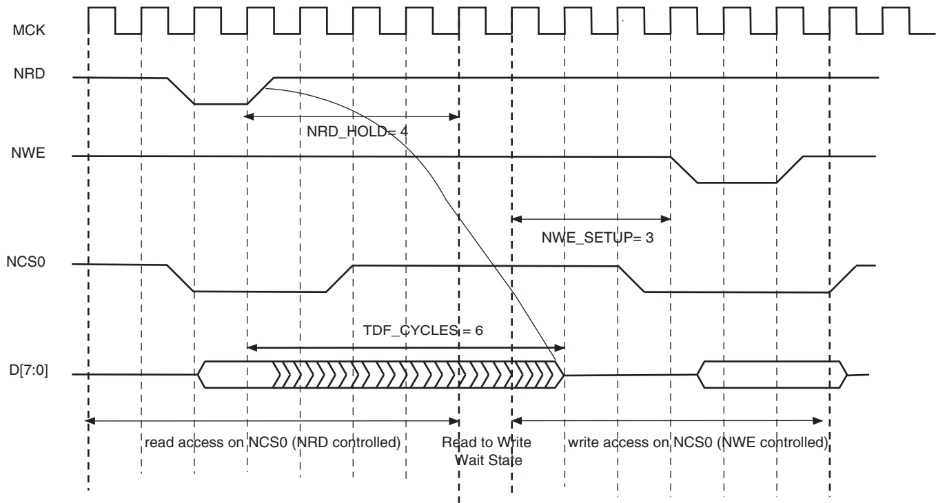
Figure 25-19. TDF Optimization: No TDF wait states are inserted if the TDF period is over when the next access begins
