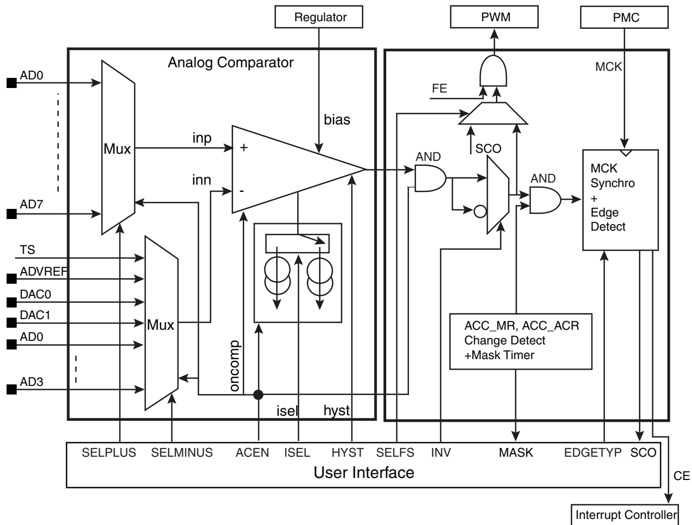
Figure 40-1. Analog Comparator Controller Block Diagram
