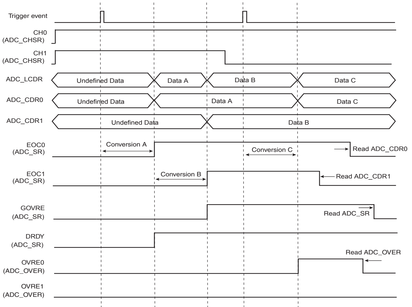
Figure 41-5. GOVRE and OVREx Flag Behavior
