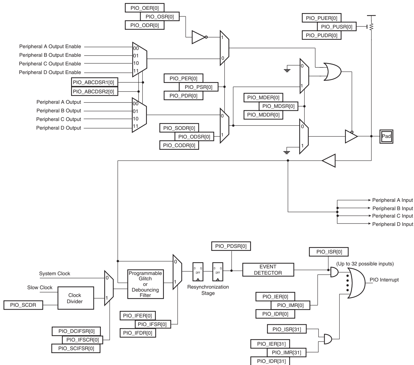
Figure 30-3. I/O Line Control Logic
