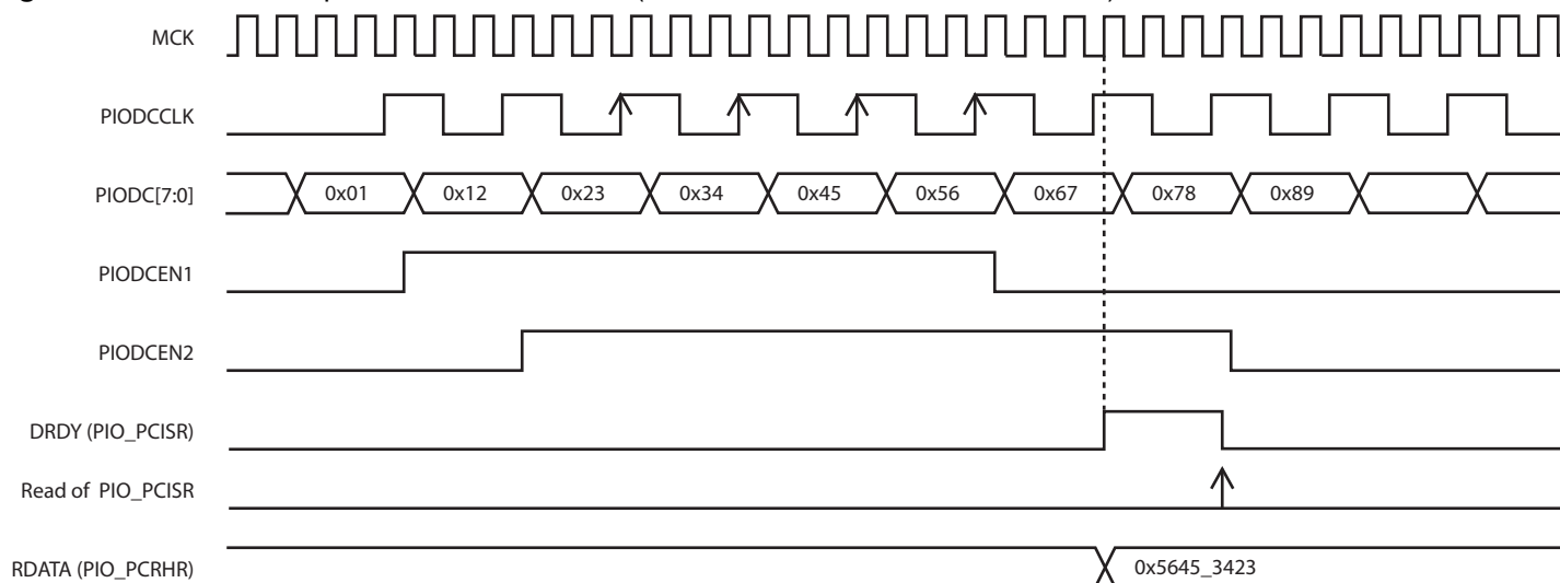
Figure 30-10. Parallel Capture Mode Waveforms (DSIZE = 2, ALWAYS = 0, HALFS = 0)
