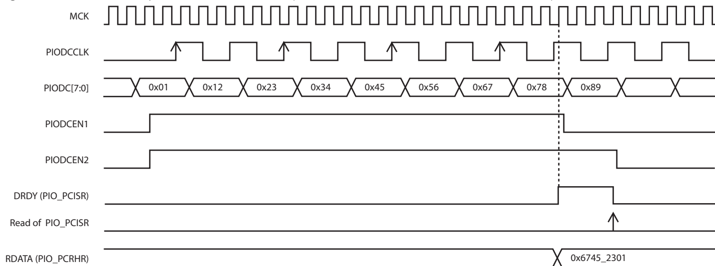
Figure 30-12. Parallel Capture Mode Waveforms (DSIZE=2, ALWAYS=0, HALFS=1, FRSTS=0)
