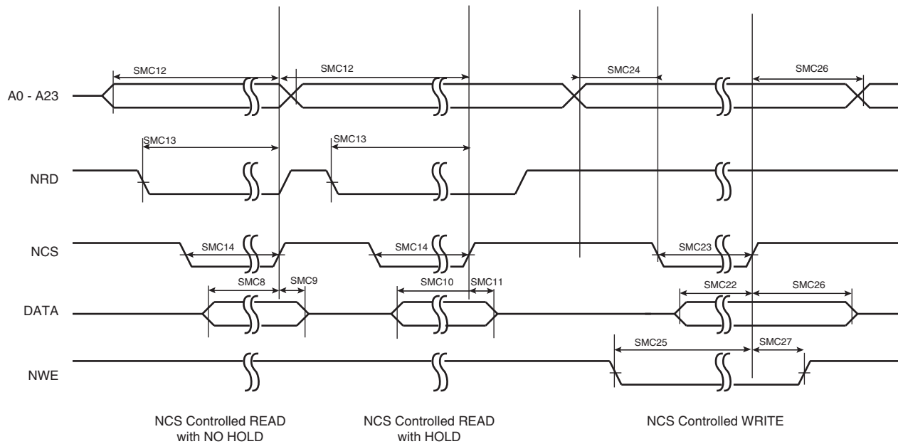
Figure 43-26. SMC Timings - NCS Controlled Read and Write
