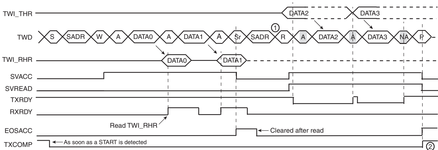
Figure 33-32. Repeated Start + Reversal from Write to Read Mode
