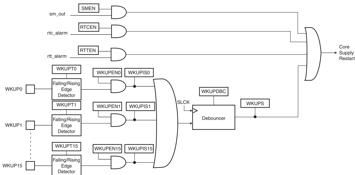
Figure 18-4. Wake Up Sources
