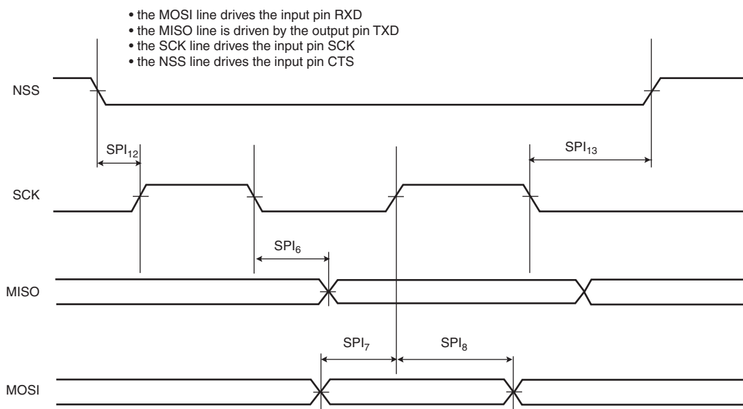
Figure 43-29. USART SPI Slave Mode: (Mode 1 or 2)
