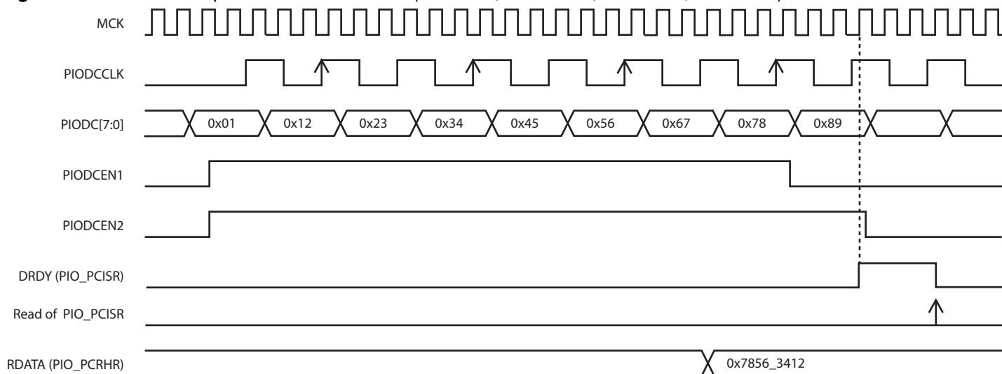
Figure 30-13. Parallel Capture Mode Waveforms (DSIZE=2, ALWAYS=0, HALFS=1, FRSTS=1)
