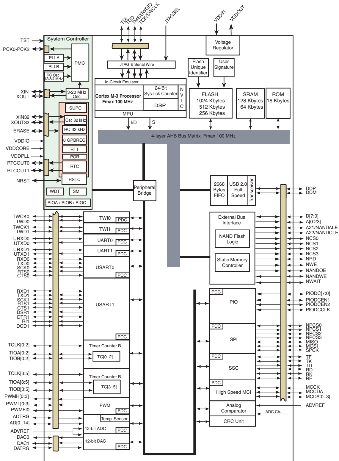
Figure 2-1. SAM3S16 100-pin Version Block Diagram
