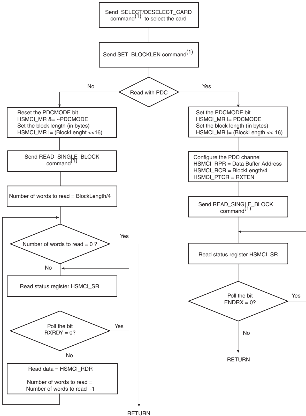
Figure 37-8. Read Functional Flow Diagram
