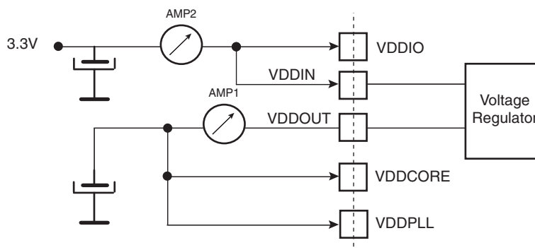
Figure 43-7. Measurement Setup for Wait Mode
