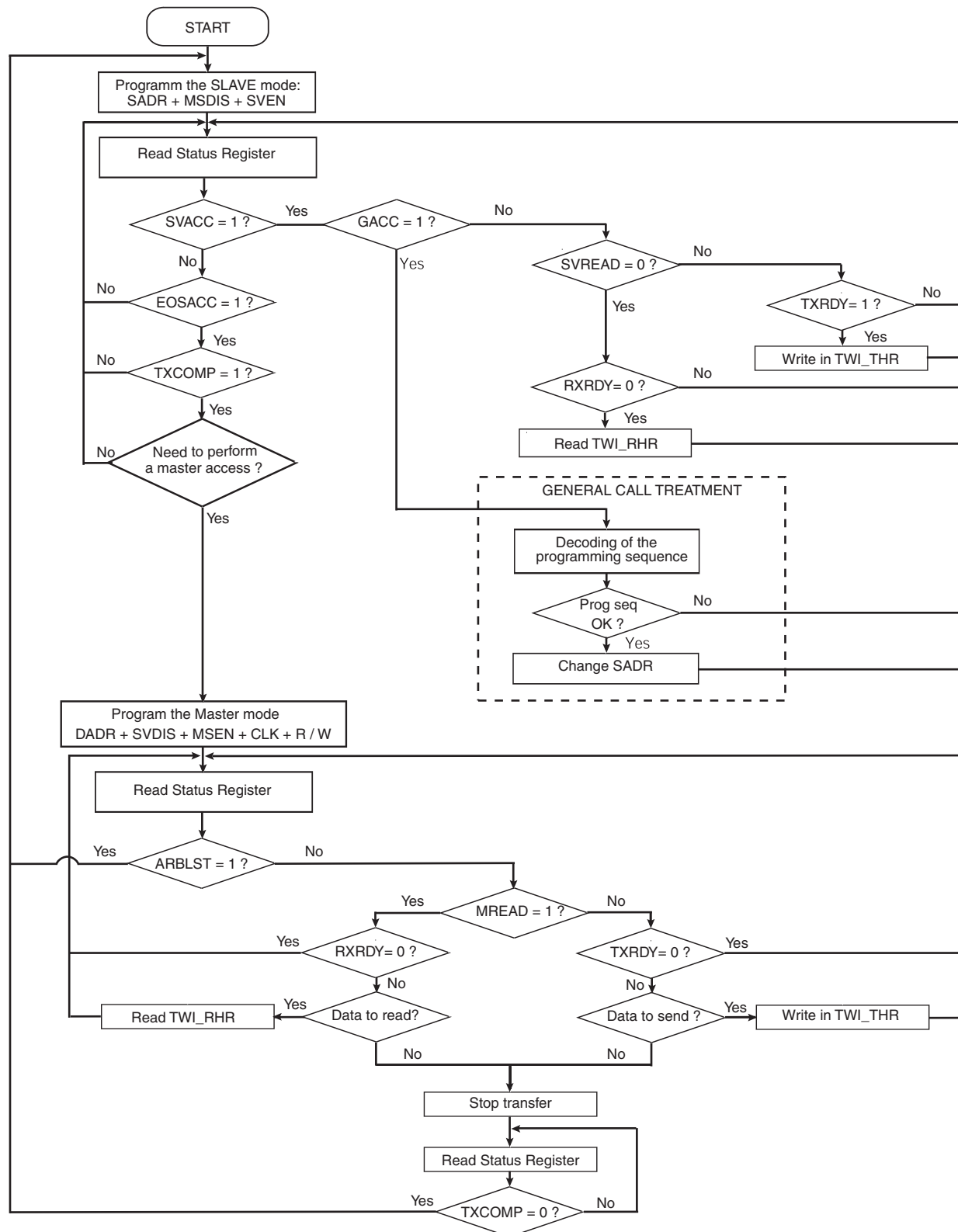
Figure 33-24. Multi-master Flowchart
