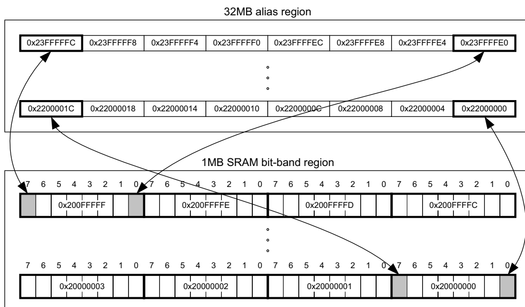
Figure 12-2. Bit-band mapping
