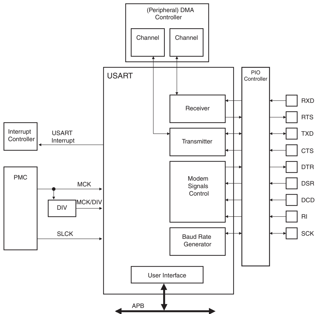
Figure 35-1. USART Block Diagram
