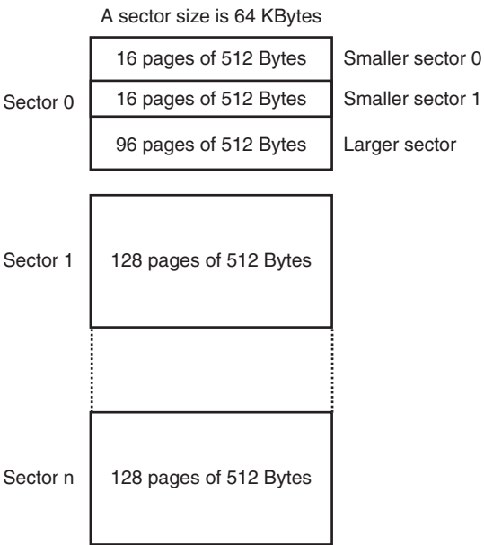
Figure 9-2. Flash Sector Organization
