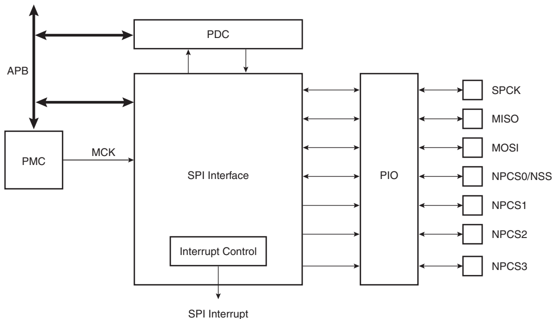
Figure 32-1. Block Diagram
