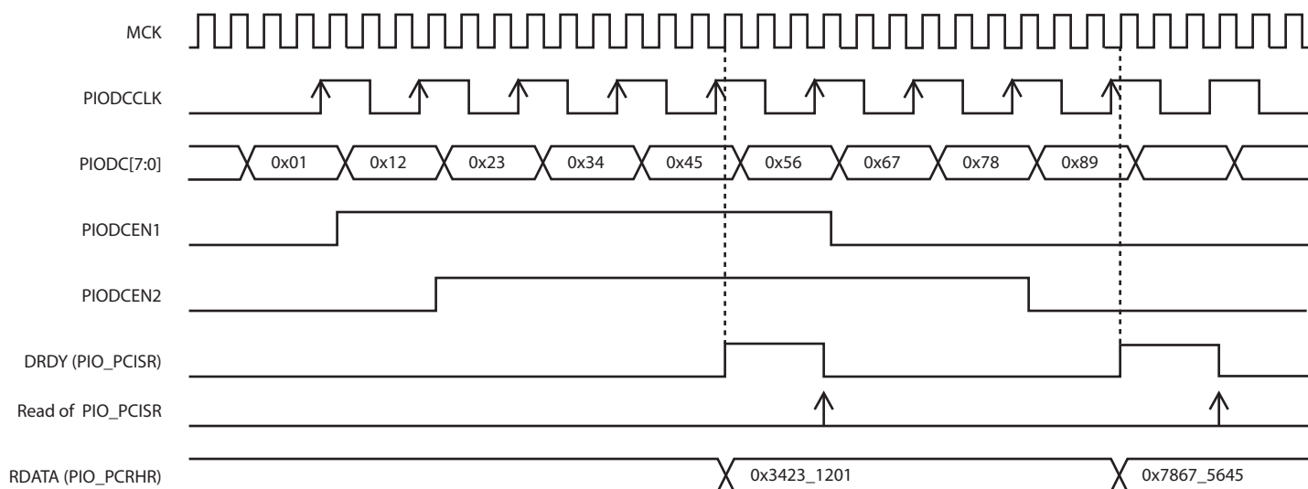
Figure 30-11. Parallel Capture Mode Waveforms (DSIZE=2, ALWAYS=1, HALFS=0)
