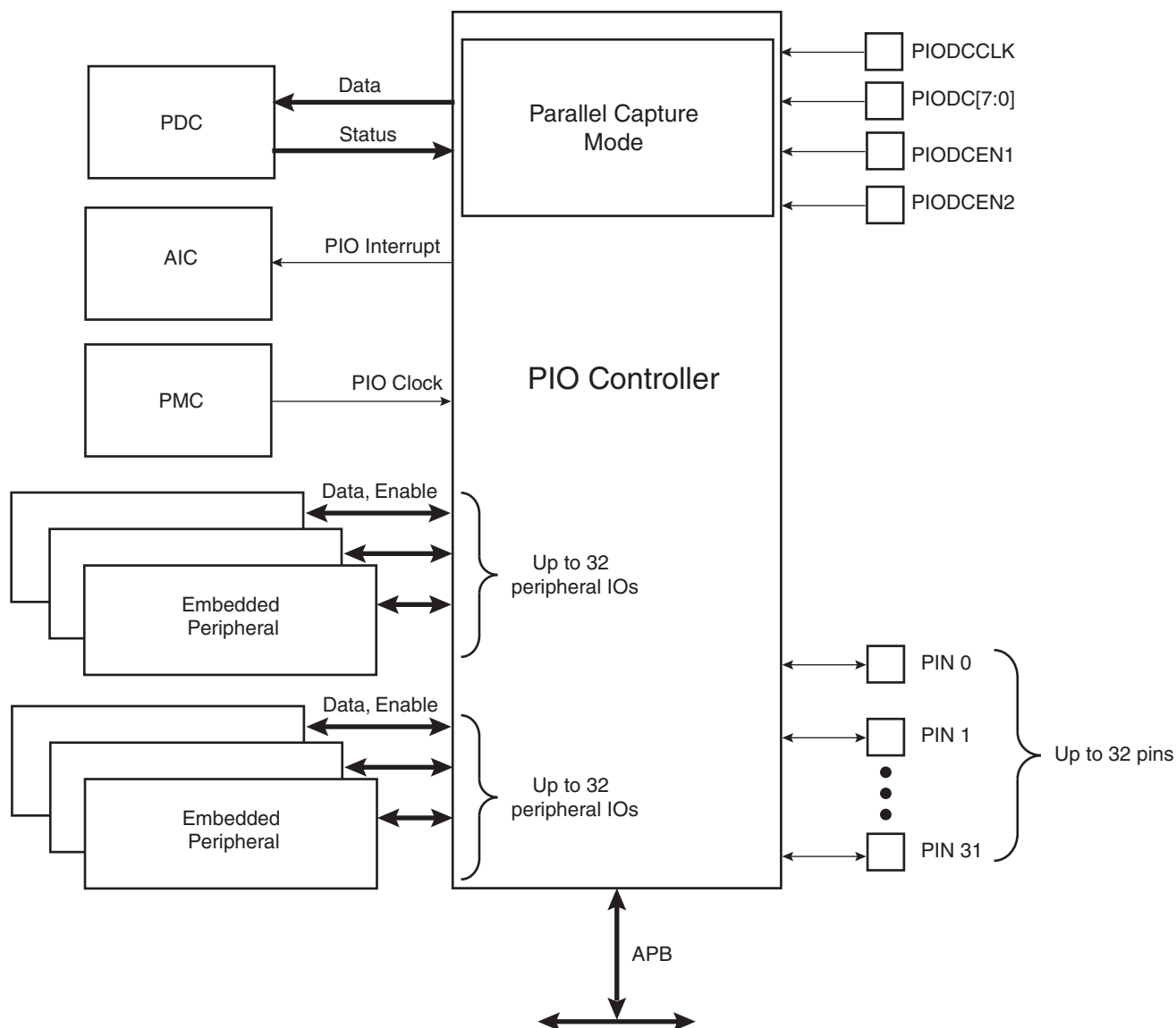
Figure 30-1. Block Diagram
