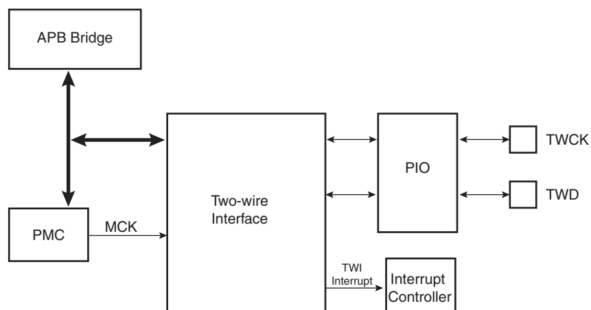
Figure 33-1. Block Diagram
