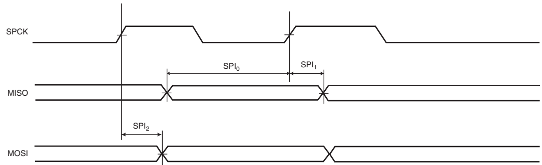
Figure 43-13. SPI Master Mode with (CPOL= NCPHA = 0) or (CPOL= NCPHA= 1)
