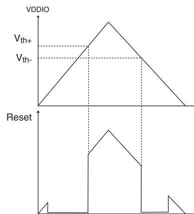
Figure 43-3. Zero-Power-on Reset Characteristics
