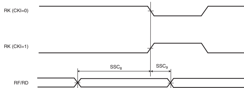
Figure 43-21. SSC Receiver RK and RF as input
