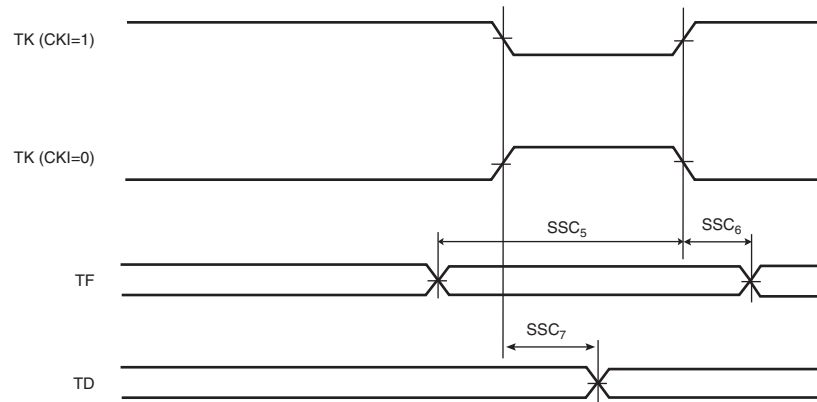
Figure 43-20. SSC Transmitter, TK and TF as input
