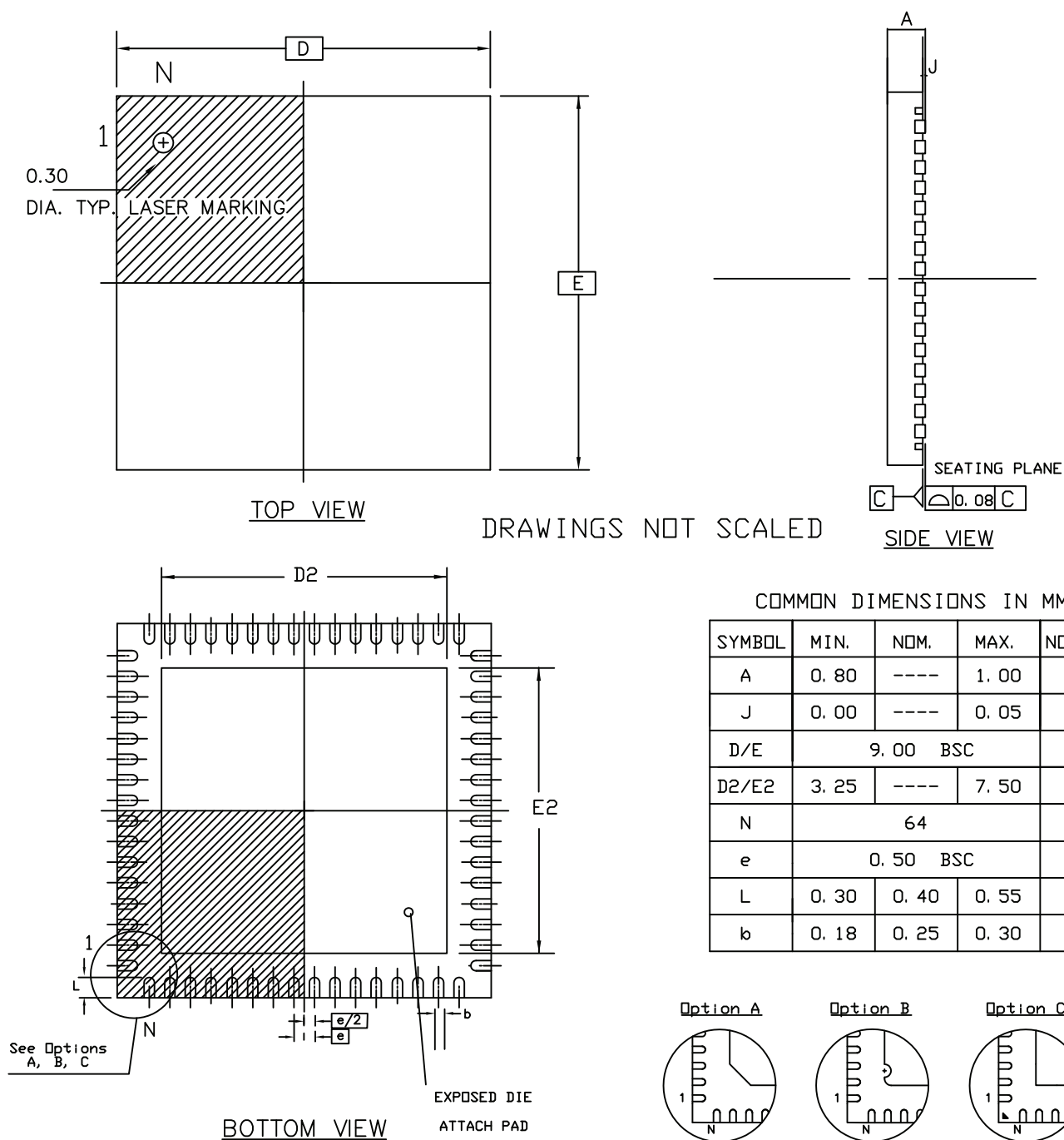
Figure 44-2. 64-pad QFN Package Drawing
