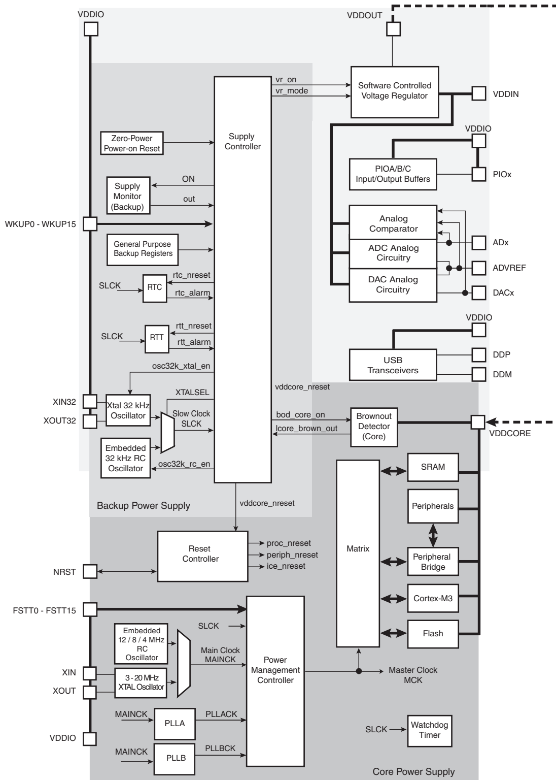
Figure 18-1. Supply Controller Block Diagram
