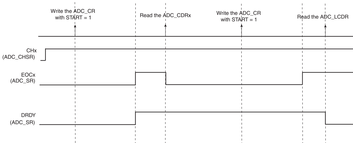
Figure 41-4. EOCx and DRDY Flag Behavior
