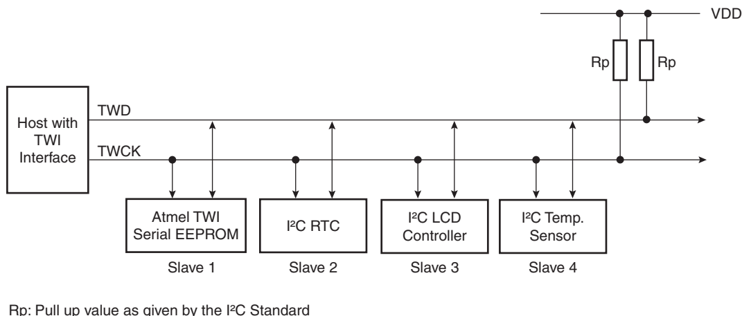
Figure 33-2. Application Block Diagram
