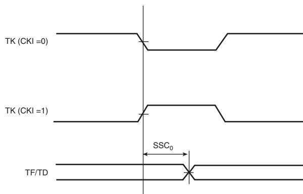
Figure 43-17. SSC Transmitter, TK and TF as output
