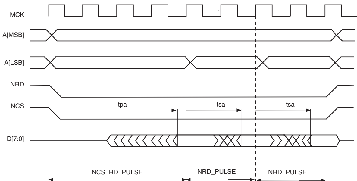
Figure 25-31. Page Mode Read Protocol (Address MSB and LSB are defined in Table 25-5 )
