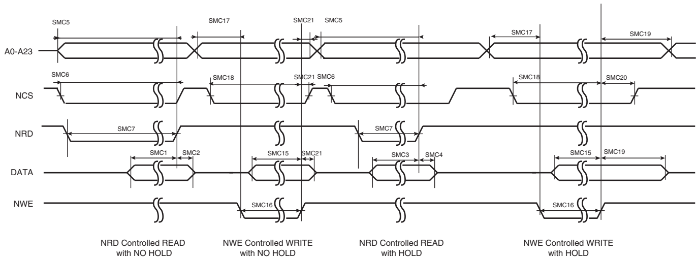
Figure 43-27. SMC Timings - NRD Controlled Read and NWE Controlled Write
