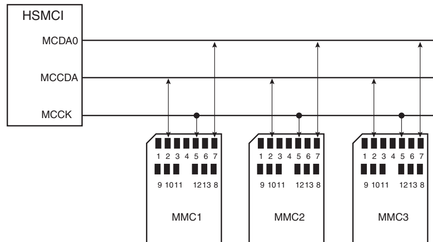
Figure 37-4. MMC Bus Connections (One Slot)
