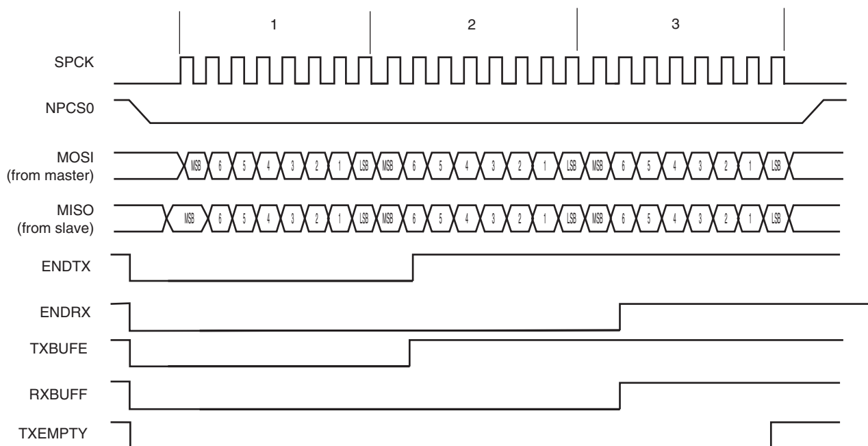
Figure 32-8. PDC Status Register Flags Behavior
