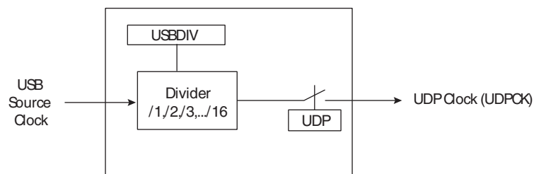
Figure 28-3. USB Clock Controller
