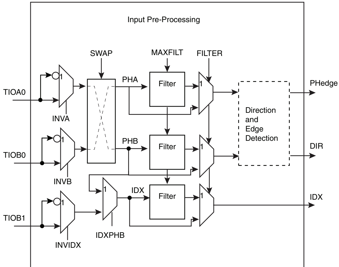
Figure 36-17. Input Stage
