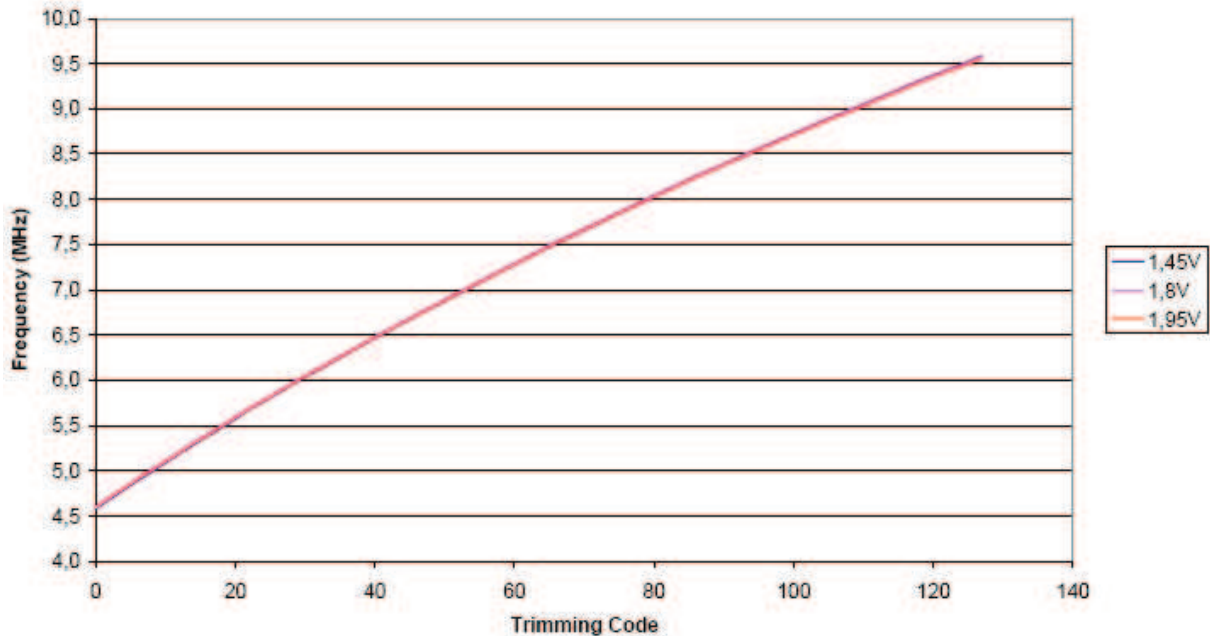
Figure 43-9. RC 8 MHz trimming
