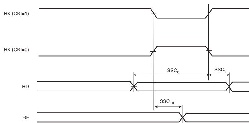
Figure 43-22. SSC Receiver, RK as input and RF as output
