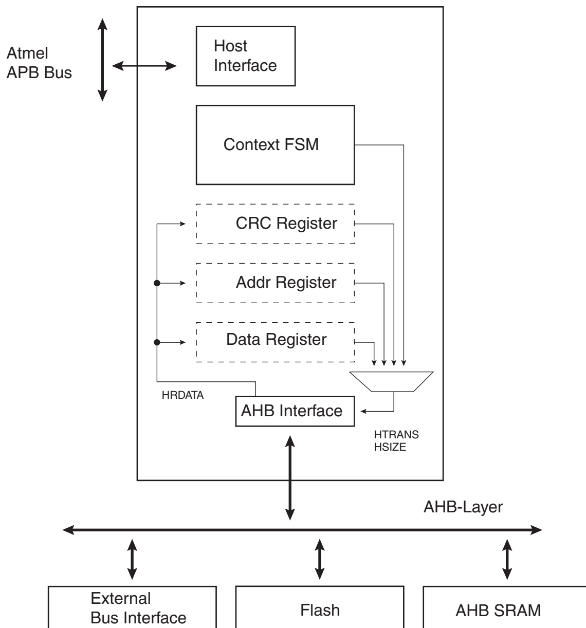
Figure 22-1. Block Diagram
