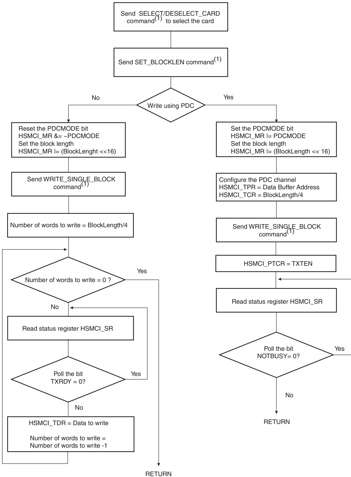
Figure 37-9. Write Functional Flow Diagram
