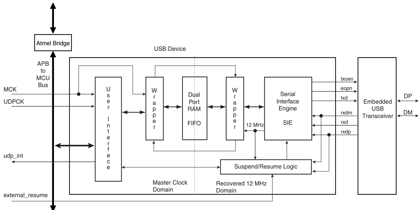
Figure 39-1. Block Diagram
