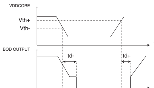
Figure 43-1. Core Brownout Output Waveform
