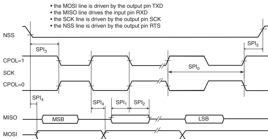
Figure 43-28. USART SPI Master Mode
