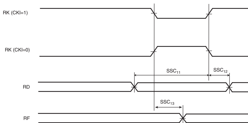
Figure 43-23. SSC Receiver, RK and RF as output
