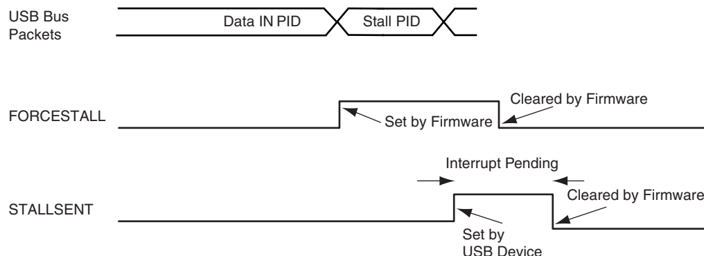
Figure 39-12. Stall Handshake (Data IN Transfer)
