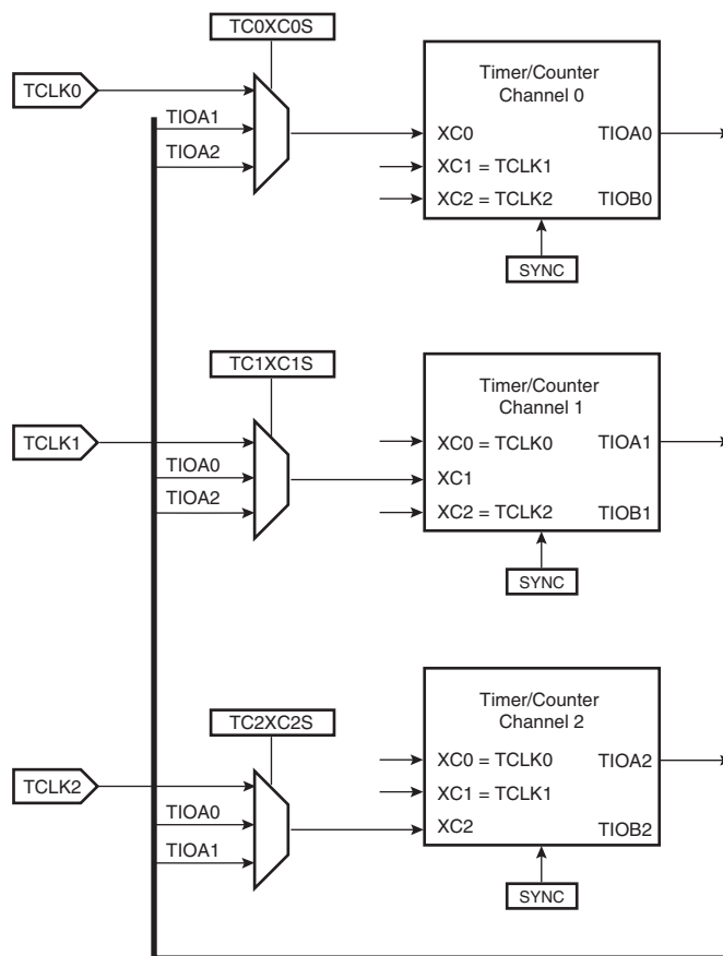
Figure 36-3. Clock Chaining Selection
