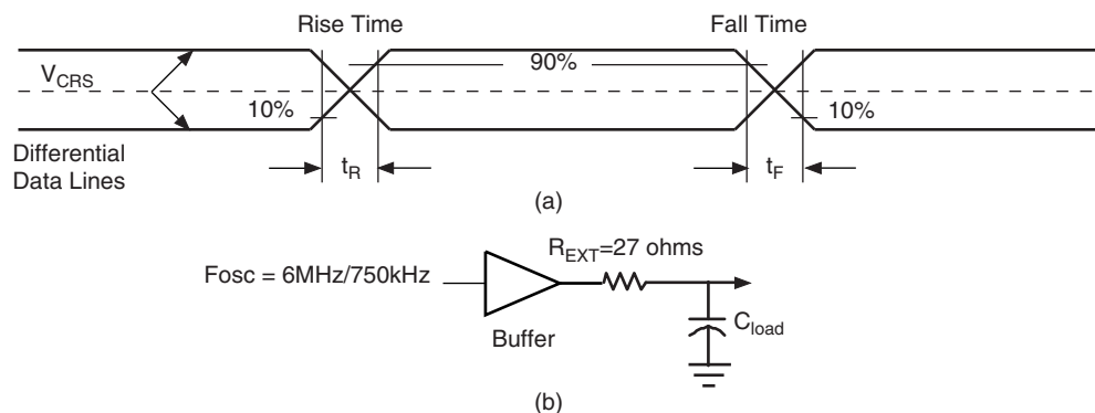
Figure 43-11. USB Data Signal Rise and Fall Times
