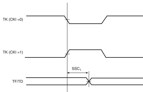
Figure 43-18. SSC Transmitter, TK as input and TF as output
