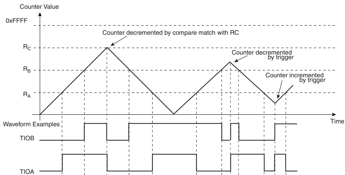
Figure 36-15. WAVSEL = 11 With Trigger
