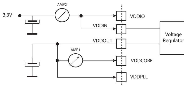
Figure 43-5. Measurement Setup for Sleep Mode
