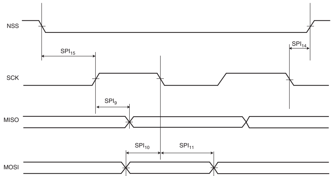
Figure 43-30. USART SPI Slave mode: (Mode 0 or 3)
