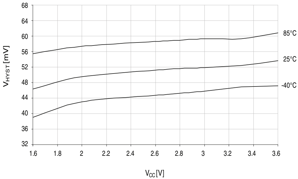
Figure 34-50. Analog comparator hysteresis vs. V_{CC} .
