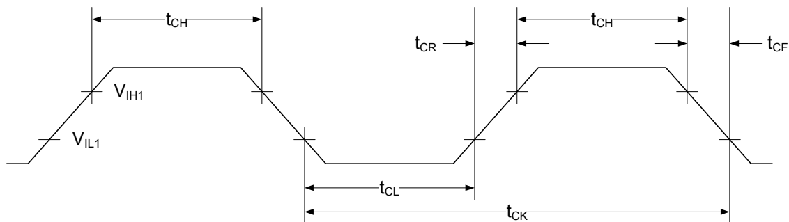
Figure 33-3. External clock drive waveform .
