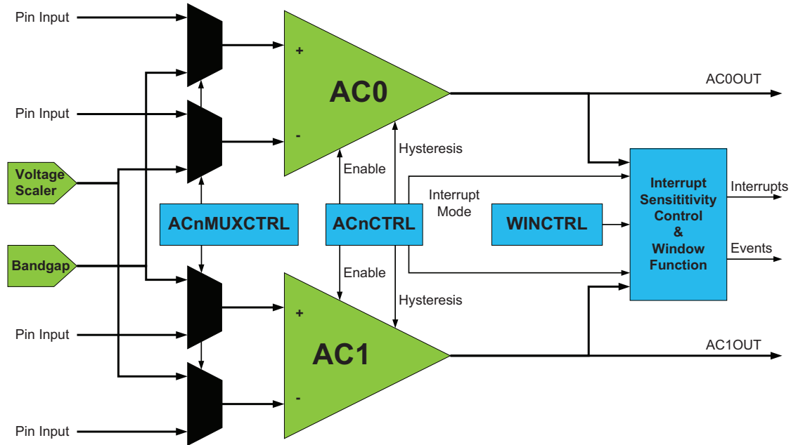
Figure 27-1. Analog comparator overview.
