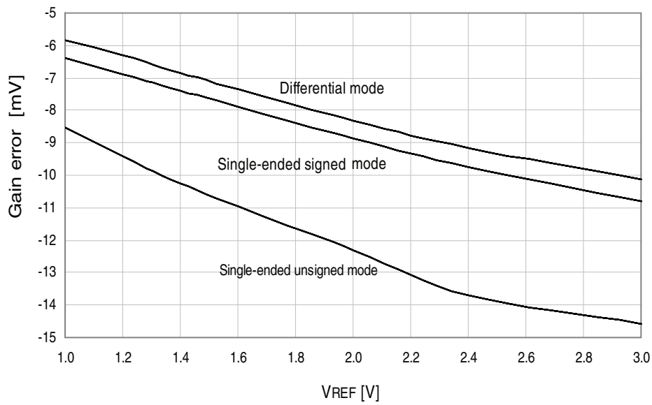
Figure 34-104. Gain error vs. V_{REF} .
