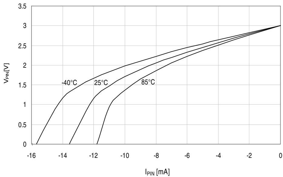
Figure 34-157. I/O pin output voltage vs. source current.
