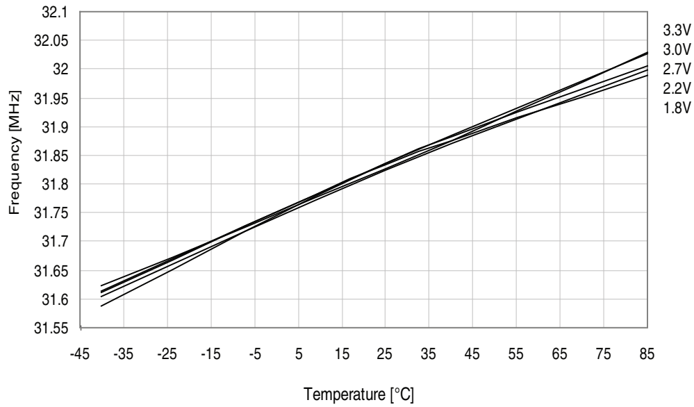
Figure 34-128.32MHz internal oscillator frequency vs. temperature. DPLL enabled, from the 32.768kHz internal oscillator.
