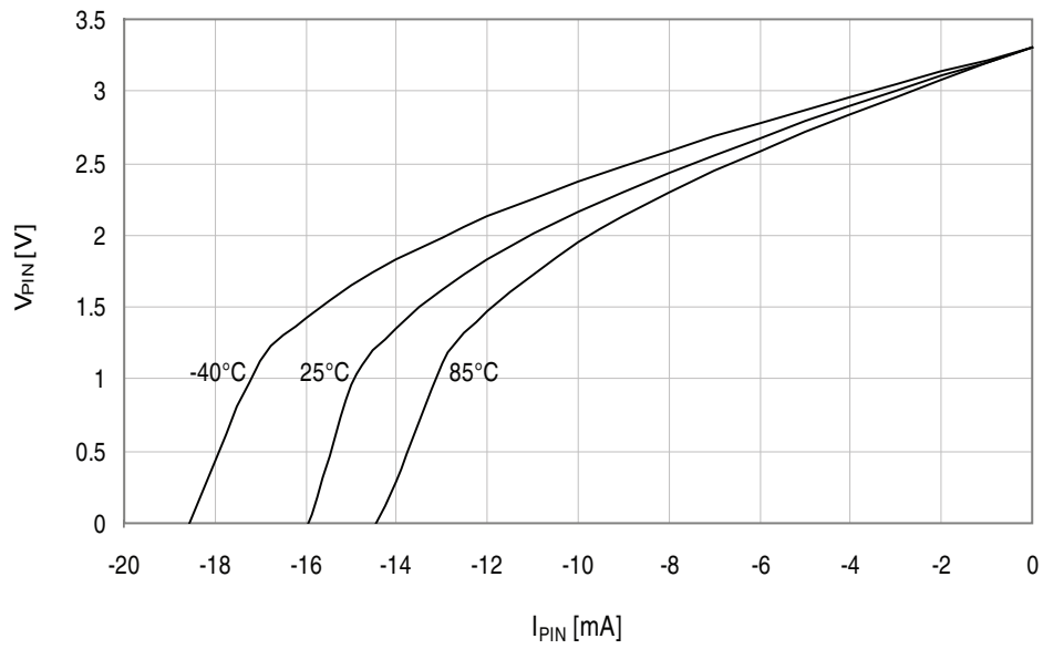
Figure 34-92. I/O pin output voltage vs. sink current.
