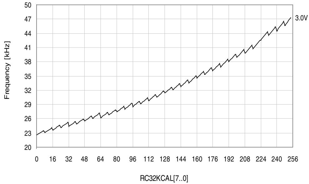
Figure 34-257. 32.768kHz internal oscillator frequency vs. calibration value.
