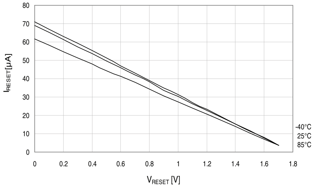
Figure 34-252. Reset pin pull-up resistor current vs. reset pin voltage.
