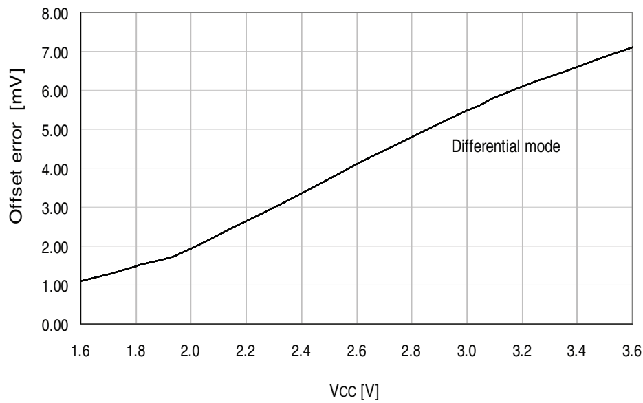
Figure 34-175. Offset error vs. V_{CC} .
