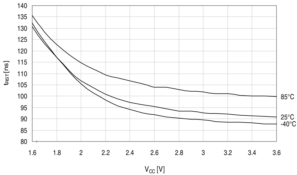
Figure 34-250. Minimum Reset pin pulse width vs. V CC .
