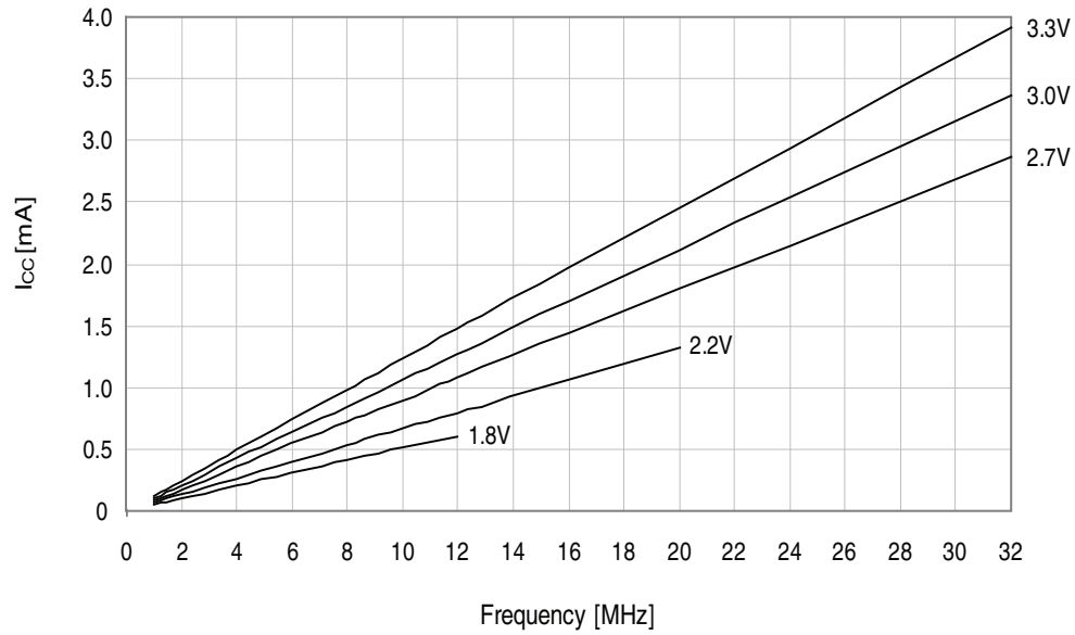
Figure 34-145. Idle mode supply current vs. V_{CC} .
