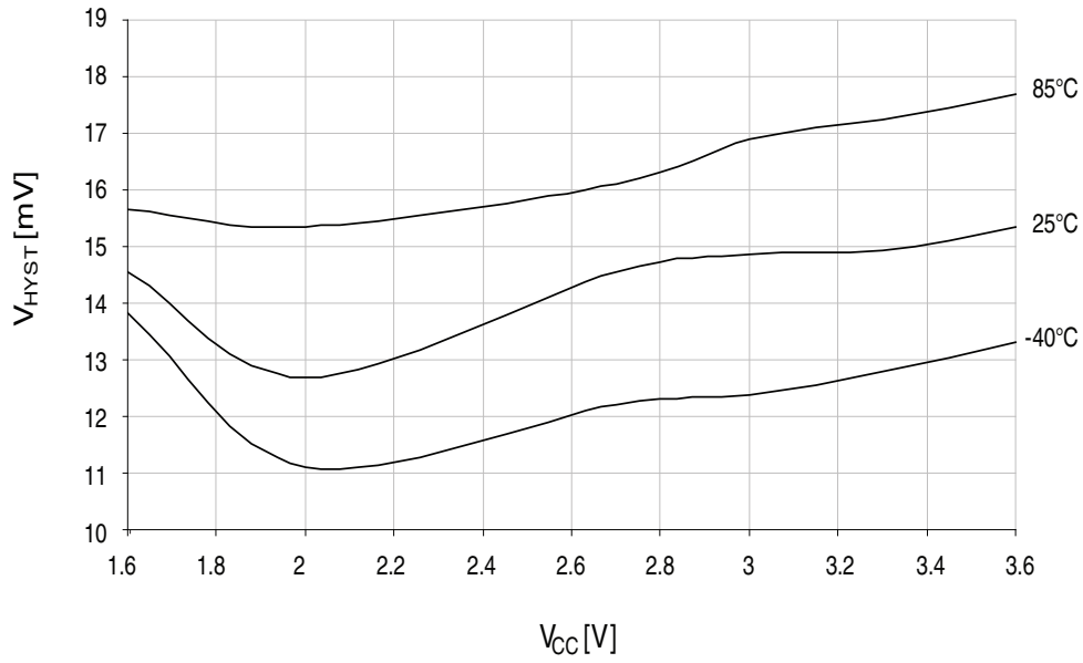
Figure 34-244. Analog comparator hysteresis vs. V_{CC} . Large hysteresis.
