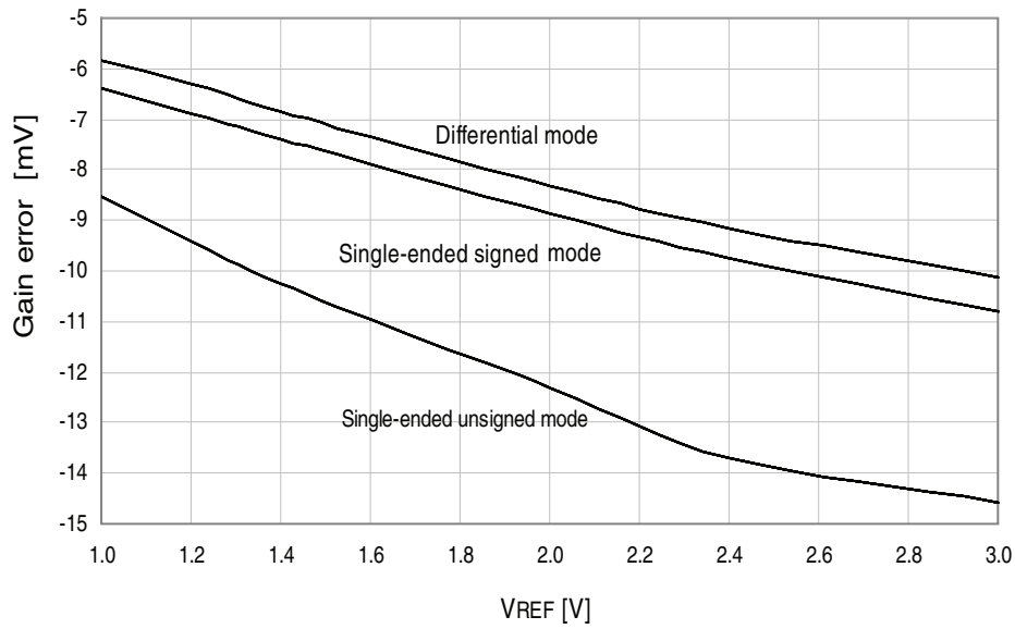
Figure 34-238. Gain error vs. V_{REF} .
