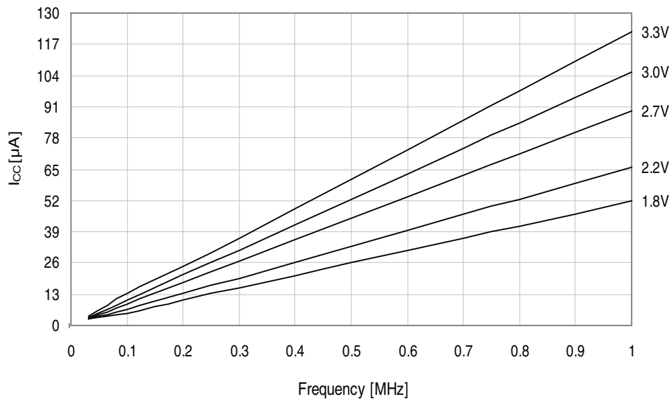
Figure 34-210. Idle mode supply current vs. frequency.
