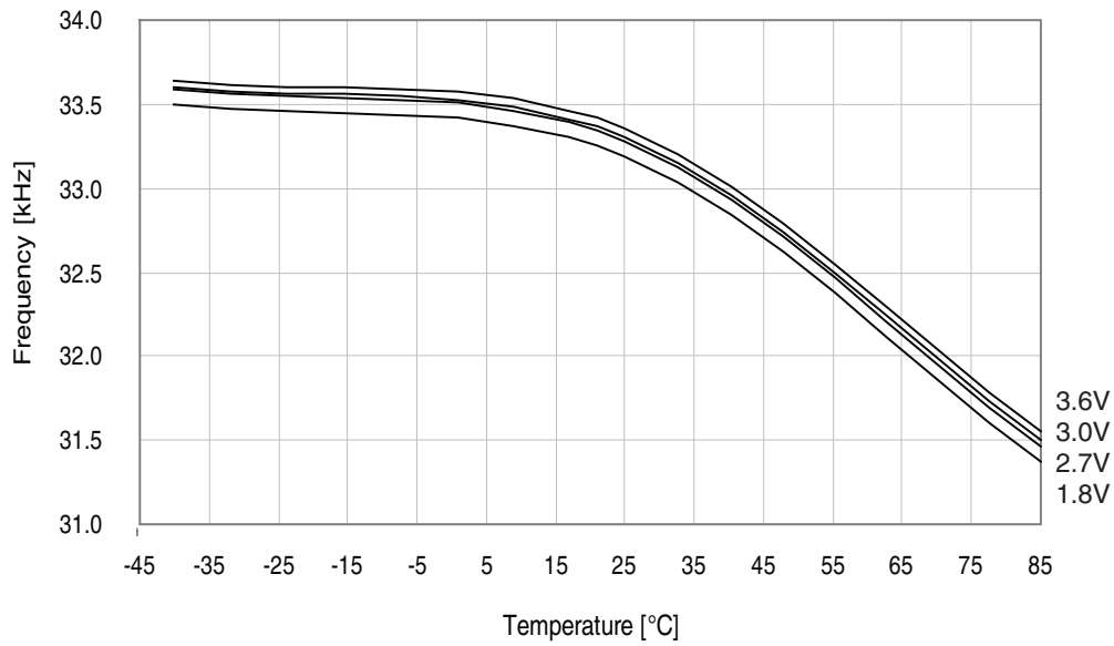
Figure 34-255.Ultra Low-Power internal oscillator frequency vs. temperature.
