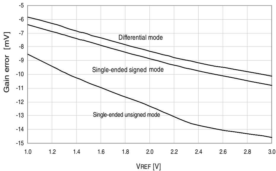
Figure 34-171. Gain error vs. V_{REF} .
