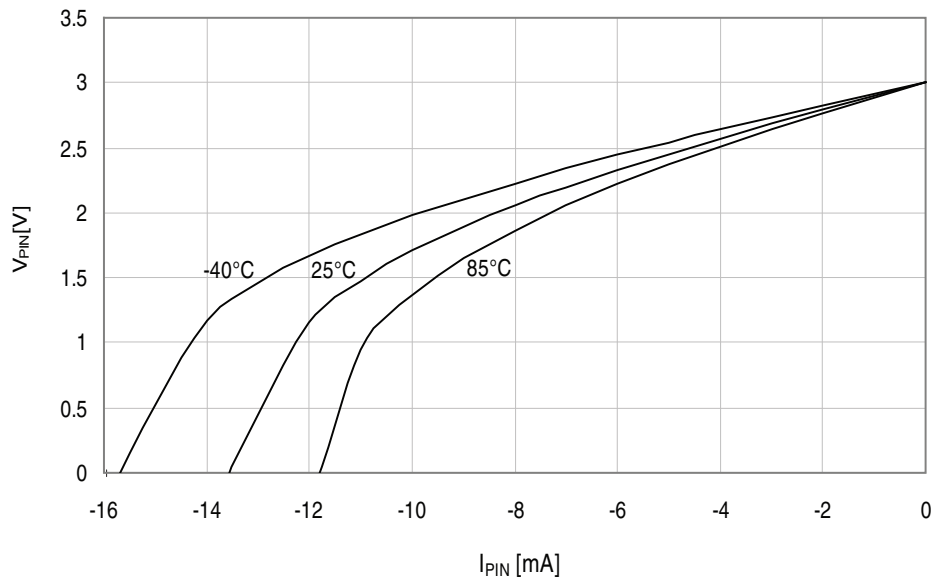
Figure 34-90. I/O pin output voltage vs. source current.
