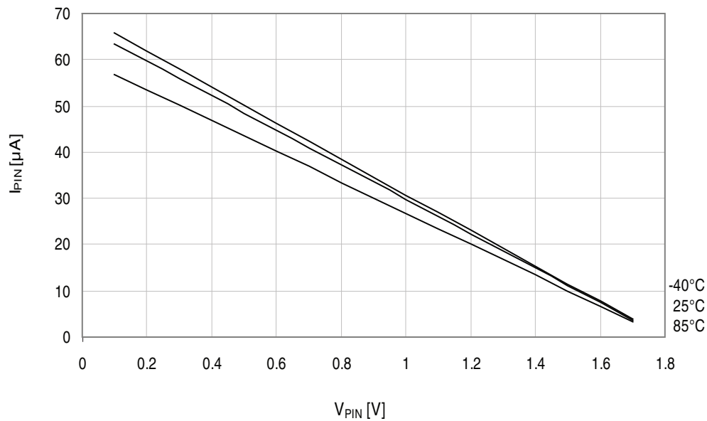
Figure 34-86. I/O pin pull-up resistor current vs. input voltage.
