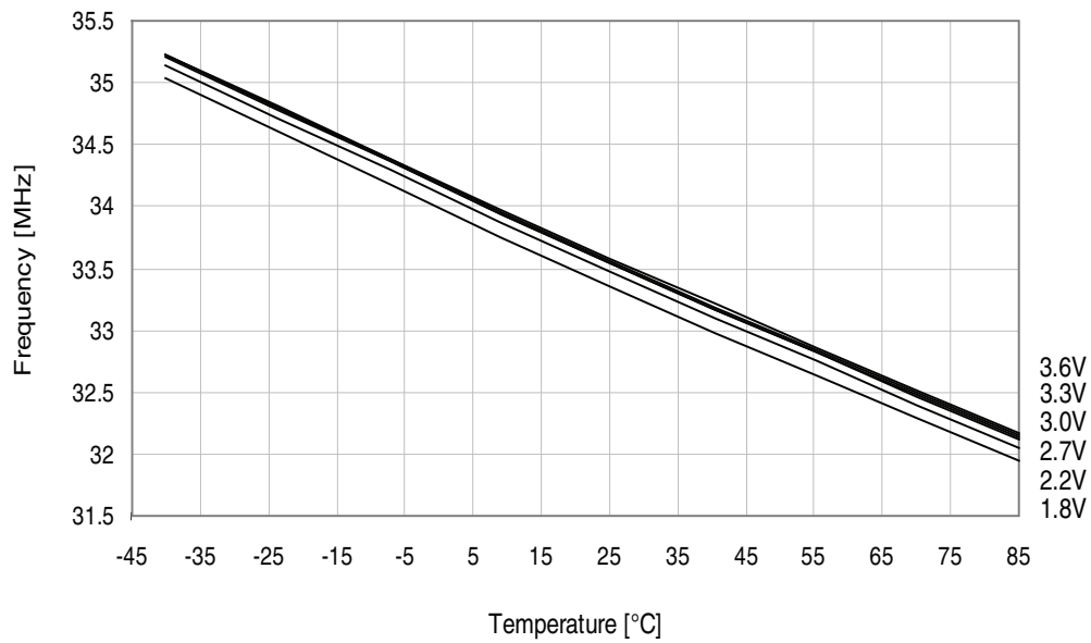
Figure 34-262.32MHz internal oscillator frequency vs. temperature. DPLL enabled, from the 32.768kHz internal oscillator.
