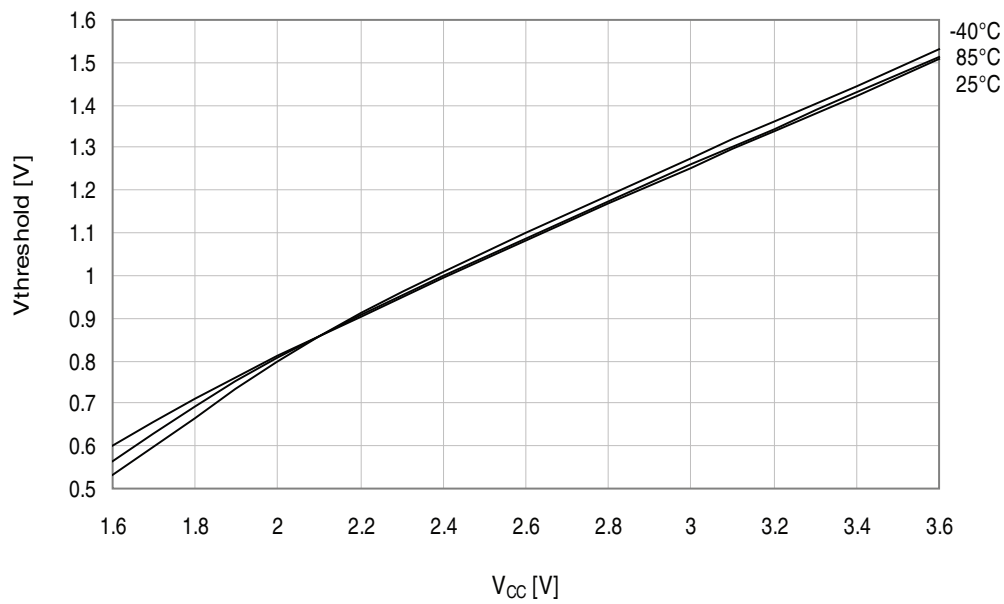
Figure 34-163. I/O pin input threshold voltage vs. V_{CC} .
