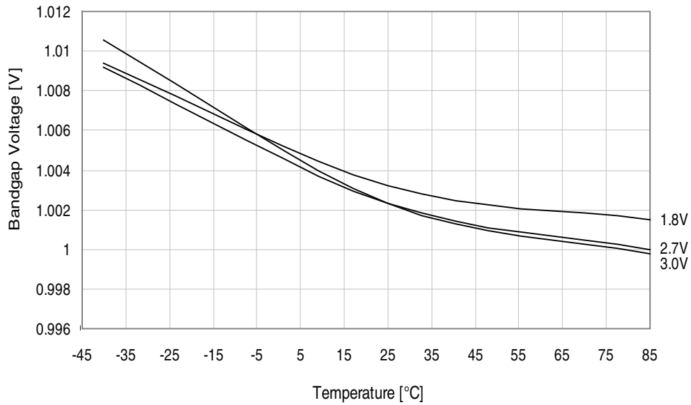
Figure 34-113.ADC Internal 1.0V reference vs. temperature.
