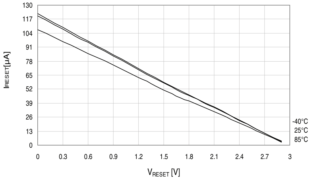
Figure 34-185. Reset pin pull-up resistor current vs. reset pin voltage.
