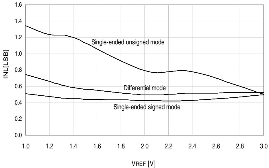
Figure 34-165. INL error vs. external V_{REF} .
