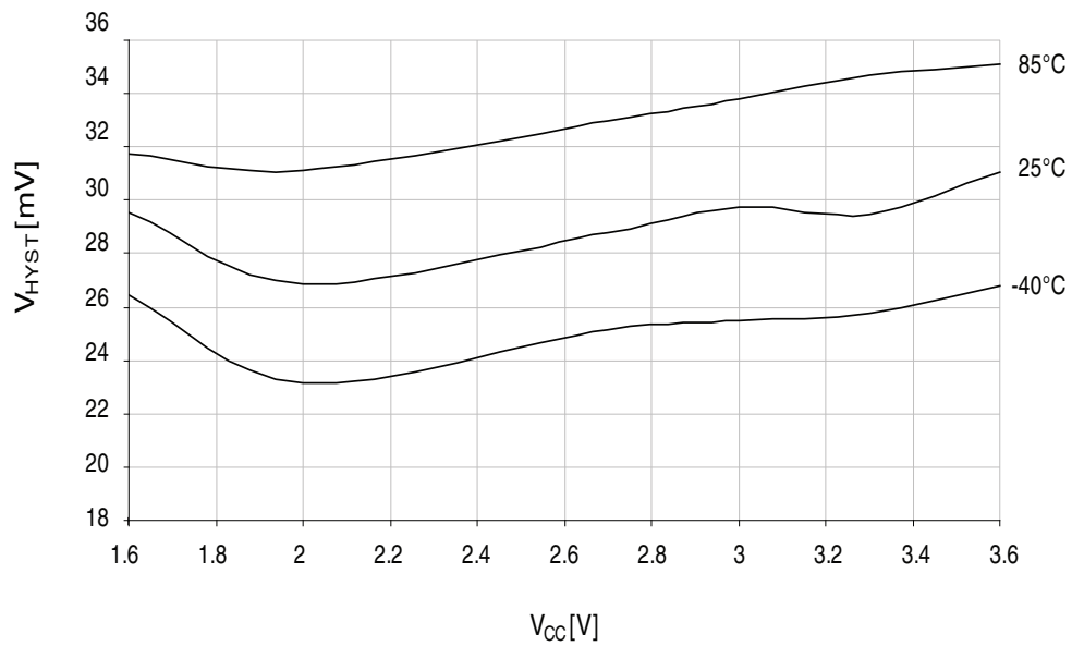
Figure 34-110. Analog comparator hysteresis vs. V_{CC} . Large hysteresis.
