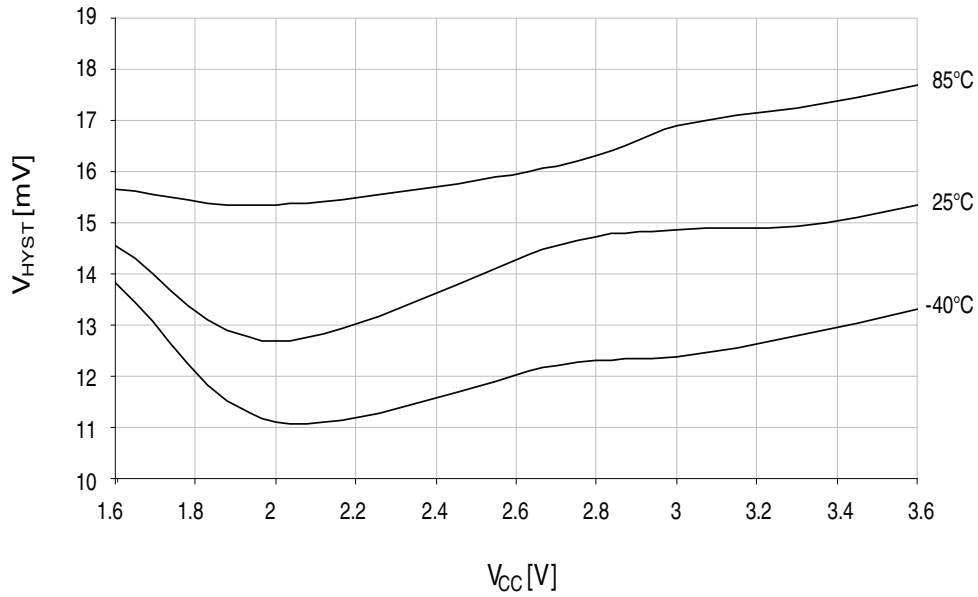
Figure 34-177. Analog comparator hysteresis vs. V_{CC} . Large hysteresis.
