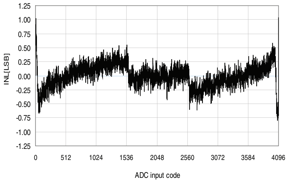
Figure 34-100. INL error vs. input code.
