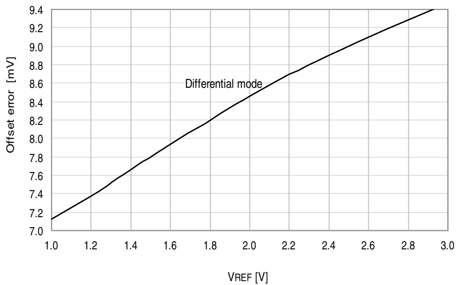
Figure 34-106. Offset error vs. V_{REF} .
