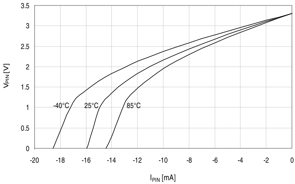
Figure 34-226. I/O pin output voltage vs. sink current.
