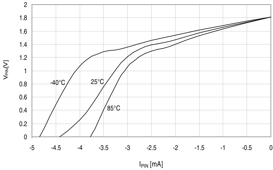
Figure 34-90. I/O pin output voltage vs. source current.
