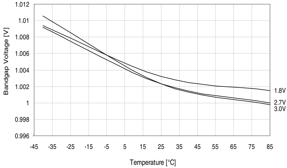
Figure 34-247.ADC Internal 1.0V reference vs. temperature.
