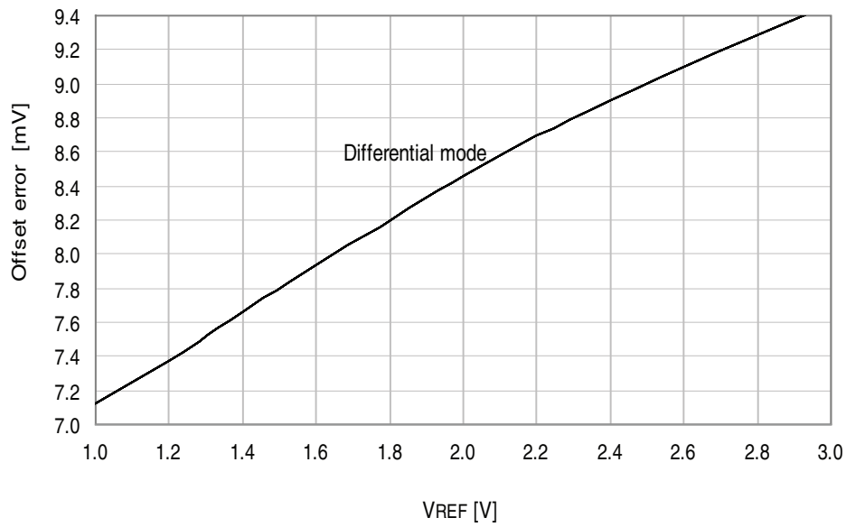
Figure 34-173. Offset error vs. V_{REF} .
