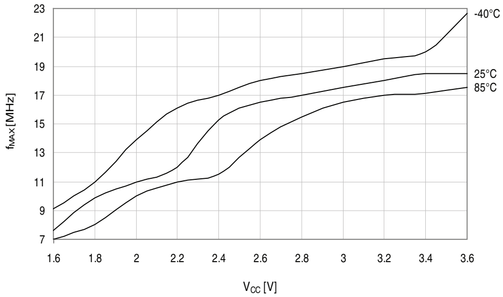
Figure 34-202. Maximum PDI frequency vs. V_{CC} .
