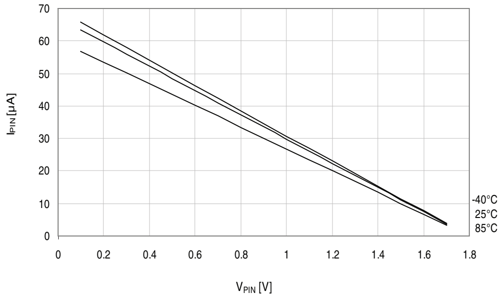
Figure 34-220. I/O pin pull-up resistor current vs. input voltage.
