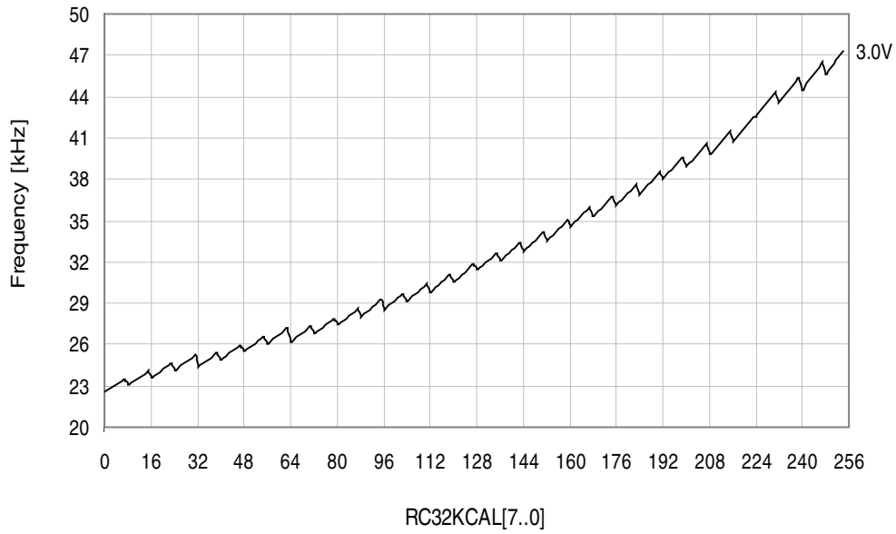
Figure 34-123. 32.768kHz internal oscillator frequency vs. calibration value.
