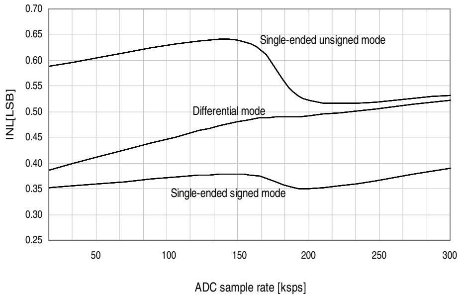
Figure 34-32. INL error vs. sample rate.
