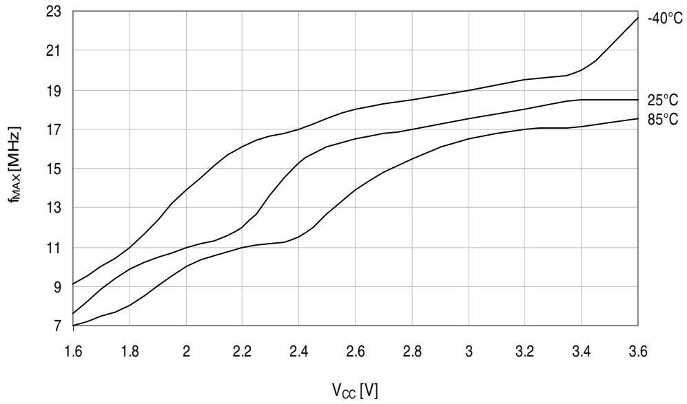
Figure 34-269. Maximum PDI frequency vs. V_{CC} .
