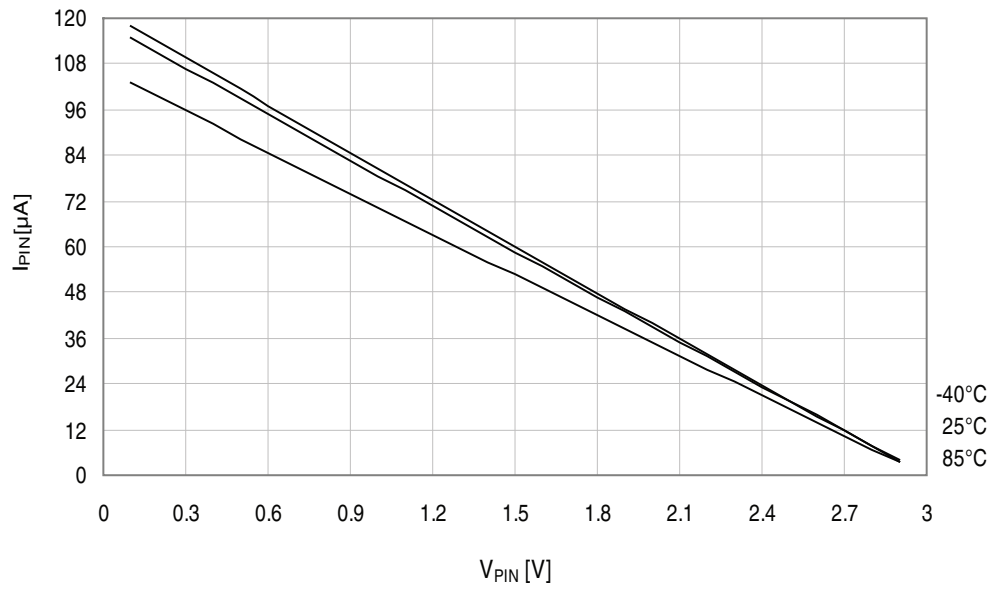
Figure 34-222. I/O pin pull-up resistor current vs. input voltage.
