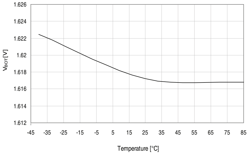
Figure 34-181.BOD thresholds vs. temperature.
