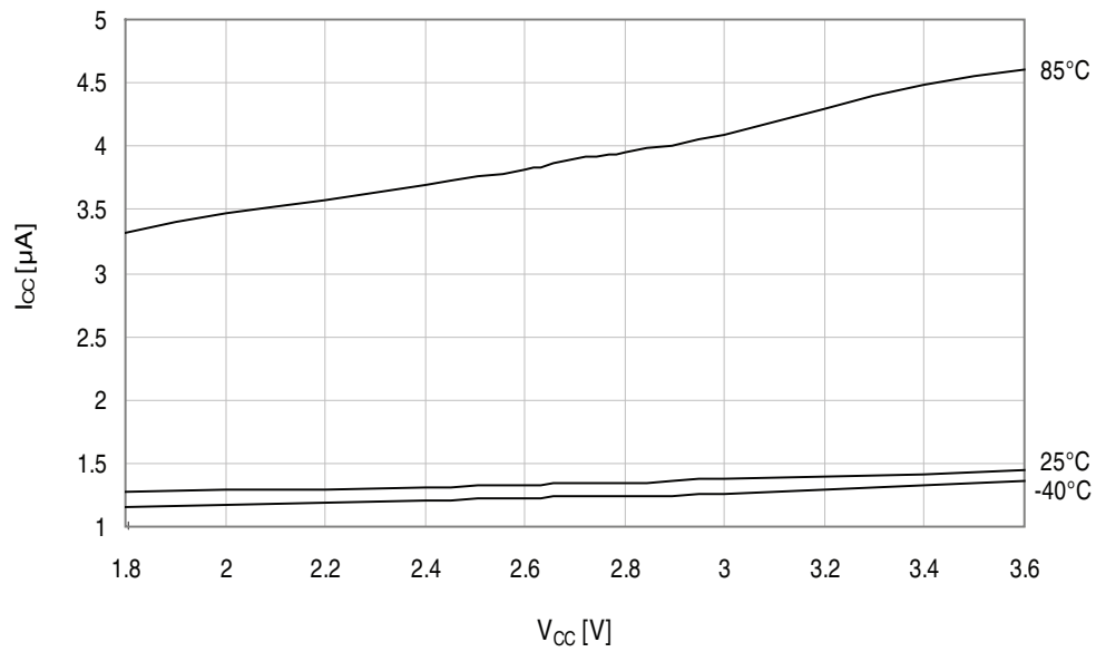
Figure 34-218. Power-down mode supply current vs. V_{CC} . Watchdog and sampled BOD enabled.
