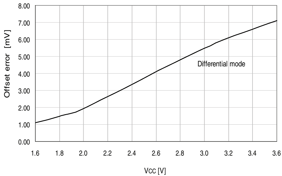
Figure 34-242. Offset error vs. V_{CC} .
