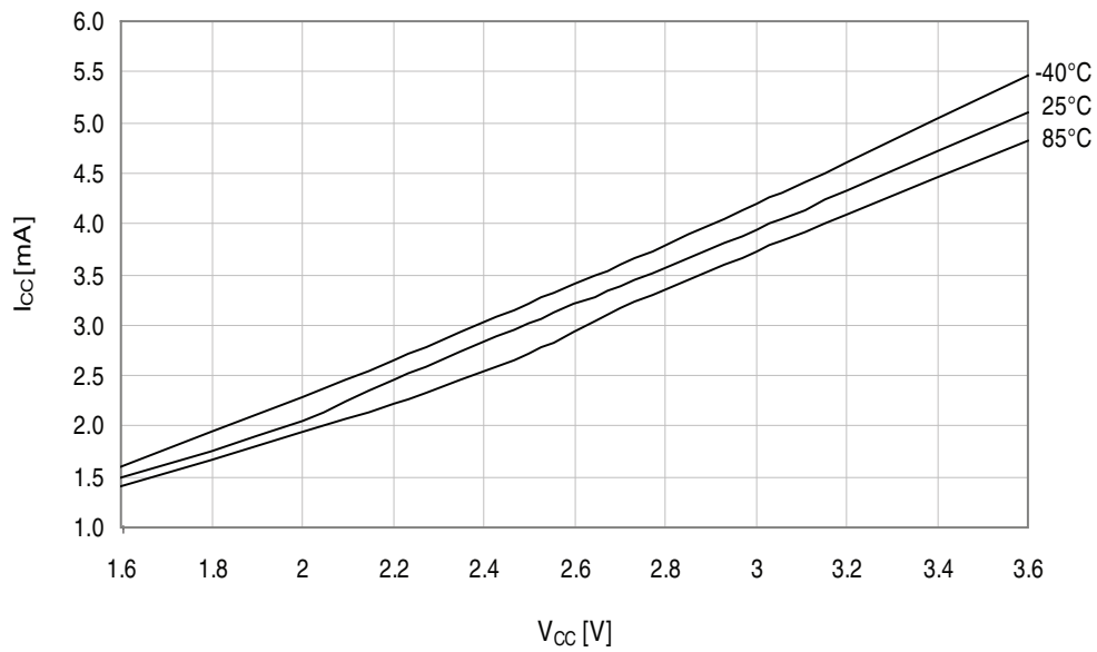
Figure 34-208. Active mode supply current vs. V_{CC} .
