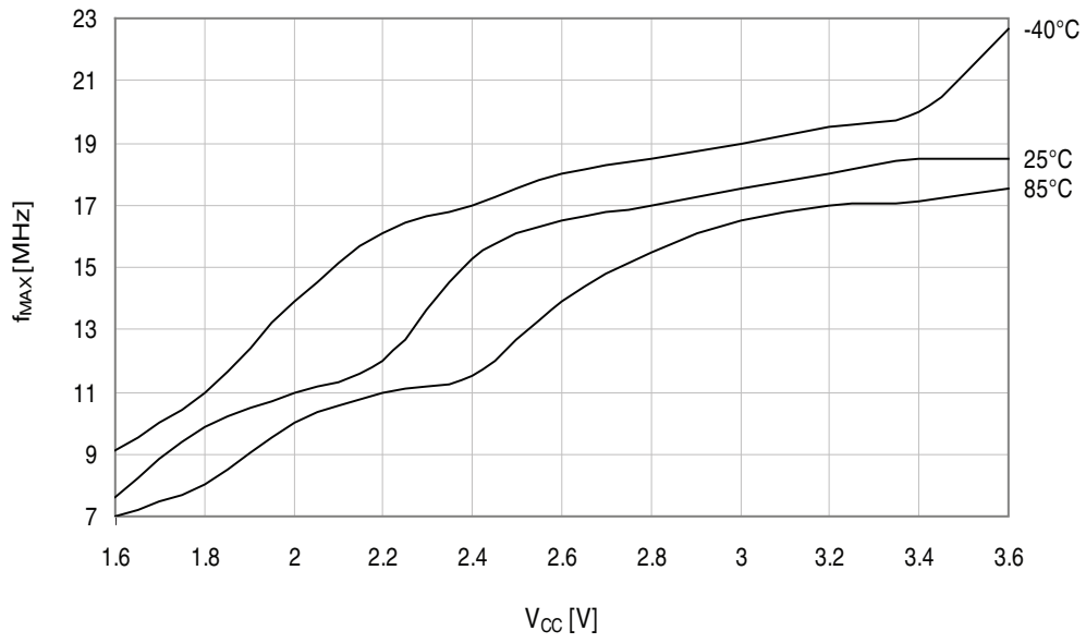
Figure 34-135. Maximum PDI frequency vs. V_{CC} .
