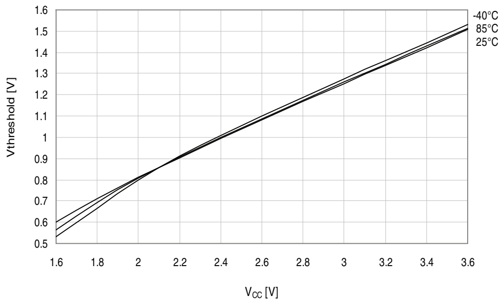
Figure 34-230. I/O pin input threshold voltage vs. V_{CC} .
