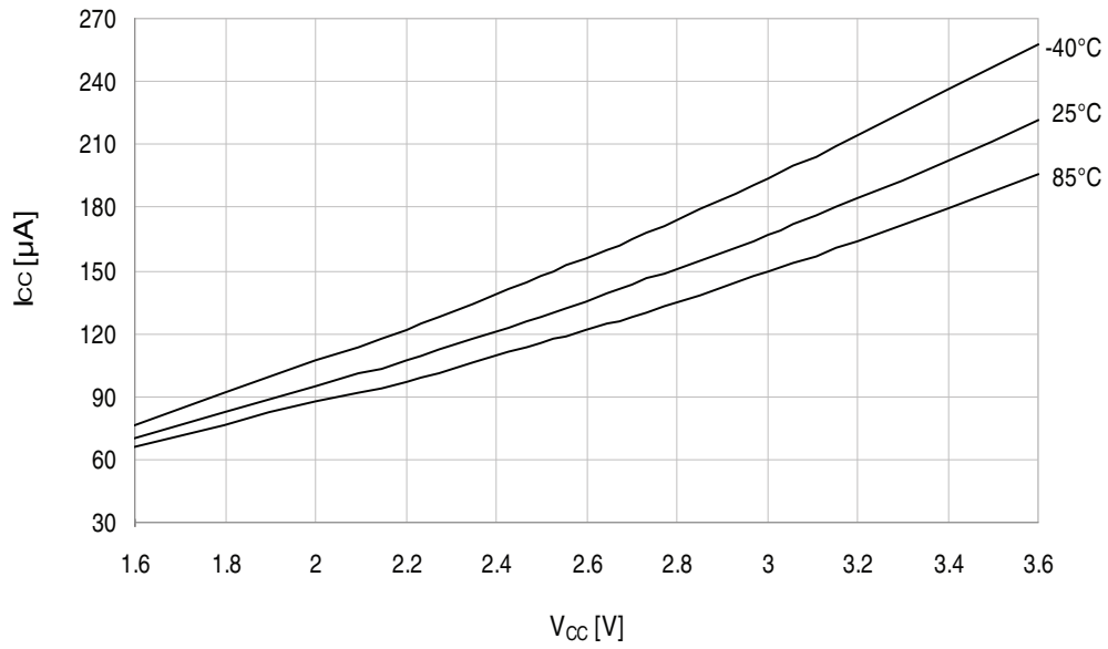
Figure 34-139. Active mode supply current vs. V_{CC} .
