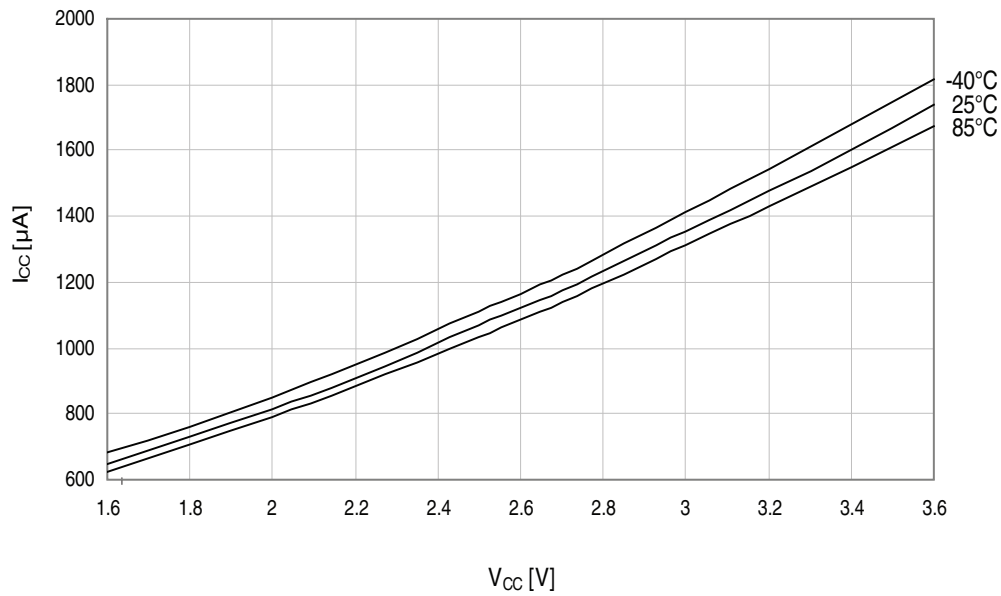
Figure 34-216. Idle mode current vs. V_{CC} .
