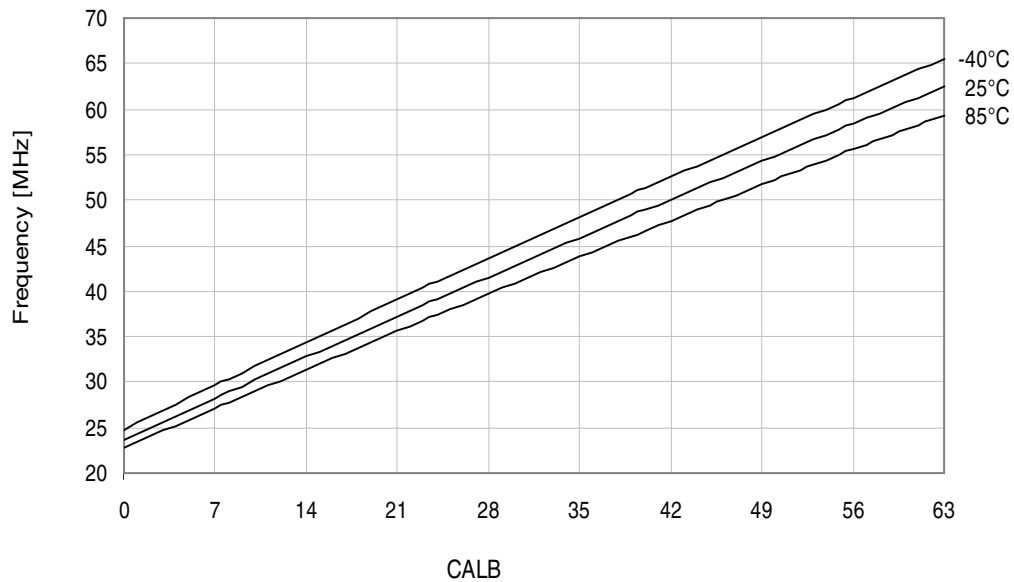
Figure 34-264.32MHz internal oscillator frequency vs. CALB calibration value.
