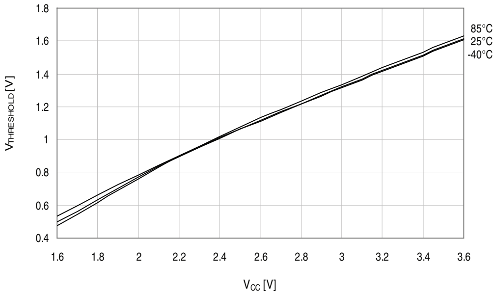
Figure 34-254. Reset pin input threshold voltage vs. V_{CC} .
