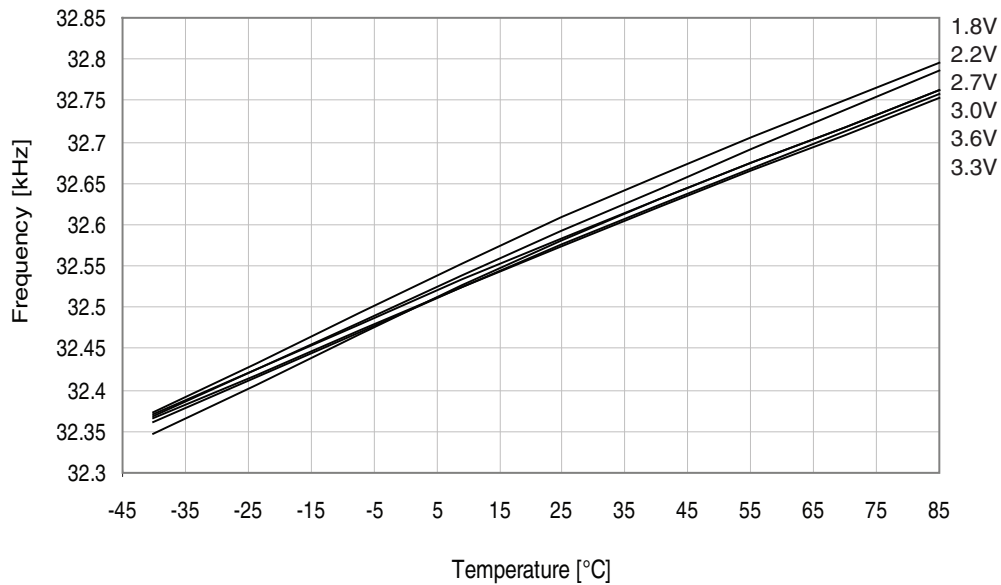
Figure 34-122. 32.768kHz internal oscillator frequency vs. temperature.
