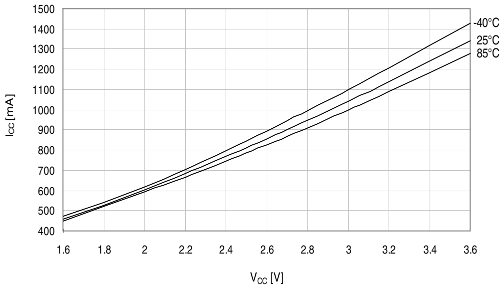
Figure 34-208. Active mode supply current vs. V_{CC} .
