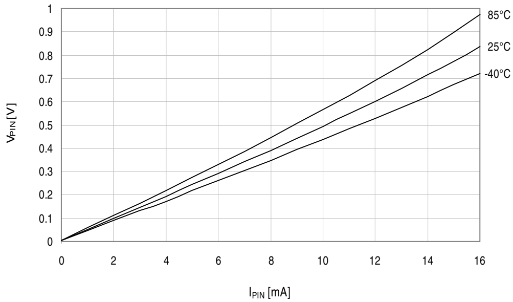
Figure 34-228. I/O pin output voltage vs. sink current.
