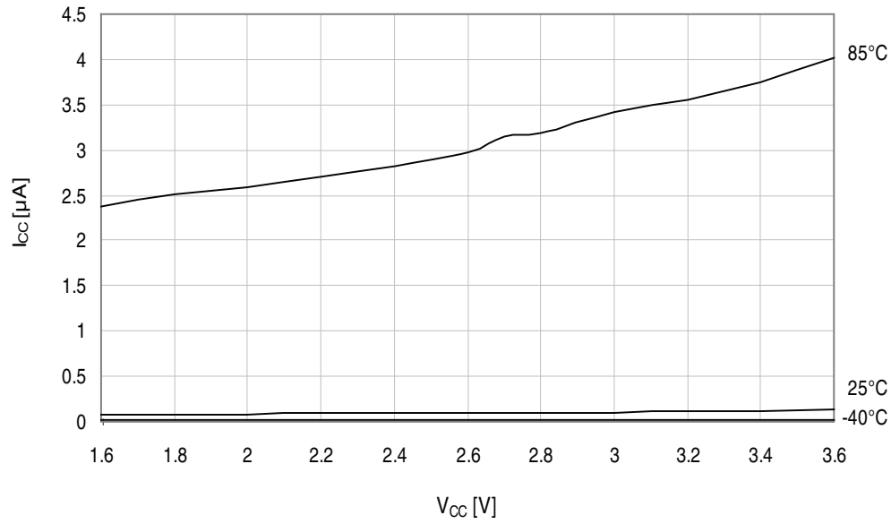
Figure 34-151. Power-down mode supply current vs. V_{CC} . Watchdog and sampled BOD enabled.
