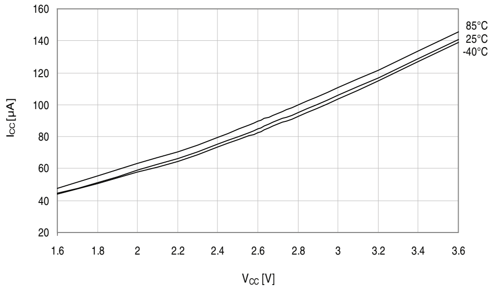
Figure 34-214. Idle mode supply current vs. V_{CC} .
