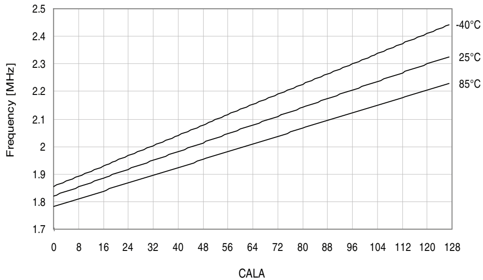
Figure 34-260. 2MHz internal oscillator frequency vs. CALA calibration value.
