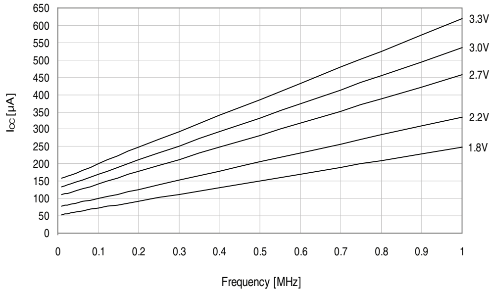
Figure 34-137. Active supply current vs. frequency.
