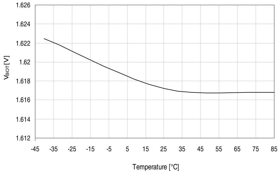
Figure 34-248.BOD thresholds vs. temperature.
