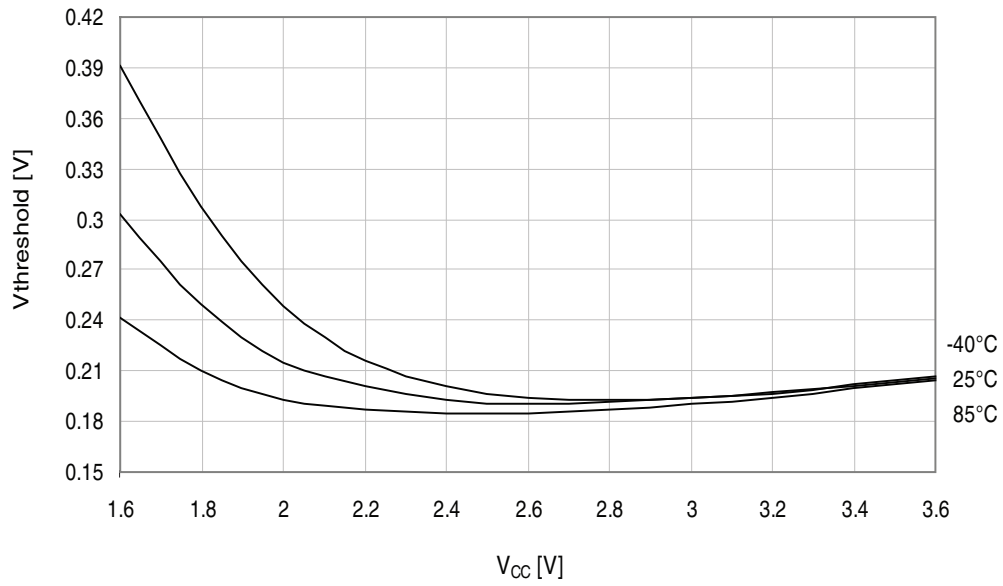
Figure 34-164. I/O pin input hysteresis vs. V_{CC} .
