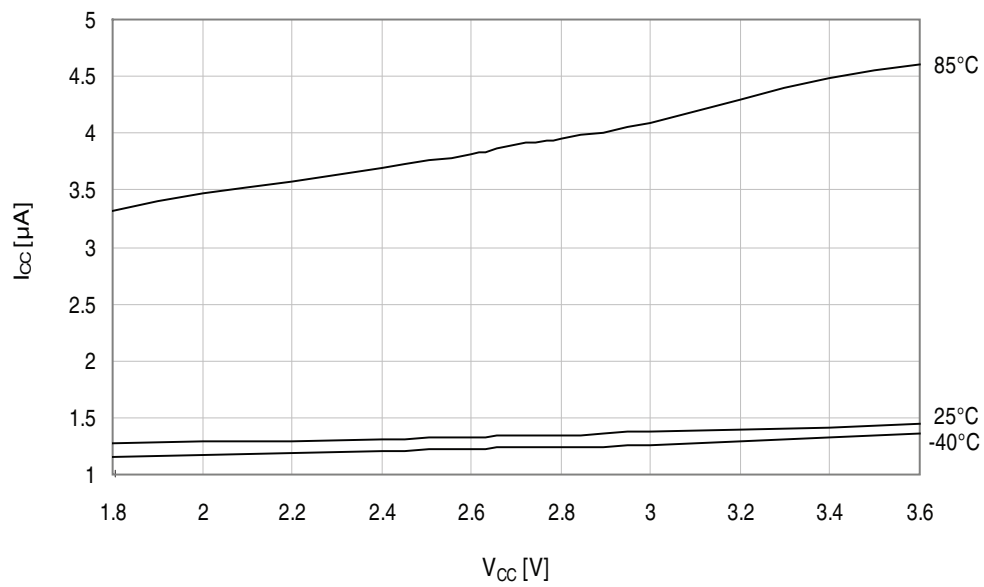
Figure 34-151. Power-down mode supply current vs. V_{CC} . Watchdog and sampled BOD enabled.
