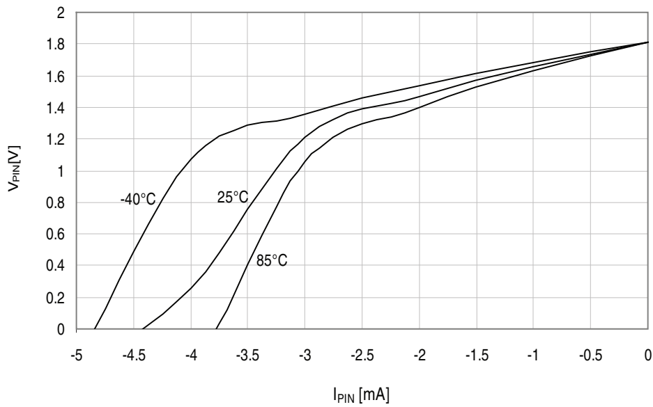
Figure 34-157. I/O pin output voltage vs. source current.
