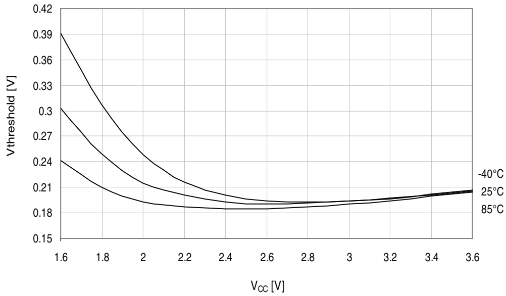
Figure 34-231. I/O pin input hysteresis vs. V_{CC} .
