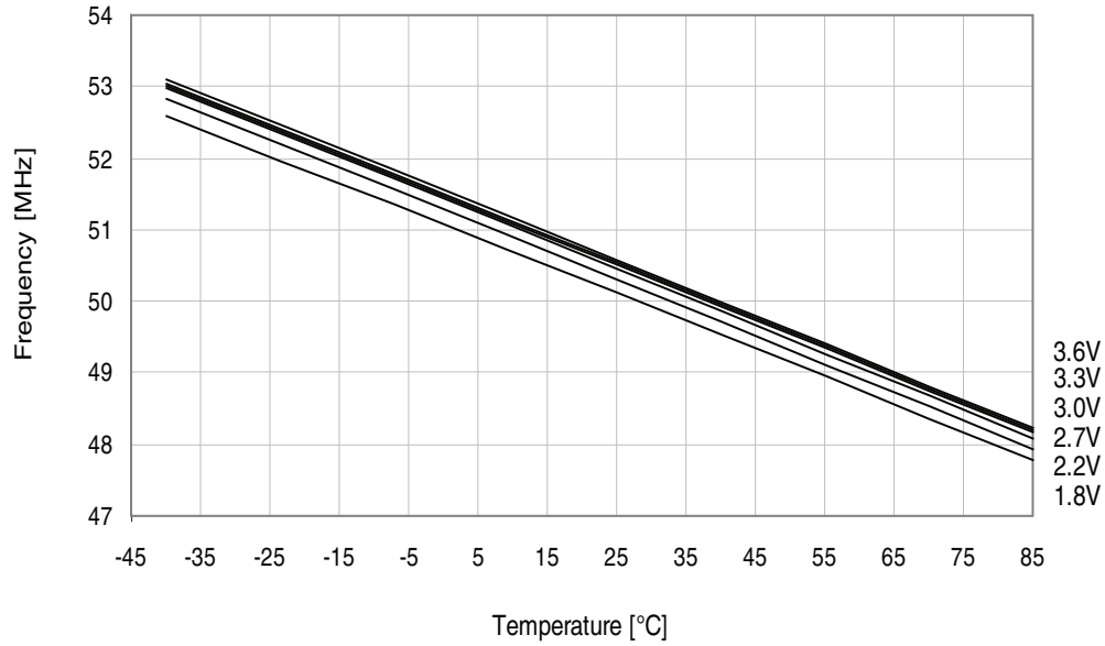
Figure 34-266.48MHz internal oscillator frequency vs. temperature.
