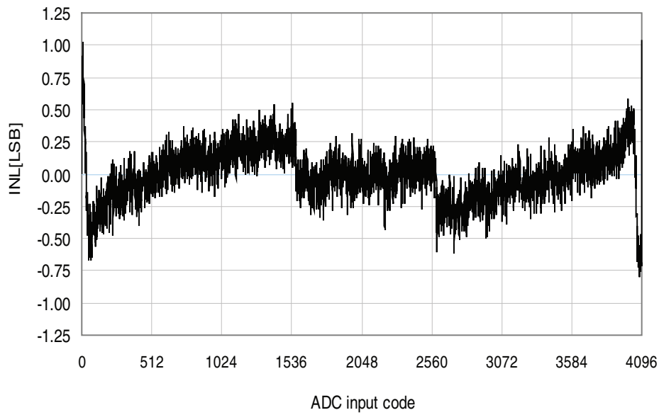
Figure 34-167. INL error vs. input code.
