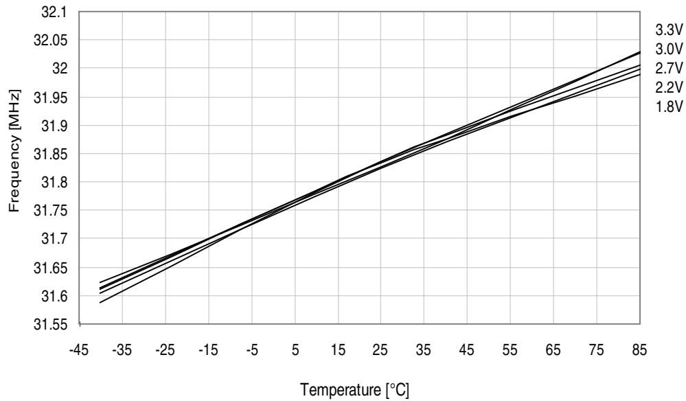
Figure 34-195.32MHz internal oscillator frequency vs. temperature. DPLL enabled, from the 32.768kHz internal oscillator.
