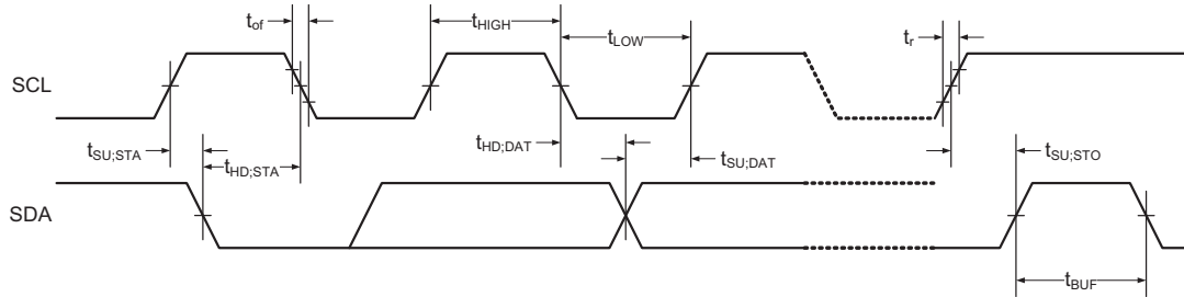
Figure 33-28. Two-wire interface bus timing.
