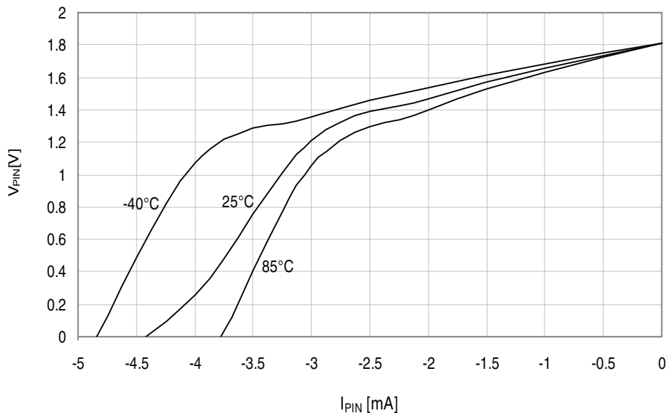
Figure 34-224. I/O pin output voltage vs. source current.
