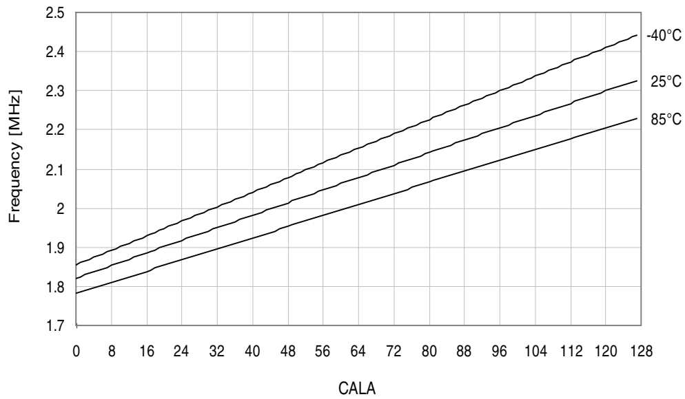
Figure 34-126.2MHz internal oscillator frequency vs. CALA calibration value.
