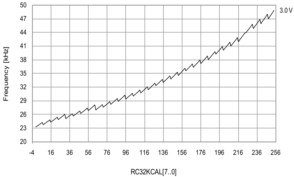
Figure 34-56. 32.768kHz internal oscillator frequency vs. calibration value.
