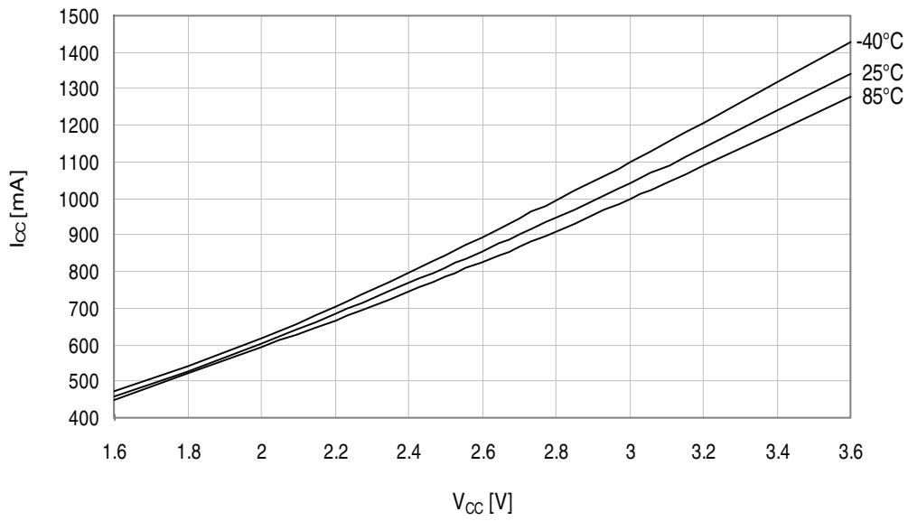
Figure 34-141. Active mode supply current vs. V_{CC} .
