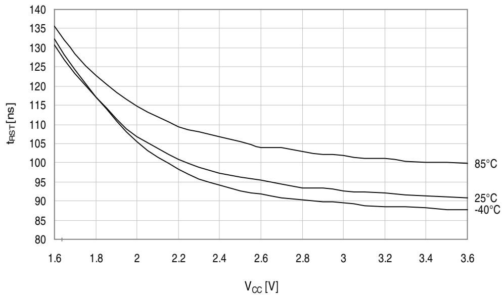
Figure 34-183. Minimum Reset pin pulse width vs. V CC .
