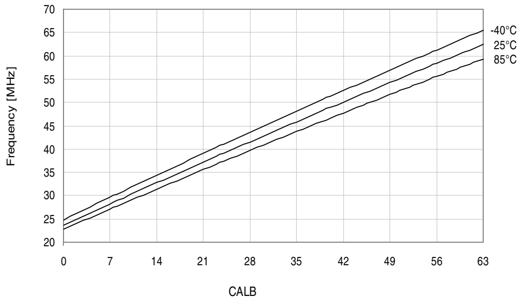
Figure 34-130.32MHz internal oscillator frequency vs. CALB calibration value.
