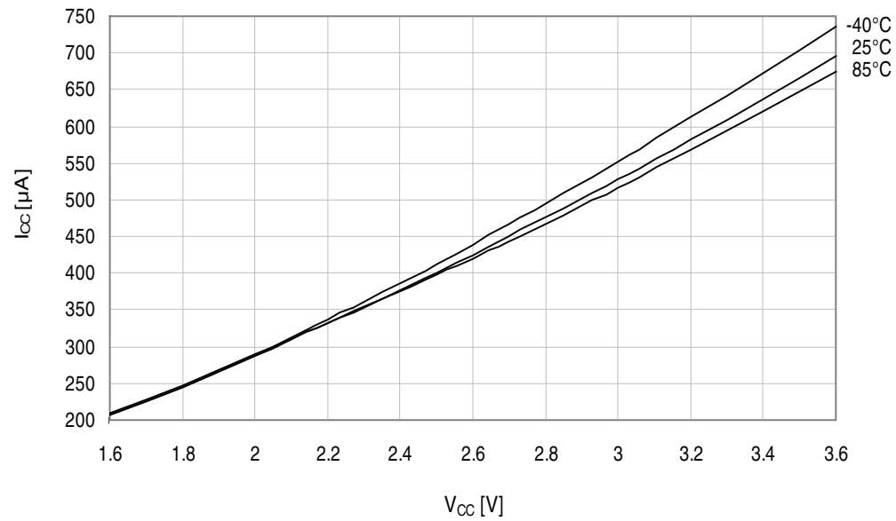
Figure 34-206.Active mode supply current vs. V_{CC} .
