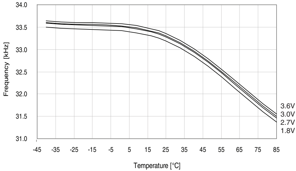
Figure 34-121. Ultra Low-Power internal oscillator frequency vs. temperature.
