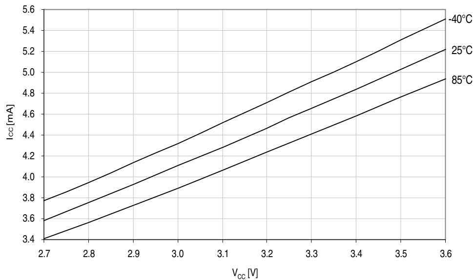
Figure 37-14. Idle mode current vs. V_{CC} . f_{SYS} = 32\text{MHz} internal oscillator.
