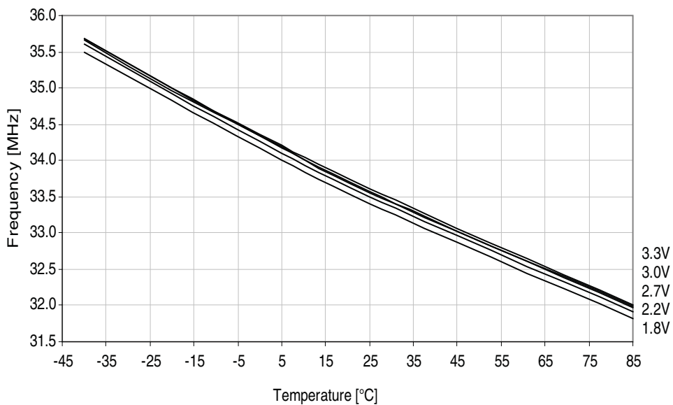
Figure 37-77. 32MHz internal oscillator frequency vs. temperature. DPLL enabled, from the 32.768kHz internal oscillator.
