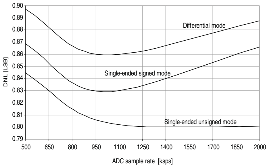
Figure 37-40. DNL error vs. sample rate.
