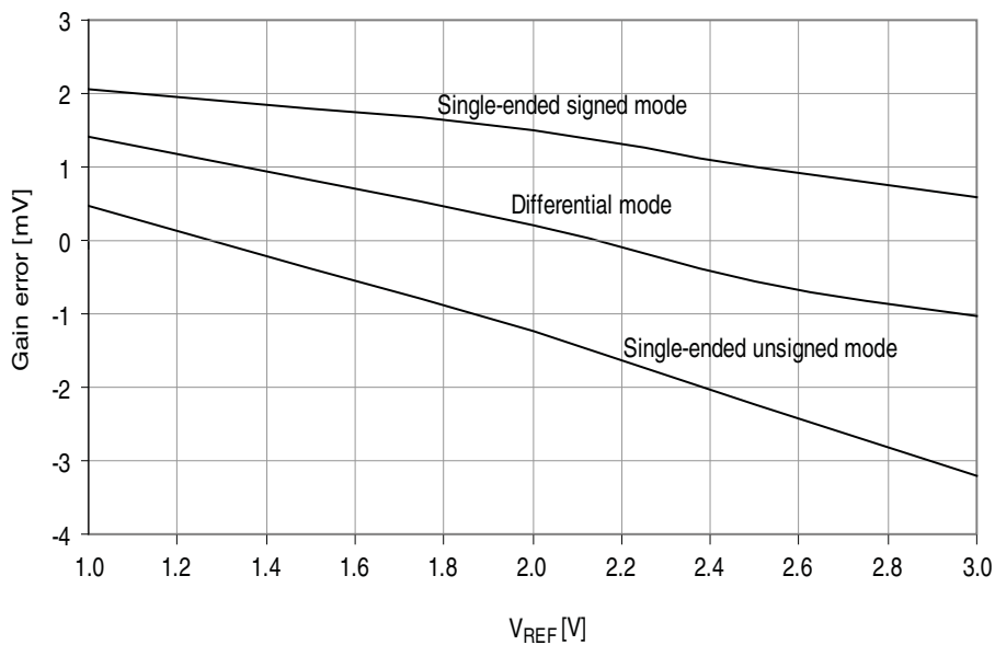
Figure 37-42. Gain error vs. V_{REF} . T = 25^{\circ}\text{C} , V_{CC} = 3.6\text{V} , ADC sampling speed = 500kps.
