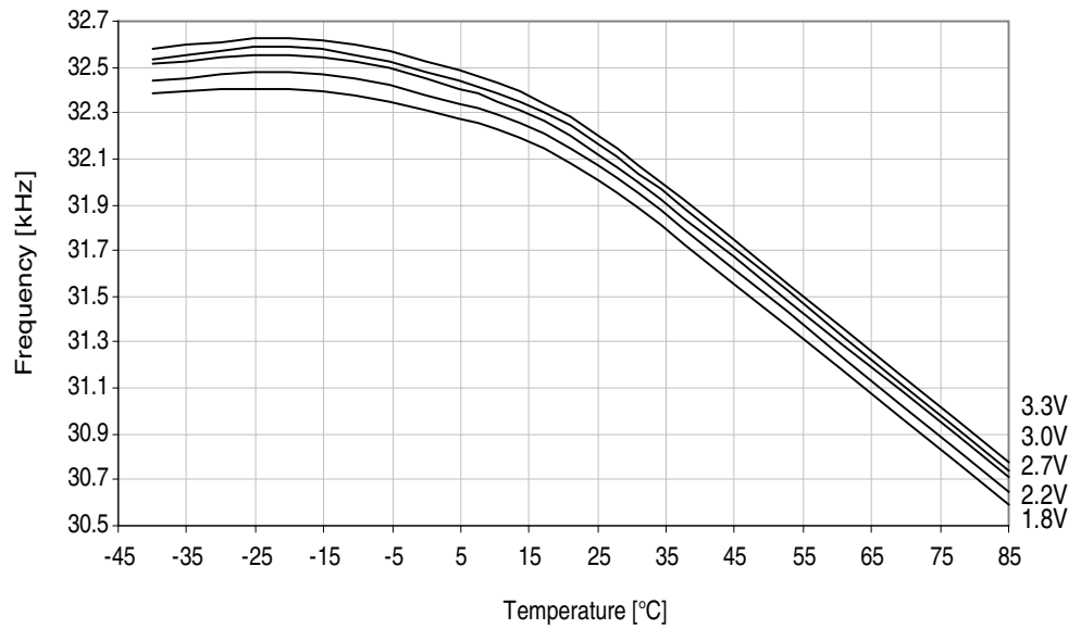
Figure 37-70. Ultra Low-Power internal oscillator frequency vs. temperature.
