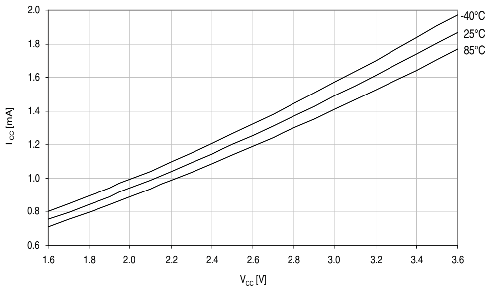
Figure 37-14. Idle mode current vs. V_{CC} . f_{SYS} = 32\text{MHz} internal oscillator.
