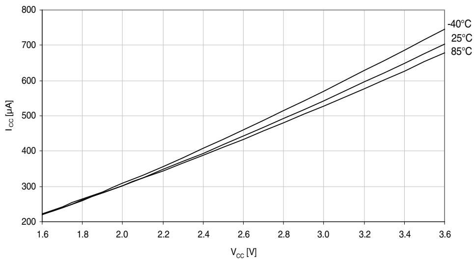
Figure 37-4. Active mode supply current vs. V_{CC} . f_{SYS} = 1MHz external clock.
