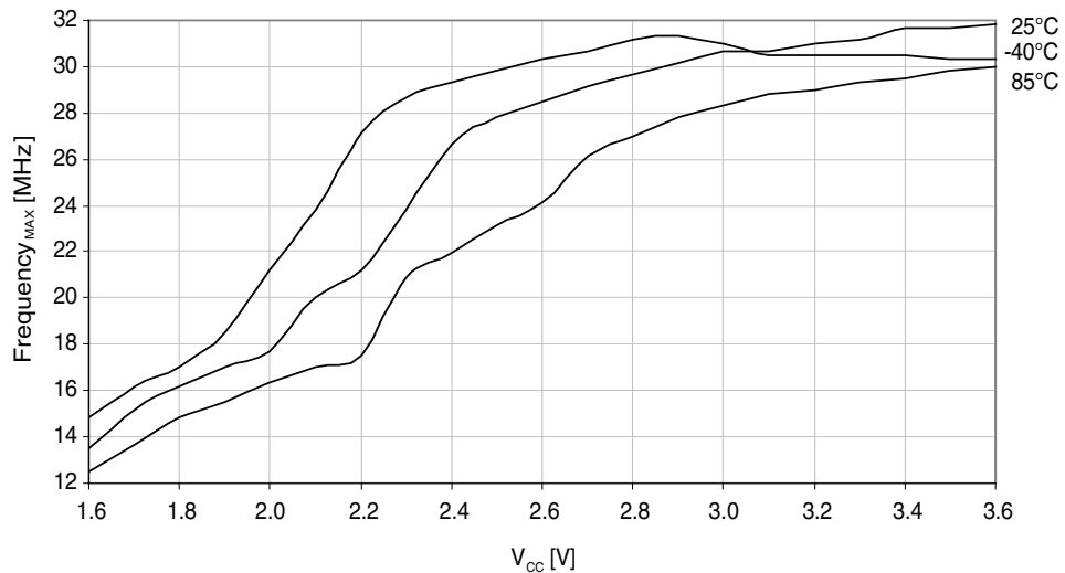
Figure 37-85. Maximum PDI frequency vs. V CC .
