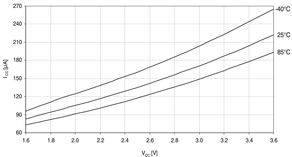
Figure 37-3. Active mode supply current vs. V_{CC} . f_{SYS} = 32.768kHz internal oscillator.
