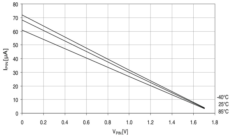
Figure 37-62. Reset pin pull-up resistor current vs. reset pin voltage.
