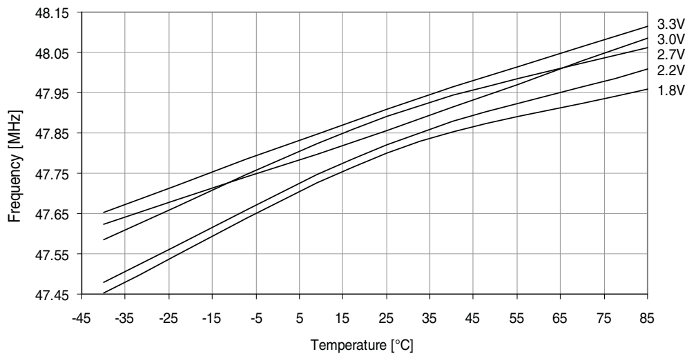
Figure 37-79. 48MHz internal oscillator frequency vs. temperature. DFLL enabled, from the 32.768kHz internal oscillator.
