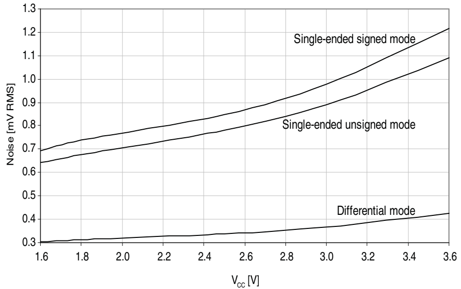
Figure 37-47. Noise vs. V_{CC} .
