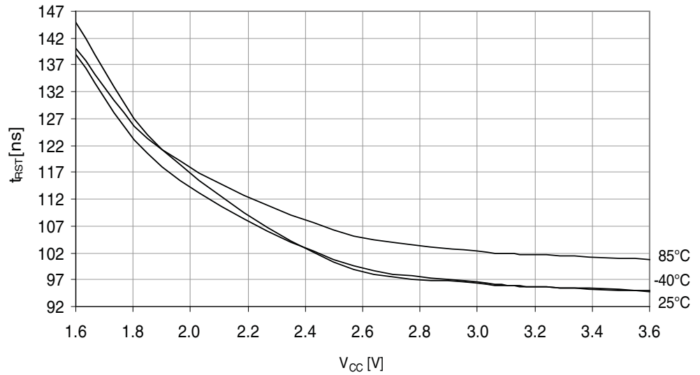
Figure 37-61. Minimum Reset pin pulse width vs. V_{CC} .
