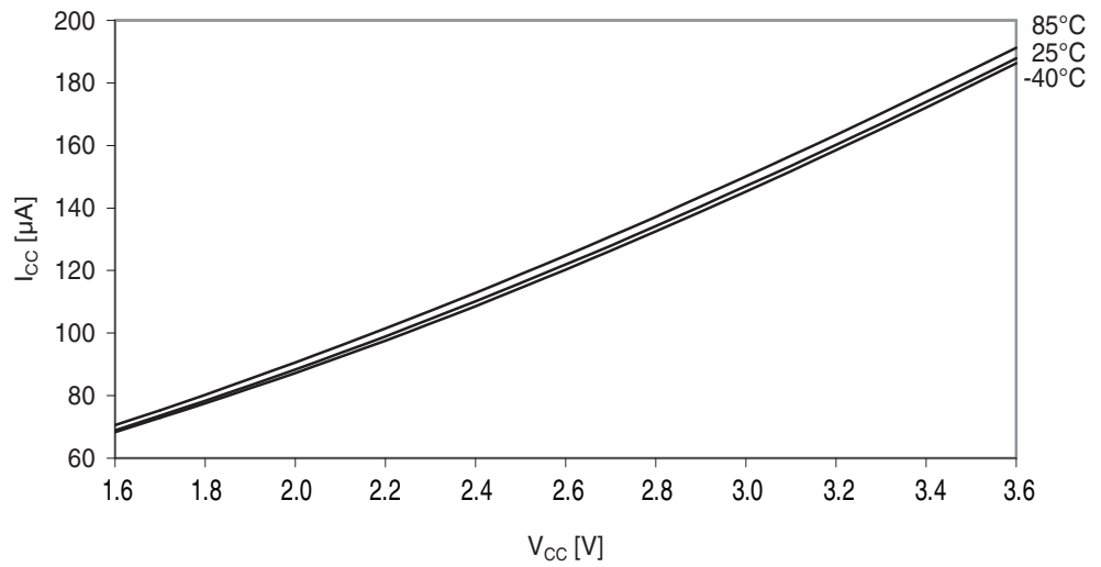
Figure 37-12. Idle mode supply current vs. V_{CC} .
