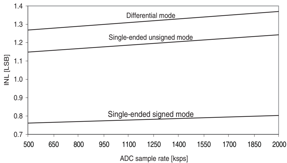
Figure 37-36. INL error vs. sample rate.
