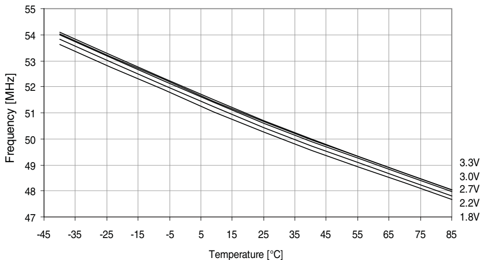
Figure 37-78. 48MHz internal oscillator frequency vs. temperature. DFLL disabled.
