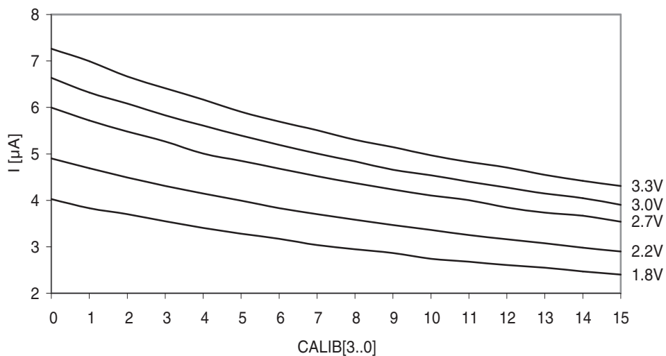
Figure 37-55. Analog comparator current source vs. calibration value. Temperature = 25°C.
