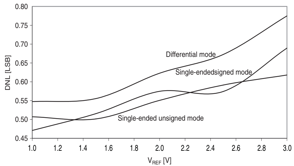
Figure 37-38. DNL error vs. external V_{REF} .
