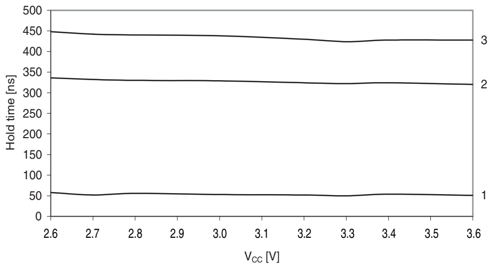
Figure 37-82. SDA hold time vs. supply voltage.
