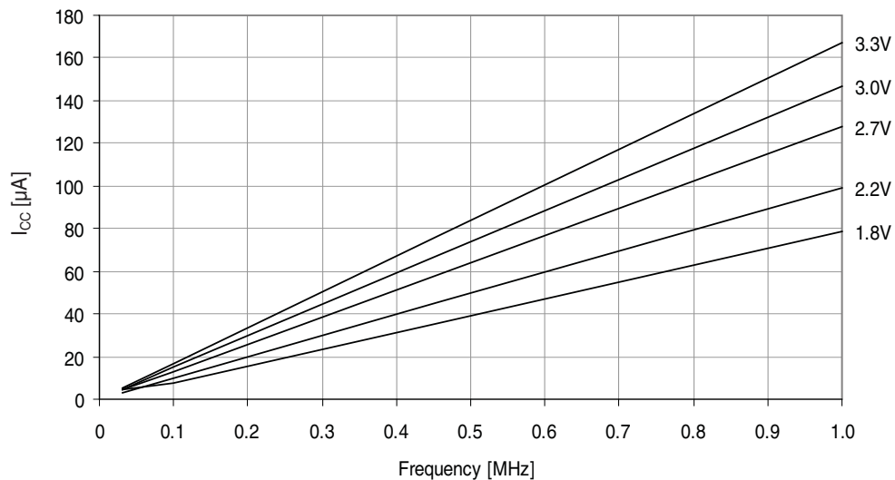
Figure 37-8. Idle mode supply current vs. frequency. f_{SYS} = 0 - 1\text{MHz} external clock, T = 25^\circ\text{C} .
