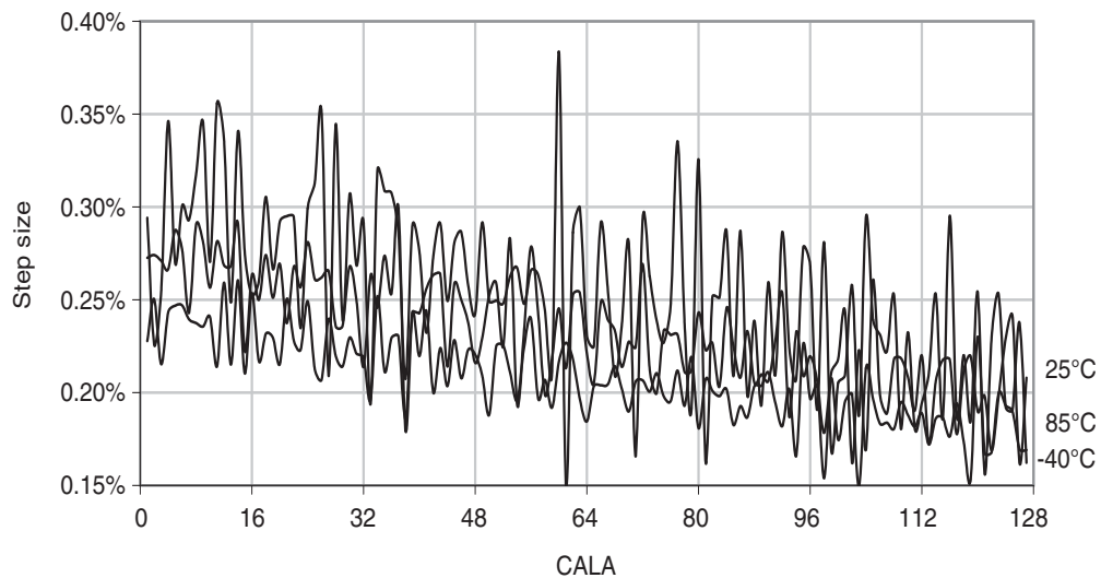
Figure 37-80. 48MHz internal oscillator CALA calibration step size.
