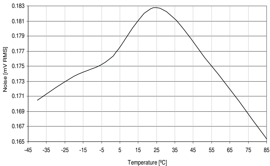
Figure 37-50. DAC noise vs. temperature.
