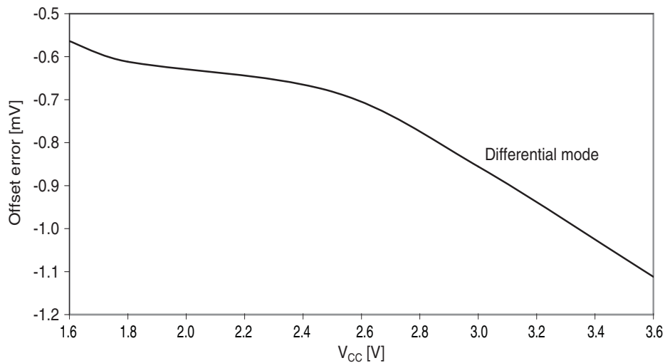
Figure 37-45. Offset error vs. V_{CC} .
