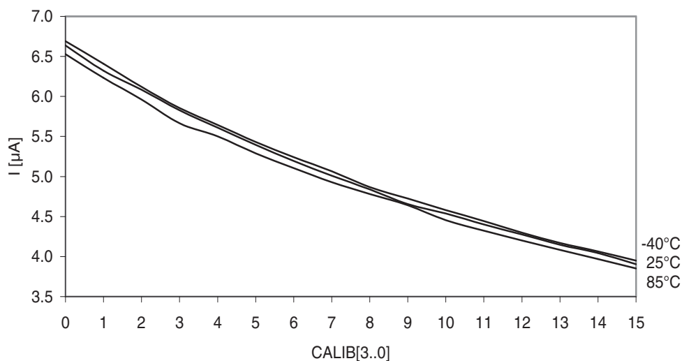
Figure 37-56. Analog comparator current source vs. calibration value. V_{CC} = 3.0\text{V} .
