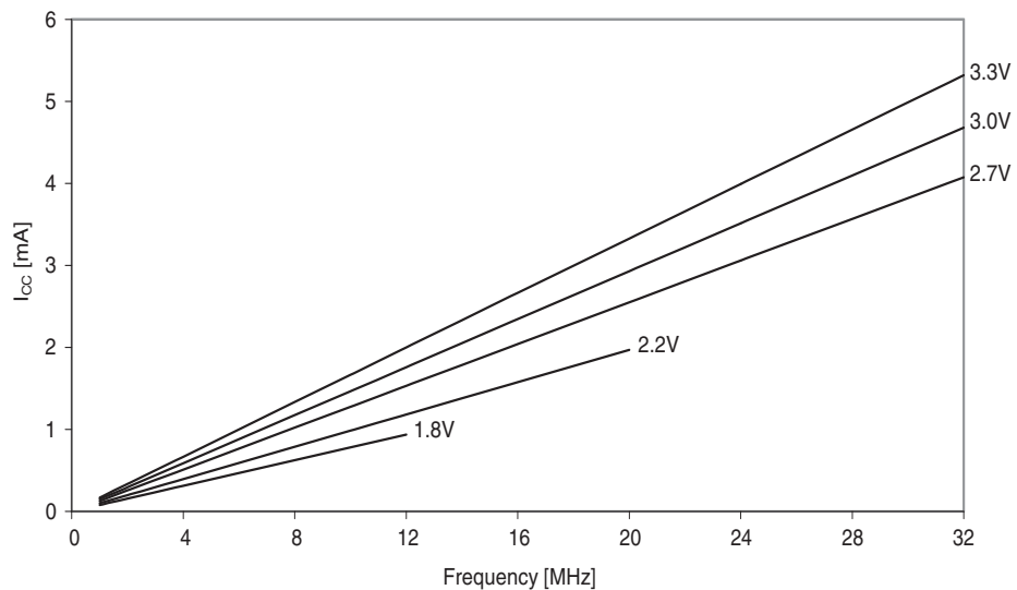
Figure 37-9. Idle mode supply current vs. frequency.
