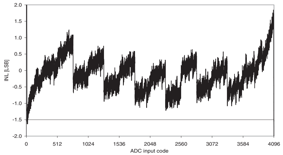
Figure 37-37. INL error vs. input code.
