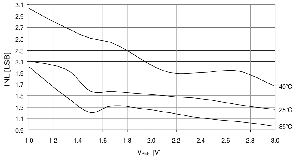
Figure 37-48. DAC INL error vs. V_{REF} .
