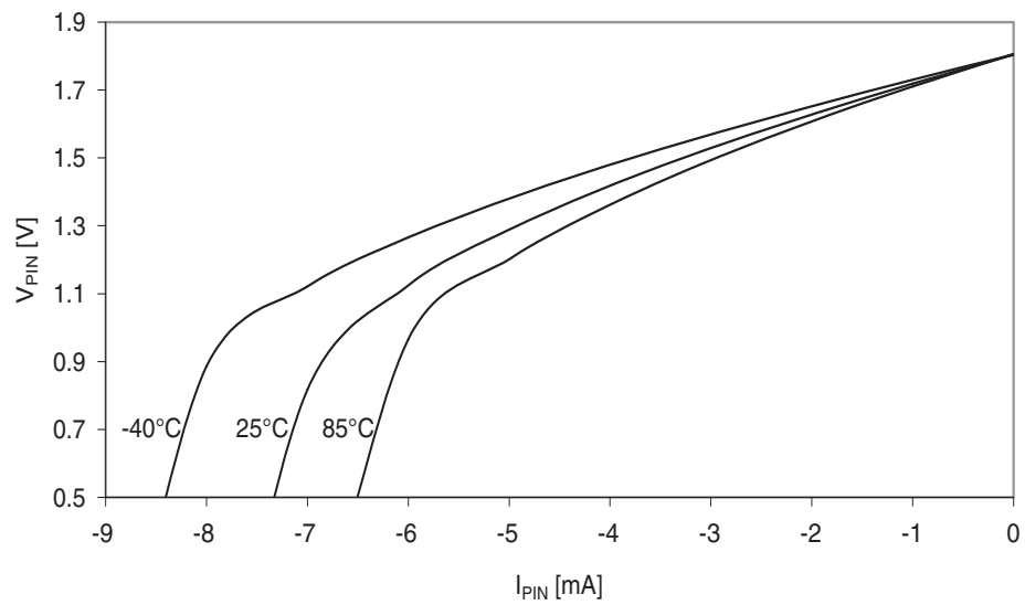
Figure 37-24. I/O pin output voltage vs. source current.
