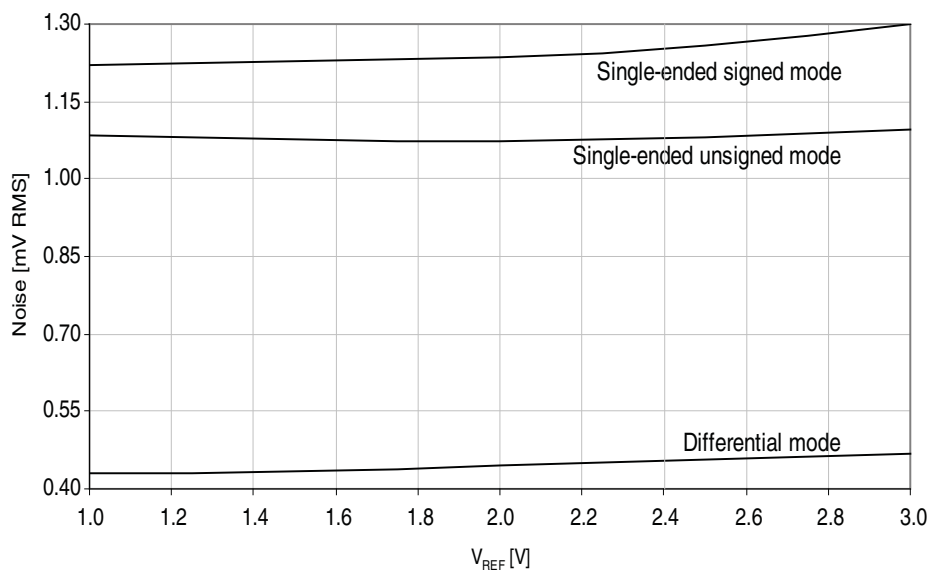
Figure 37-46. Noise vs. V_{REF} .
