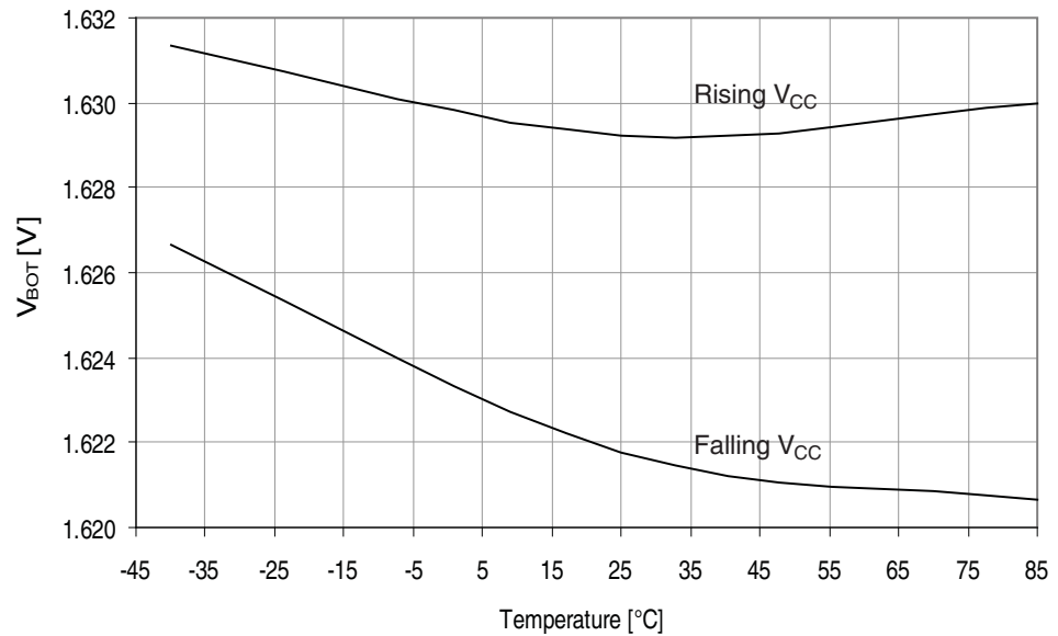
Figure 38-60. BOD thresholds vs. temperature.
