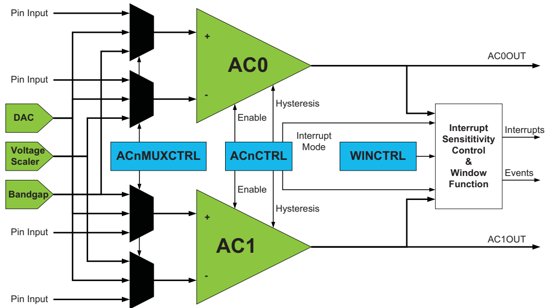
Figure 31-1. Analog comparator overview.
