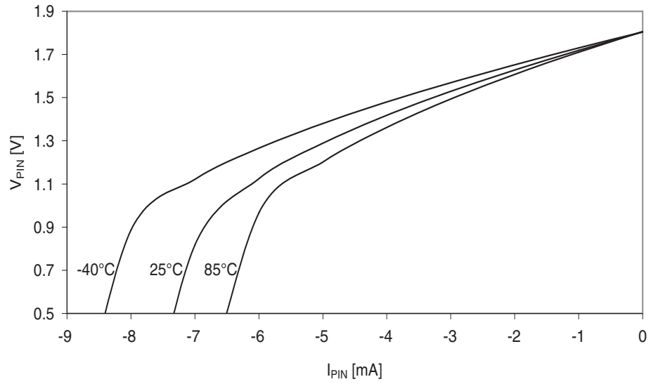
Figure 38-23. I/O pin output voltage vs. source current. V_{CC} = 1.8V .
