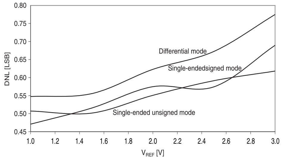
Figure 38-38. DNL error vs. external V_{REF} .
