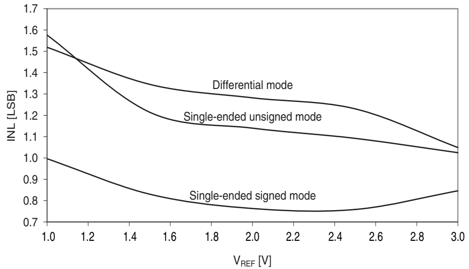
Figure 38-35. INL error vs. external V_{REF} . T = 25^{\circ}\text{C} , V_{CC} = 3.6\text{V} , external reference.
