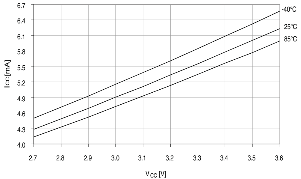
Figure 38-14. Idle mode current vs. V_{CC} . f_{SYS} = 32\text{MHz} internal oscillator.
