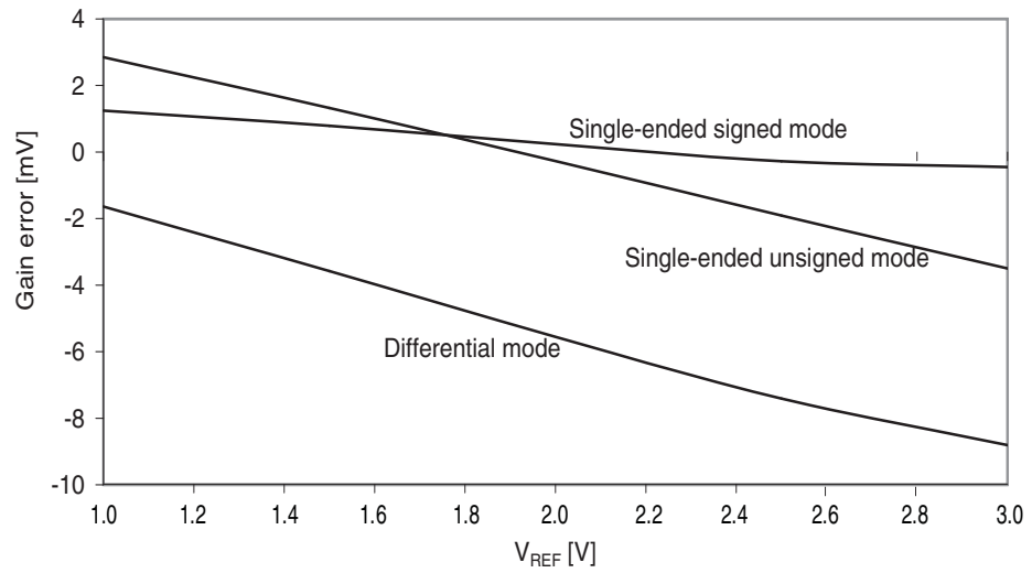
Figure 38-41. Gain error vs. V_{REF} . T = 25^{\circ}\text{C} , V_{CC} = 3.6\text{V} , ADC sampling speed = 500ksps.
