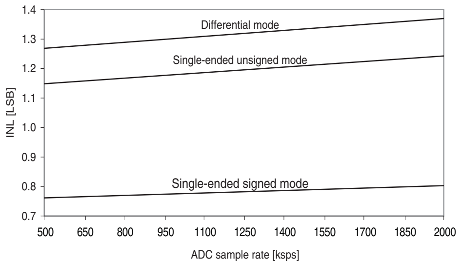
Figure 38-36. INL error vs. sample rate. T = 25^{\circ}\text{C} , V_{CC} = 3.6\text{V} , V_{REF} = 3.0\text{V} external.
