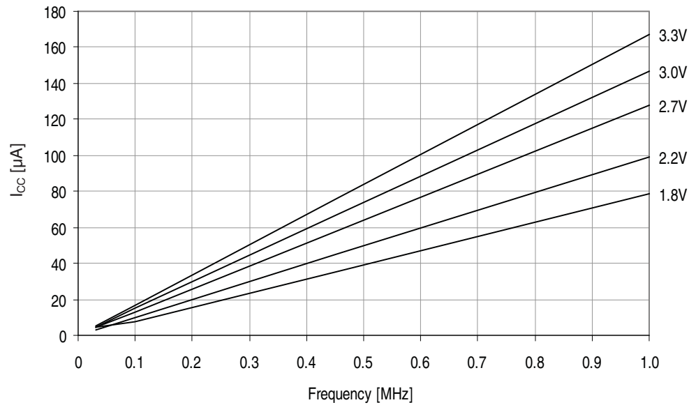
Figure 38-8. Idle mode supply current vs. frequency. f_{SYS} = 0 - 1\text{MHz} external clock, T = 25^{\circ}\text{C} .
