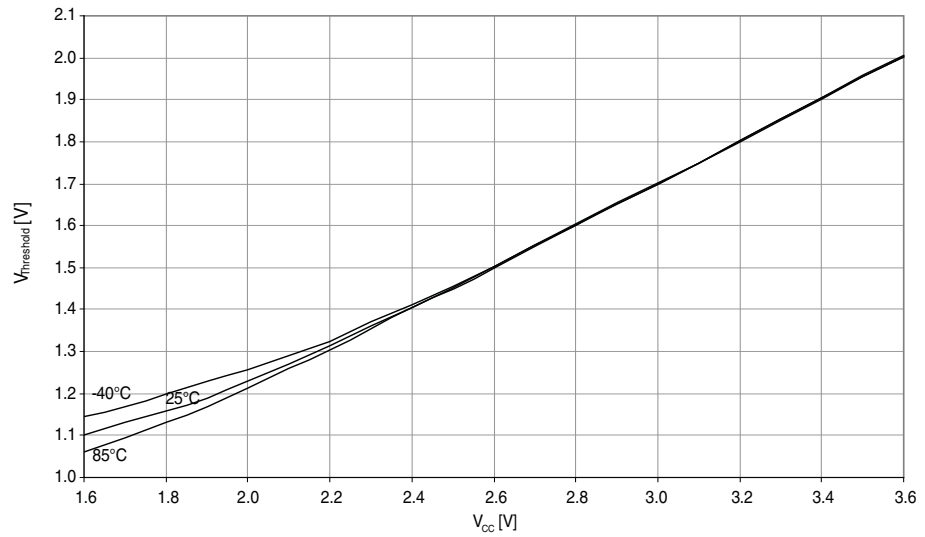
Figure 38-65. Reset pin input threshold voltage vs. V_{CC} .
