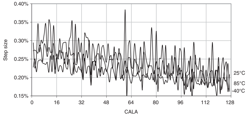
Figure 38-80. 48MHz internal oscillator CALA calibration step size.
