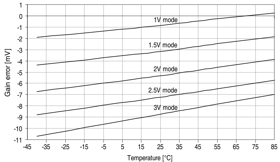
Figure 38-44. Gain error vs. temperature.
