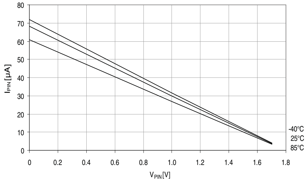
Figure 38-20. I/O pin pull-up resistor current vs. input voltage. V_{CC} = 1.8V .
