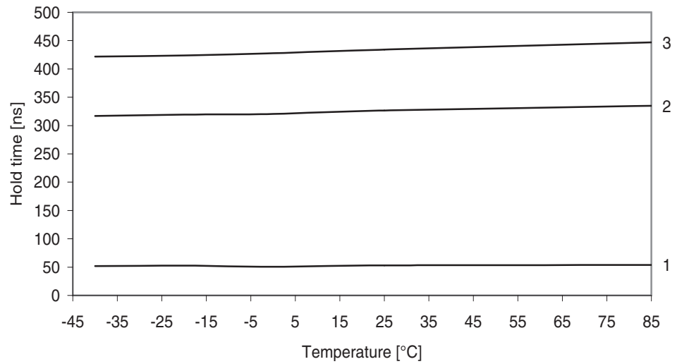
Figure 38-81. SDA hold time vs. temperature.
