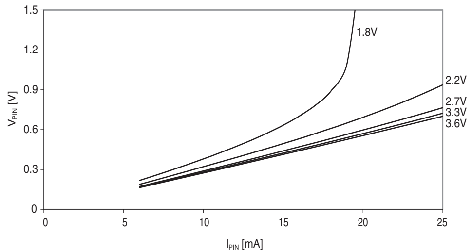
Figure 38-30. I/O pin output voltage vs. sink current.
