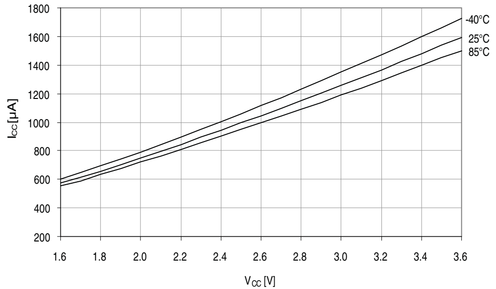
Figure 38-5. Active mode supply current vs. V_{CC} .
