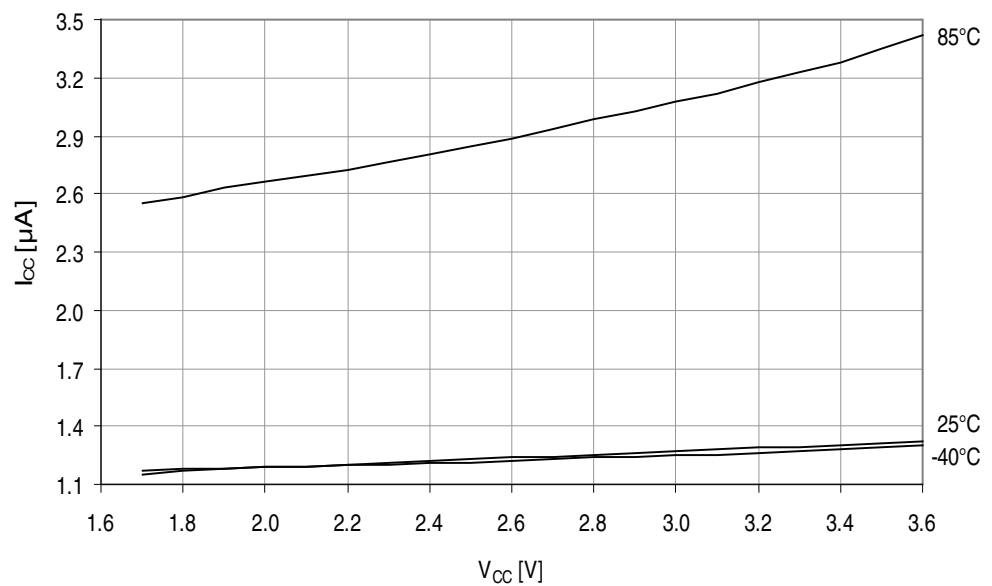
Figure 38-16. Power-down mode supply current vs. V_{CC} . Watchdog and sampled BOD enabled.
