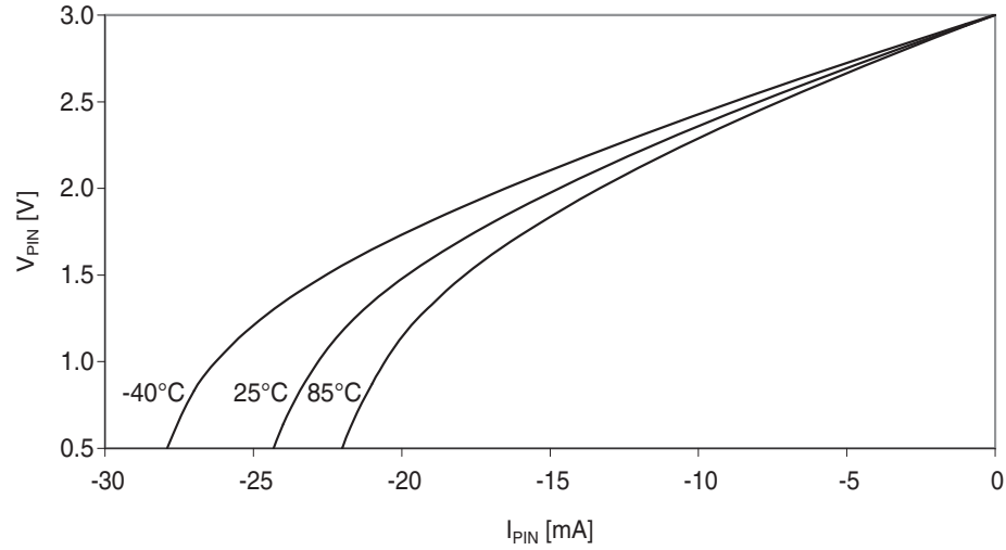
Figure 38-24. I/O pin output voltage vs. source current. V_{CC} = 3.0V .
