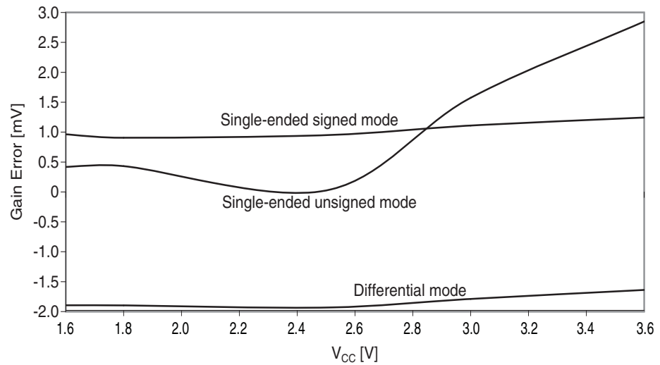
Figure 38-42. Gain error vs. V_{CC} . T = 25^{\circ}\text{C} , V_{REF} = \text{external } 1.0\text{V} , ADC sampling speed = 500ksps.
