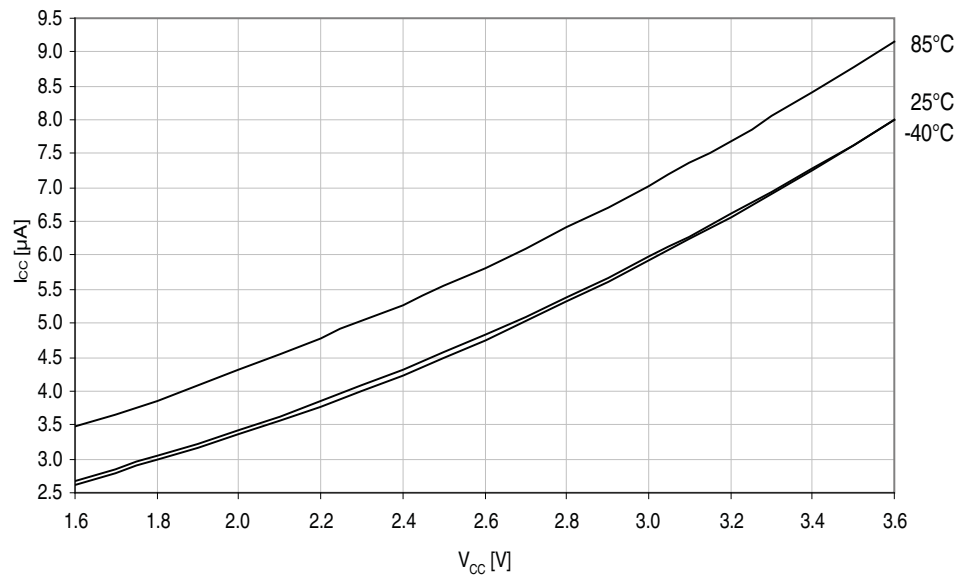
Figure 38-18. Standby supply current vs. V_{CC} .
