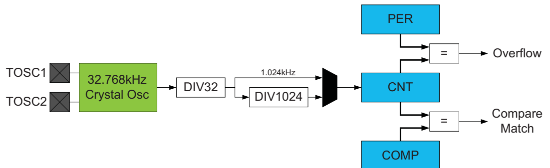
Figure 21-1. Real Time Counter overview.
