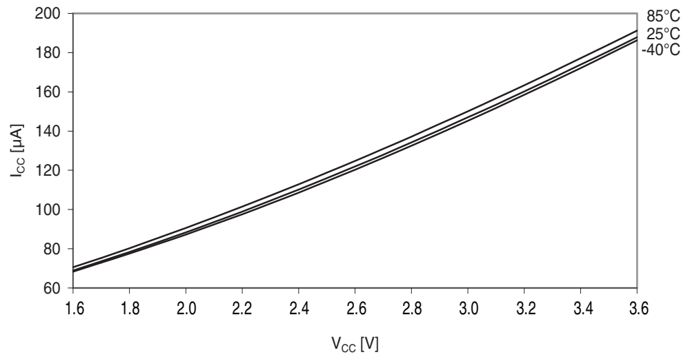
Figure 38-12. Idle mode supply current vs. V_{CC} .
