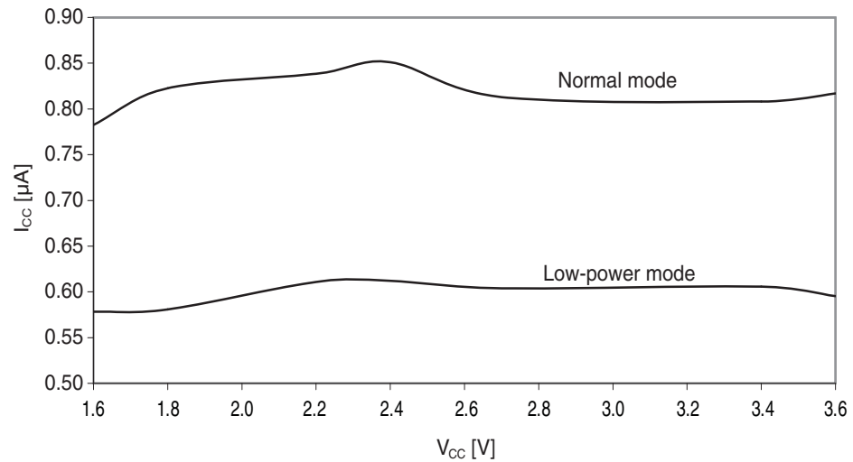
Figure 38-17. Power-save mode supply current vs. V_{CC} .
