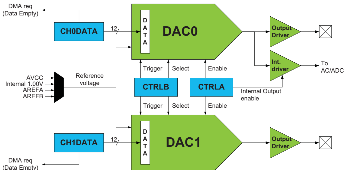
Figure 30-1. DAC overview.
