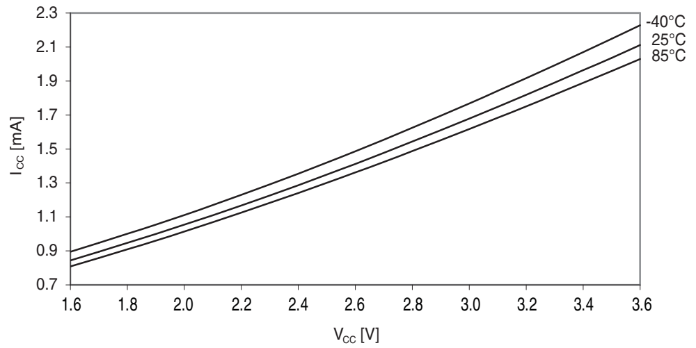
Figure 38-13. Idle mode supply current vs. V_{CC} . f_{SYS} = 32\text{MHz} internal oscillator prescaled to 8MHz.
