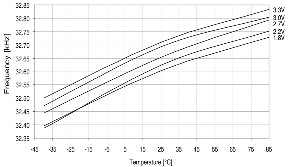
Figure 38-69. 32.768kHz internal oscillator frequency vs. temperature.
