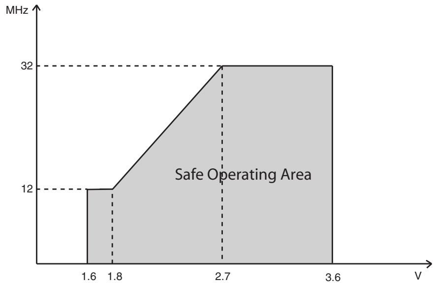
Figure 37-1. Maximum frequency vs. V CC .
