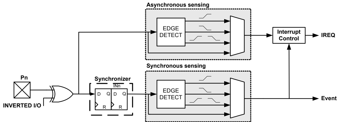
Figure 16-7. Input sensing system overview.
