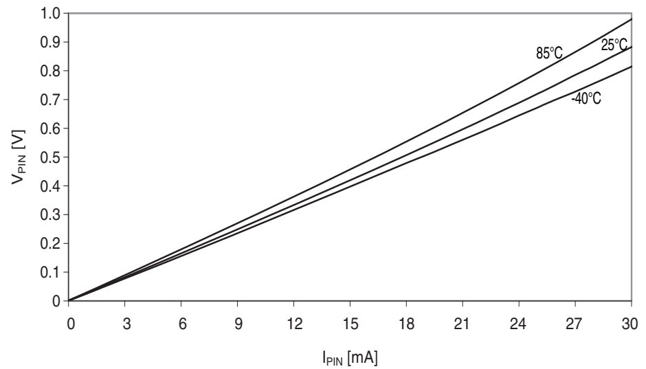
Figure 38-28. I/O pin output voltage vs. sink current.
