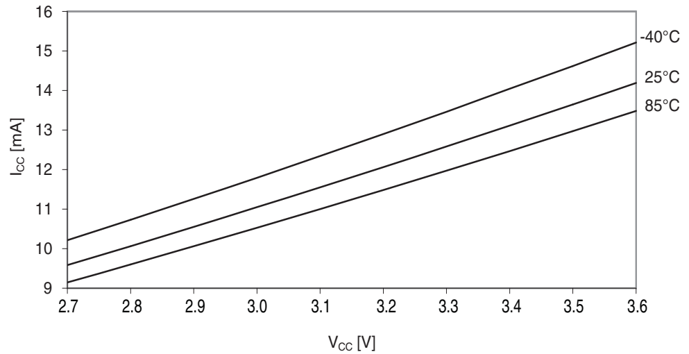
Figure 38-7. Active mode supply current vs. V_{CC} . f_{SYS} = 32\text{MHz} internal oscillator.
