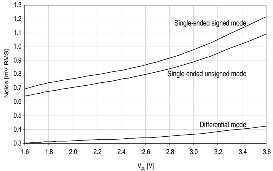
Figure 38-47. Noise vs. V_{CC} .
