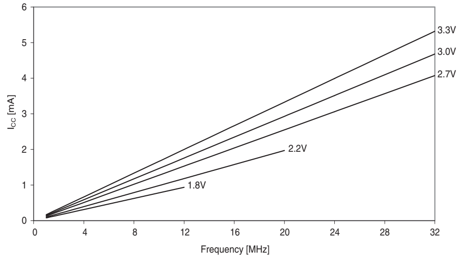
Figure 38-9. Idle mode supply current vs. frequency.
