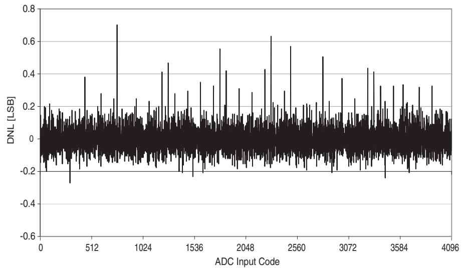
Figure 38-40. DNL error vs. input code.
