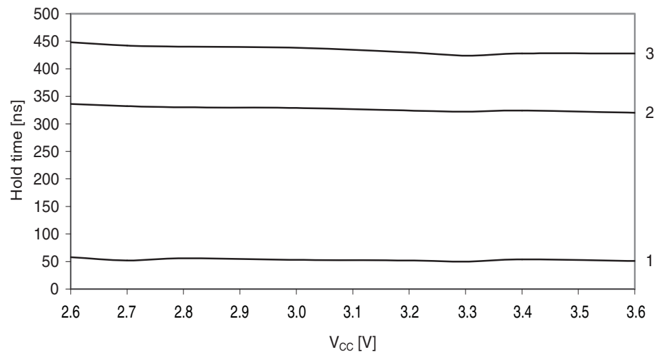
Figure 38-82. SDA hold time vs. supply voltage.
