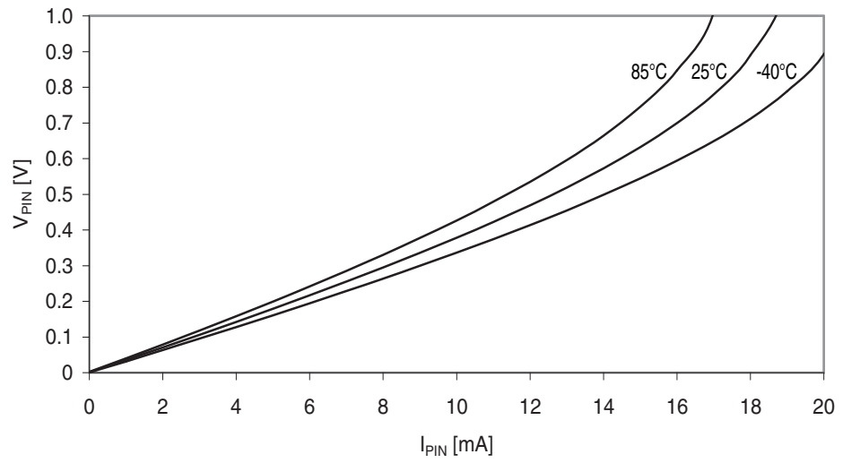
Figure 38-28. I/O pin output voltage vs. sink current.
