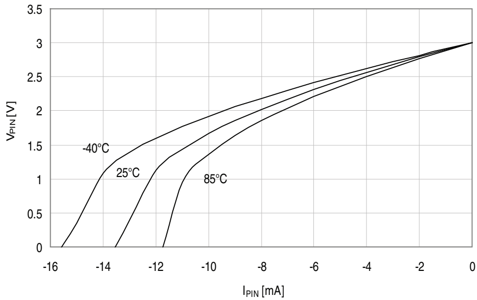
Figure 36-22. I/O pin output voltage vs. source current.
