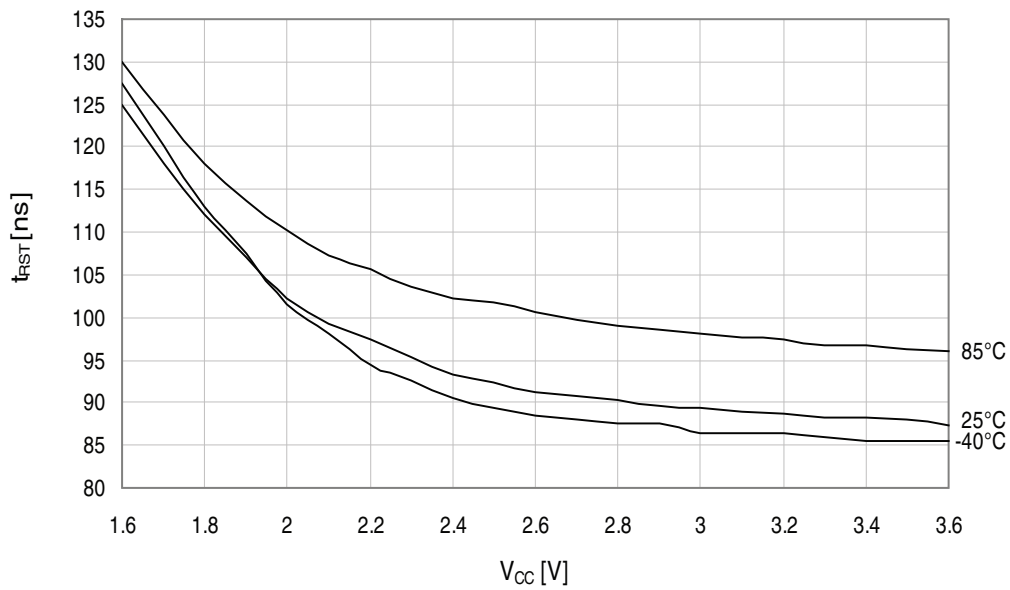
Figure 36-48. Minimum Reset pin pulse width vs. V_{CC} .
