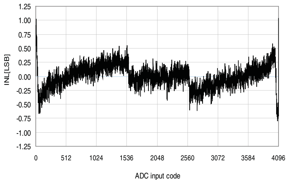
Figure 37-26. INL error vs. input code.
