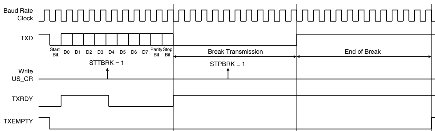
Figure 32-16. Break Transmission
