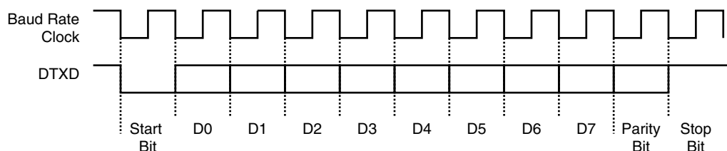
Figure 28-10. Character Transmission
