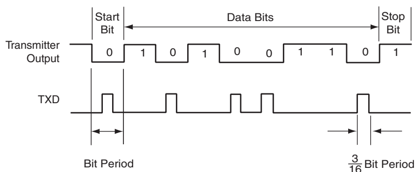
Figure 32-24. IrDA Modulation
