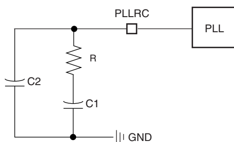
Figure 24-5. PLL Capacitors and Resistors
