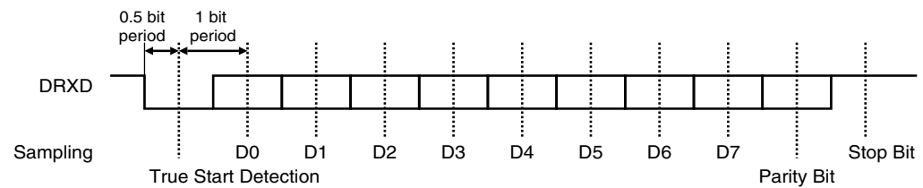
Figure 28-5. Character Reception
