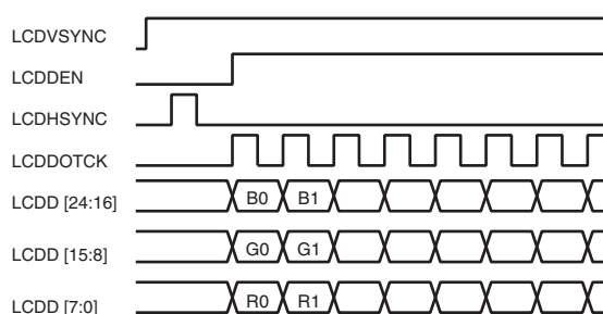
Figure 38-6. TFT Timing (First Line Expanded View)
