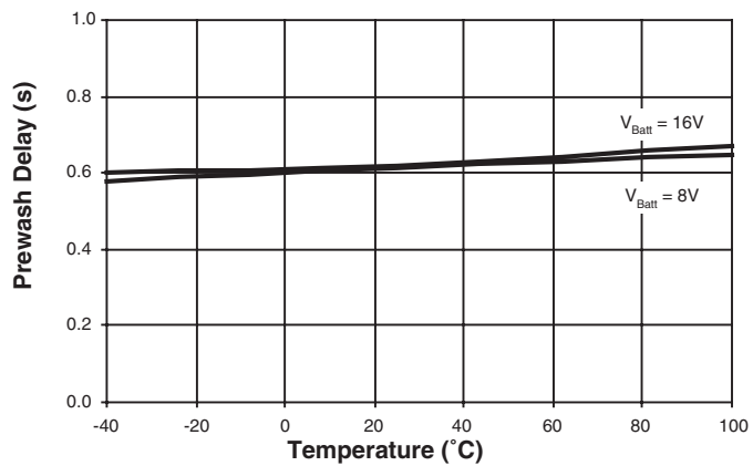
Figure 8-3. Prewash Time = f(T) ; C_t = 22 \mu\text{F}
