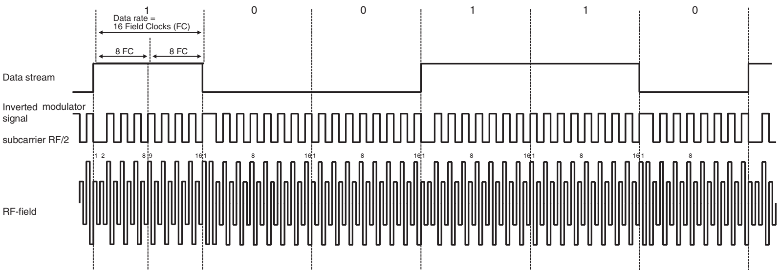
Figure 5-8. Example of PSK Coding with Data Rate RF/16
