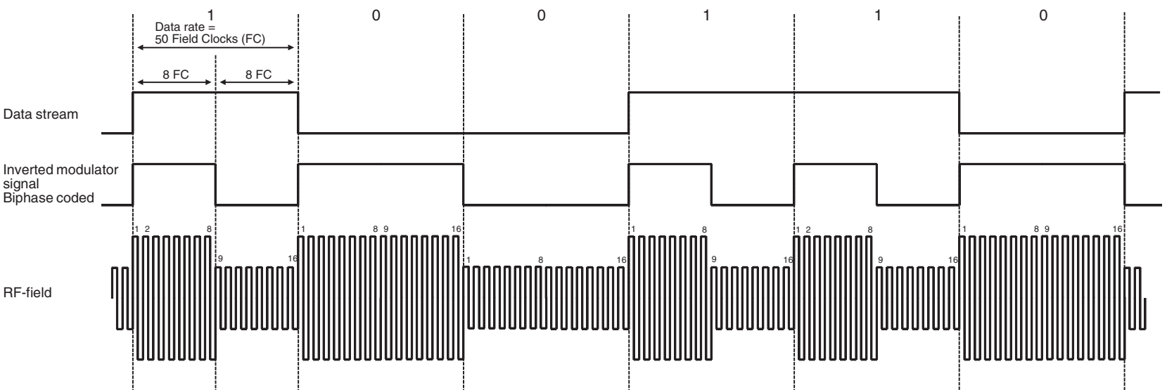
Figure 5-6. Example of Biphas Coding with Data Rate RF/16
