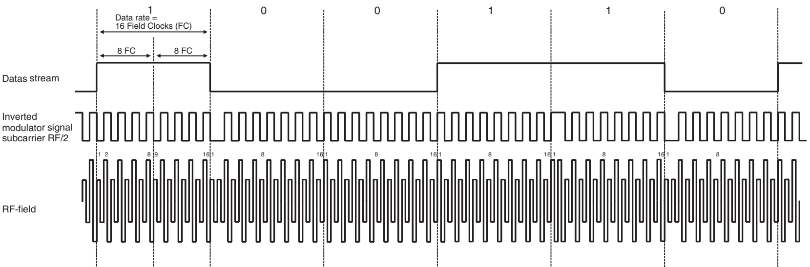
Figure 5-9. Example of PSK2 Coding with Data Rate RF/16
