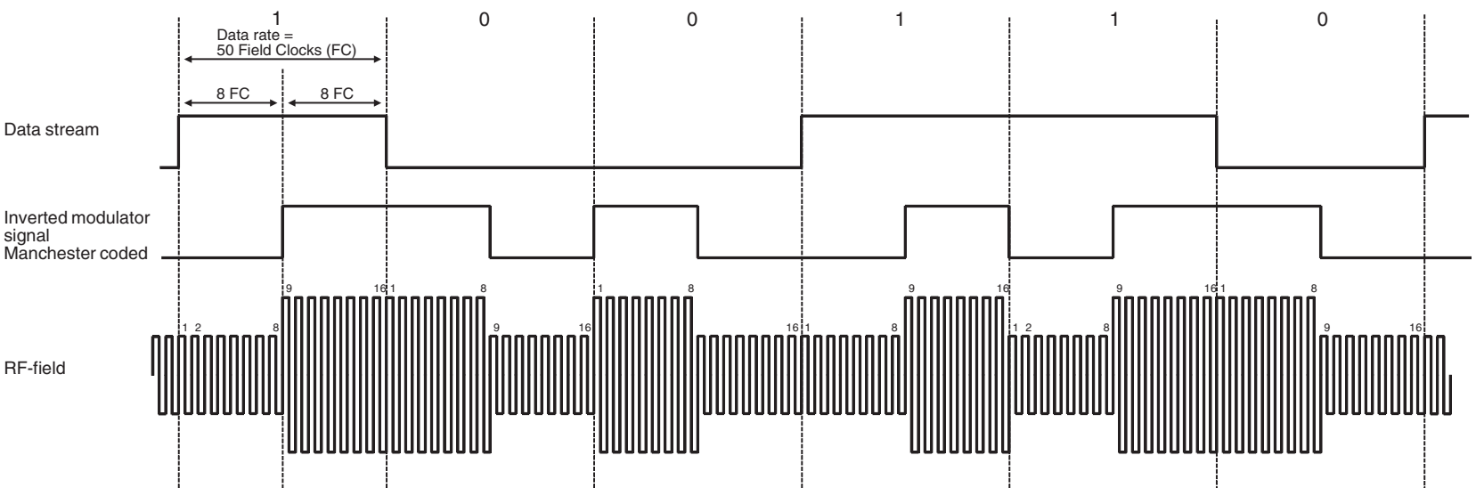
Figure 5-5. Example of Manchester Coding with Data Rate RF/16
