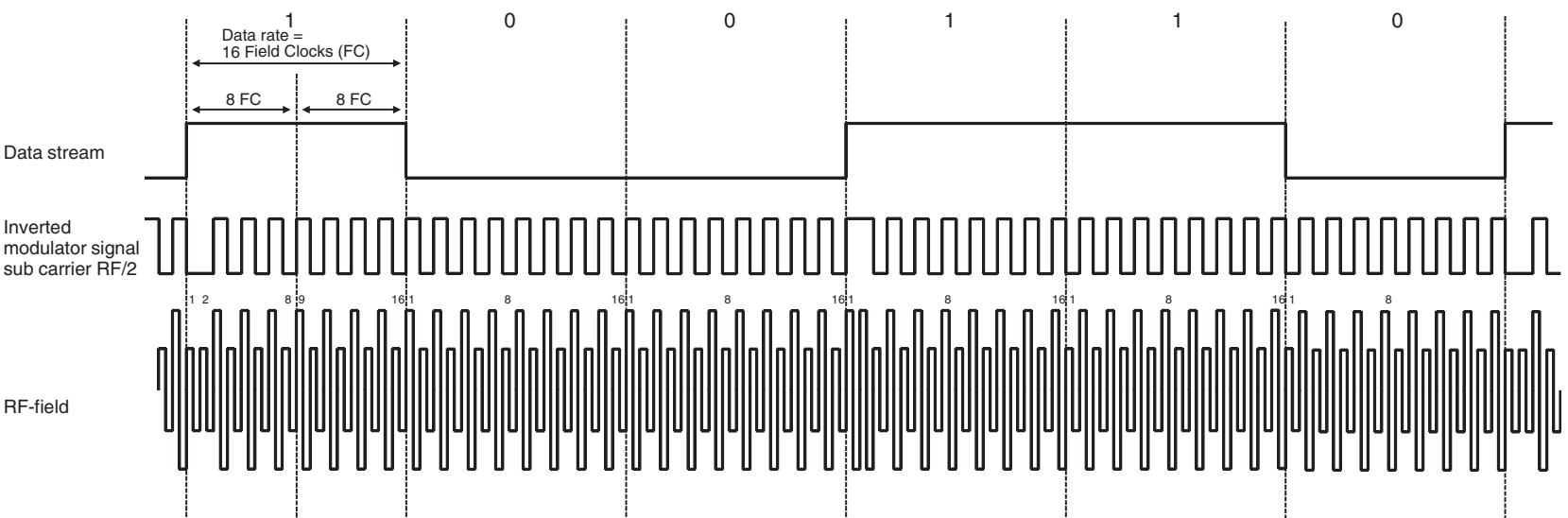
Figure 5-10. Example of PSK3 Coding with Data Rate RF/16
