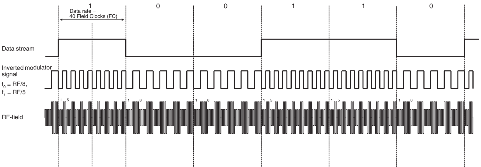
Figure 5-7. Example of FSK Coding with Data Rate RF/40 , Subcarrier f_0 = RF/8 , f_1 = RF/5
