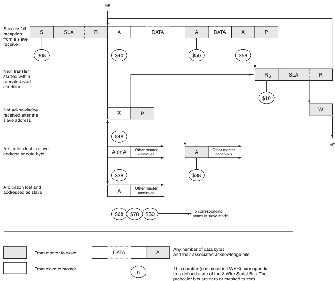
Figure 15-14. Formats and States in the Master Receiver Mode
