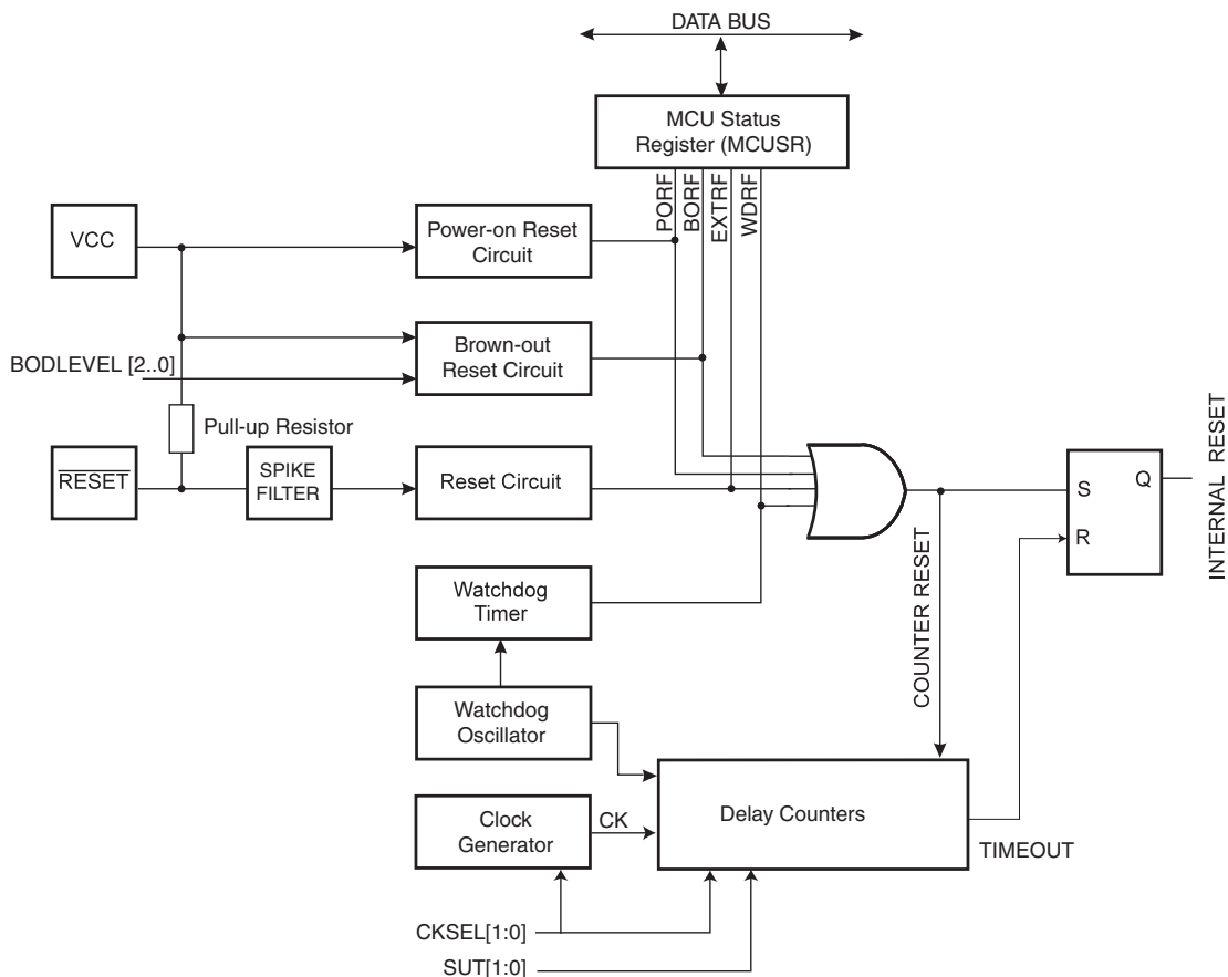
Figure 8-1. Reset Logic
