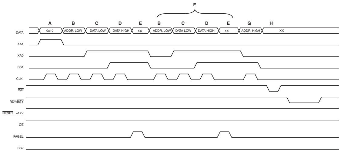
Figure 20-3. Programming the Flash Waveforms (1)
