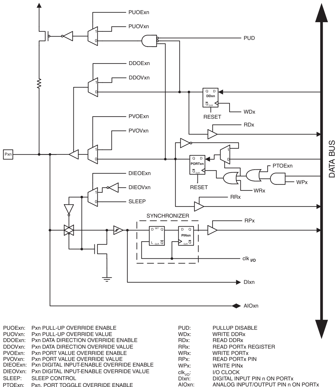
Figure 11-5. Alternate Port Functions (1)
