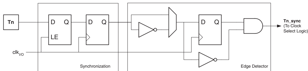
Figure 13-1. T_n Pin Sampling
