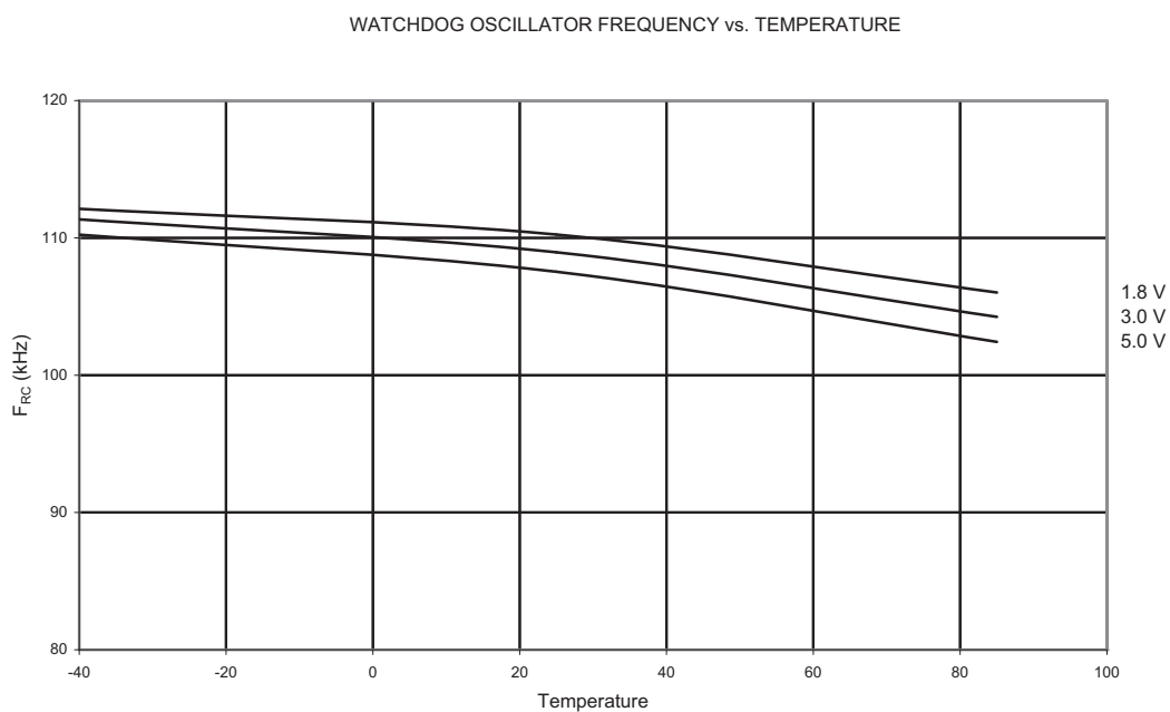
Figure 21-49. Frequency of Watchdog Oscillator vs. Temperature
