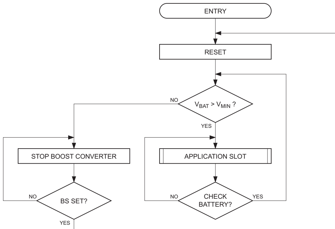
Figure 8-9. Block Diagram of Typical Program.
