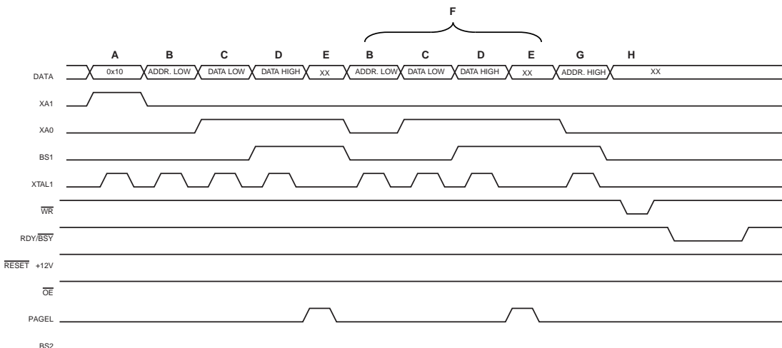
Figure 23-3. Flash Programming Waveforms
