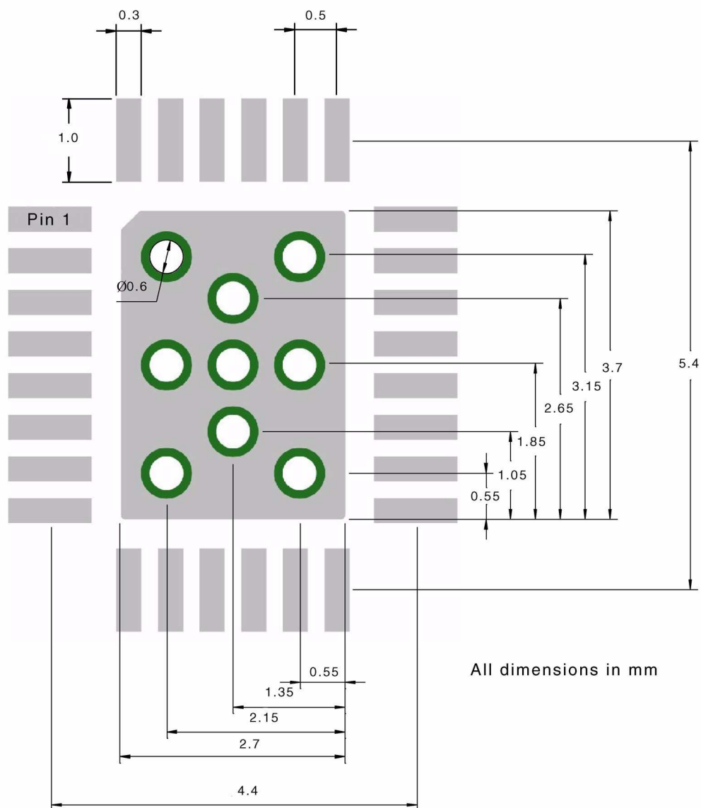
Figure 8-4. Recommended Footprint
