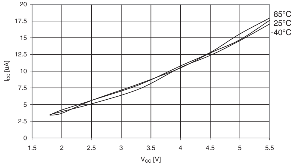
Figure 29-299. ATmega3250A: Watchdog Timer Current vs. V_{CC}
