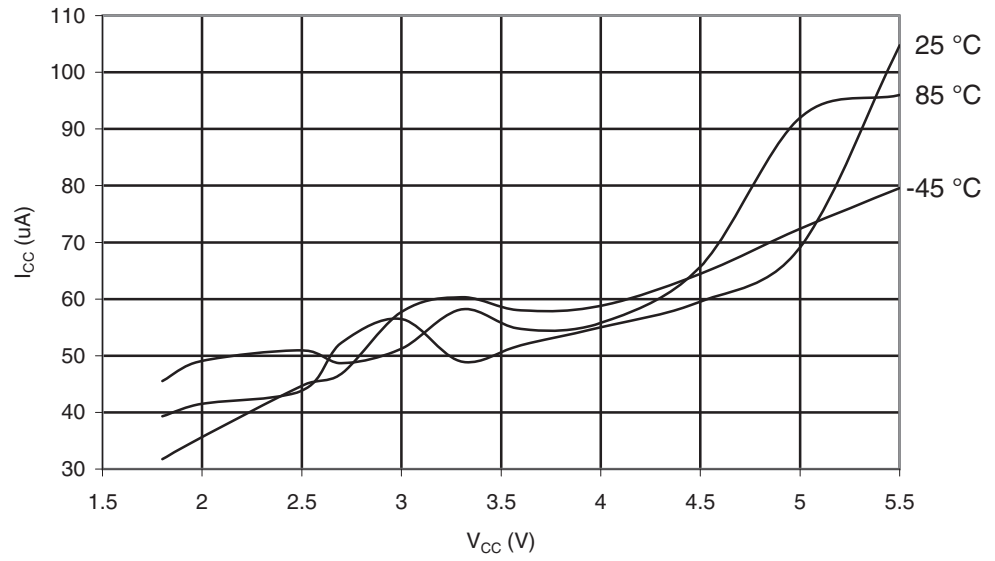
Figure 29-482. ATmega645P: Analog Comparator Current vs. V_{CC}
