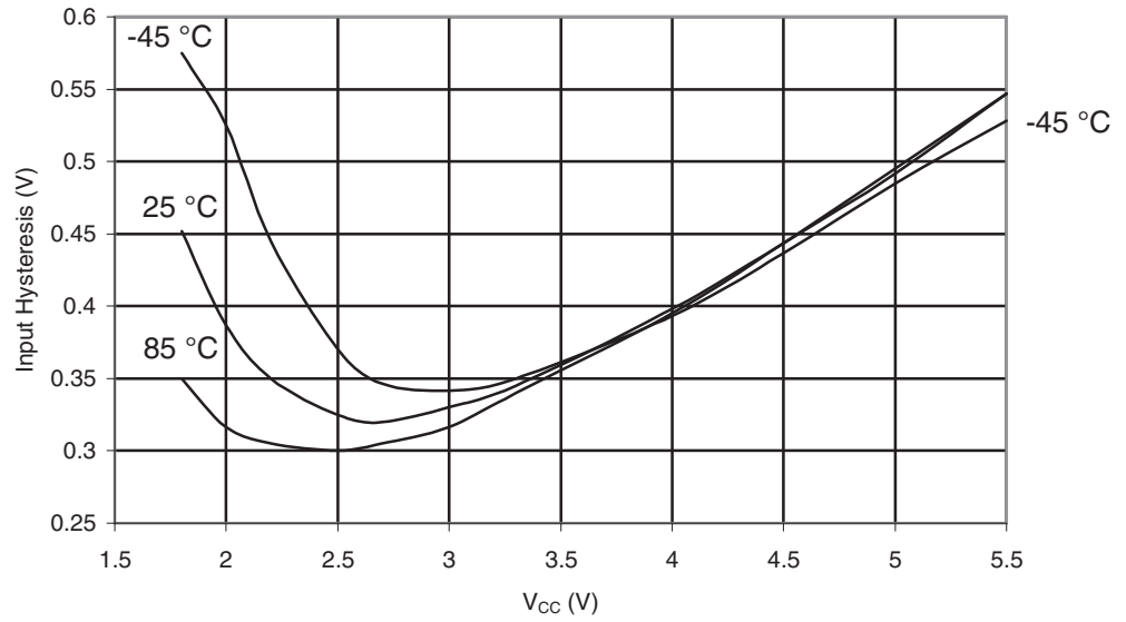
Figure 29-523. ATmega6450A: I/O Pin Input Hysteresis vs. V_{CC}
