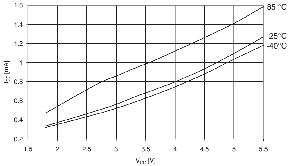
Figure 29-308. ATmega3250PA: Active Supply Current vs. V_{CC} (Internal RC Oscillator, 1MHz)
