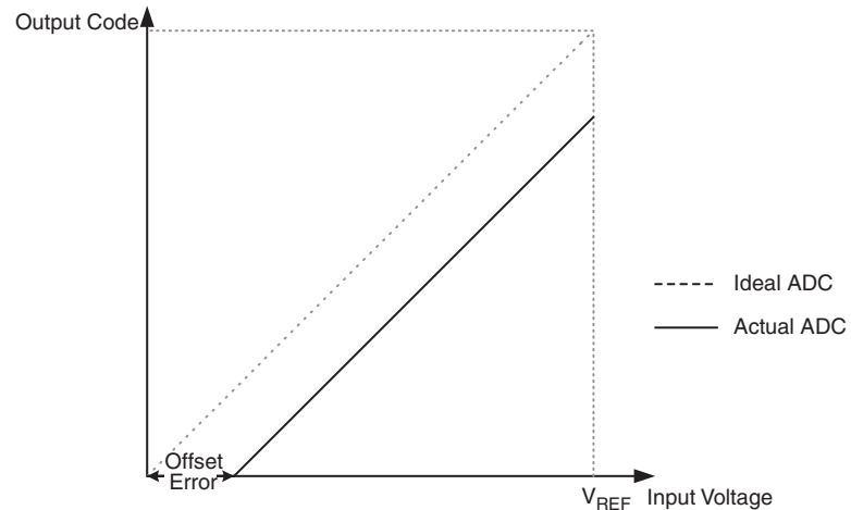
Figure 23-10. Offset Error
