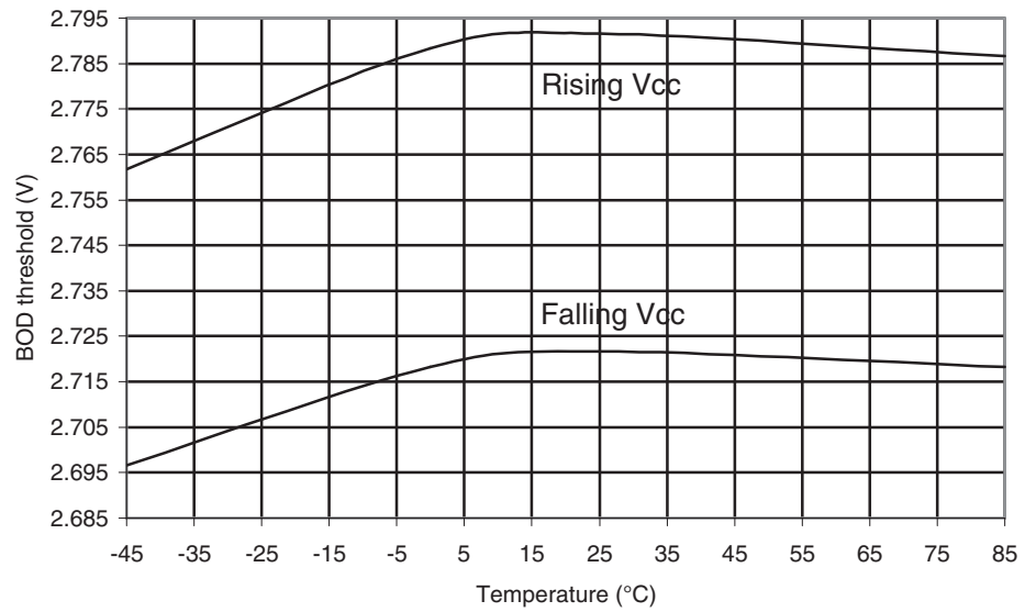
Figure 29-467. ATmega645P: BOD Thresholds vs. Temperature (BOD Level is 2.7V)
