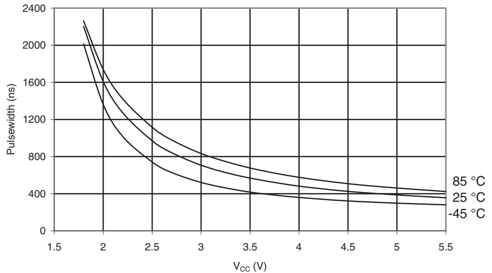
Figure 29-124. ATmega165PA: Minimum Reset Pulse Width vs. V_{CC}
