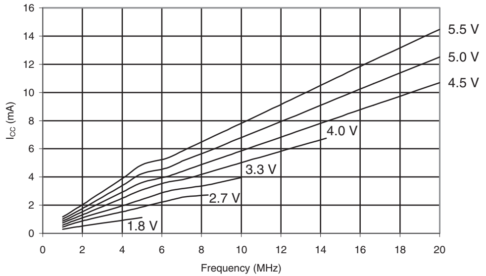
Figure 29-488. ATmega6450A: Active Supply Current vs. Frequency (1 - 20MHz)
