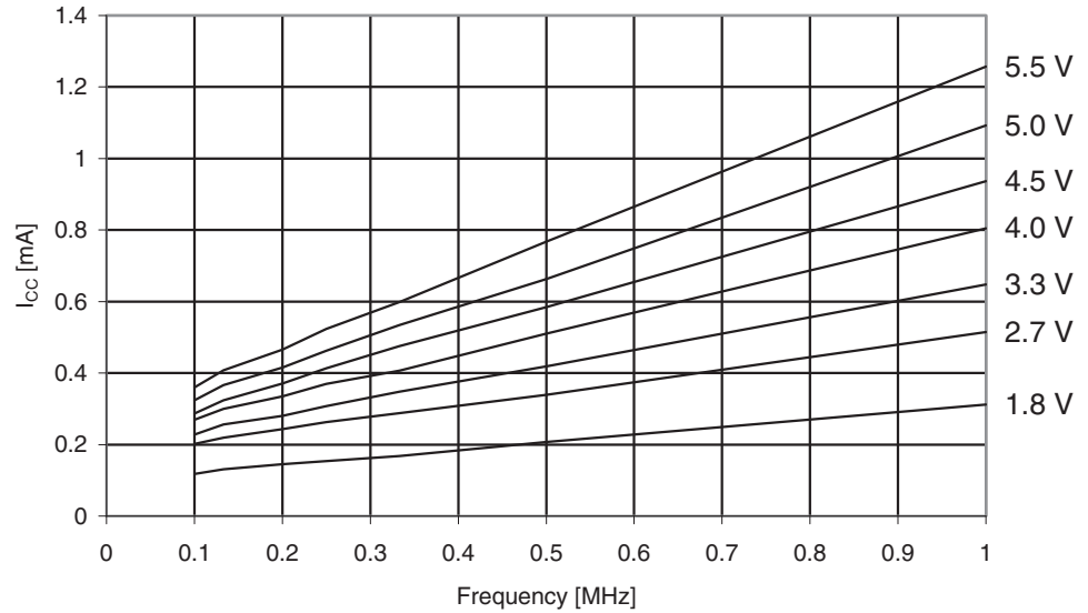
Figure 29-245. ATmega3250A: Active Supply Current vs. Frequency (0.1 - 1.0MHz)
