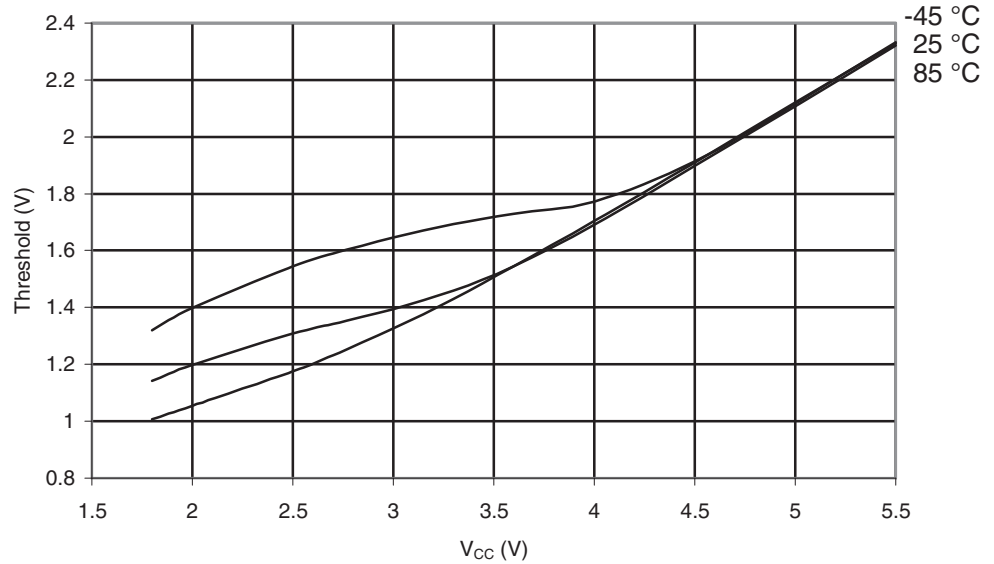
Figure 29-585. ATmega6450P: Reset Input Threshold Voltage vs. V_{CC} ( V_{IH} , Reset Pin Read as "1")
