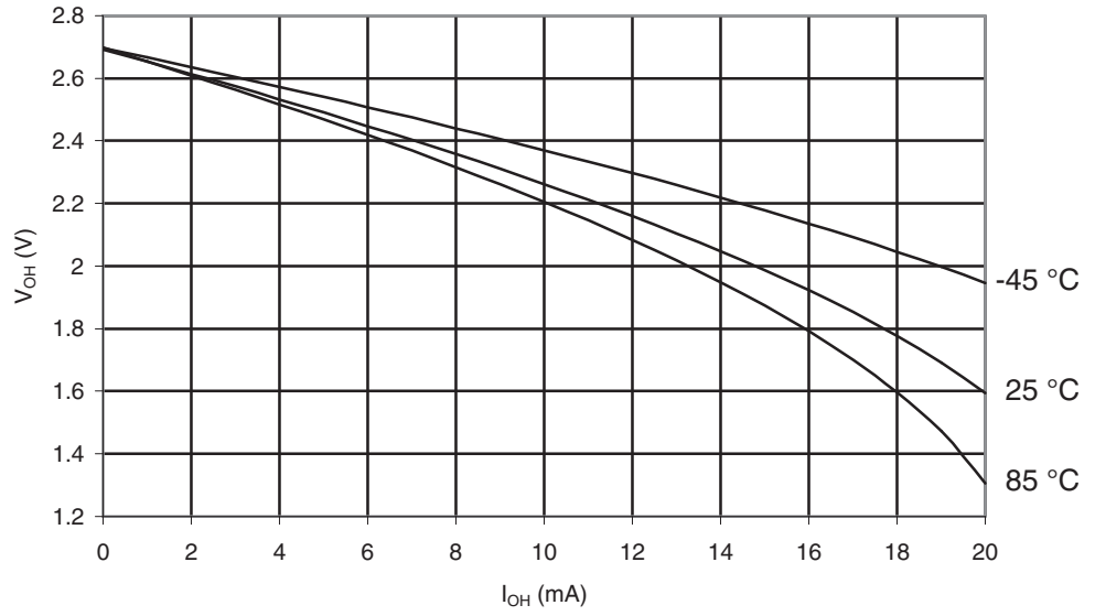
Figure 29-391. ATmega645A: I/O Pin Output Voltage vs. Source Current, Port B ( V_{CC} = 2.7V )
