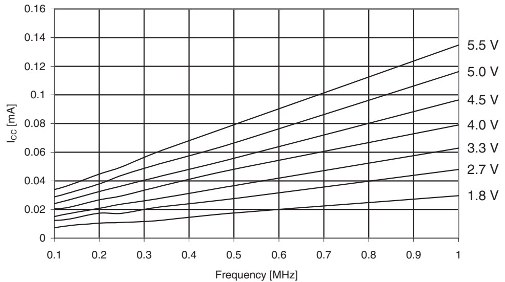
Figure 29-362. ATmega3250PA: Reset Supply Current vs. V_{CC} (0.1 - 1.0MHz, Excluding Current Through The Reset Pull-up)
