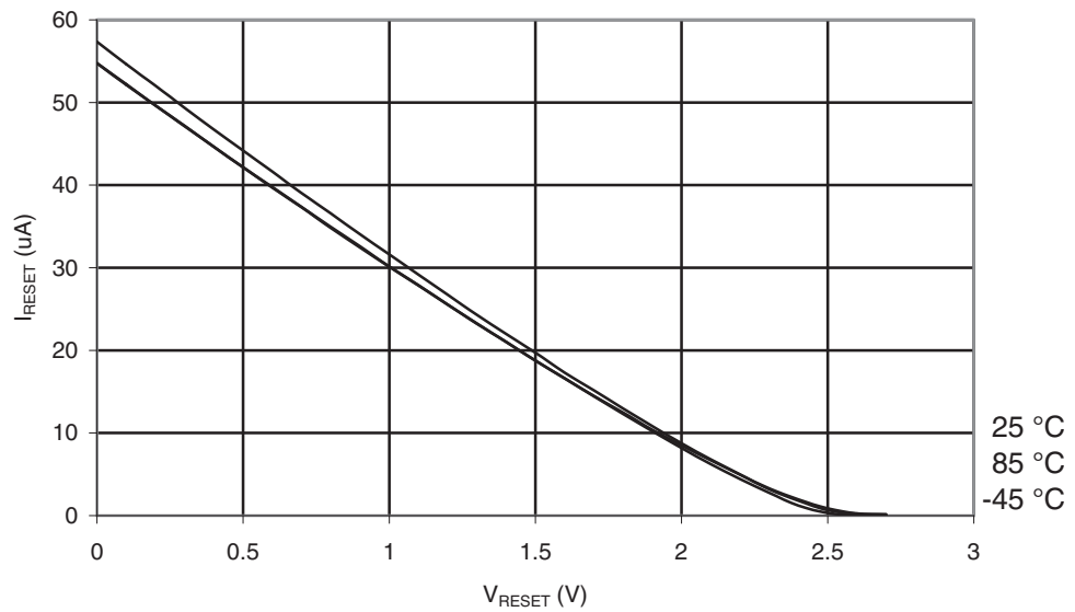
Figure 29-82. ATmega165PA: Reset Pull-up Resistor Current vs. Reset Pin Voltage ( V_{CC} = 2.7V )
