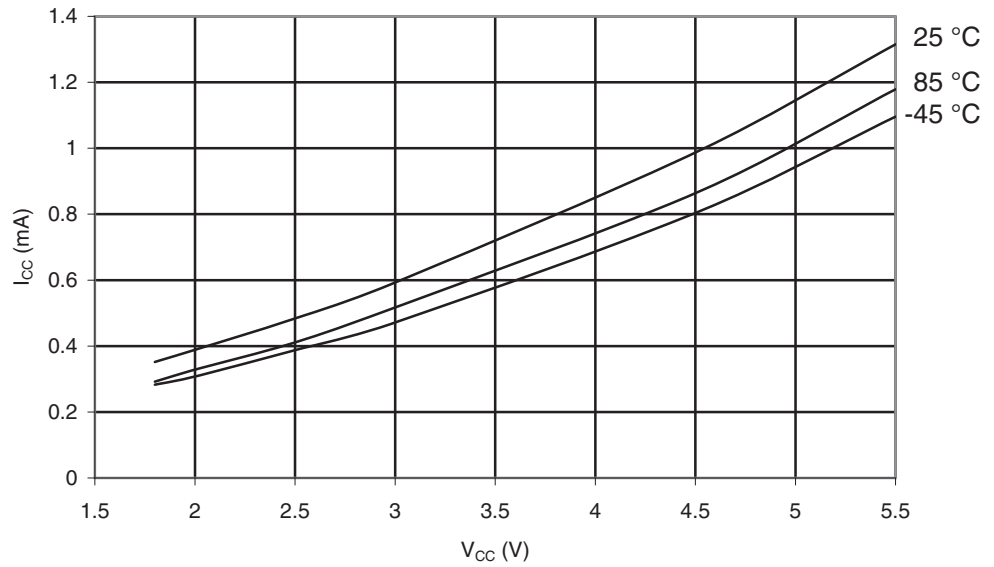
Figure 29-4. ATmega165A: Active Supply Current vs. V_{CC} (Internal RC Oscillator, 1MHz)
