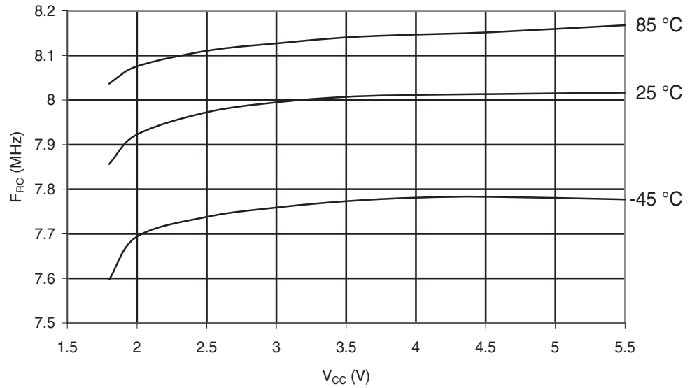
Figure 29-112. ATmega165PA: Calibrated 8MHz RC Oscillator Frequency vs. V_{CC}
