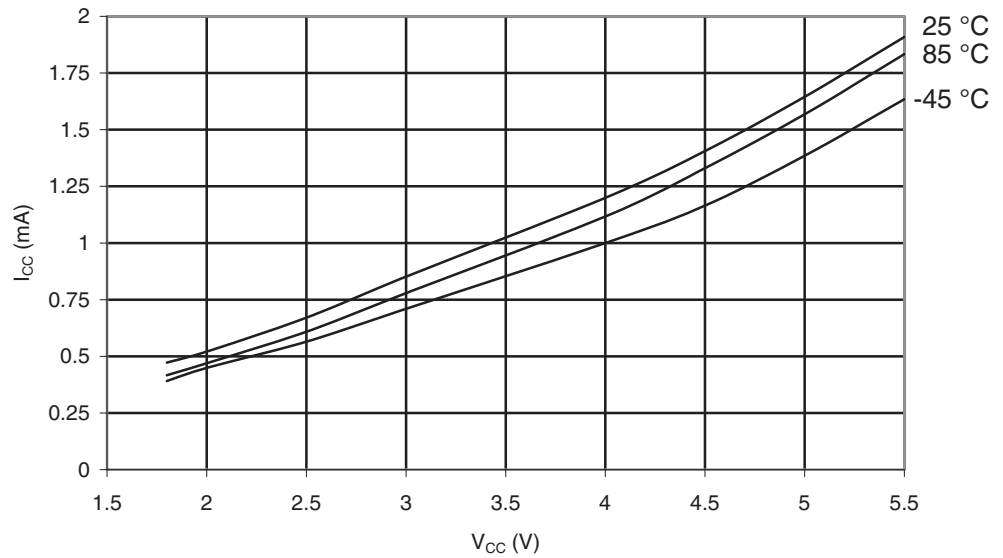
Figure 29-8. ATmega165A: Idle Supply Current vs. V_{CC} (Internal RC Oscillator, 8MHz)
