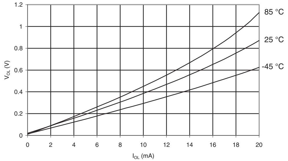
Figure 29-580. ATmega6450P: I/O Pin Output Voltage vs. Sink Current, Port B ( V_{CC} = 2.7V )
