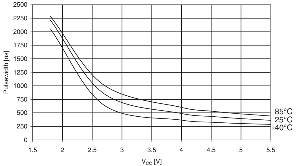
Figure 29-364. ATmega3250PA: Minimum Reset Pulse Width vs. V_{CC}
