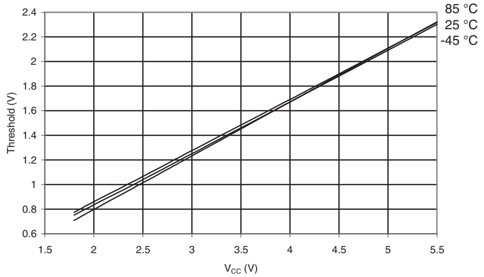
Figure 29-586. ATmega6450P: Reset Input Threshold Voltage vs. V_{CC} ( V_{IL,Reset} Pin Read as "0")
