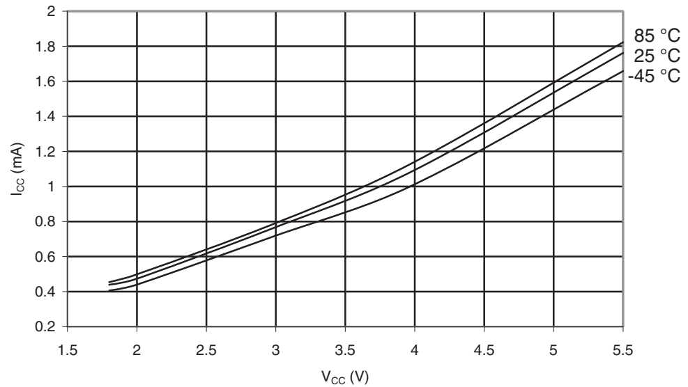
Figure 29-555. ATmega6450A: Idle Supply Current vs. V_{CC} (Internal RC Oscillator, 8MHz)
