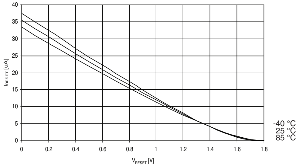
Figure 29-205. ATmega325PA: Reset Pull-up Resistor Current vs. Reset Pin Voltage ( V_{CC} = 1.8V )
