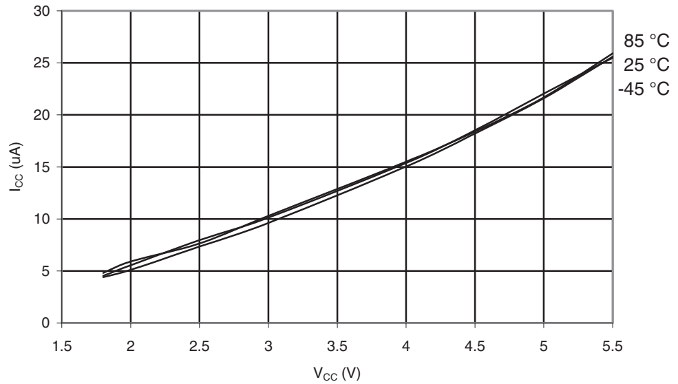
Figure 29-57. ATmega165A: Watchdog Timer Current vs. V_{CC}
