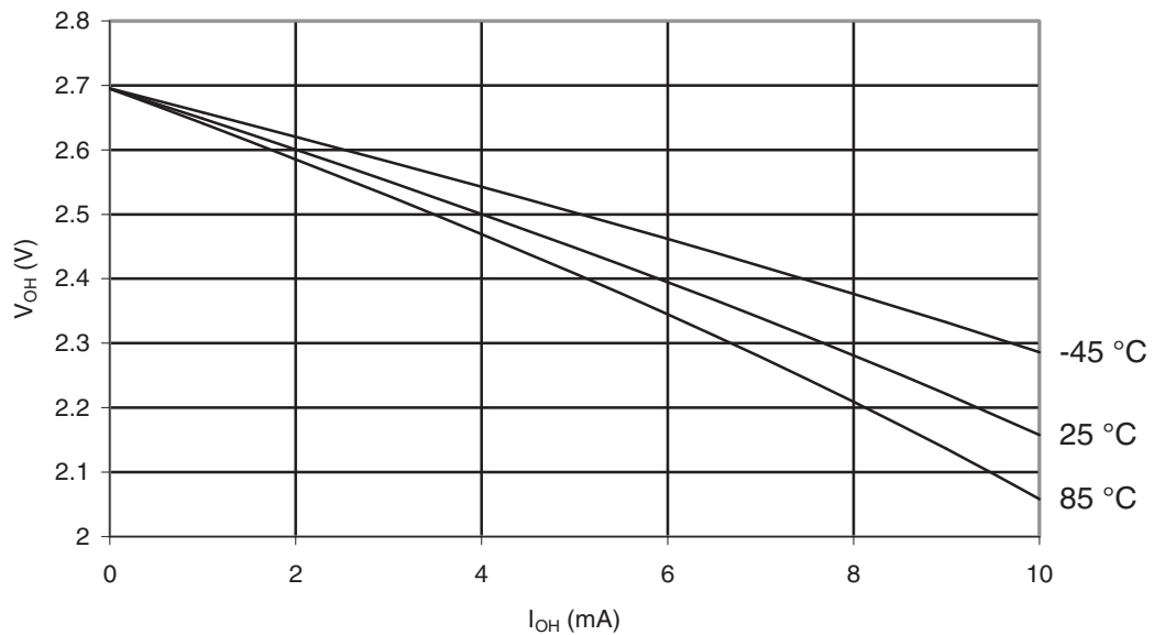
Figure 29-23. ATmega165A: I/O Pin Output Voltage vs. Source Current, Ports A, C, D, E, F, G ( V_{CC} = 2.7V )
