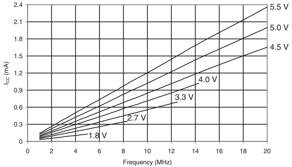
Figure 29-546. ATmega6450A: Reset Supply Current vs. V_{CC} (1 - 16MHz, Excluding Current Through The Reset Pull-up)
