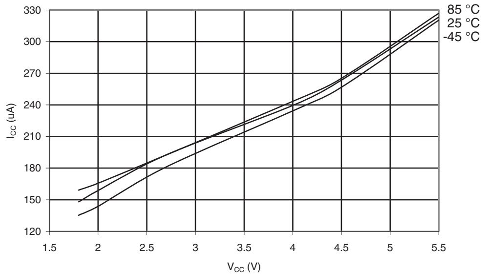
Figure 29-416. ATmega645A: Active Supply Current with ADC at 50kHz vs. V_{CC}
