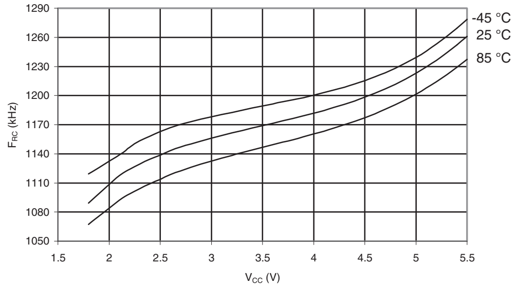
Figure 29-410. ATmega645A: Watchdog Oscillator Frequency vs. V_{CC}
