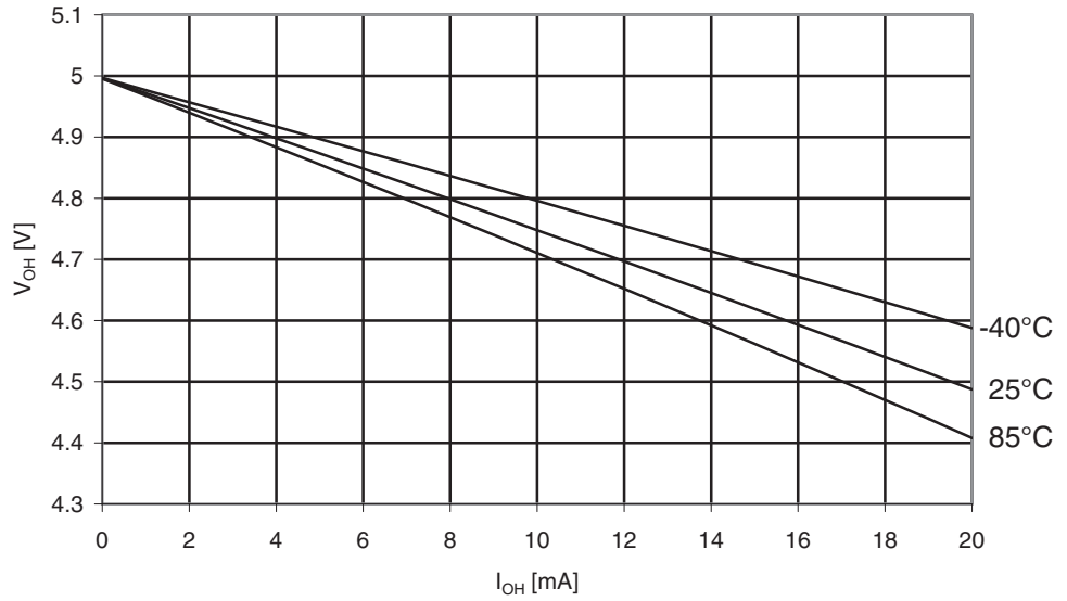
Figure 29-209. ATmega325PA: I/O Pin Output Voltage vs. Source Current, Port B ( V_{CC} = 5V )
