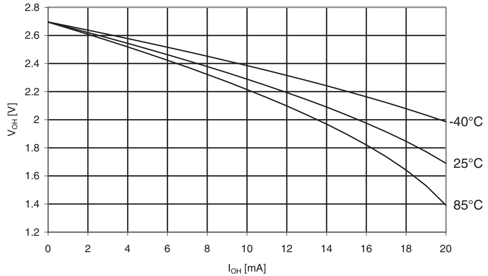
Figure 29-210. ATmega325PA: I/O Pin Output Voltage vs. Source Current, Port B ( V_{CC} = 2.7V )
