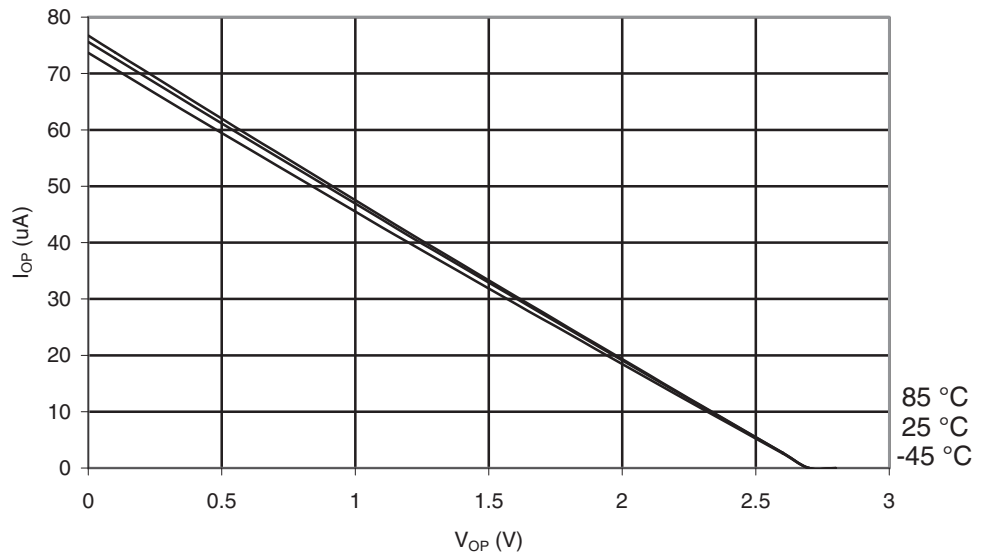
Figure 29-17. ATmega165A: I/O Pin Pull-up Resistor Current vs. Input Voltage ( V_{CC} = 2.7V )
