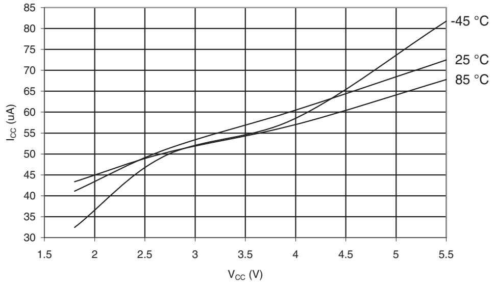
Figure 29-58. ATmega165A: Analog Comparator Current vs. V_{CC}
