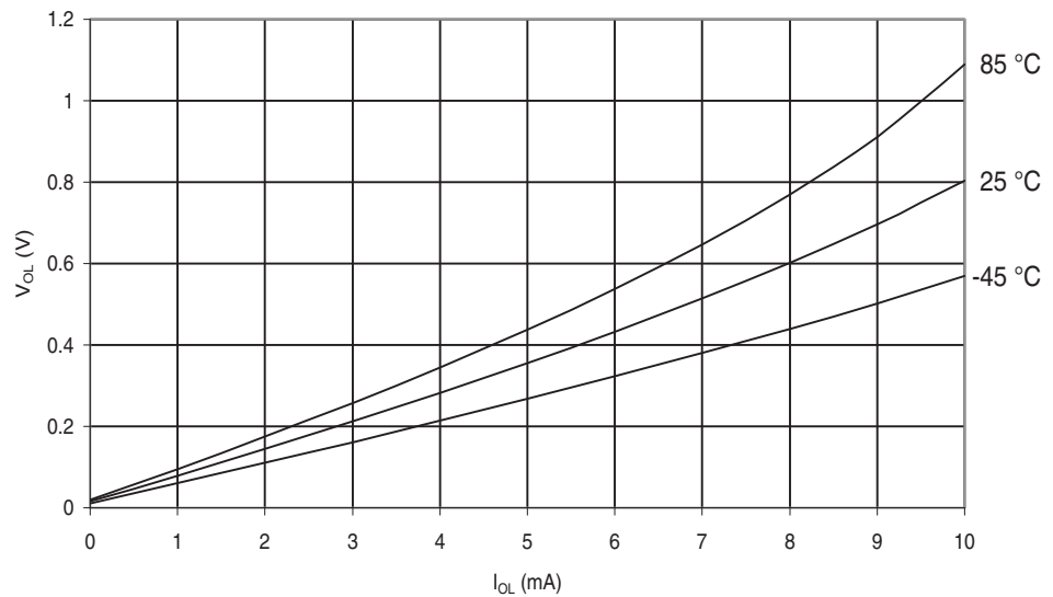
Figure 29-516. ATmega6450A: I/O Pin Output Voltage vs. Sink Current, Ports A, C, D, E, F, G ( V_{CC} = 2.7V )
