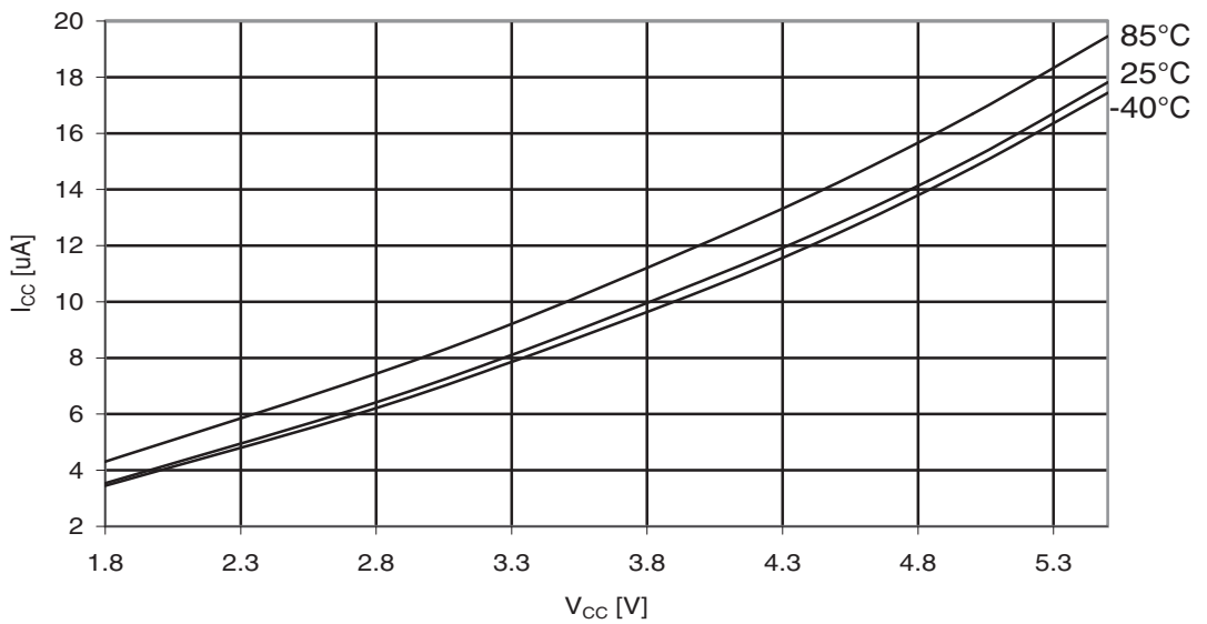
Figure 29-136. ATmega325A: Power-down Supply Current vs. V_{CC} (Watchdog Timer Enabled)
