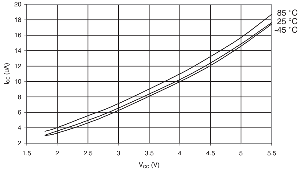
Figure 29-376. ATmega645A: Power-down Supply Current vs. V_{CC} (Watchdog Timer Enabled)
