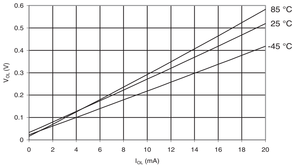
Figure 29-518. ATmega6450A: I/O Pin Output Voltage vs. Sink Current, Port B ( V_{CC} = 5V )
