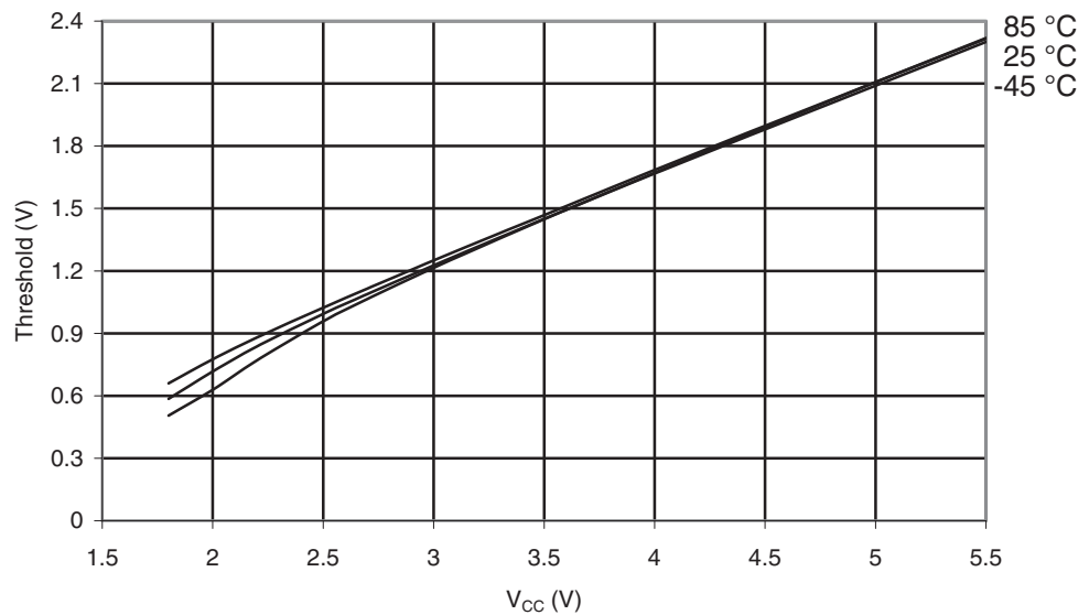
Figure 29-35. ATmega165A: I/O Pin Input Threshold Voltage vs. V_{CC} ( V_{IL} , I/O Pin Read as “0”)
