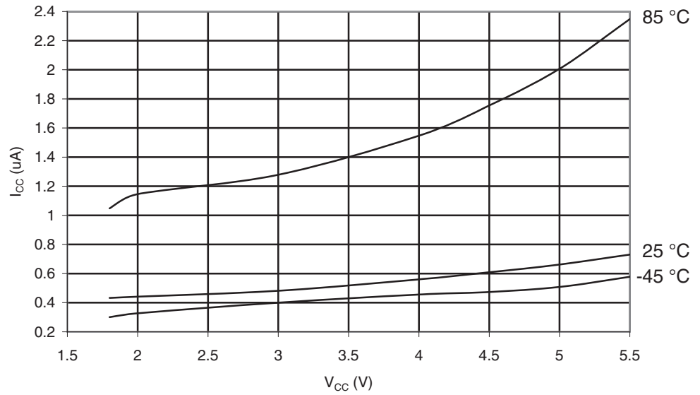
Figure 29-375. ATmega645A: Power-down Supply Current vs. V_{CC} (Watchdog Timer Disabled)
