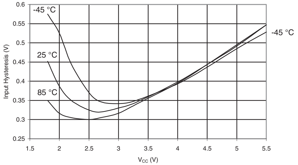
Figure 29-401. ATmega645A: I/O Pin Input Hysteresis vs. V_{CC}
