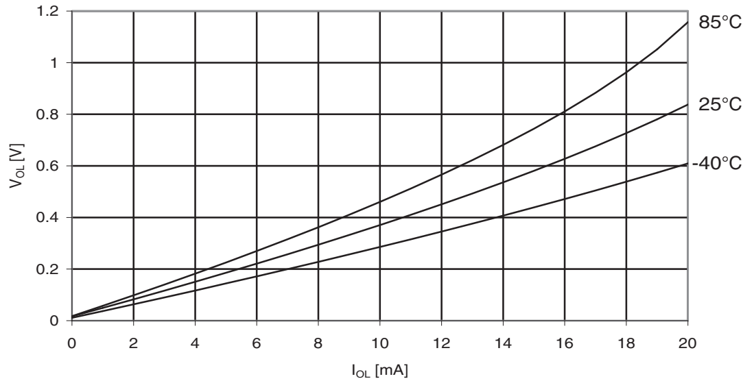
Figure 29-216. ATmega325A: I/O Pin Output Voltage vs. Sink Current, Port B ( V_{CC} = 2.7V )
