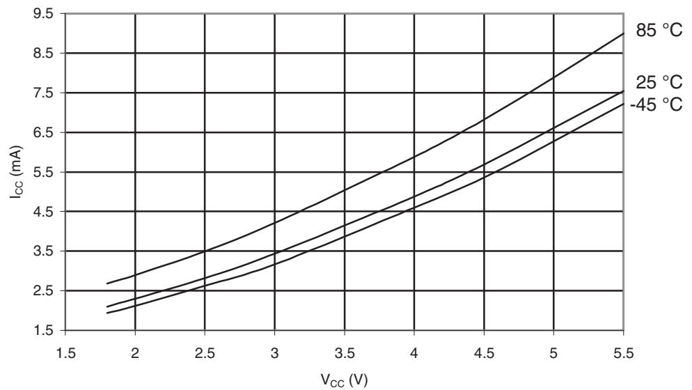
Figure 29-496. ATmega6450A: Idle Supply Current vs. V_{CC} (32kHz Watch Crystal)
