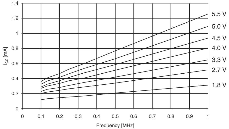
Figure 29-125. ATmega325A: Active Supply Current vs. Frequency (0.1 - 1.0MHz)
