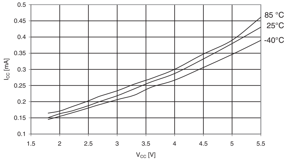
Figure 29-133. ATmega325A: Idle Supply Current vs. V_{CC} (Internal RC Oscillator, 1 MHz)
