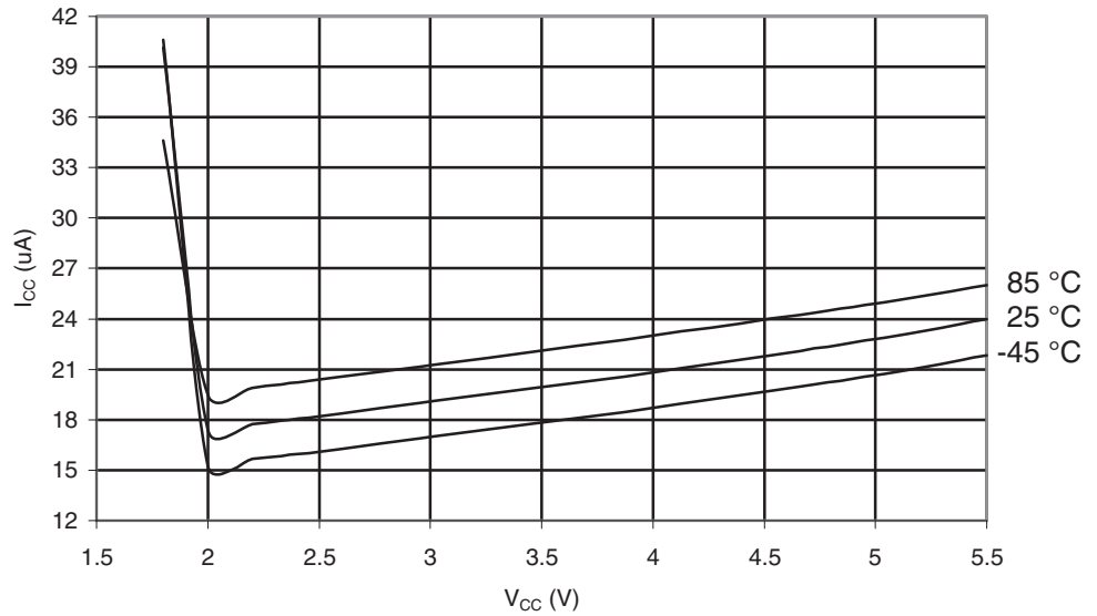
Figure 29-476. ATmega645P: Brownout Detector Current vs. V_{CC}
