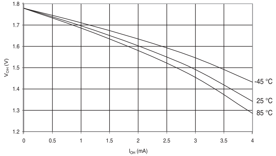
Figure 29-511. ATmega6450A: I/O Pin Output Voltage vs. Source Current, Ports A, C, D, E, F, G ( V_{CC} = 1.8V )
