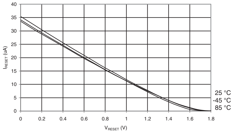
Figure 29-569. ATmega6450A: Reset Pull-up Resistor Current vs. Reset Pin Voltage ( V_{CC} = 1.8V )
