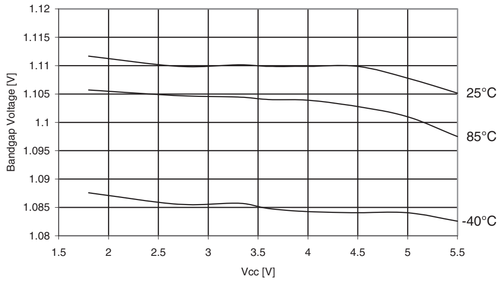
Figure 29-347. ATmega3250PA: Bandgap Voltage vs. V_{CC}
