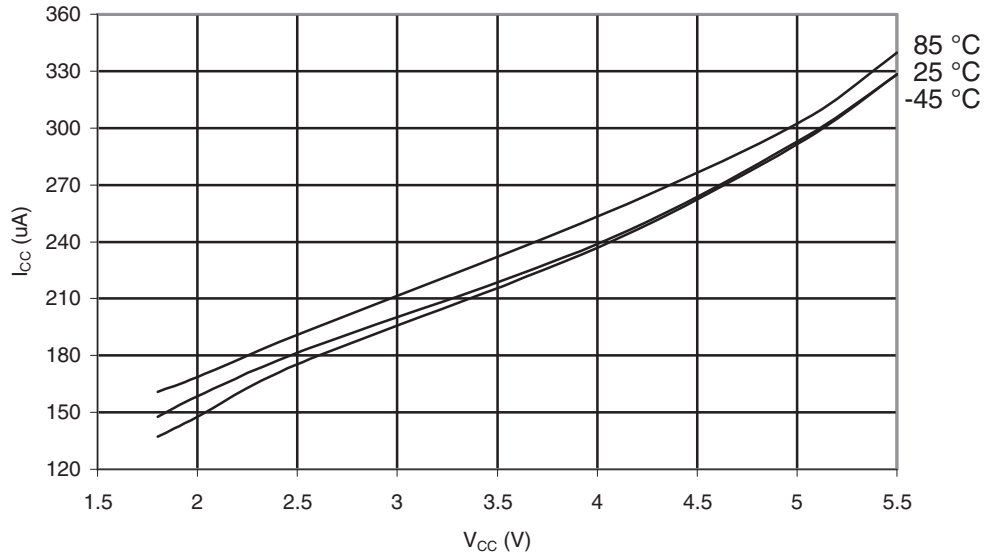
Figure 29-539. ATmega645P: Active Supply Current with ADC at 200kHz vs. V_{CC}
