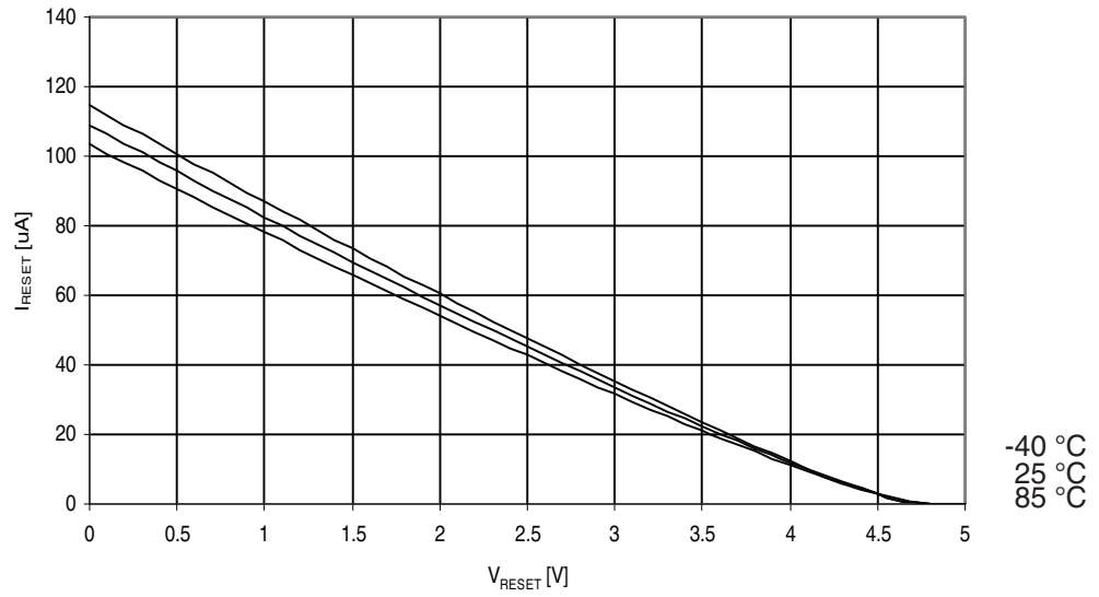
Figure 29-323. ATmega3250PA: Reset Pull-up Resistor Current vs. Reset Pin Voltage ( V_{CC} = 5V )
