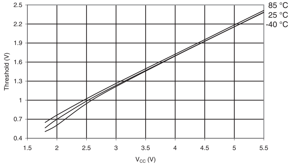
Figure 29-159. ATmega325A: I/O Pin Input Threshold Voltage vs. V_{CC} ( V_{IL} , I/O Pin Read as "0")
