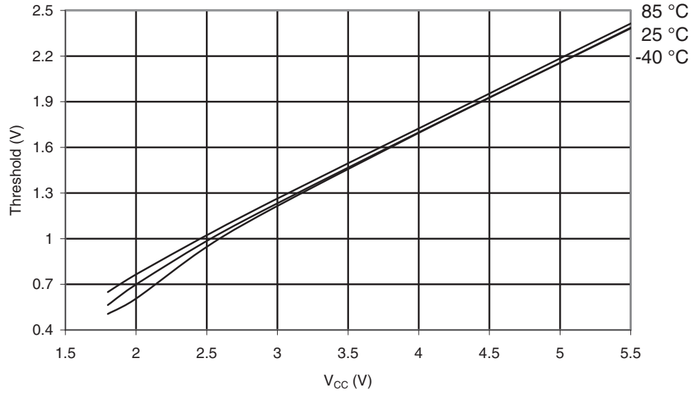
Figure 29-339. ATmega3250PA: I/O Pin Input Threshold Voltage vs. V_{CC} ( V_{IL} , I/O Pin Read as "0")
