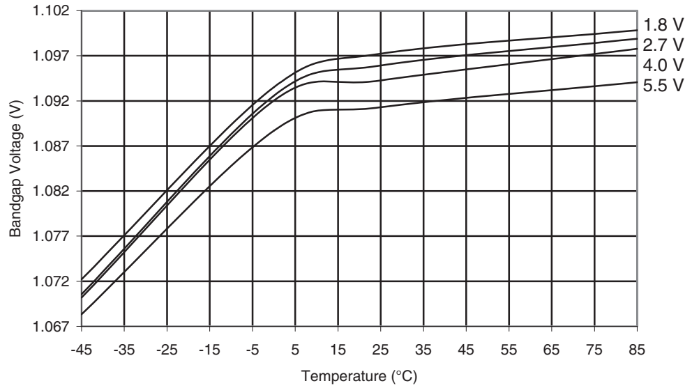
Figure 29-44. ATmega165A: Bandgap Voltage vs. Temperature
