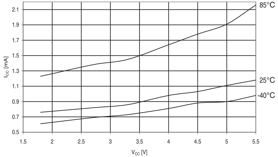
Figure 29-257. ATmega3250A: Power-save Supply Current vs. V_{CC} (Watchdog Timer Disabled and 32kHz Crystal Oscillator Running)
