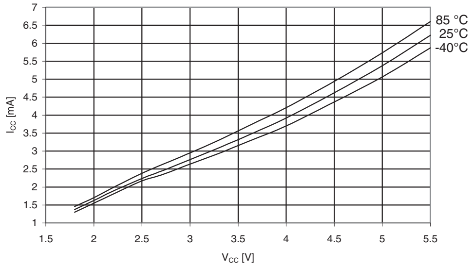
Figure 29-307. ATmega3250PA: Active Supply Current vs. V_{CC} (Internal RC Oscillator, 8MHz)
