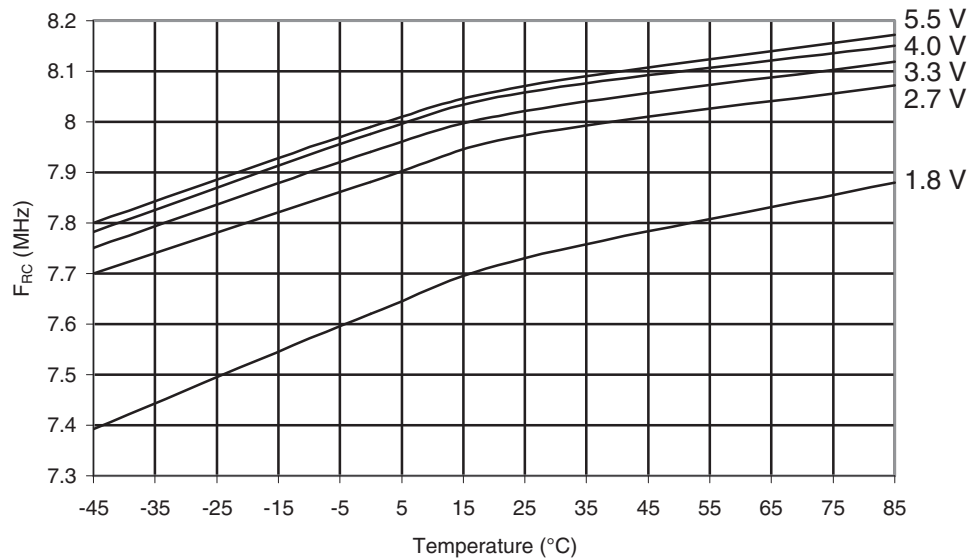
Figure 29-595. ATmega6450P: Calibrated 8MHz RC Oscillator Frequency vs. Temperature
