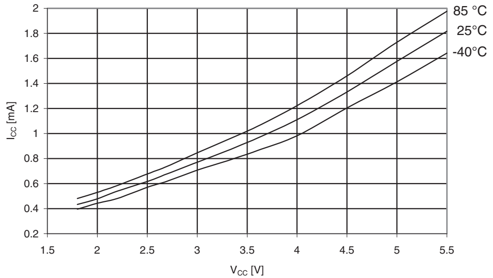
Figure 29-132. ATmega325A: Idle Supply Current vs. V_{CC} (Internal RC Oscillator, 8MHz)
