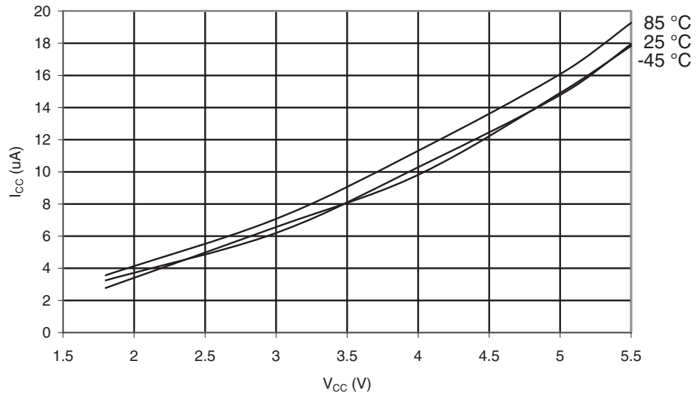
Figure 29-12. ATmega165A: Power-down Supply Current vs. V_{CC} (Watchdog Timer Enabled)
