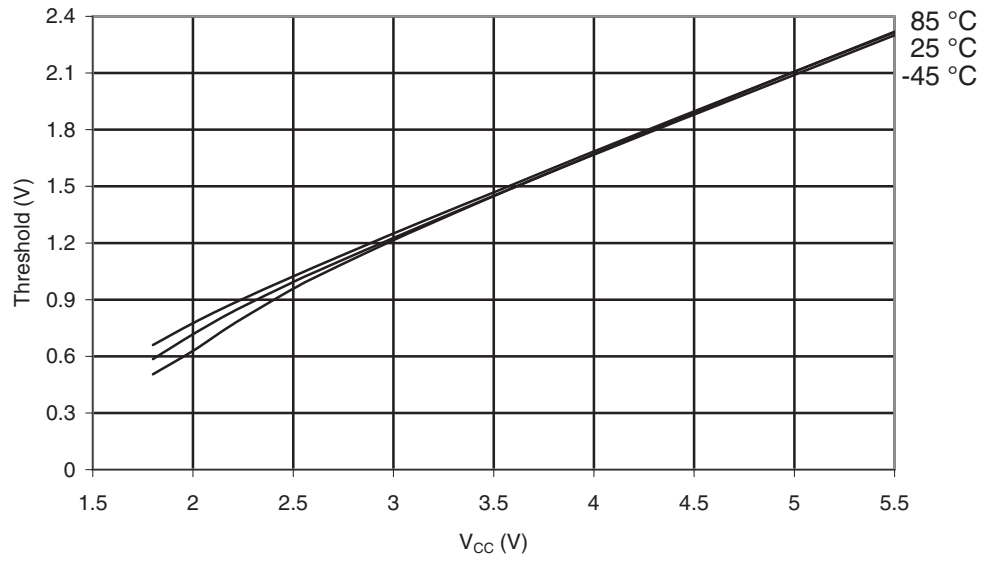
Figure 29-97. ATmega165PA: I/O Pin Input Threshold Voltage vs. V_{CC} ( V_{IL} , I/O Pin Read as "0")
