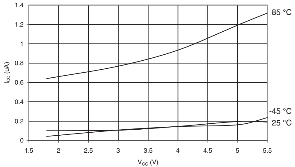
Figure 29-11. ATmega165A: Power-down Supply Current vs. V_{CC} (Watchdog Timer Disabled)
