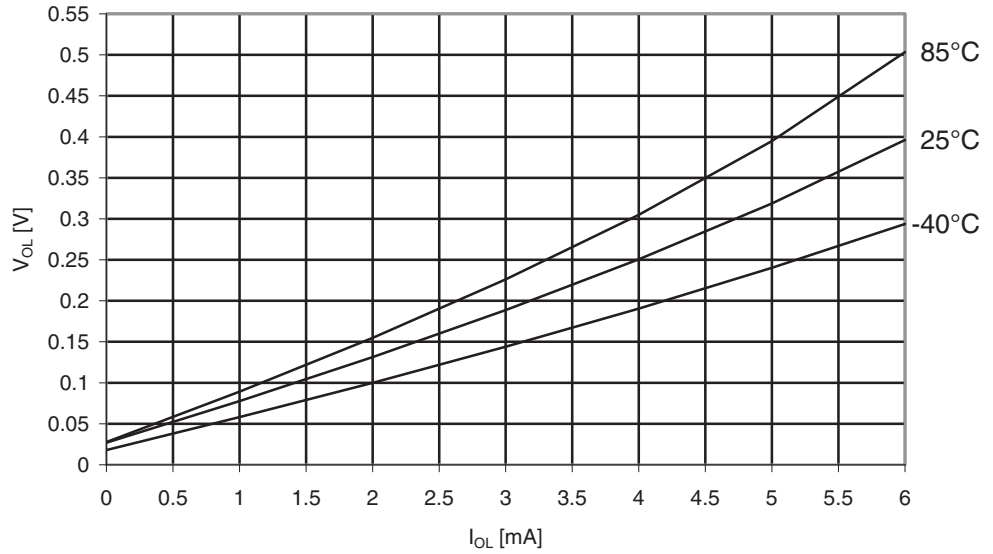
Figure 29-277. ATmega3250A: I/O Pin Output Voltage vs. Sink Current, Port B ( V_{CC} = 1.8V )
