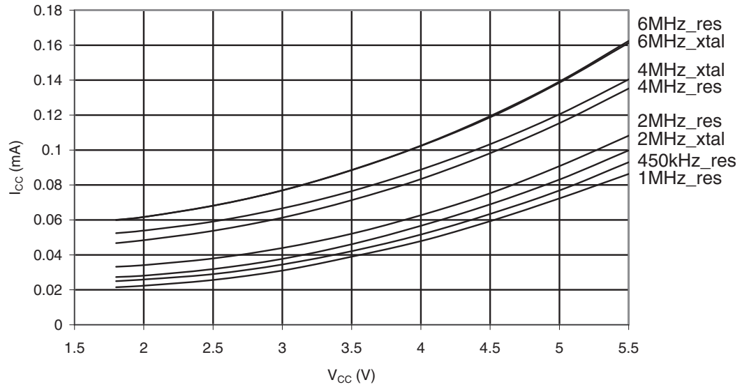
Figure 29-77. ATmega165PA: Standby Supply Current vs. V_{CC} (Xtall and Resonator, Watchdog Timer Disabled)
