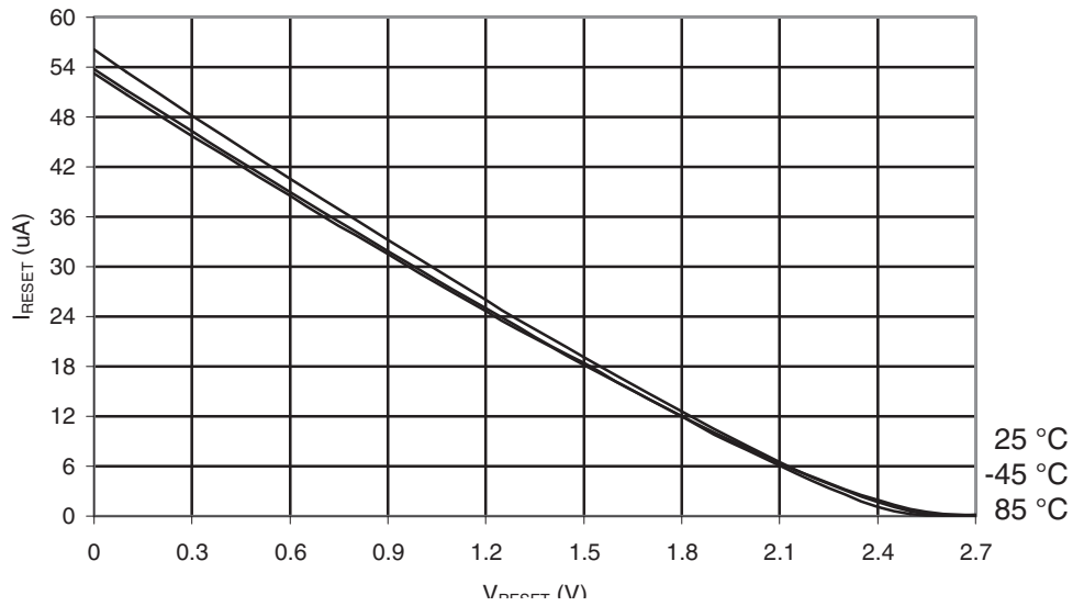
Figure 29-385. ATmega645A: Reset Pull-up Resistor Current vs. Reset Pin Voltage ( V_{CC} = 2.7V )
