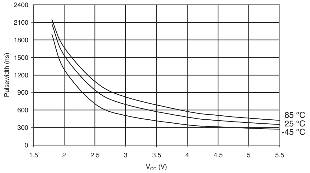
Figure 29-608. ATmega6450P: Minimum Reset Pulse Width vs. V_{CC}
