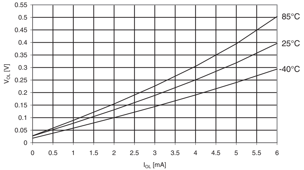
Figure 29-157. ATmega325A: I/O Pin Output Voltage vs. Sink Current, Port B ( V_{CC} = 1.8V )
