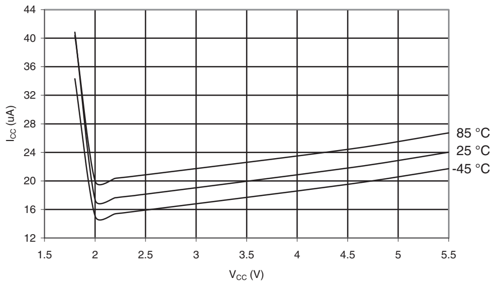
Figure 29-114. ATmega165PA: Brownout Detector Current vs. V_{CC}
