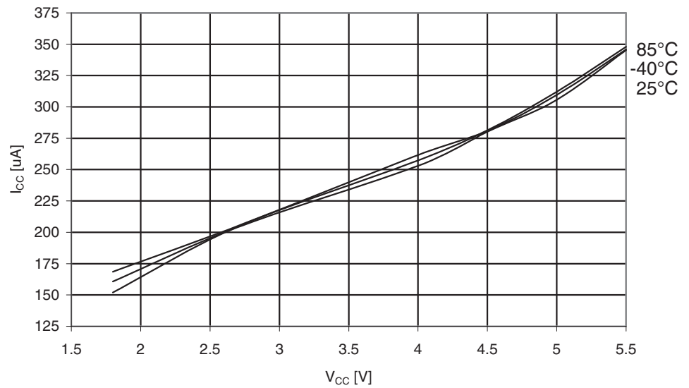
Figure 29-296. ATmega3250A: Active Supply Current with ADC at 200kHz vs. V_{CC}
