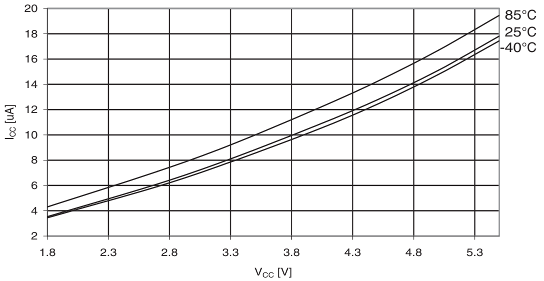
Figure 29-196. ATmega325PA: Power-down Supply Current vs. V_{CC} (Watchdog Timer Enabled)
