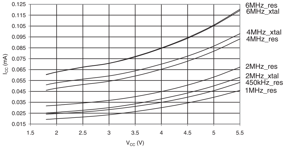
Figure 29-563. ATmega6450A: Standby Supply Current vs. V_{CC} (Xtall and Resonator, Watchdog Timer Disabled)
