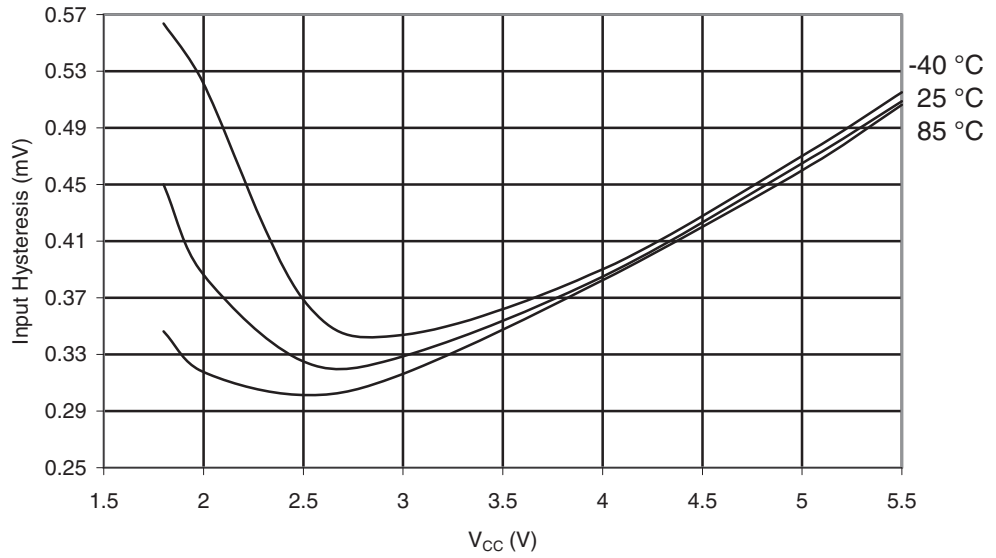
Figure 29-340. ATmega3250PA: I/O Pin Input Hysteresis vs. V_{CC}
