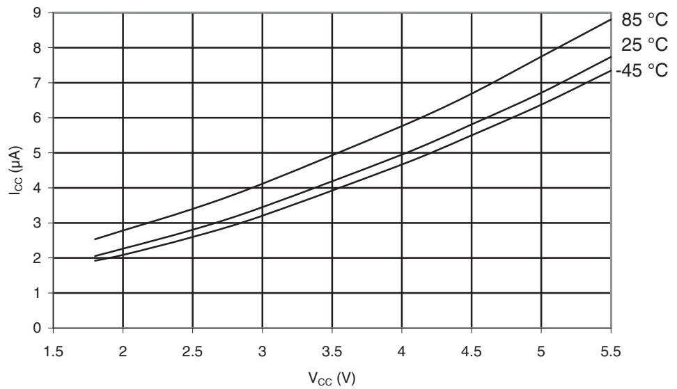
Figure 29-72. ATmega165A: Idle Supply Current vs. V_{CC} (32kHz Watch Crystal)
