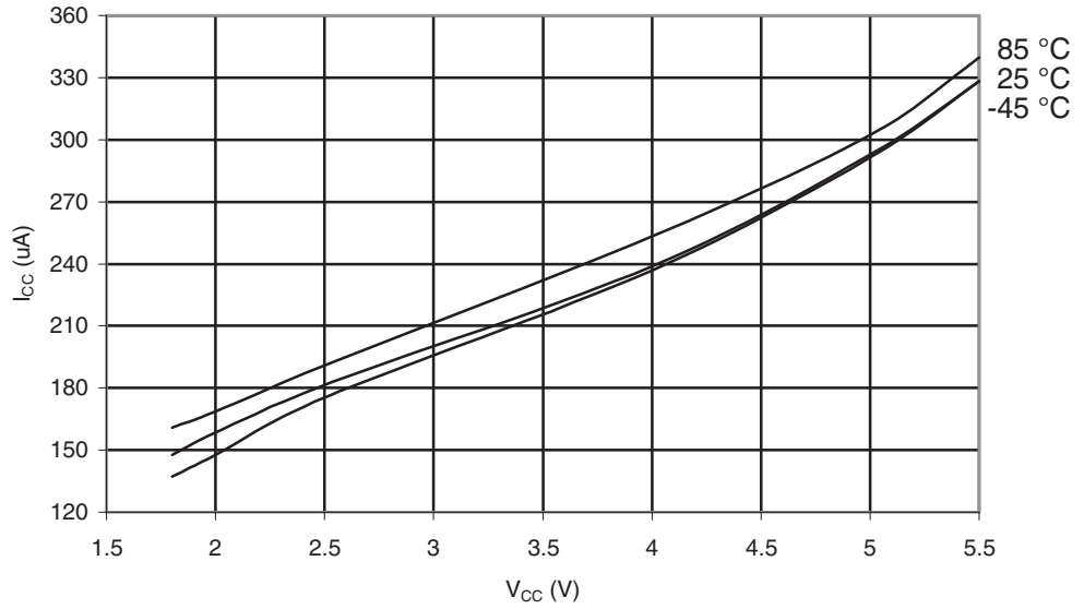
Figure 29-600. ATmega6450P: Active Supply Current with ADC at 200kHz vs. V_{CC}
