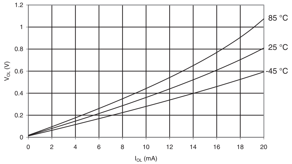
Figure 29-32. ATmega165A: I/O Pin Output Voltage vs. Sink Current, Port B ( V_{CC} = 2.7V )
