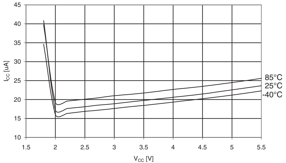
Figure 29-354. ATmega3250PA: Brownout Detector Current vs. V_{CC}
