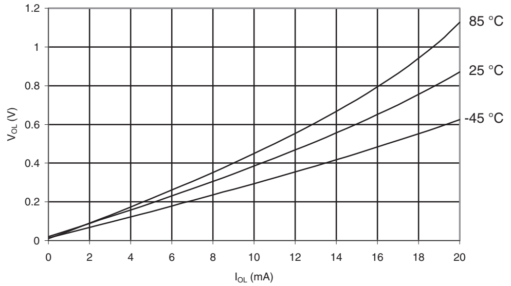
Figure 29-458. ATmega645P: I/O Pin Output Voltage vs. Sink Current, Port B ( V_{CC} = 2.7V_9 )
