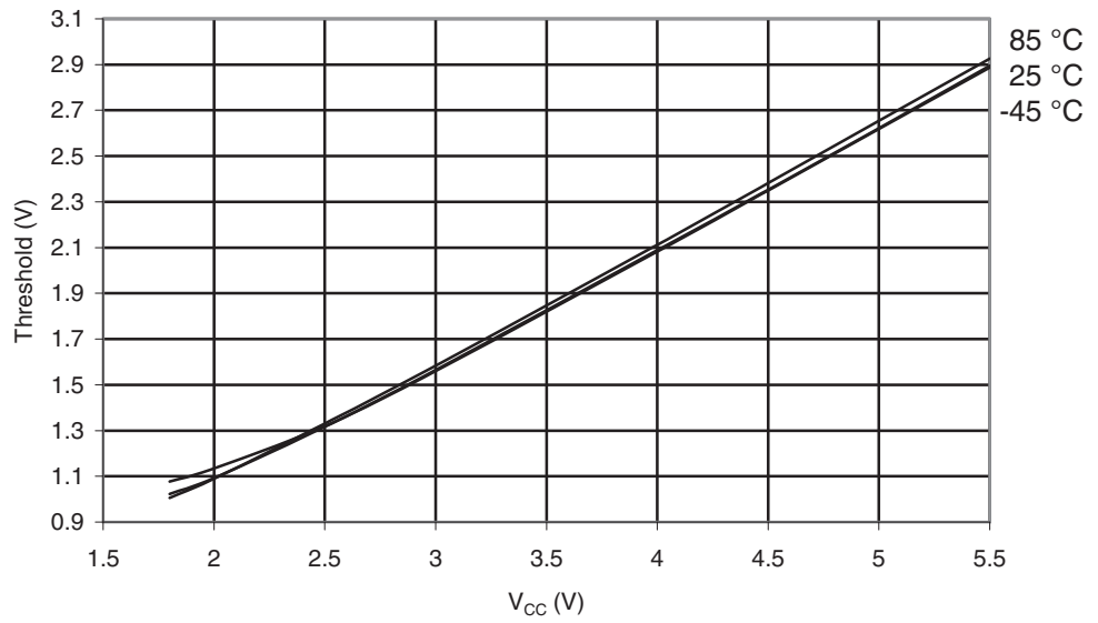
Figure 29-521. ATmega6450A: I/O Pin Input Threshold Voltage vs. V_{CC} ( V_{IH} , I/O Pin Read as "1")
