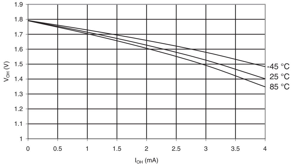
Figure 29-86. ATmega165PA: I/O Pin Output Voltage vs. Source Current, Ports A, C, D, E, F, G ( V_{CC} = 1.8V )
