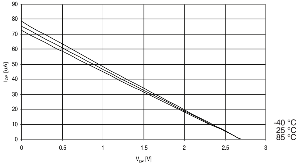
Figure 29-141. ATmega325A: I/O Pin Pull-up Resistor Current vs. Input Voltage ( V_{CC} = 2.7V )
