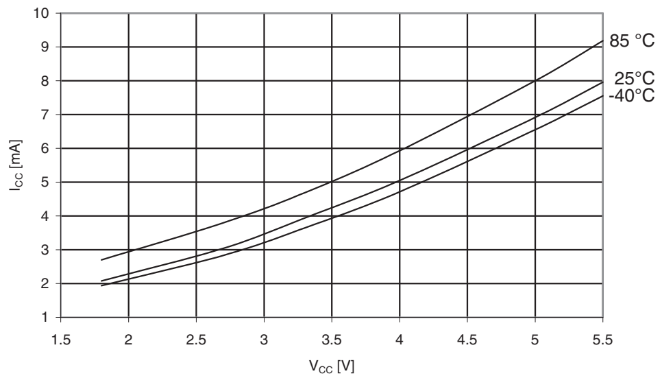
Figure 29-314. ATmega3250PA: Idle Supply Current vs. V_{CC} (32kHz Watch Crystal)
