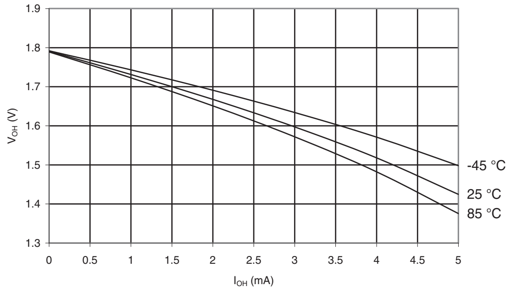
Figure 29-89. ATmega165PA: I/O Pin Output Voltage vs. Source Current, Port B ( V_{CC} = 1.8V )
