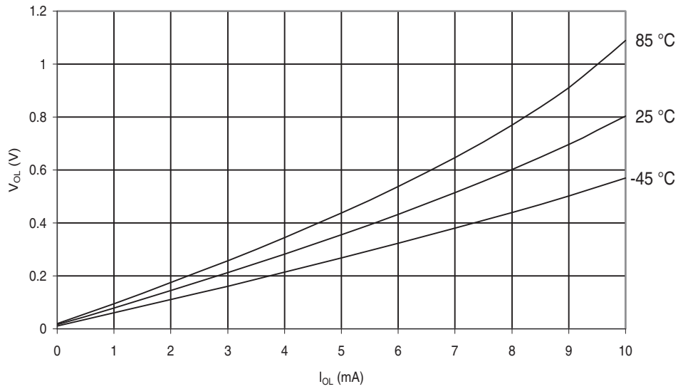
Figure 29-455. ATmega645P: I/O Pin Output Voltage vs. Sink Current, Ports A, C, D, E, F, G ( V_{CC} = 2.7V )
