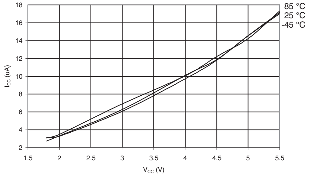
Figure 29-603. ATmega6450P: Watchdog Timer Current vs. V_{CC}
