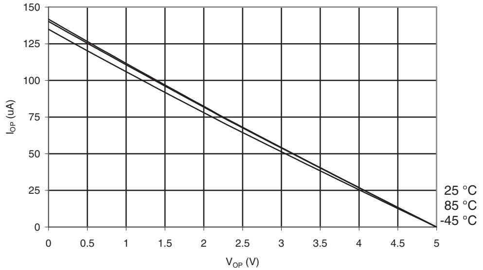
Figure 29-16. ATmega165A: I/O Pin Pull-up Resistor Current vs. Input Voltage ( V_{CC} = 5V )
