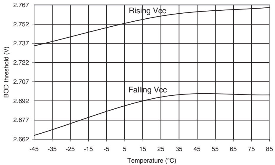
Figure 29-41. ATmega165A: BOD Thresholds vs. Temperature (BOD Level is 2.7V)
