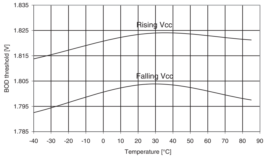
Figure 29-346. ATmega3250PA: BOD Thresholds vs. Temperature (BOD Level is 1.8V)
