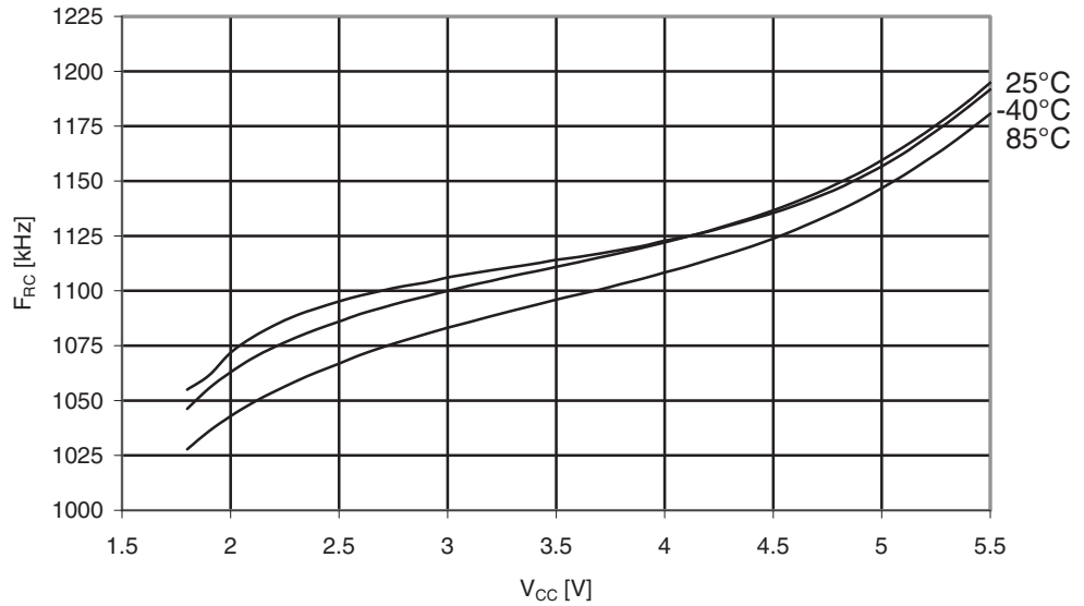
Figure 29-349. ATmega3250PA: Watchdog Oscillator Frequency vs. V_{CC}
