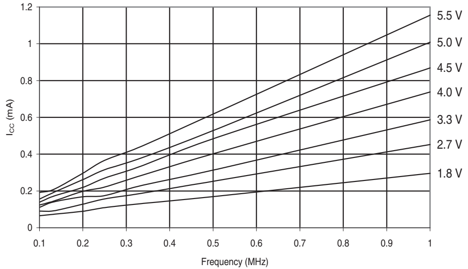
Figure 29-365. ATmega645A: Active Supply Current vs. Low Frequency (0.1 - 1.0MHz)
