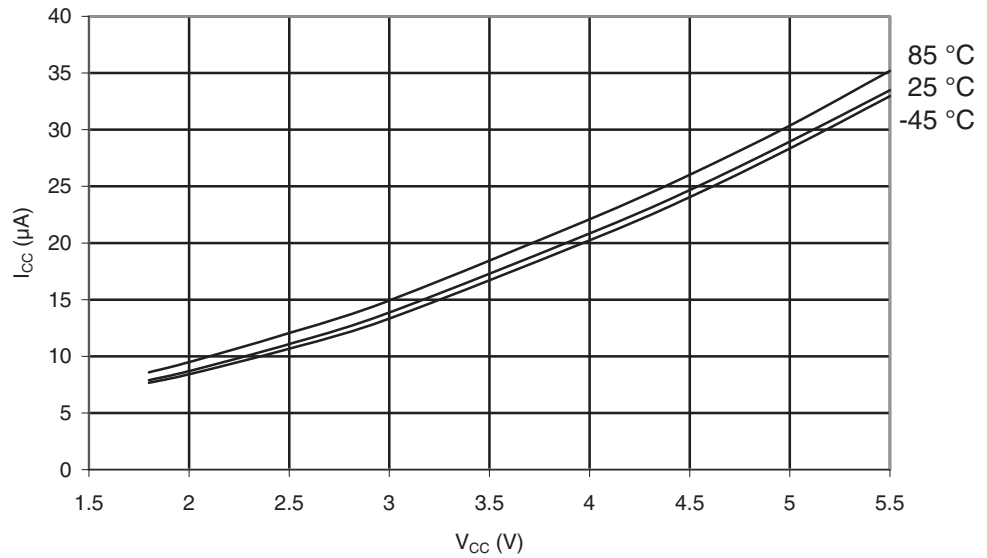
Figure 29-67. ATmega165PA: Active Supply Current vs. V_{CC} (32kHz Watch Crystal)
