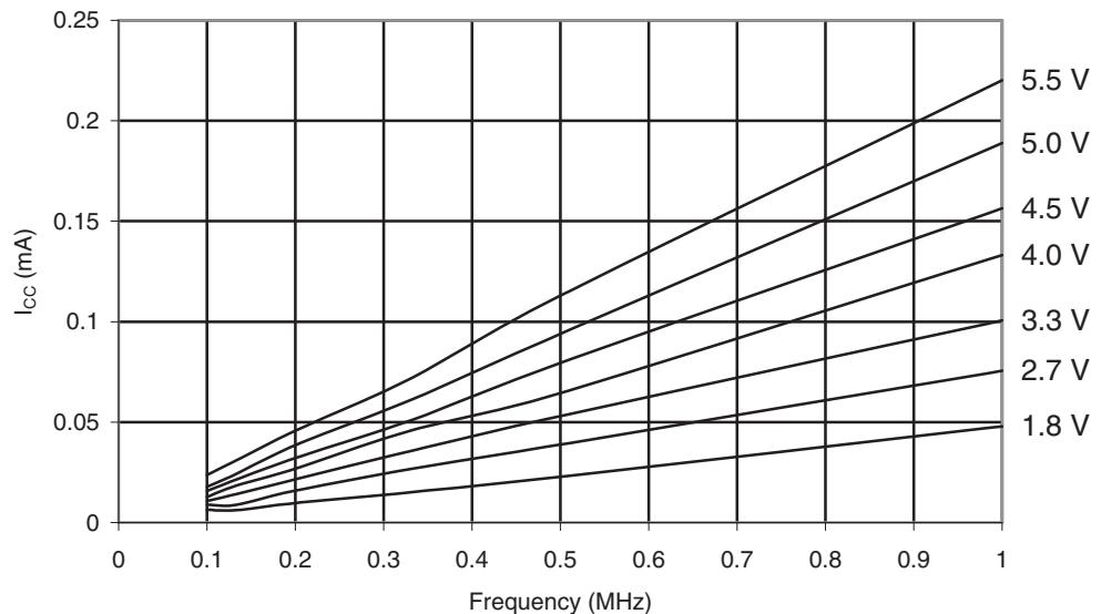
Figure 29-1. ATmega165A: Active Supply Current vs. Frequency (0.1 - 1.0MHz)
