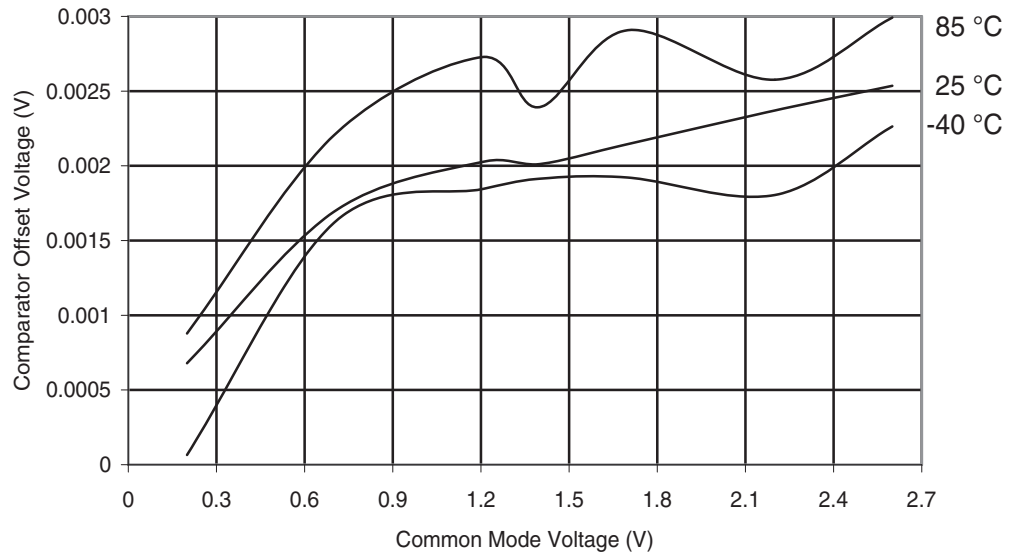
Figure 29-46. ATmega165A: Analog Comparator Offset Voltage vs. Common Mode Voltage ( V_{CC} = 2.7V )
