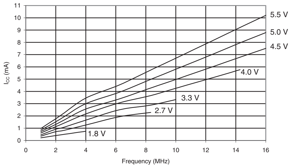
Figure 29-64. ATmega165PA: Active Supply Current vs. Frequency (1 - 16MHz)
