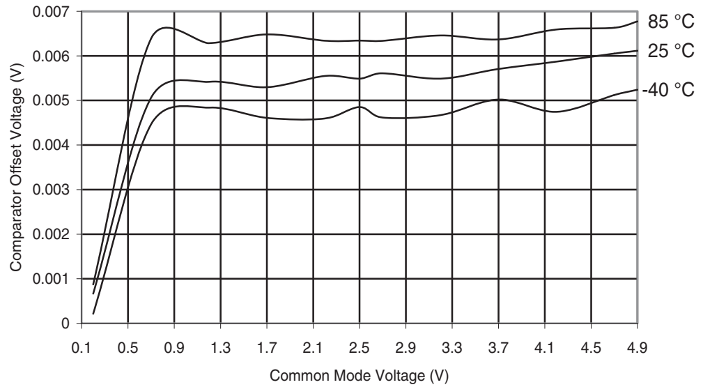
Figure 29-107. ATmega165PA: Analog Comparator Offset Voltage vs. Common Mode Voltage ( V_{CC} = 5V )
