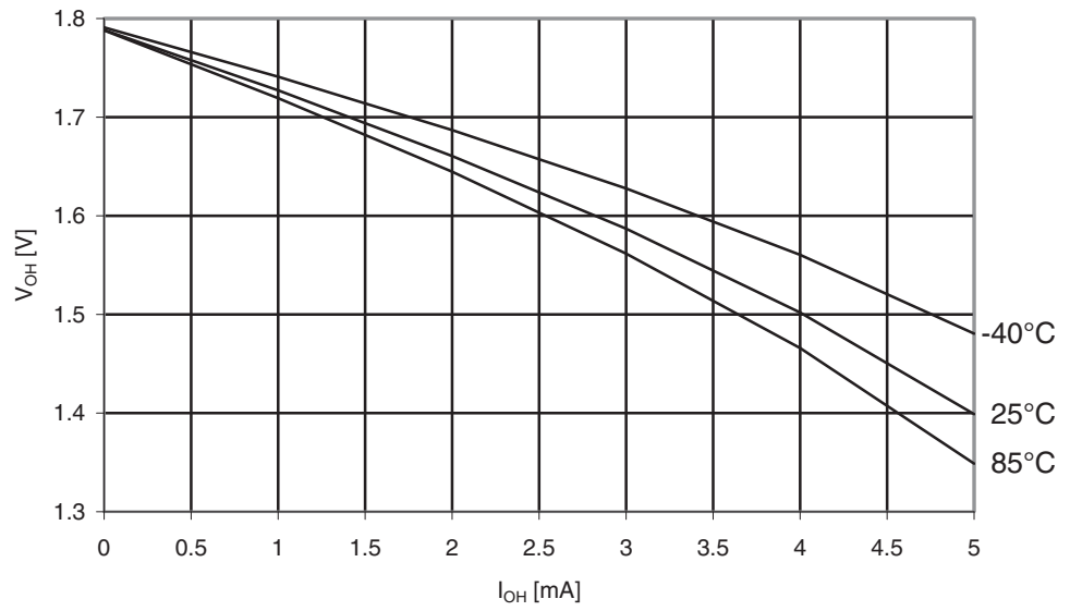
Figure 29-271. ATmega3250A: I/O Pin Output Voltage vs. Source Current, Port B ( V_{CC} = 1.8V )
