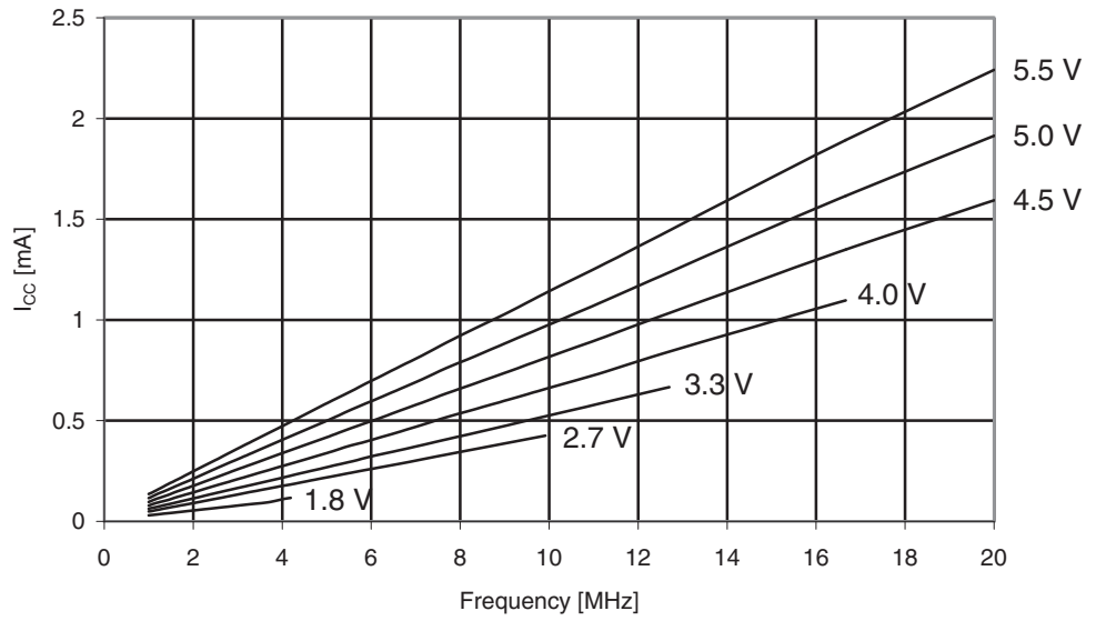
Figure 29-303. ATmega3250A: Reset Supply Current vs. V_{CC} (1 - 20MHz, Excluding Current Through The Reset Pull-up)
