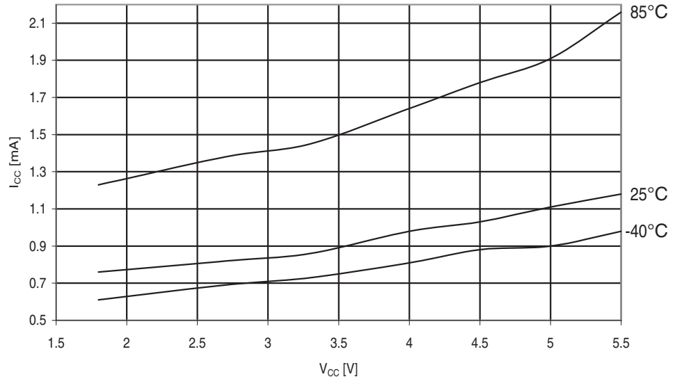
Figure 29-137. ATmega325A: Power-save Supply Current vs. V_{CC} (Watchdog Timer Disabled and 32kHz Crystal Oscillator Running)
