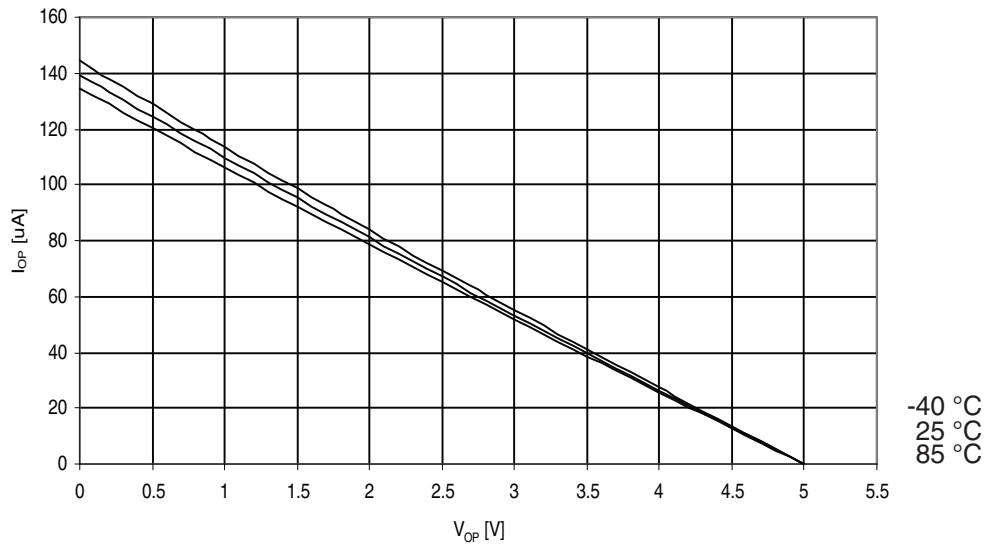
Figure 29-200. ATmega325PA: I/O Pin Pull-up Resistor Current vs. Input Voltage ( V_{CC} = 5V )
