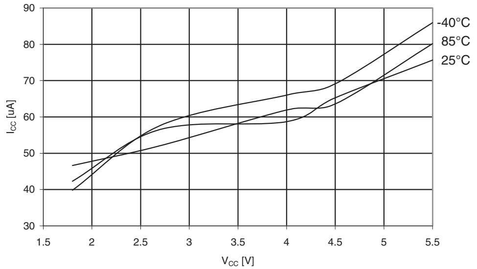
Figure 29-300. ATmega3250A: Analog Comparator Current vs. V_{CC}
