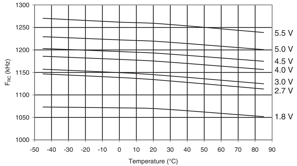
Figure 29-110. ATmega165PA: Watchdog Oscillator Frequency vs. Temperature
