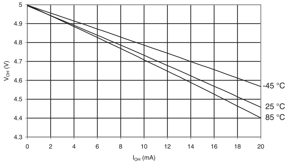
Figure 29-451. ATmega645A: I/O Pin Output Voltage vs. Source Current, Port B ( V_{CC} = 5V )
