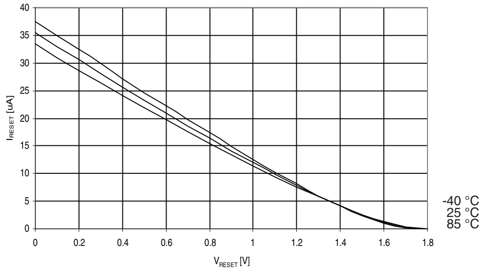
Figure 29-265. ATmega3250A: Reset Pull-up Resistor Current vs. Reset Pin Voltage ( V_{CC} = 1.8V )
