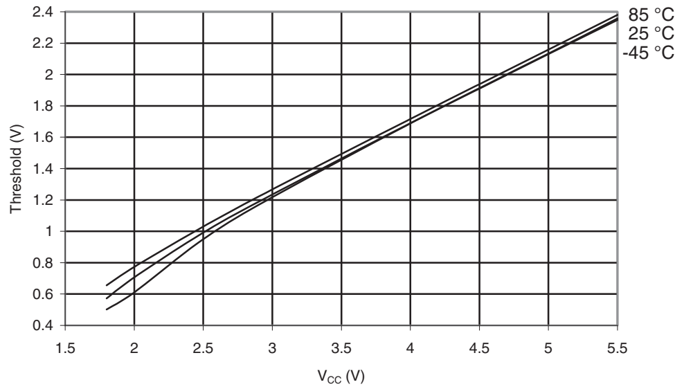
Figure 29-400. ATmega645A: I/O Pin Input Threshold Voltage vs. V_{CC} ( V_{IL} , I/O Pin Read as "0")
