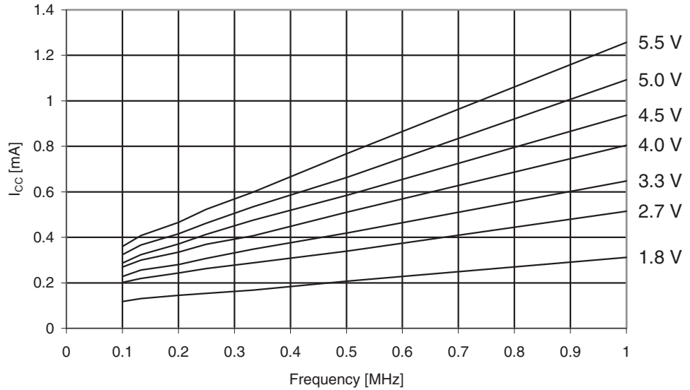
Figure 29-305. ATmega3250PA: Active Supply Current vs. Frequency (0.1 - 1.0MHz)
