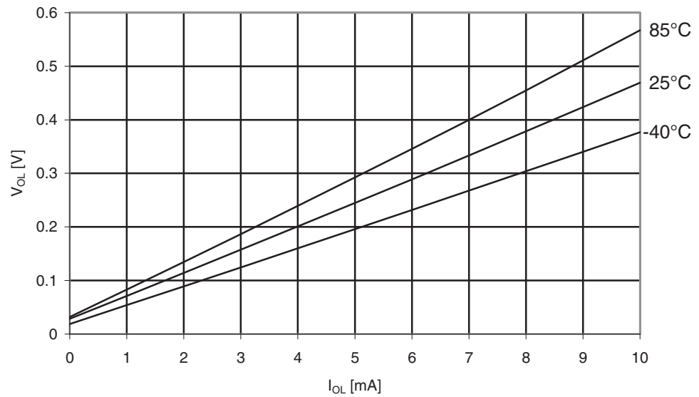
Figure 29-332. ATmega3250PA: I/O Pin Output Voltage vs. Sink Current, Ports A, C, D, E, F, G ( V_{CC} = 5V )
