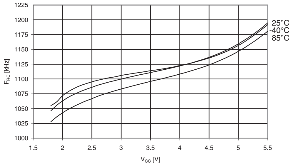
Figure 29-229. ATmega325PA: Watchdog Oscillator Frequency vs. V_{CC}
