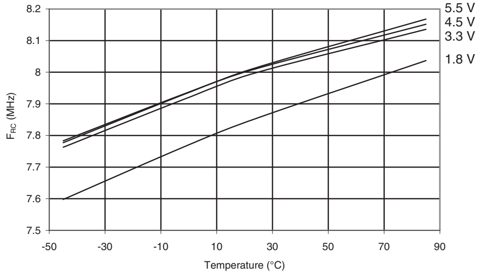
Figure 29-111. ATmega165PA: Calibrated 8MHz RC Oscillator Frequency vs. Temperature
