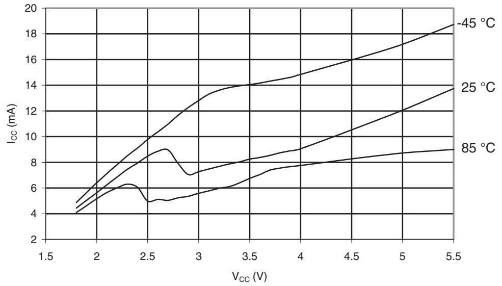
Figure 29-422. ATmega645A: Programming Current vs. V_{CC}
