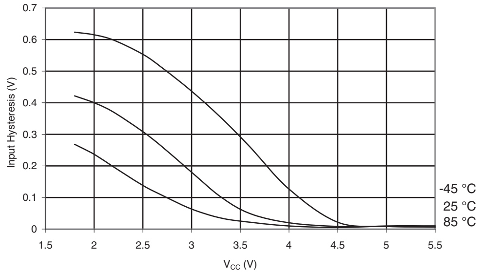
Figure 29-101. ATmega165PA: Reset Input Pin Hysteresis vs. V_{CC}
