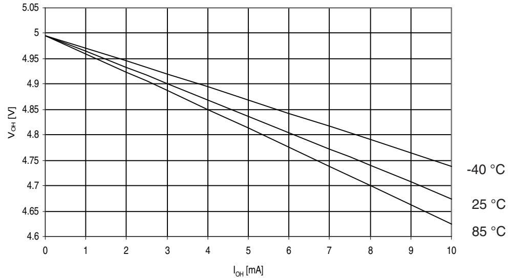
Figure 29-146. ATmega325A: I/O Pin Output Voltage vs. Source Current, Ports A, C, D, E, F, G ( V_{CC} = 5V )
