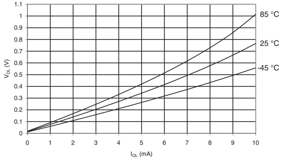
Figure 29-91. ATmega165PA: I/O Pin Output Voltage vs. Sink Current, Ports A, C, D, E, F, G ( V_{CC} = 2.7V )
