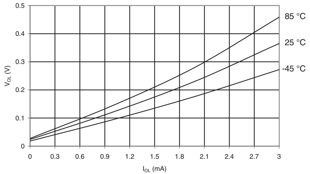
Figure 29-92. ATmega165PA: I/O Pin Output Voltage vs. Sink Current, Ports A, C, D, E, F, G ( V_{CC} = 1.8V )
