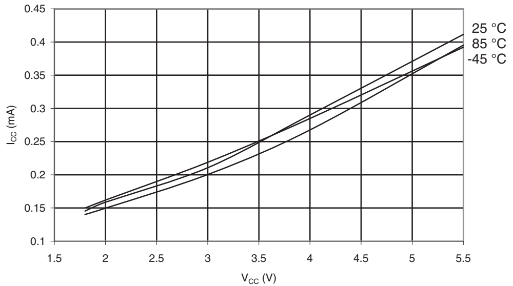
Figure 29-553. ATmega6450A: Idle Supply Current vs. Low Frequency (0.1 - 1.0MHz)
