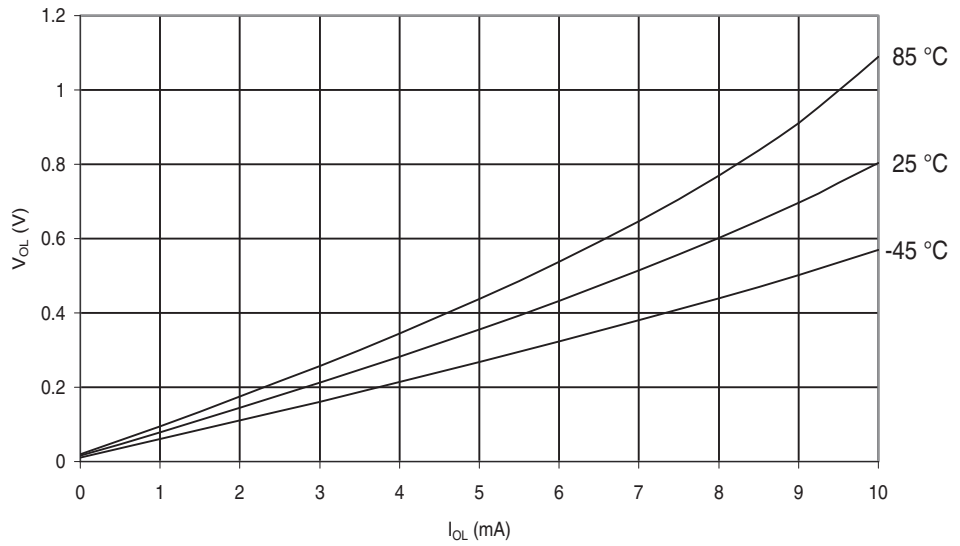
Figure 29-394. ATmega645A: I/O Pin Output Voltage vs. Sink Current, Ports A, C, D, E, F, G ( V_{CC} = 2.7V )
