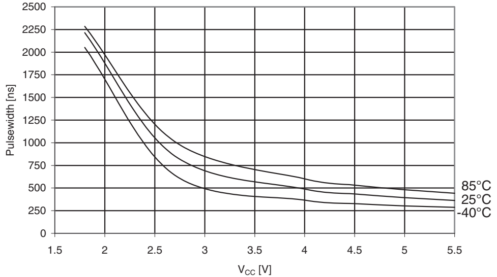
Figure 29-184. ATmega325A: Minimum Reset Pulse Width vs. V_{CC}
