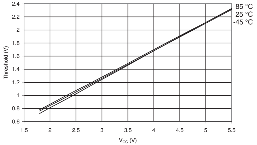
Figure 29-100. ATmega165PA: Reset Input Threshold Voltage vs. V_{CC} ( V_{IL} , Reset Pin Read as “0”)
