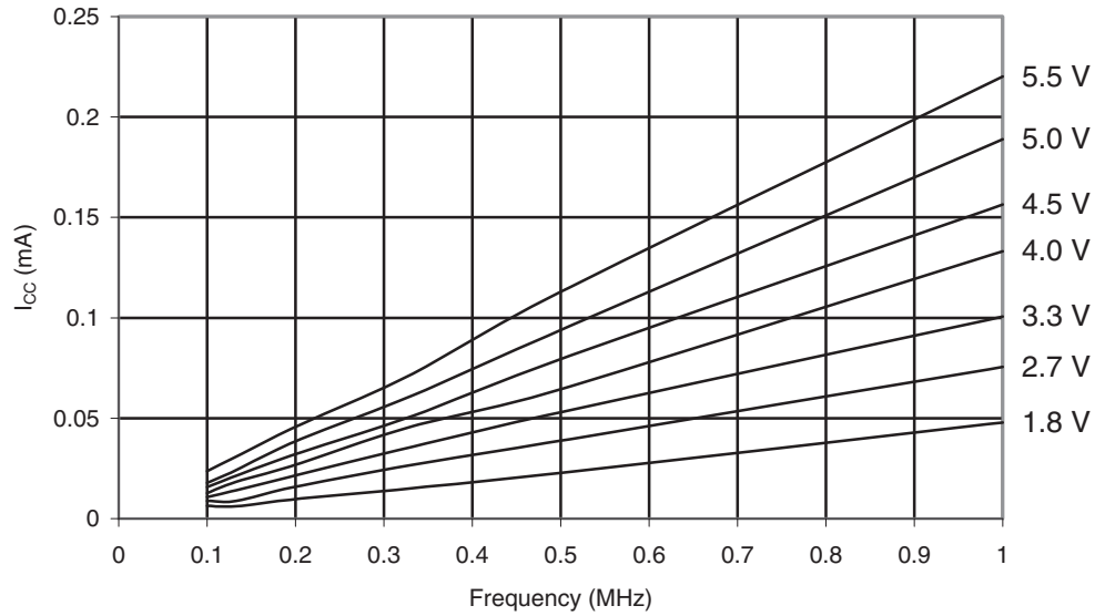
Figure 29-63. ATmega165PA: Active Supply Current vs. Frequency (0.1 - 1.0MHz)
