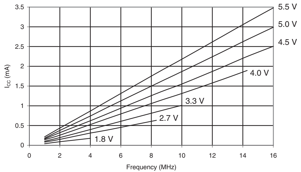
Figure 29-7. ATmega165A: Idle Supply Current vs. Frequency (1 - 16MHz)
