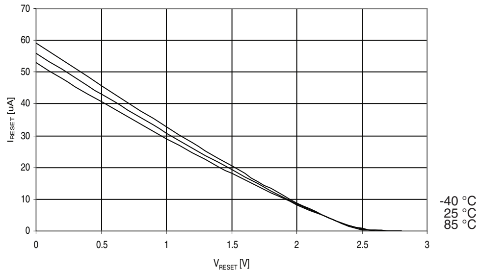
Figure 29-144. ATmega325A: Reset Pull-up Resistor Current vs. Reset Pin Voltage ( V_{CC} = 2.7V )
