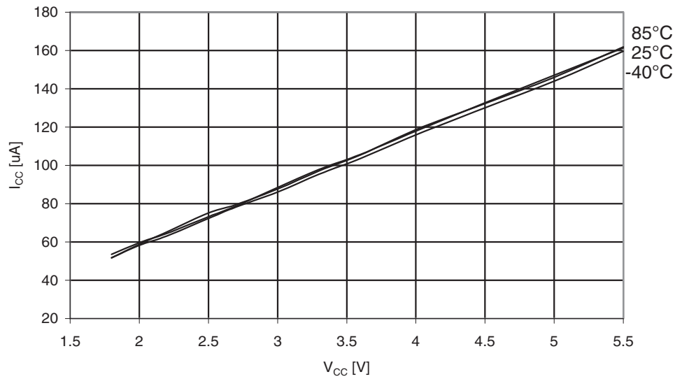
Figure 29-178. ATmega325A: AREF External Reference Current vs. V_{CC}
