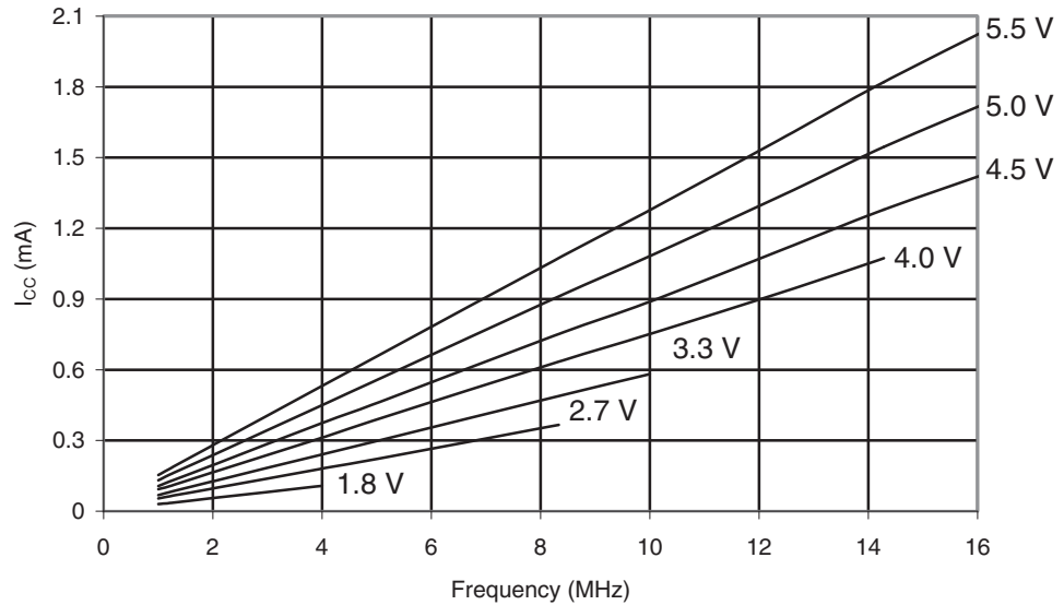
Figure 29-61. ATmega165A: Reset Supply Current vs. V_{CC} (1 - 16MHz, Excluding Current Through The Reset Pull-up)
