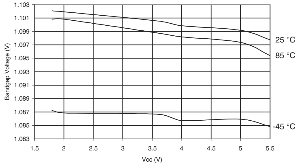
Figure 29-408. ATmega645A: Bandgap Voltage vs. V_{CC}
