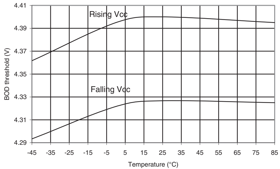
Figure 29-527. ATmega6450A: BOD Thresholds vs. Temperature (BOD Level is 4.3V)
