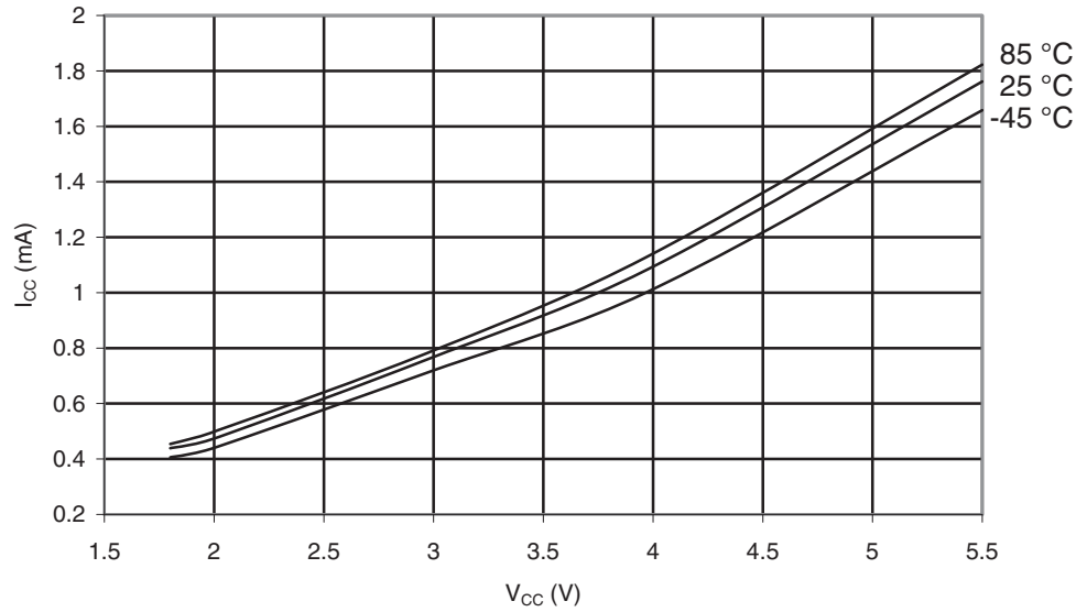
Figure 29-494. ATmega6450A: Idle Supply Current vs. V_{CC} (Internal RC Oscillator, 8MHz)
