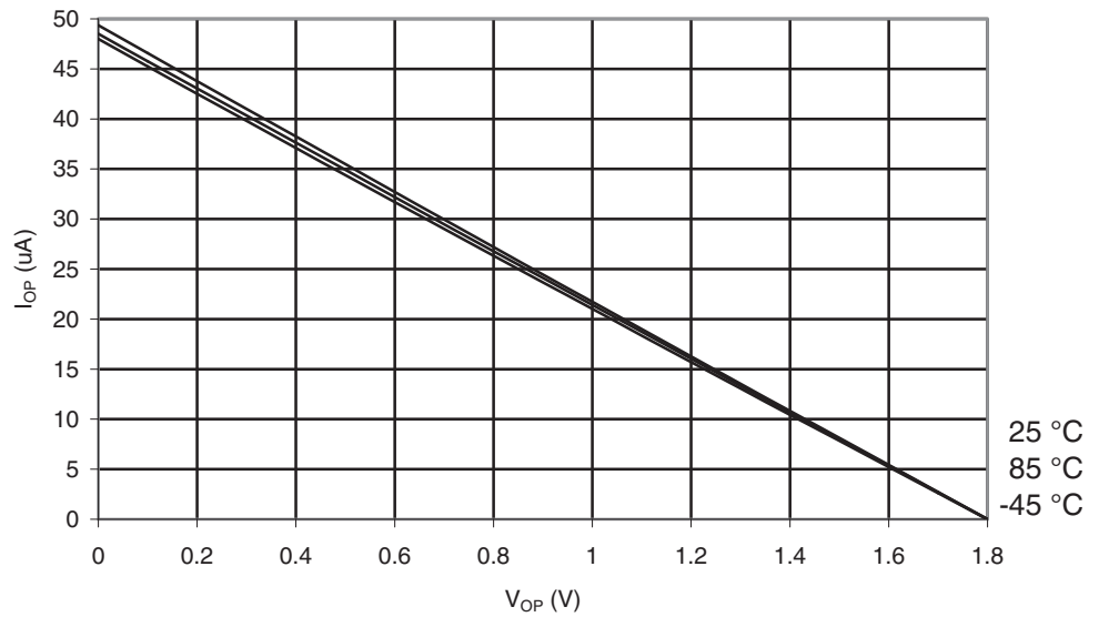
Figure 29-18. ATmega165A: I/O Pin Pull-up Resistor Current vs. Input Voltage ( V_{CC} = 1.8V )
