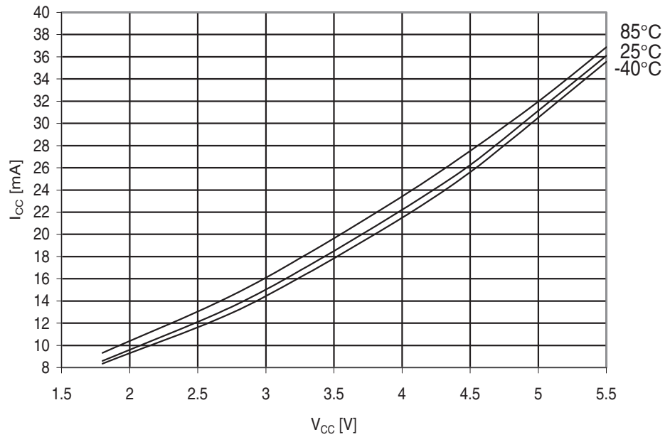
Figure 29-129. ATmega325A: Active Supply Current vs. V_{CC} (32kHz Watch Crystal)
