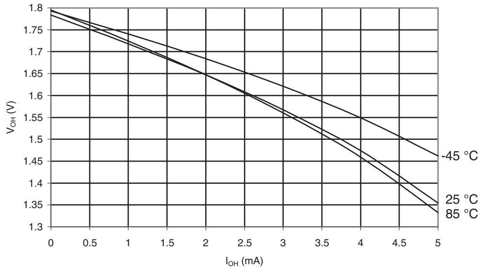
Figure 29-392. ATmega645A: I/O Pin Output Voltage vs. Source Current, Port B ( V_{CC} = 1.8V )
