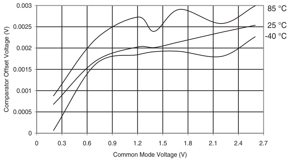
Figure 29-108. ATmega165PA: Analog Comparator Offset Voltage vs. Common Mode Voltage ( V_{CC} = 2.7V )
