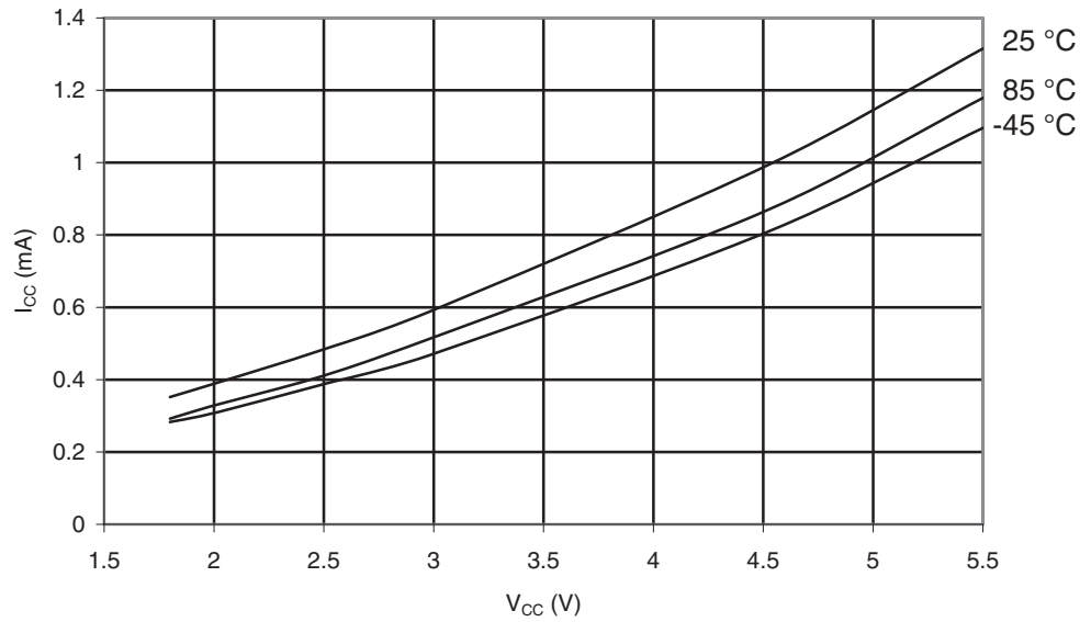
Figure 29-71. ATmega165PA: Idle Supply Current vs. V_{CC} (Internal RC Oscillator, 1 MHz)
