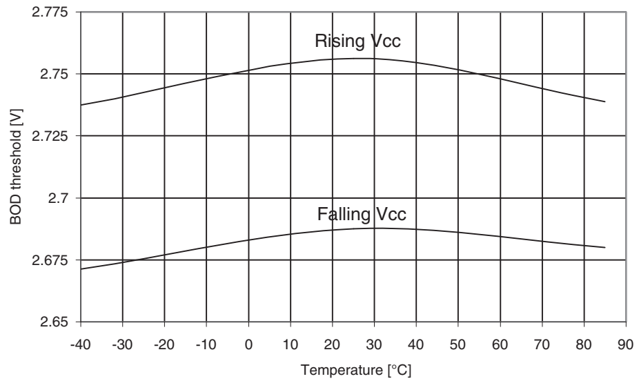
Figure 29-225. ATmega325PA: BOD Thresholds vs. Temperature (BOD Level is 2.7V)
