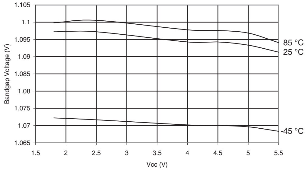
Figure 29-105. ATmega165PA: Bandgap Voltage vs. V_{CC}
