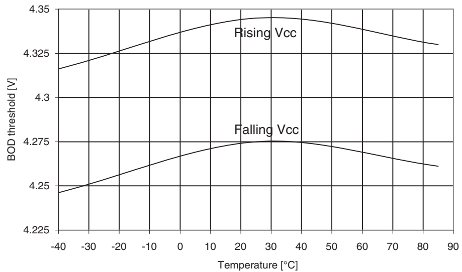
Figure 29-284. ATmega3250A: BOD Thresholds vs. Temperature (BOD Level is 4.3V)
