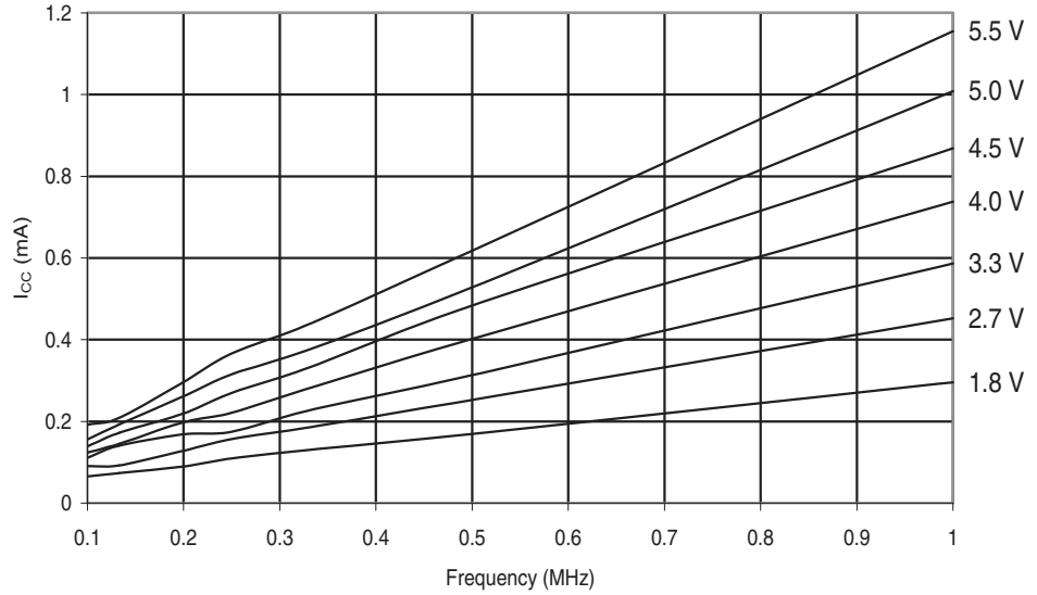
Figure 29-548. ATmega6450A: Active Supply Current vs. Low Frequency (0.1 - 1.0MHz)
