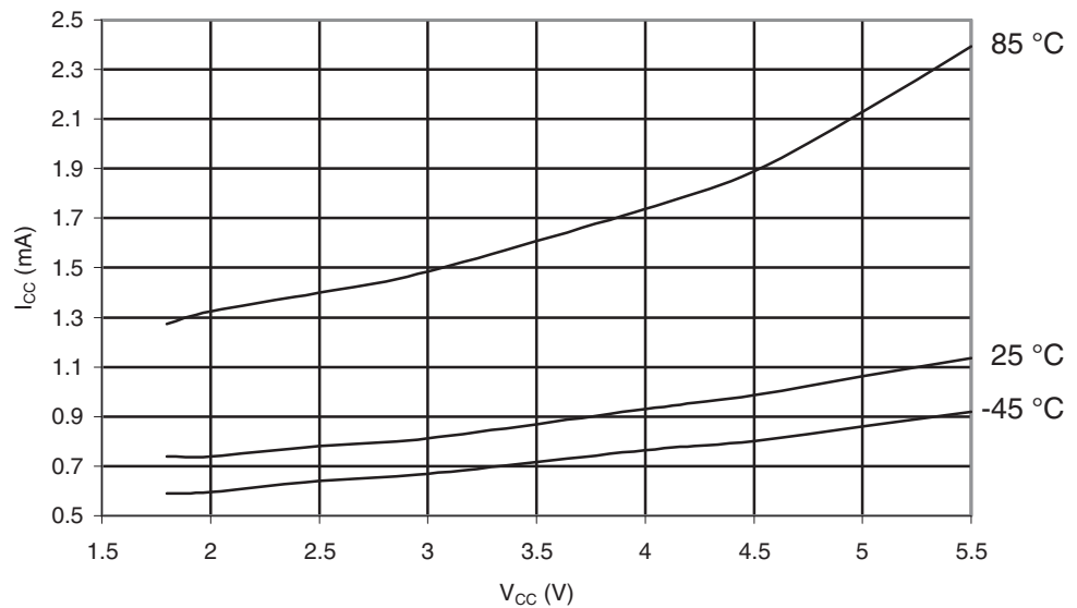
Figure 29-500. ATmega6450A: Power-save Supply Current vs. V_{CC} (Watchdog Timer Disabled and 32kHz Crystal Oscillator Running)
