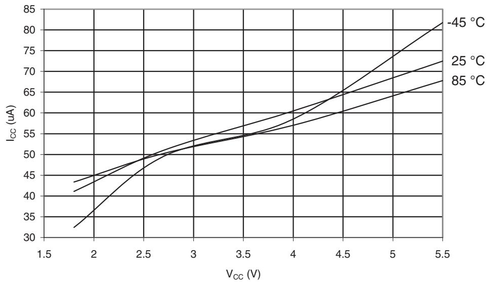
Figure 29-120. ATmega165PA: Analog Comparator Current vs. V_{CC}
