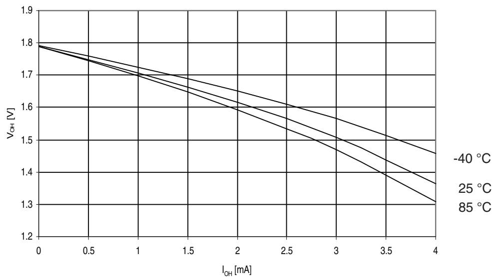
Figure 29-208. ATmega325PA: I/O Pin Output Voltage vs. Source Current, Ports A, C, D, E, F, G ( V_{CC} = 1.8V )
