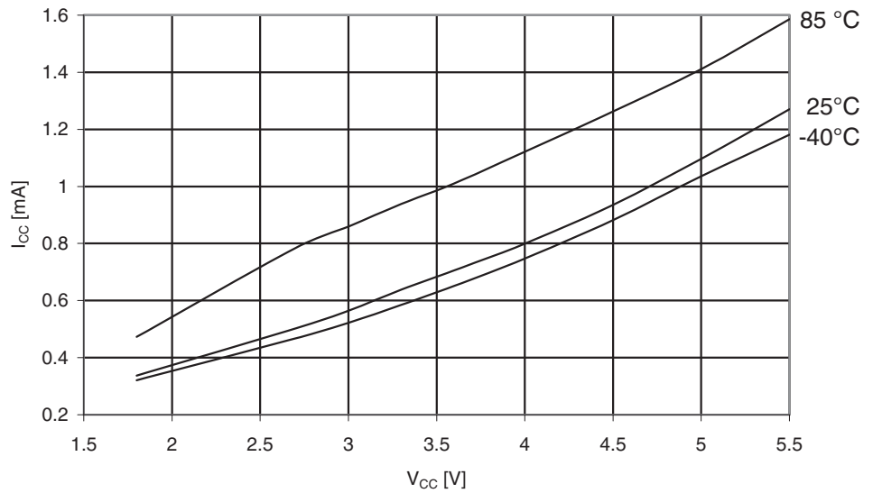
Figure 29-128. ATmega325A: Active Supply Current vs. V_{CC} (Internal RC Oscillator, 1MHz)
