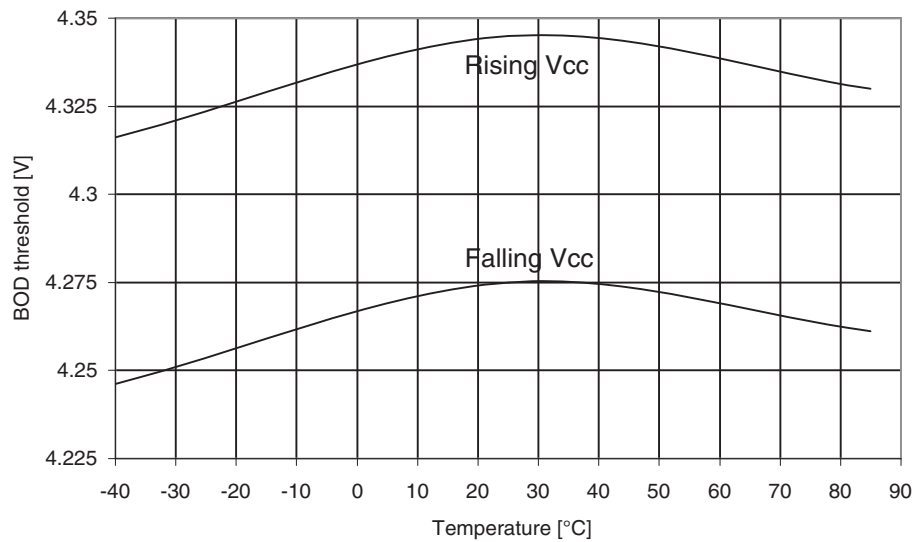
Figure 29-164. ATmega325A: BOD Thresholds vs. Temperature (BOD Level is 4.3V)
