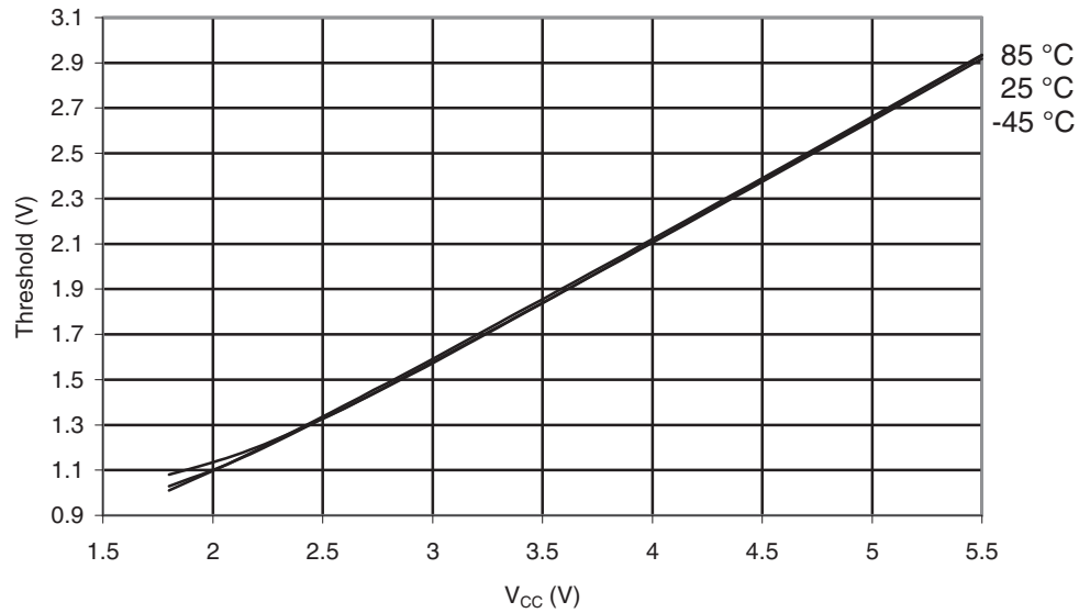
Figure 29-34. ATmega165A: I/O Pin Input Threshold Voltage vs. V_{CC} ( V_{IH} , I/O Pin Read as “1”)
