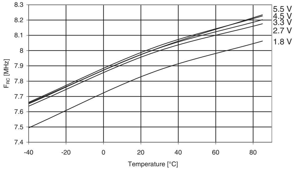
Figure 29-171. ATmega325A: Calibrated 8MHz RC Oscillator Frequency vs. Temperature
