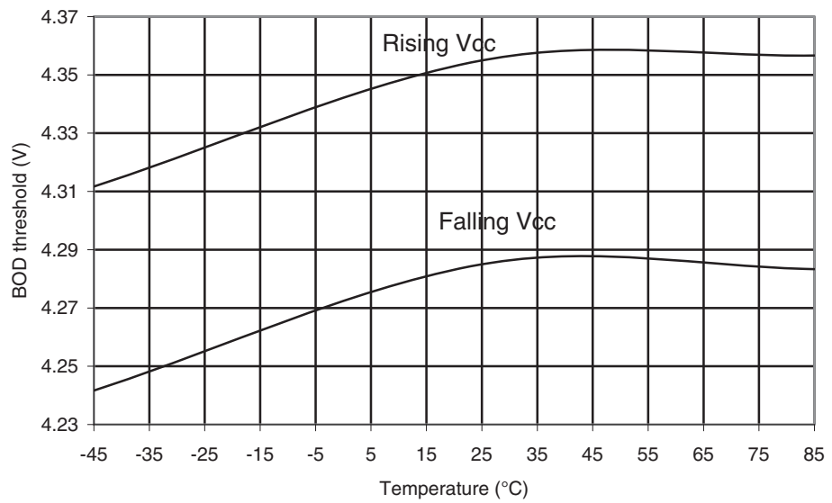
Figure 29-102. ATmega165PA: BOD Thresholds vs. Temperature (BOD Level is 4.3V)
