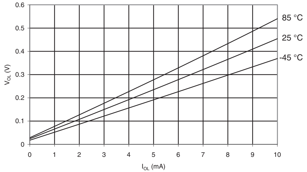
Figure 29-28. ATmega165A: I/O Pin Output Voltage vs. Sink Current, Ports A, C, D, E, F, G ( V_{CC} = 5V )
