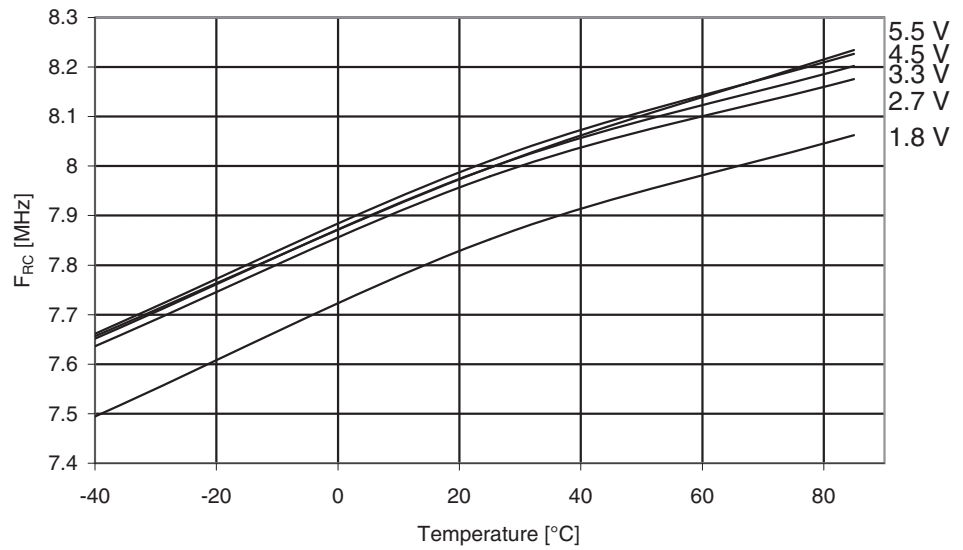
Figure 29-291. ATmega3250A: Calibrated 8MHz RC Oscillator Frequency vs. Temperature
