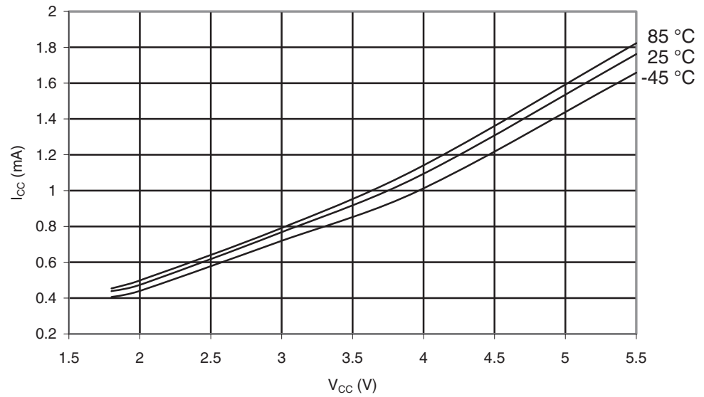
Figure 29-372. ATmega645A: Idle Supply Current vs. V_{CC} (Internal RC Oscillator, 8MHz)
