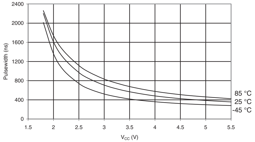
Figure 29-62. ATmega165A: Minimum Reset Pulse Width vs. V_{CC}
