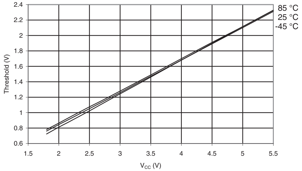
Figure 29-38. ATmega165A: Reset Input Threshold Voltage vs. V_{CC} ( V_{IL,Reset} Pin Read as "0")
