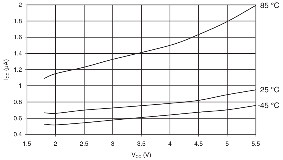
Figure 29-15. ATmega165A: Standby Supply Current vs. V_{CC} (Xtall and Resonator, Watchdog Timer Disabled)
