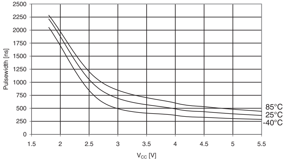
Figure 29-304. ATmega3250A: Minimum Reset Pulse Width vs. V_{CC}
