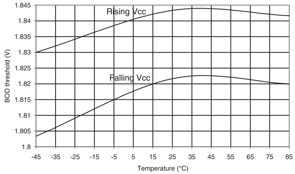
Figure 29-407. ATmega645A: BOD Thresholds vs. Temperature (BOD Level is 1.8V)
