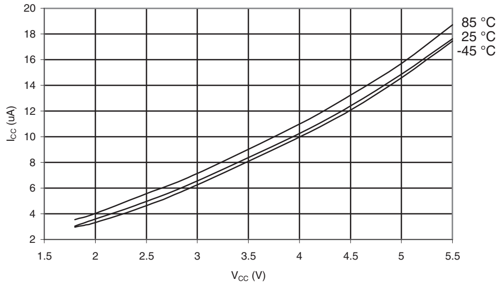
Figure 29-437. ATmega645P: Power-down Supply Current vs. V_{CC} (Watchdog Timer Enabled)
