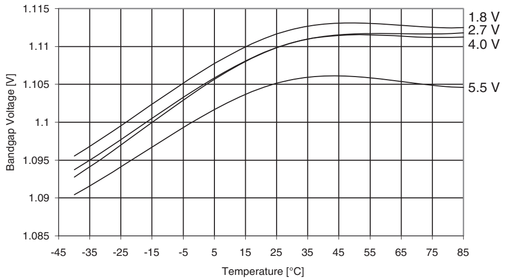
Figure 29-228. ATmega325PA: Bandgap Voltage vs. Temperature
