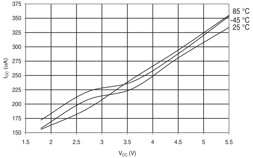
Figure 29-54. ATmega165A: Active Supply Current with ADC at 200kHz vs. V_{CC}
