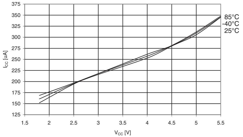
Figure 29-236. ATmega325PA: Active Supply Current with ADC at 200kHz vs. V_{CC}
