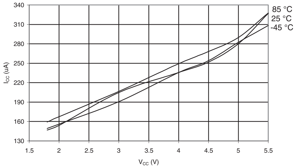
Figure 29-601. ATmega6450P: Active Supply Current with ADC at 1MHz vs. V_{CC}
