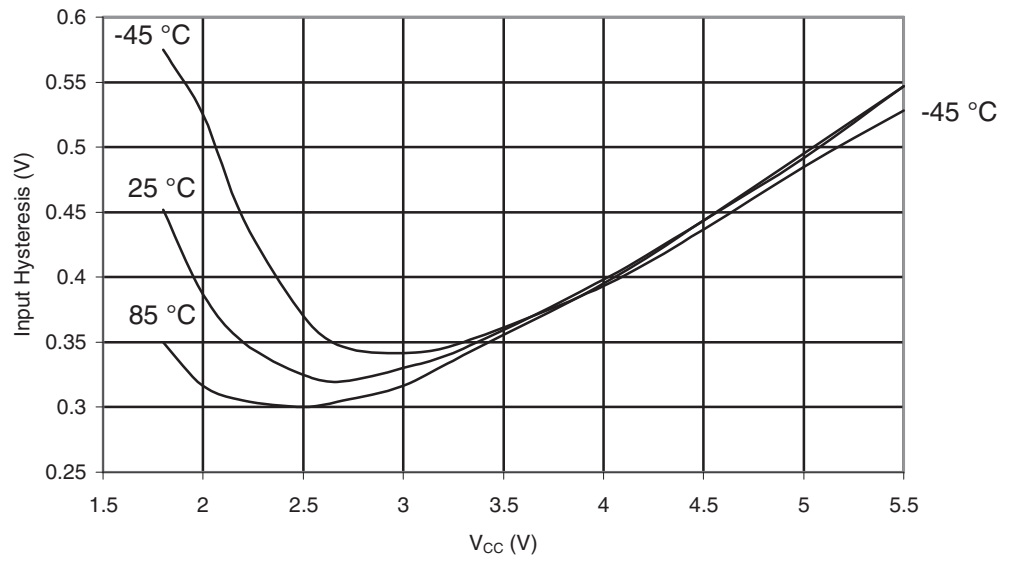
Figure 29-462. ATmega645P: I/O Pin Input Hysteresis vs. V_{CC}
