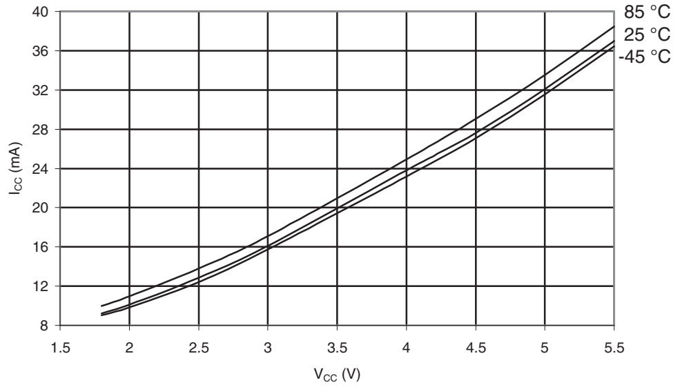
Figure 29-369. ATmega645A: Active Supply Current vs. V_{CC} (32kHz Watch Crystal)
