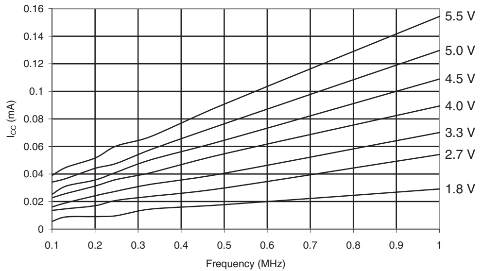
Figure 29-122. ATmega165PA: Reset Supply Current vs. V_{CC} (0.1 - 1.0MHz, Excluding Current Through The Reset Pull-up)
