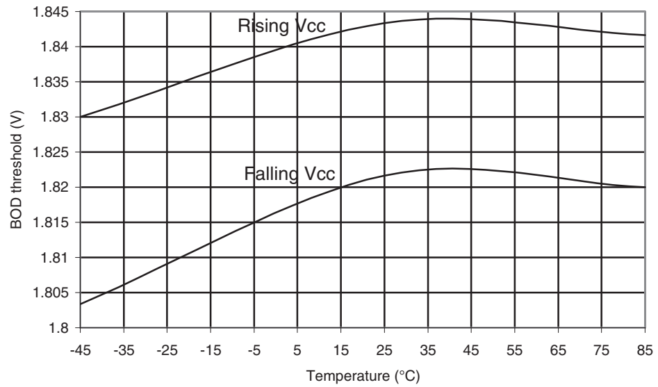
Figure 29-529. ATmega6450A: BOD Thresholds vs. Temperature (BOD Level is 1.8V)
