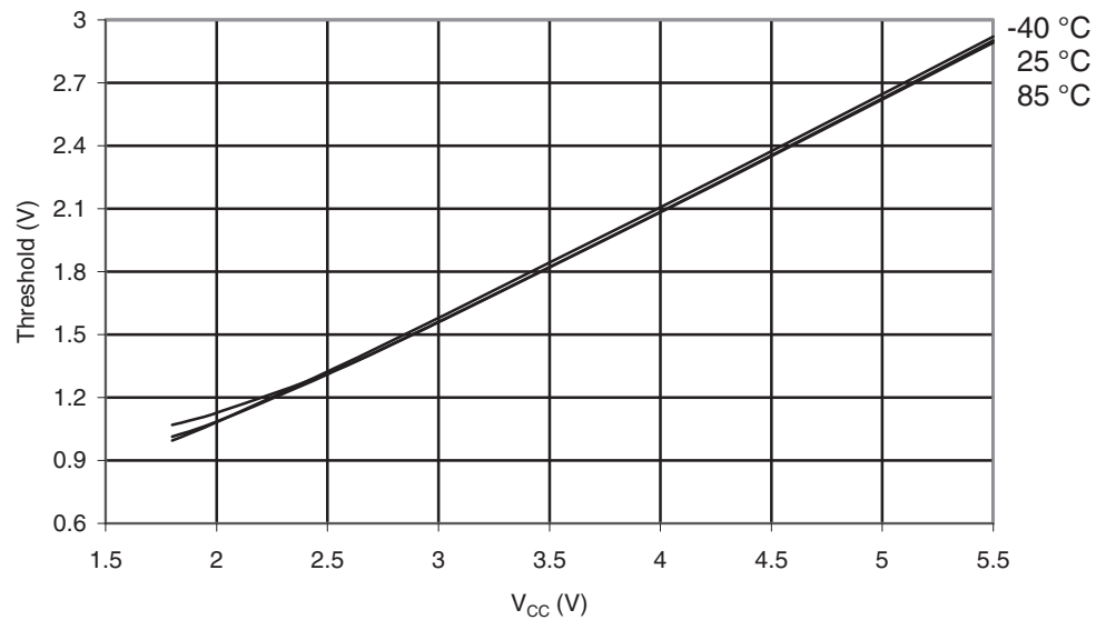
Figure 29-338. ATmega3250PA: I/O Pin Input Threshold Voltage vs. V_{CC} ( V_{IH} , I/O Pin Read as "1")
