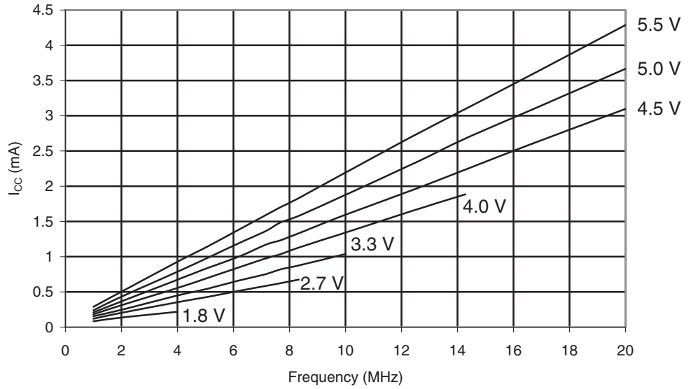
Figure 29-493. ATmega6450A: Idle Supply Current vs. Frequency (1 - 20MHz)
