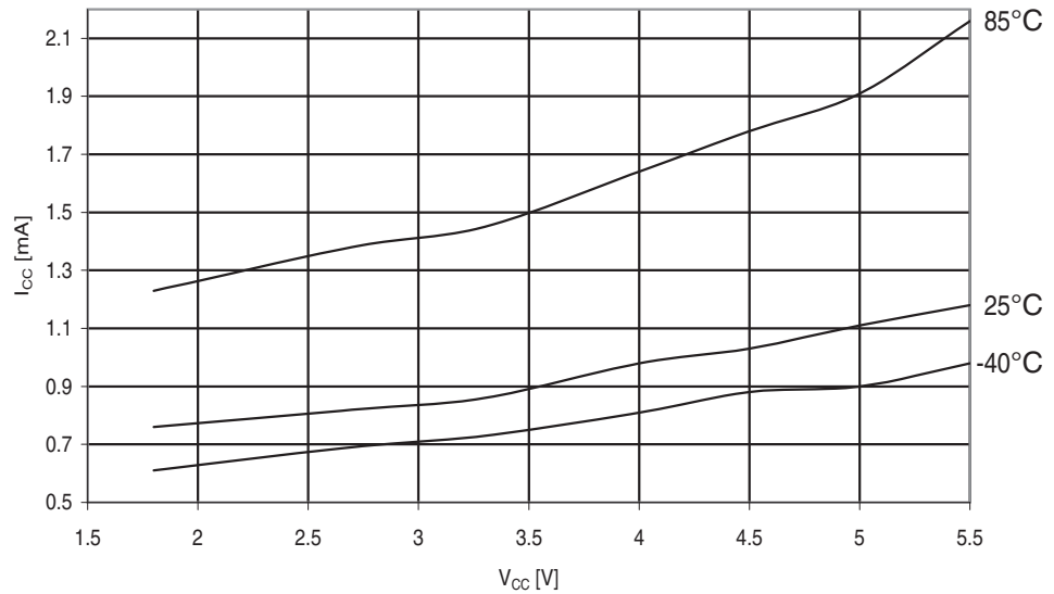
Figure 29-317. ATmega3250PA: Power-save Supply Current vs. V_{CC} (Watchdog Timer Disabled and 32kHz Crystal Oscillator Running)
