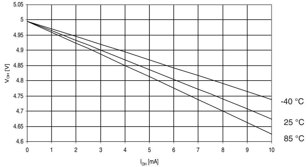
Figure 29-326. ATmega3250PA: I/O Pin Output Voltage vs. Source Current, Ports A, C, D, E, F, G ( V_{CC} = 5V )
