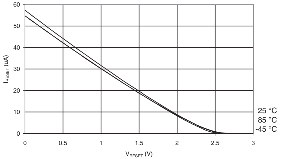
Figure 29-20. ATmega165A: Reset Pull-up Resistor Current vs. Reset Pin Voltage ( V_{CC} = 2.7V )
