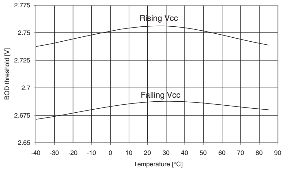
Figure 29-165. ATmega325A: BOD Thresholds vs. Temperature (BOD Level is 2.7V)
