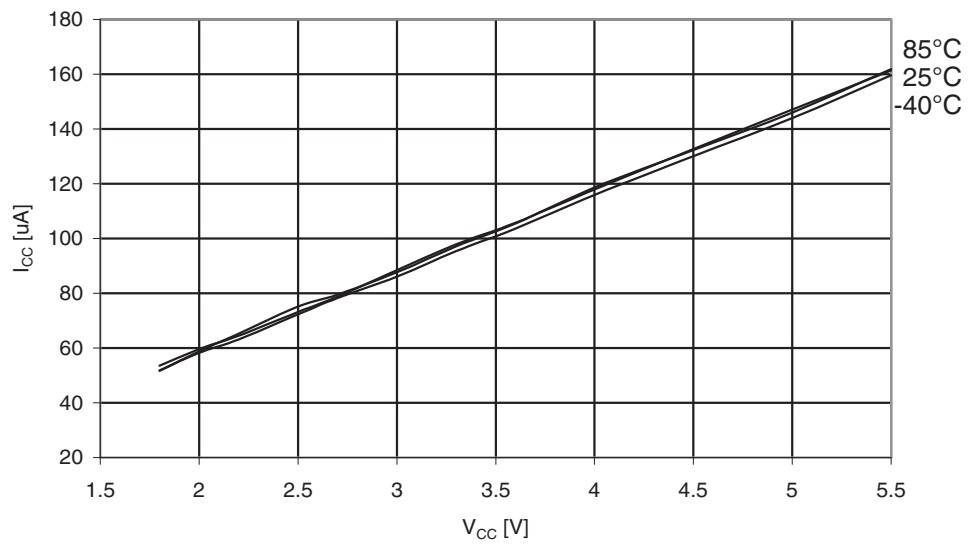
Figure 29-298. ATmega3250A: AREF External Reference Current vs. V_{CC}
