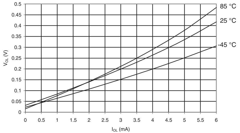
Figure 29-581. ATmega6450P: I/O Pin Output Voltage vs. Sink Current, Port B ( V_{CC} = 1.8V )
