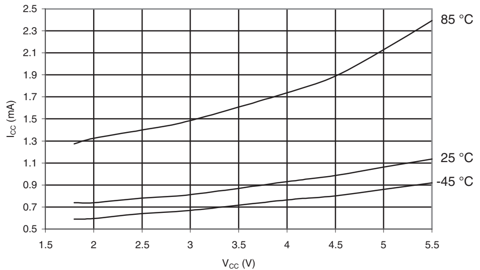
Figure 29-439. ATmega645P: Power-save Supply Current vs. V_{CC} (Watchdog Timer Disabled and 32kHz Crystal Oscillator Running)
