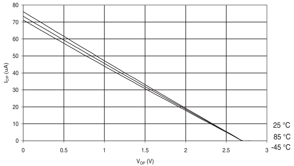
Figure 29-443. ATmega645P: I/O Pin Pull-up Resistor Current vs. Input Voltage ( V_{CC} = 2.7V )
