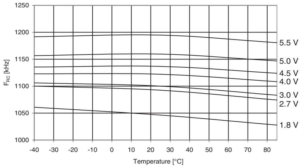
Figure 29-290. ATmega3250A: Watchdog Oscillator Frequency vs. Temperature
