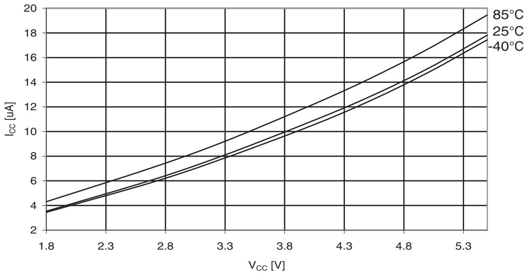
Figure 29-316. ATmega3250PA: Power-down Supply Current vs. V_{CC} (Watchdog Timer Enabled)
