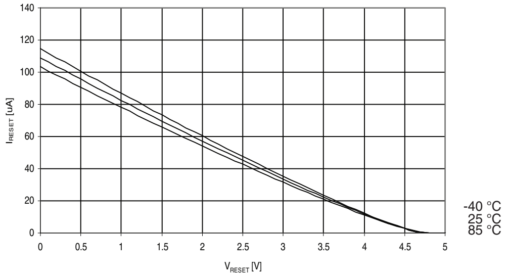
Figure 29-143. ATmega325A: Reset Pull-up Resistor Current vs. Reset Pin Voltage ( V_{CC} = 5V )
