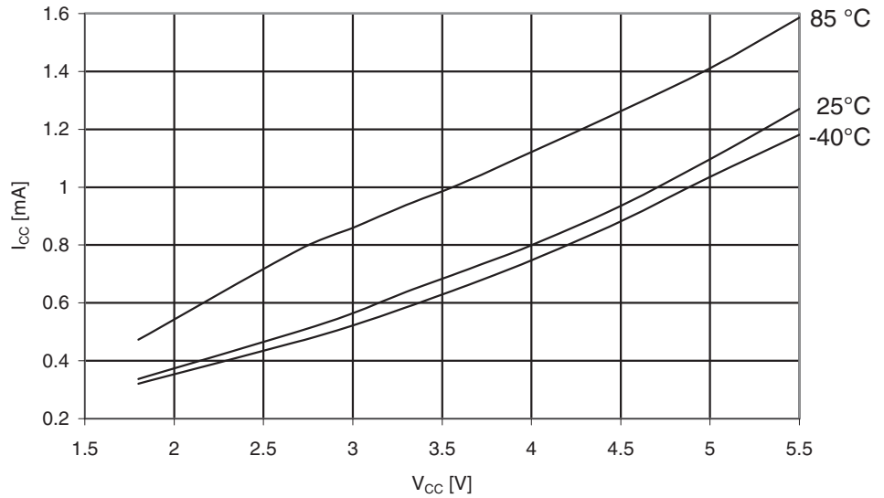
Figure 29-248. ATmega3250A: Active Supply Current vs. V_{CC} (Internal RC Oscillator, 1MHz)
