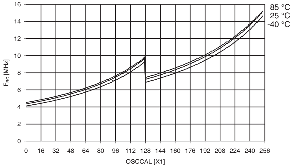
Figure 29-293. ATmega3250A: Calibrated 8MHz RC Oscillator Frequency vs. Oscscal Value
