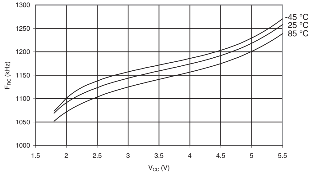
Figure 29-109. ATmega165A: Watchdog Oscillator Frequency vs. V_{CC}
