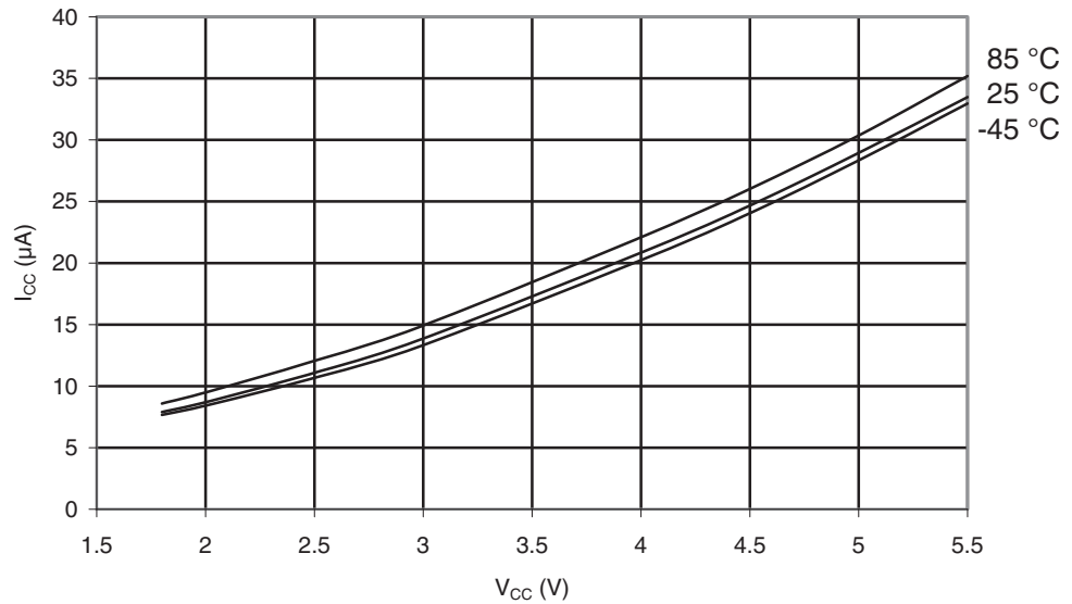
Figure 29-5. ATmega165A: Active Supply Current vs. V_{CC} (32kHz Watch Crystal)
