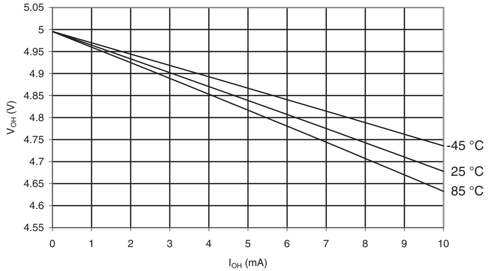
Figure 29-22. ATmega165A: I/O Pin Output Voltage vs. Source Current, Ports A, C, D, E, F, G ( V_{CC} = 5V )
