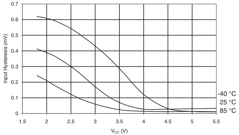
Figure 29-163. ATmega325A: Reset Input Pin Hysteresis vs. V_{CC}
