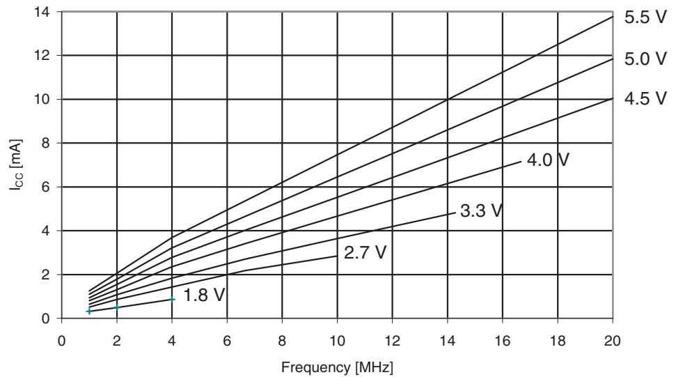
Figure 29-246. ATmega3250A: Active Supply Current vs. Frequency (1 - 20MHz)
