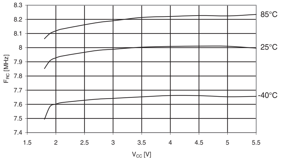
Figure 29-232. ATmega325PA: Calibrated 8MHz RC Oscillator Frequency vs. V_{CC}
