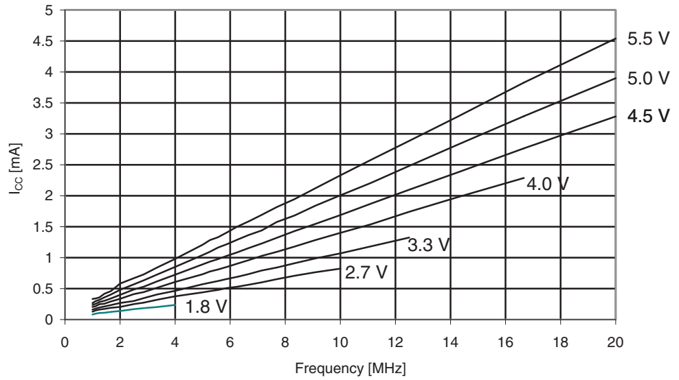
Figure 29-251. ATmega3250A: Idle Supply Current vs. Frequency (1 - 20MHz)
