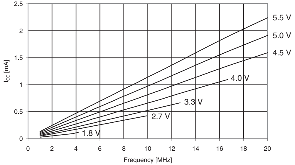
Figure 29-183. ATmega325A: Reset Supply Current vs. V_{CC} (1 - 20MHz, Excluding Current Through The Reset Pull-up)
