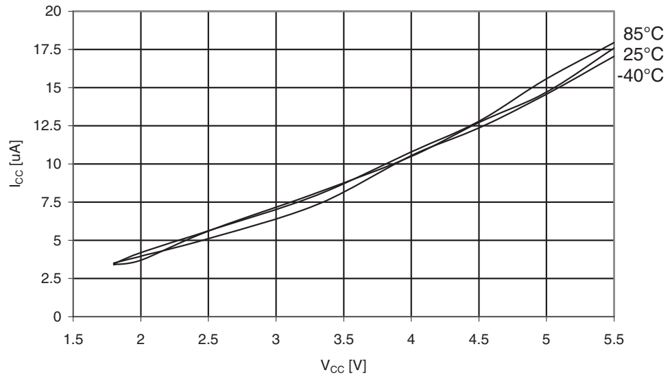
Figure 29-179. ATmega325A: Watchdog Timer Current vs. V_{CC}
