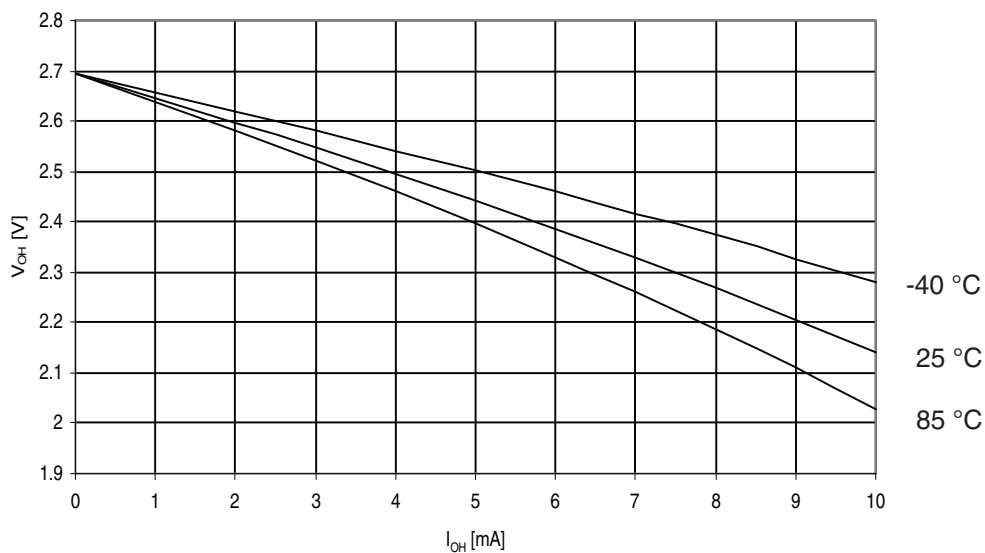
Figure 29-207. ATmega325PA: I/O Pin Output Voltage vs. Source Current, Ports A, C, D, E, F, G ( V_{CC} = 2.7V )
