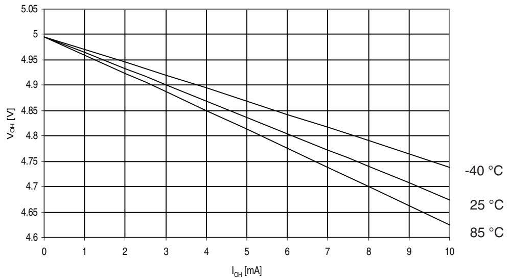
Figure 29-206. ATmega325PA: I/O Pin Output Voltage vs. Source Current, Ports A, C, D, E, F, G ( V_{CC} = 5V )
