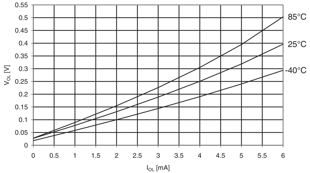
Figure 29-337. ATmega3250PA: I/O Pin Output Voltage vs. Sink Current, Port B ( V_{CC} = 1.8V )
