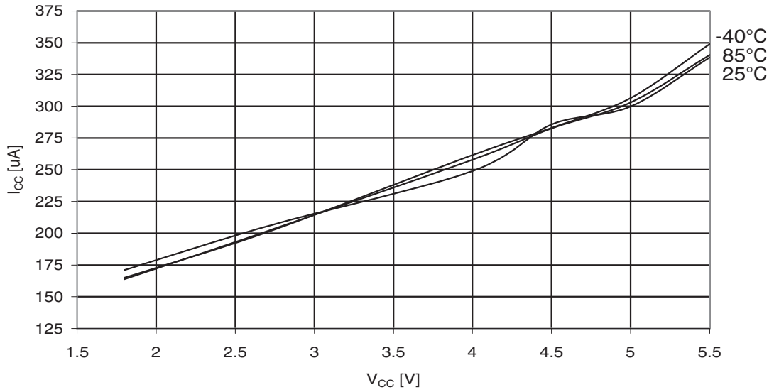
Figure 29-237. ATmega325PA: Active Supply Current with ADC at 1MHz vs. V_{CC}
