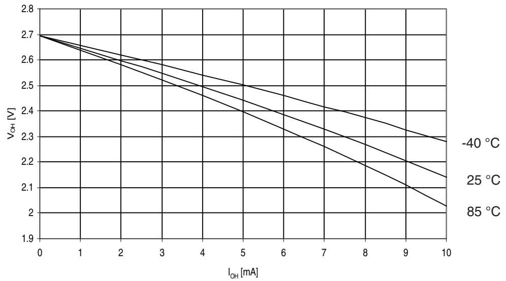
Figure 29-267. ATmega3250A: I/O Pin Output Voltage vs. Source Current, Ports A, C, D, E, F, G ( V_{CC} = 2.7V )
