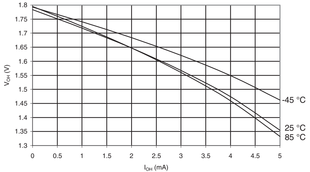
Figure 29-453. ATmega645P: I/O Pin Output Voltage vs. Source Current, Port B ( V_{CC} = 1.8V )
