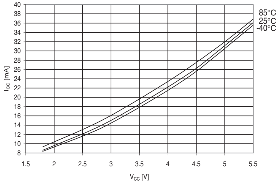
Figure 29-249. ATmega3250A: Active Supply Current vs. V_{CC} (32kHz Watch Crystal)
