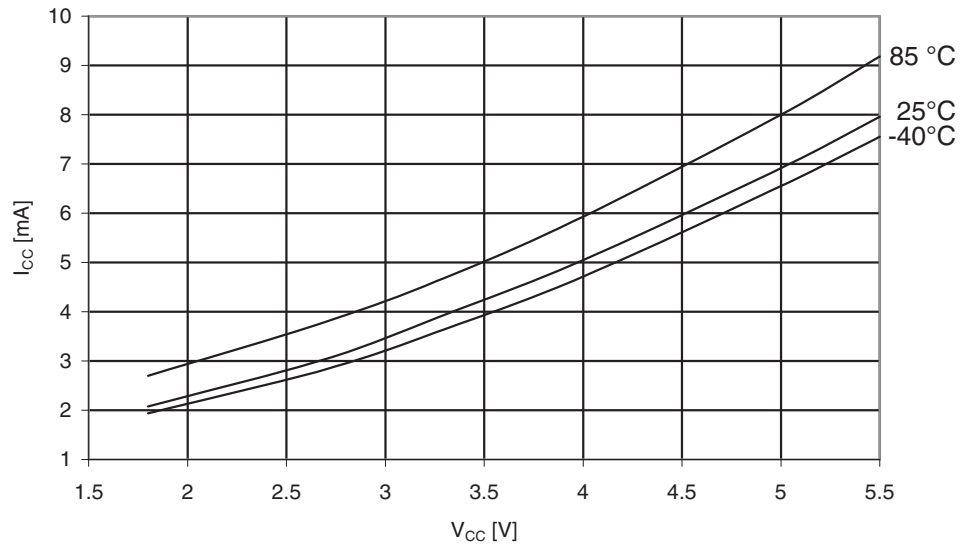
Figure 29-134. ATmega325A: Idle Supply Current vs. V_{CC} (32kHz Watch Crystal)
