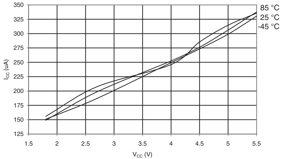
Figure 29-55. ATmega165A: Active Supply Current with ADC at 1MHz vs. V_{CC}
