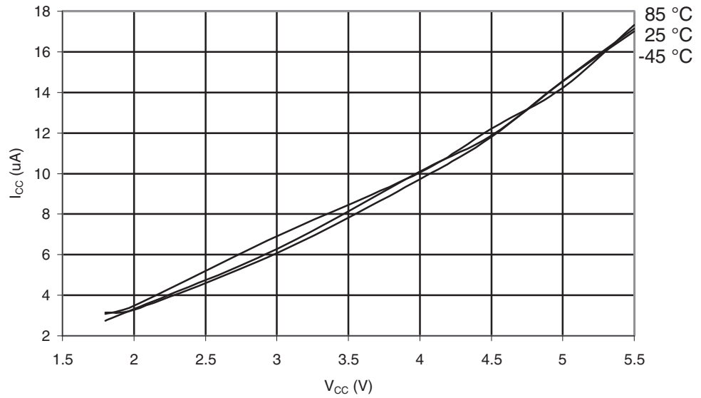
Figure 29-420. ATmega645A: Watchdog Timer Current vs. V_{CC}
