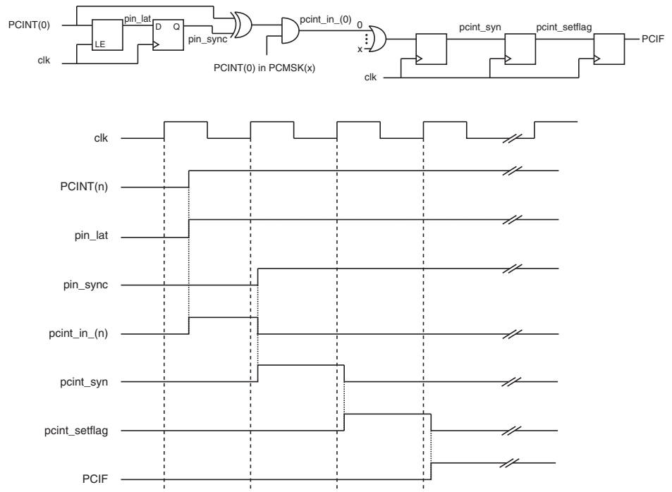
Figure 13-1. Pin Change Interrupt
