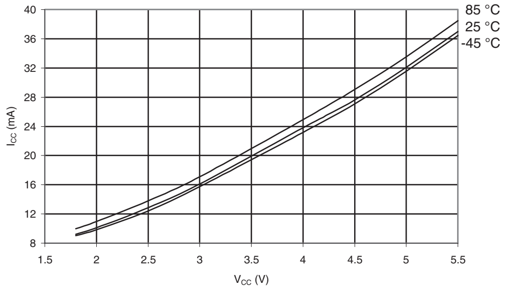
Figure 29-430. ATmega645P: Active Supply Current vs. V_{CC} (32kHz Watch Crystal)
