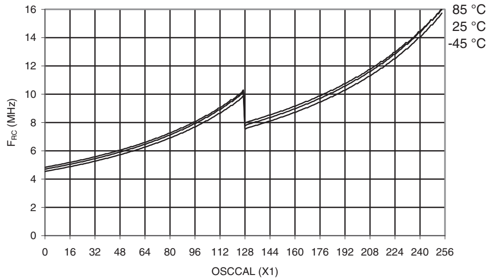
Figure 29-51. ATmega165A: Calibrated 8MHz RC Oscillator Frequency vs. OSCCAL Value
