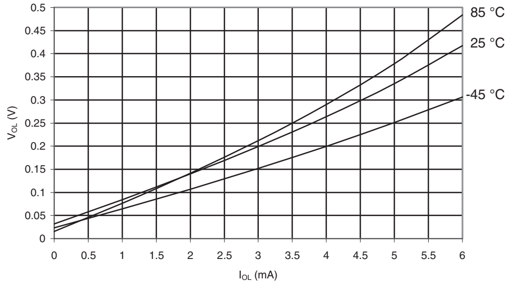
Figure 29-398. ATmega645A: I/O Pin Output Voltage vs. Sink Current, Port B ( V_{CC} = 1.8V )
