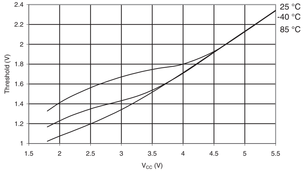
Figure 29-221. ATmega325PA: Reset Input Threshold Voltage vs. V_{CC} ( V_{IH} , Reset Pin Read as “1”)
