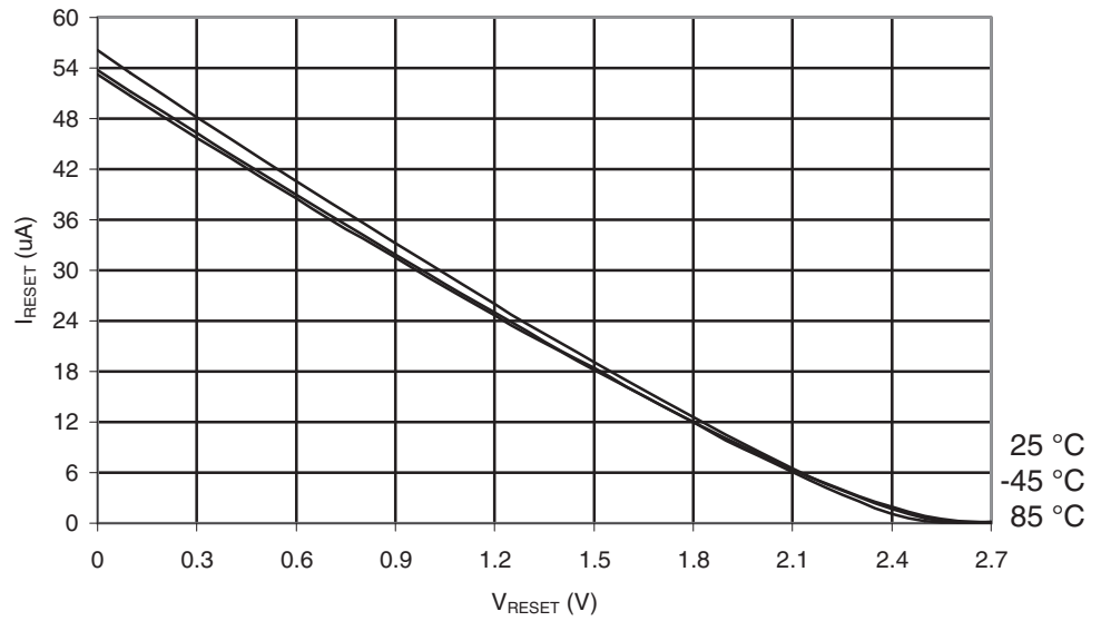
Figure 29-446. ATmega645P: Reset Pull-up Resistor Current vs. Reset Pin Voltage ( V_{CC} = 2.7V )
