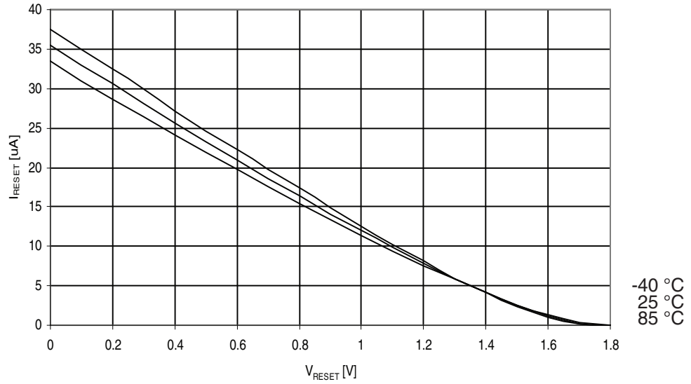
Figure 29-325. ATmega3250PA: Reset Pull-up Resistor Current vs. Reset Pin Voltage ( V_{CC} = 1.8V )
