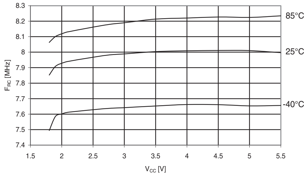
Figure 29-292. ATmega3250A: Calibrated 8MHz RC Oscillator Frequency vs. V_{CC}
