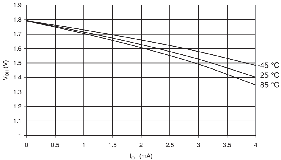
Figure 29-24. ATmega165A: I/O Pin Output Voltage vs. Source Current, Ports A, C, D, E, F, G ( V_{CC} = 1.8V )
