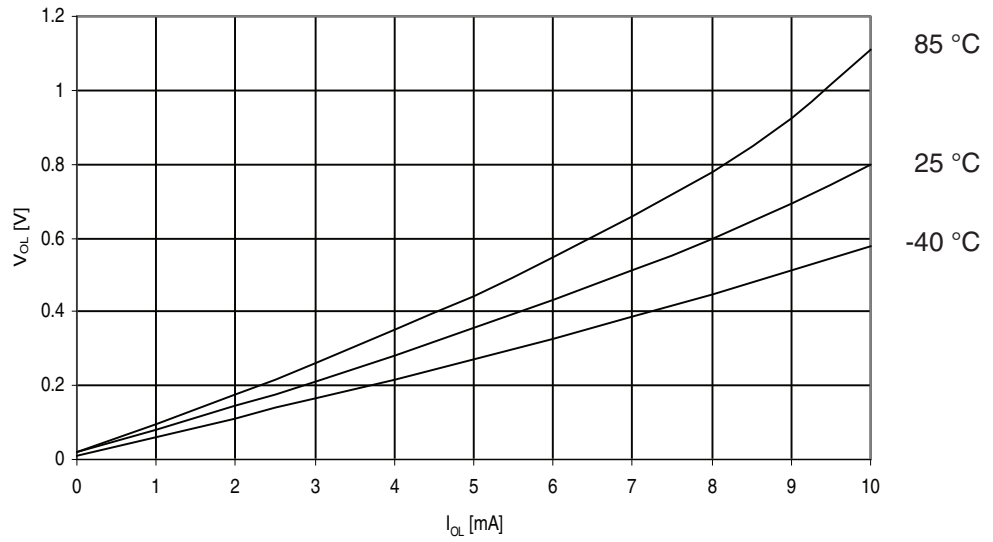
Figure 29-273. ATmega3250A: I/O Pin Output Voltage vs. Sink Current, Ports A, C, D, E, F, G ( V_{CC} = 2.7V )
