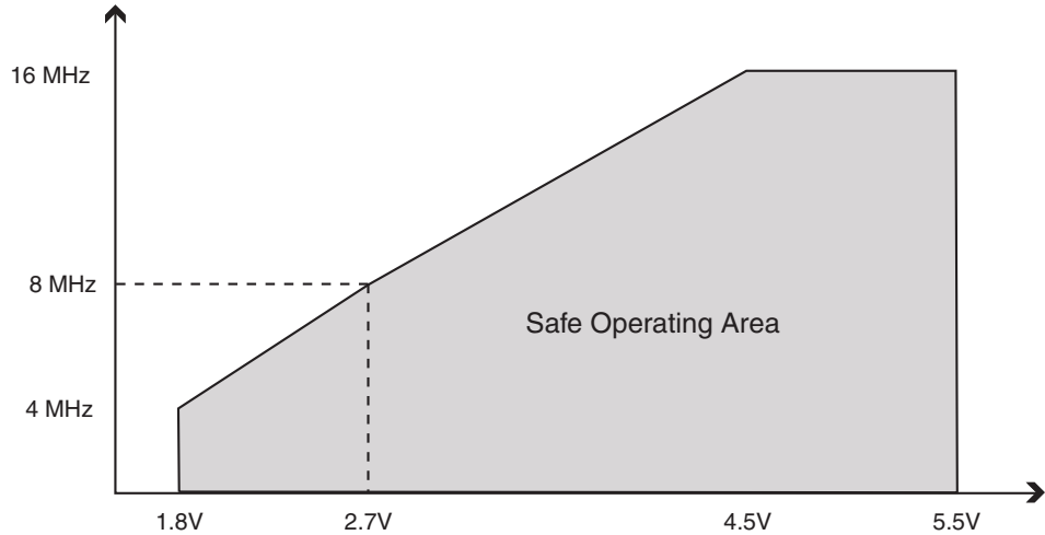
Figure 28-1. Maximum Frequency vs. V_{CC} : ATmega165A/165PA/ATmega645A/ATmega645P
