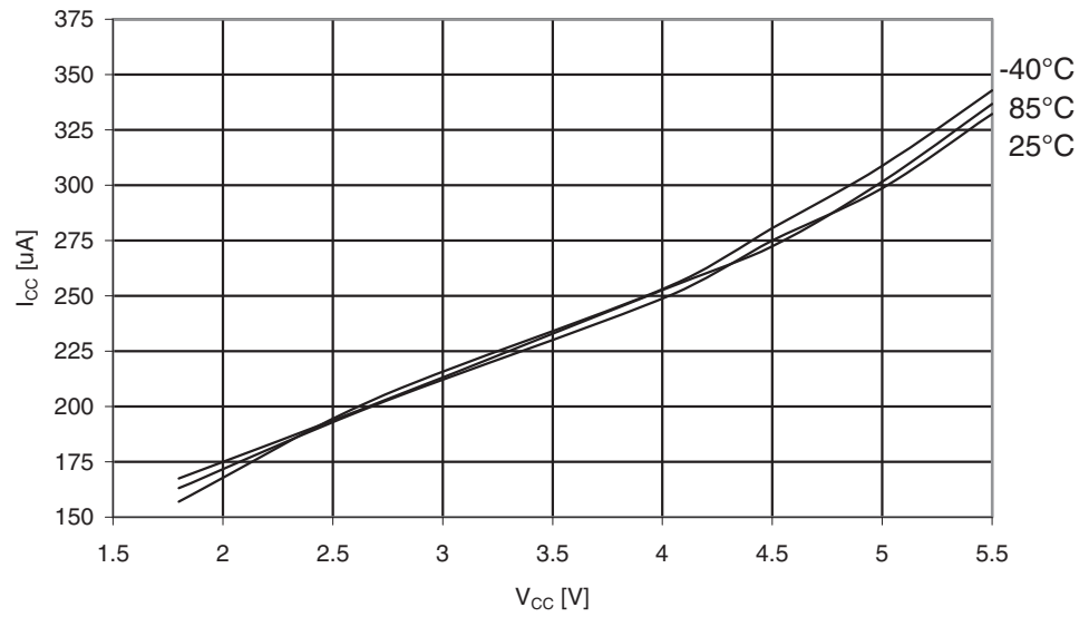
Figure 29-175. ATmega325A: Active Supply Current with ADC at 50kHz vs. V_{CC}
