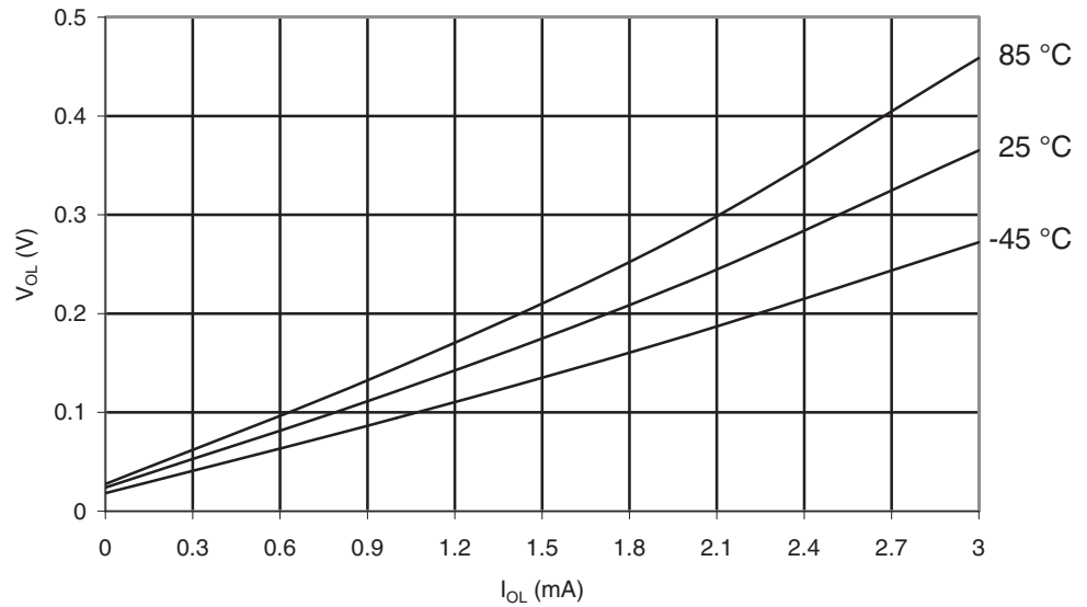
Figure 29-30. ATmega165A: I/O Pin Output Voltage vs. Sink Current, Ports A, C, D, E, F, G ( V_{CC} = 1.8V )
