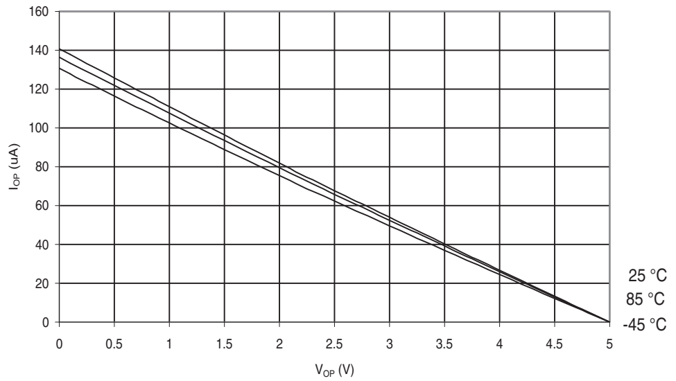
Figure 29-381. ATmega645A: I/O Pin Pull-up Resistor Current vs. Input Voltage ( V_{CC} = 5V )
