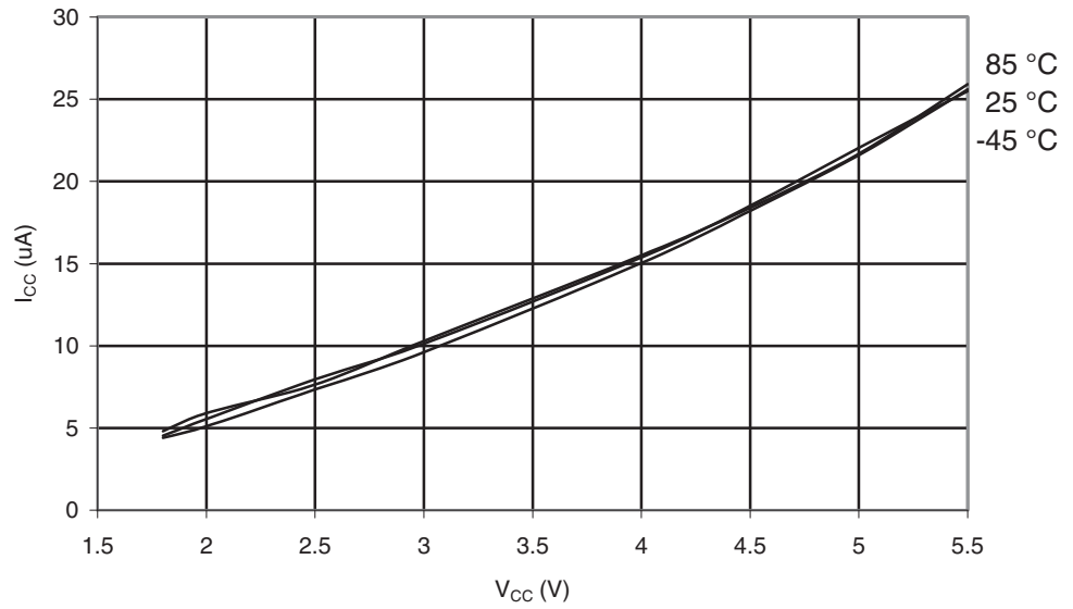
Figure 29-119. ATmega165A: Watchdog Timer Current vs. V_{CC}
