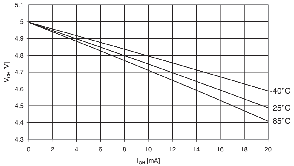
Figure 29-269. ATmega3250A: I/O Pin Output Voltage vs. Source Current, Port B ( V_{CC} = 5V )
