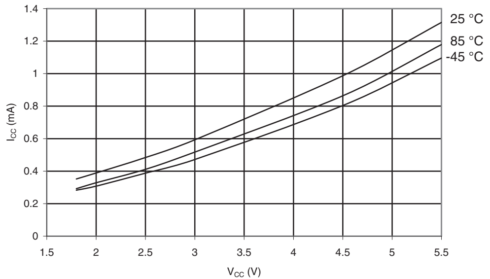
Figure 29-9. ATmega165A: Idle Supply Current vs. V_{CC} (Internal RC Oscillator, 1 MHz)
