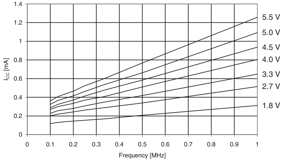
Figure 29-185. ATmega325PA: Active Supply Current vs. Frequency (0.1 - 1.0MHz)
