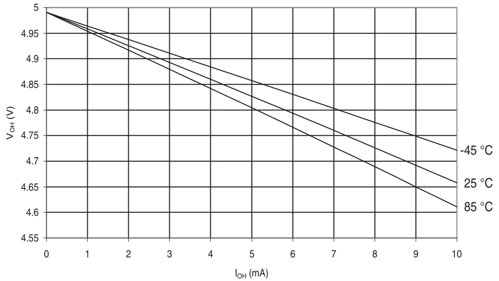
Figure 29-570. ATmega6450A: I/O Pin Output Voltage vs. Source Current, Ports A, C, D, E, F, G ( V_{CC} = 5V )
