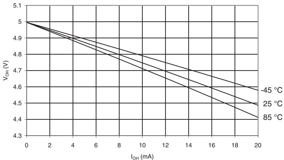
Figure 29-25. ATmega165A: I/O Pin Output Voltage vs. Source Current, Port B ( V_{CC} = 5V )
