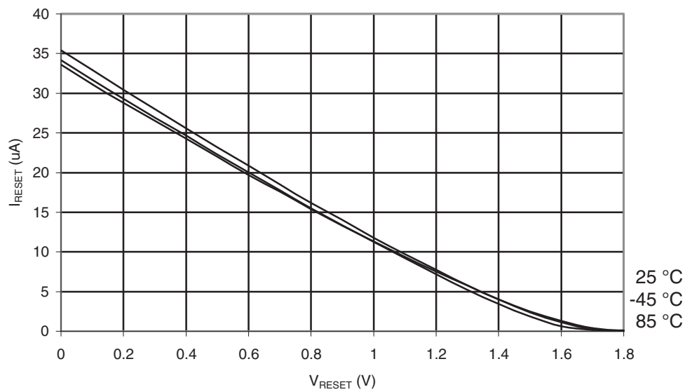
Figure 29-386. ATmega645A: Reset Pull-up Resistor Current vs. Reset Pin Voltage ( V_{CC} = 1.8V )
