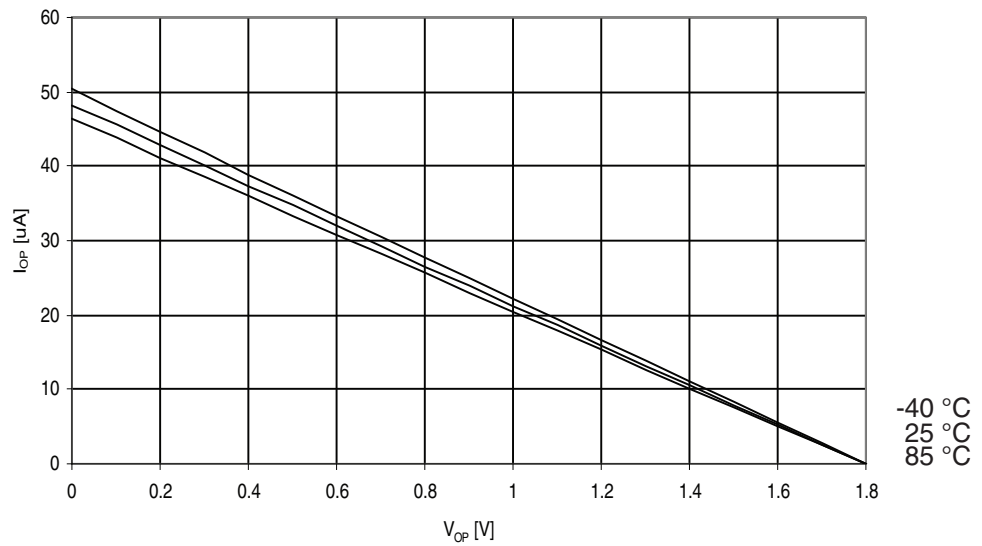
Figure 29-262. ATmega3250A: I/O Pin Pull-up Resistor Current vs. Input Voltage ( V_{CC} = 1.8V )
