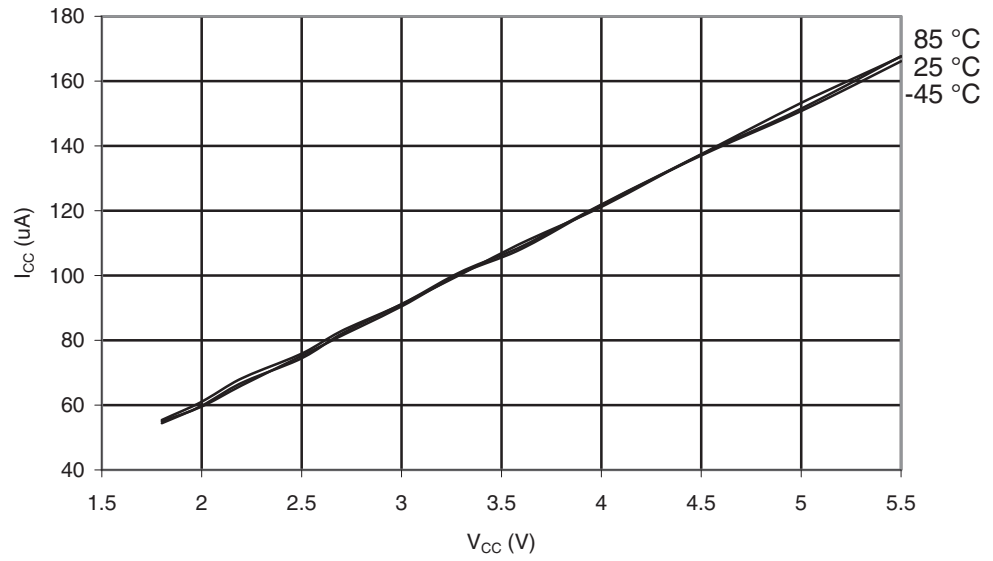
Figure 29-56. ATmega165A: AREF External Reference Current vs. V_{CC}
