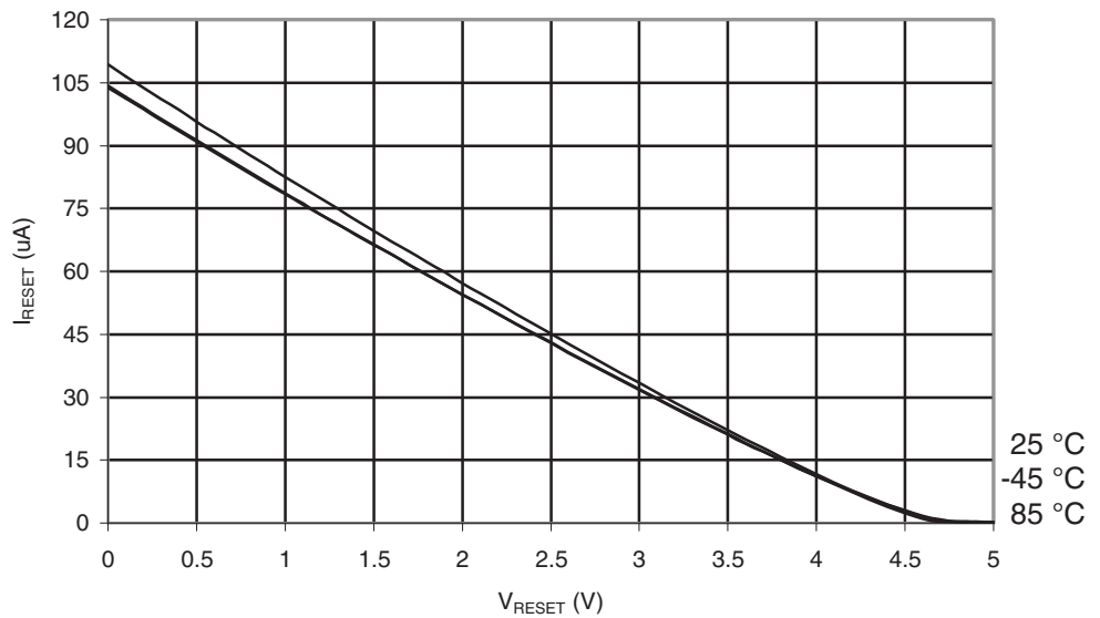
Figure 29-506. ATmega6450A: Reset Pull-up Resistor Current vs. Reset Pin Voltage ( V_{CC} = 5V )
