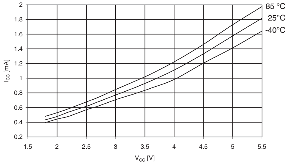
Figure 29-312. ATmega3250PA: Idle Supply Current vs. V_{CC} (Internal RC Oscillator, 8MHz)
