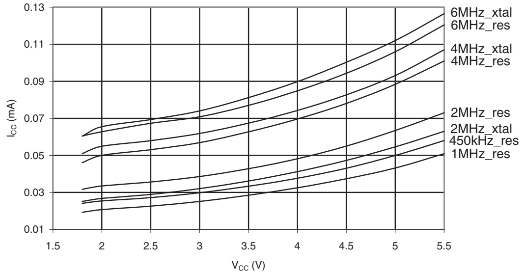
Figure 29-259. ATmega3250A: Standby Supply Current vs. V_{CC} (Xtall and Resonator, Watchdog Timer Disabled)
