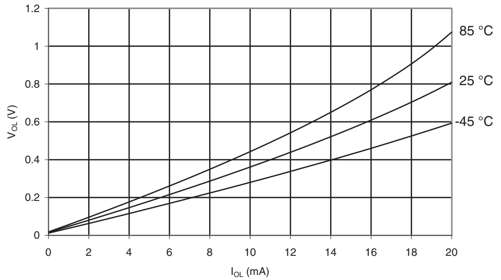
Figure 29-94. ATmega165PA: I/O Pin Output Voltage vs. Sink Current, Port B ( V_{CC} = 2.7V )
