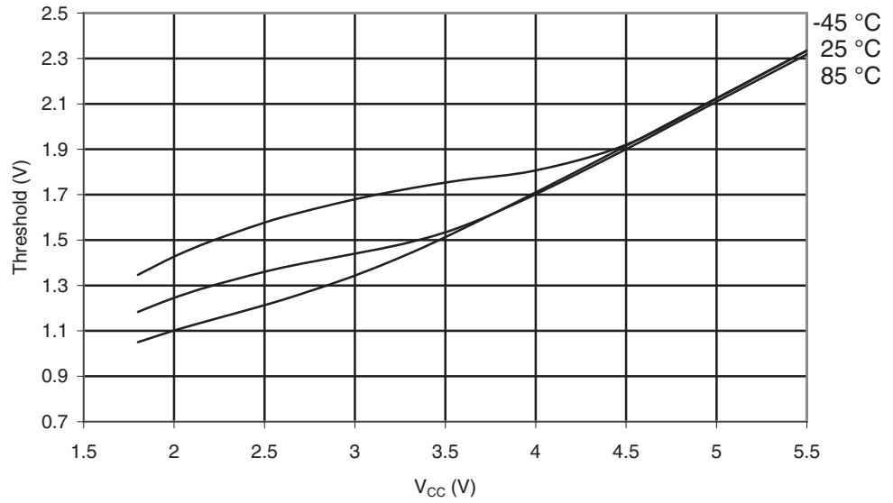
Figure 29-37. ATmega165A: Reset Input Threshold Voltage vs. V_{CC} ( V_{IH} , Reset Pin Read as “1”)
