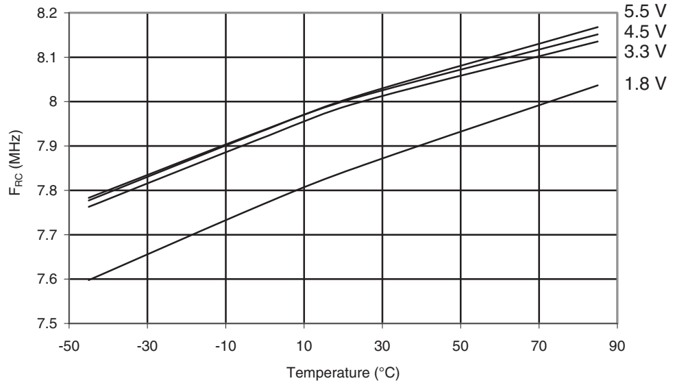
Figure 29-49. ATmega165A: Calibrated 8MHz RC Oscillator Frequency vs. Temperature
