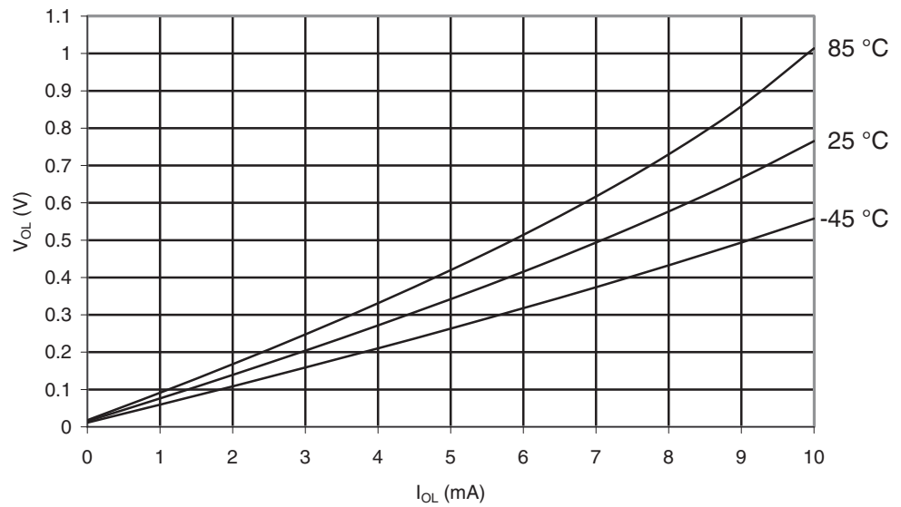
Figure 29-29. ATmega165A: I/O Pin Output Voltage vs. Sink Current, Ports A, C, D, E, F, G ( V_{CC} = 2.7V )
