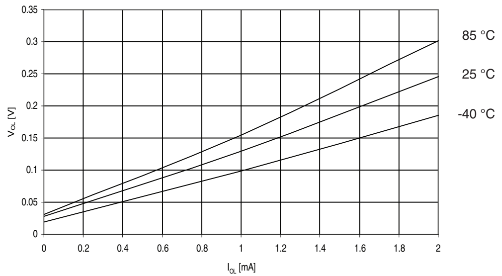
Figure 29-214. ATmega325PA: I/O Pin Output Voltage vs. Sink Current, Ports A, C, D, E, F, G ( V_{CC} = 1.8V )
