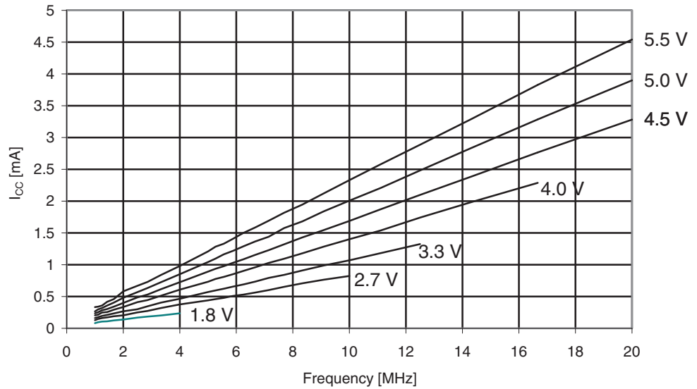
Figure 29-131. ATmega325A: Idle Supply Current vs. Frequency (1 - 20MHz)
