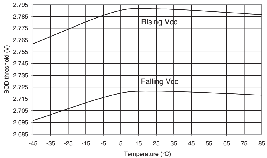
Figure 29-406. ATmega645A: BOD Thresholds vs. Temperature (BOD Level is 2.7V)
