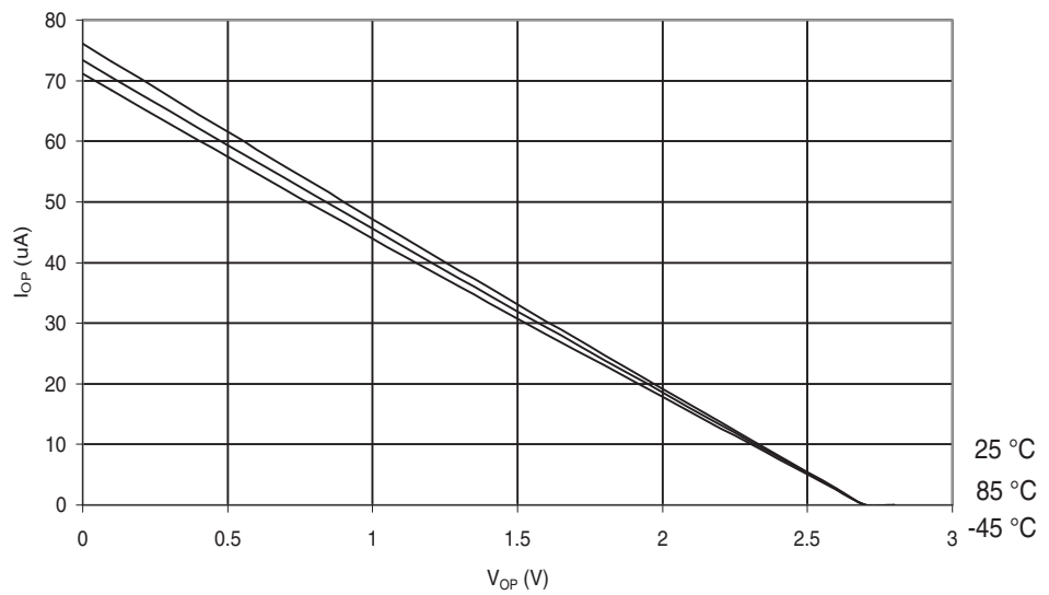
Figure 29-382. ATmega645A: I/O Pin Pull-up Resistor Current vs. Input Voltage ( V_{CC} = 2.7V )
