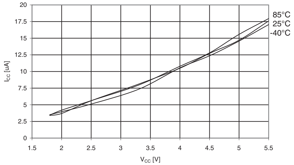
Figure 29-239. ATmega325PA: Watchdog Timer Current vs. V_{CC}
