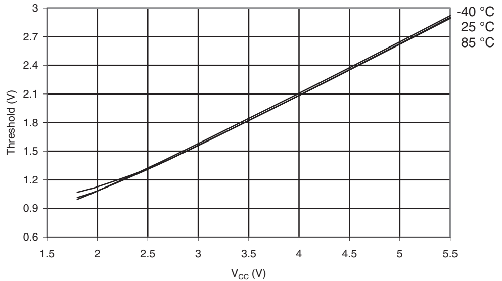
Figure 29-278. ATmega3250A: I/O Pin Input Threshold Voltage vs. V_{CC} ( V_{IH} , I/O Pin Read as "1")
