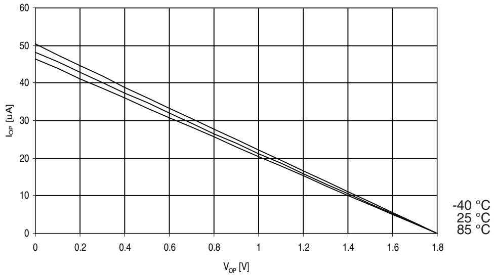
Figure 29-142. ATmega325A: I/O Pin Pull-up Resistor Current vs. Input Voltage ( V_{CC} = 1.8V )
