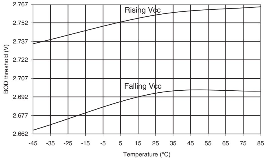
Figure 29-103. ATmega165PA: BOD Thresholds vs. Temperature (BOD Level is 2.7V)
