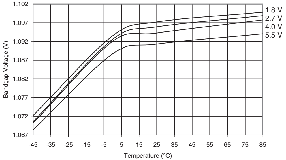
Figure 29-106. ATmega165PA: Bandgap Voltage vs. Temperature
