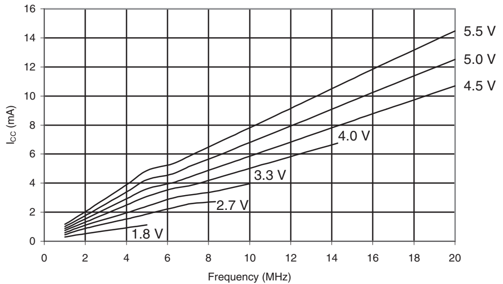
Figure 29-366. ATmega645A: Active Supply Current vs. Frequency (1 - 20MHz)
