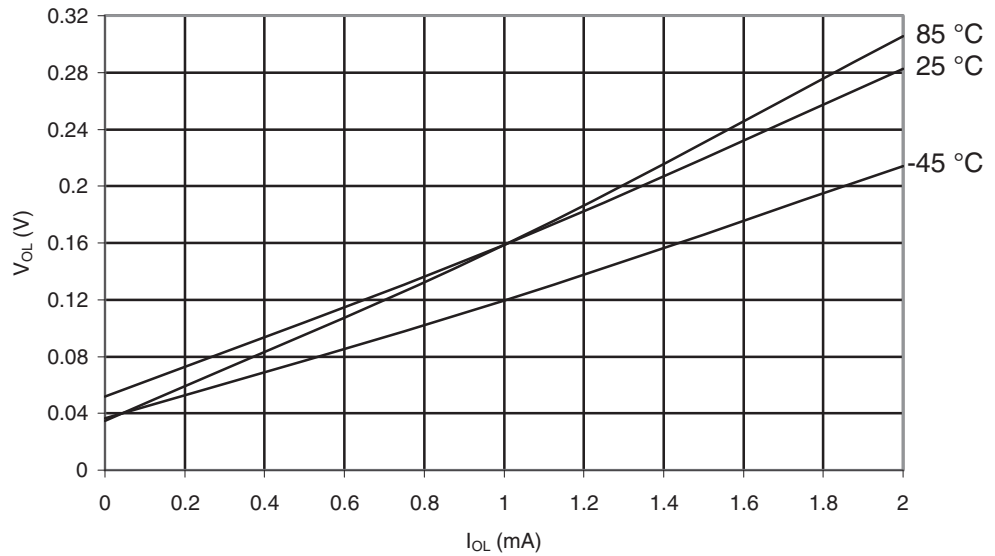
Figure 29-578. ATmega6450A: I/O Pin Output Voltage vs. Sink Current, Ports A, C, D, E, F, G ( V_{CC} = 1.8V )
