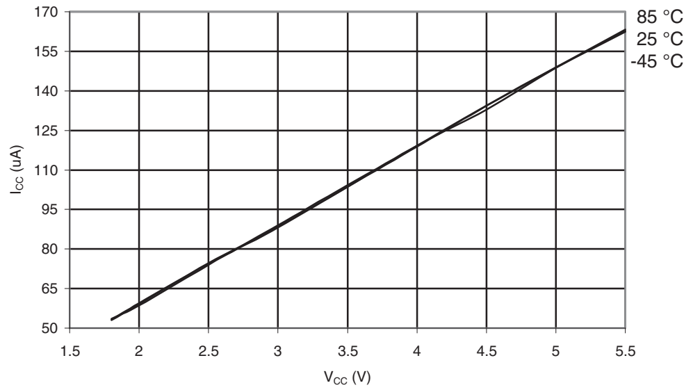
Figure 29-419. ATmega645A: AREF External Reference Current vs. V_{CC}
