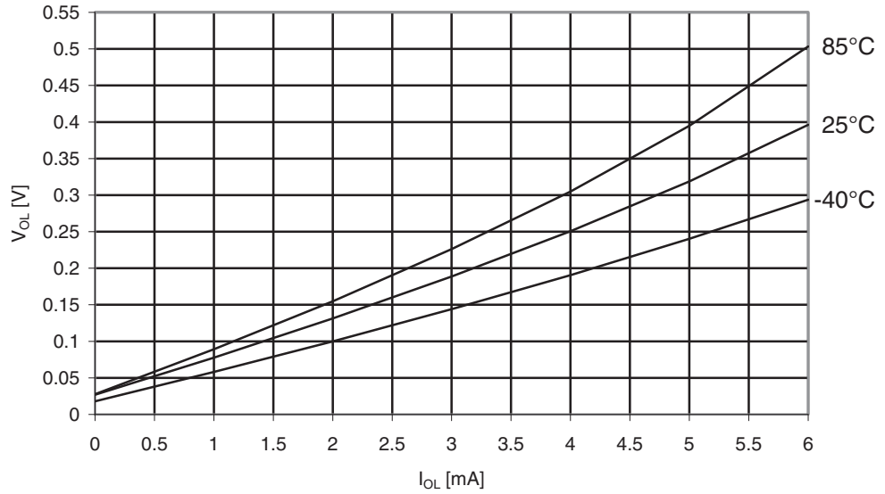
Figure 29-217. ATmega325PA: I/O Pin Output Voltage vs. Sink Current, Port B ( V_{CC} = 1.8V )
