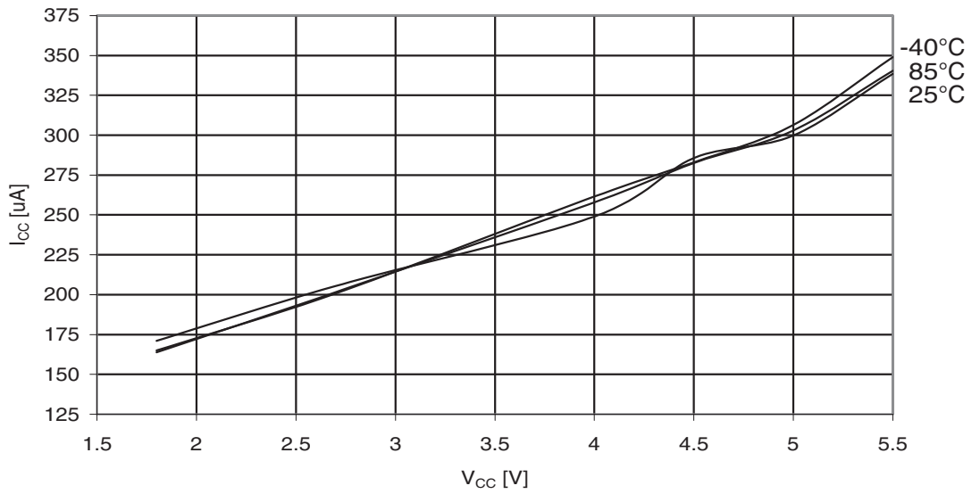
Figure 29-177. ATmega325A: Active Supply Current with ADC at 1MHz vs. V_{CC}
