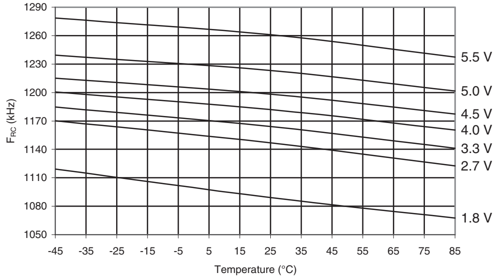
Figure 29-472. ATmega645P: Watchdog Oscillator Frequency vs. Temperature
