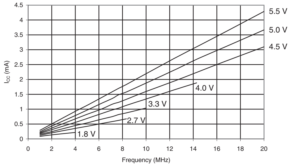
Figure 29-554. ATmega6450A: Idle Supply Current vs. Frequency (1 - 20MHz)
