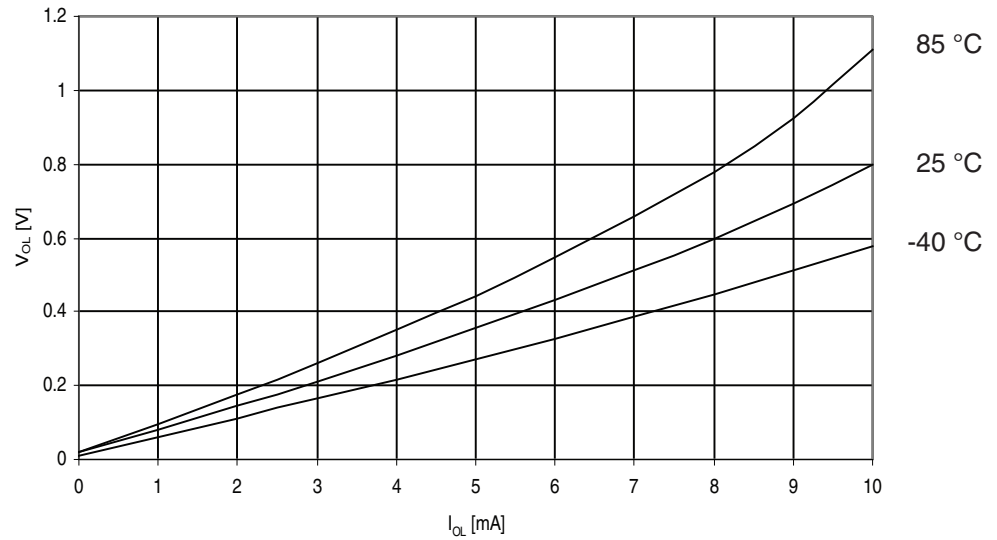
Figure 29-213. ATmega325PA: I/O Pin Output Voltage vs. Sink Current, Ports A, C, D, E, F, G ( V_{CC} = 2.7V )
