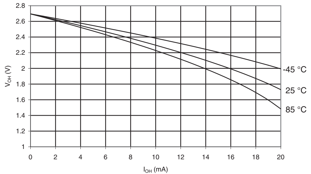
Figure 29-88. ATmega165PA: I/O Pin Output Voltage vs. Source Current, Port B ( V_{CC} = 2.7V )
