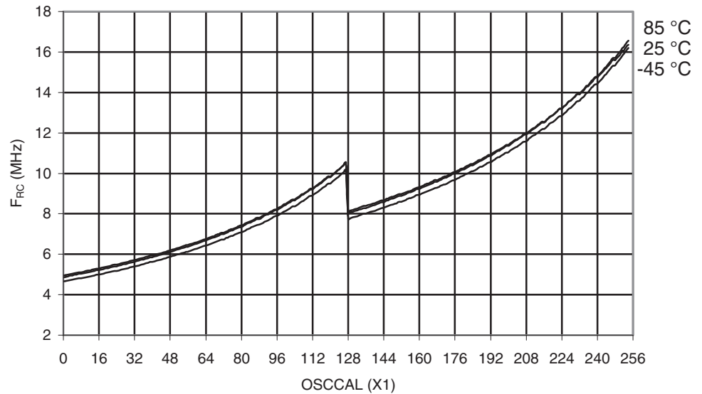
Figure 29-475. ATmega645P: Calibrated 8MHz RC Oscillator Frequency vs. OSCCAL Value
