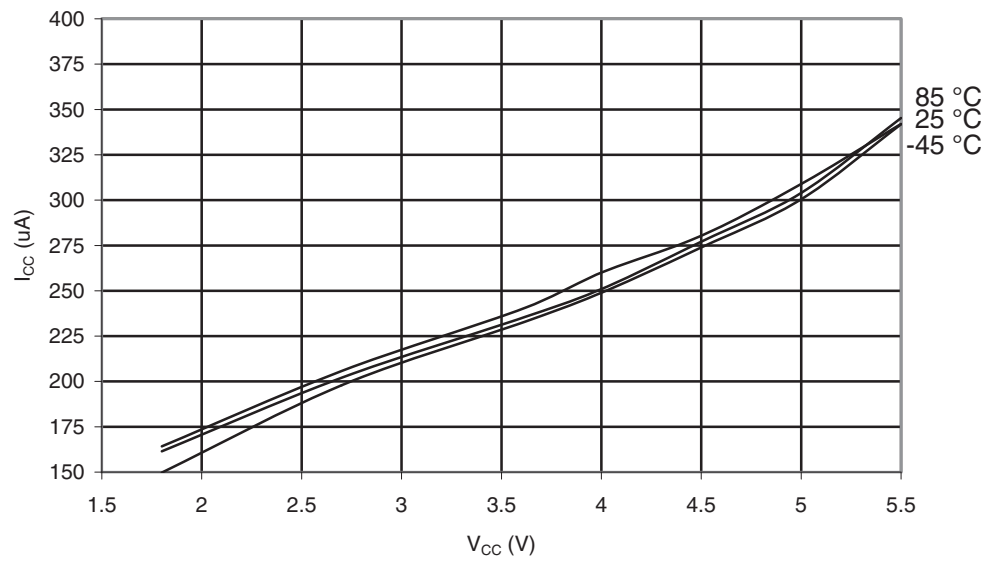
Figure 29-53. ATmega165A: Active Supply Current with ADC at 50kHz vs. V_{CC}
