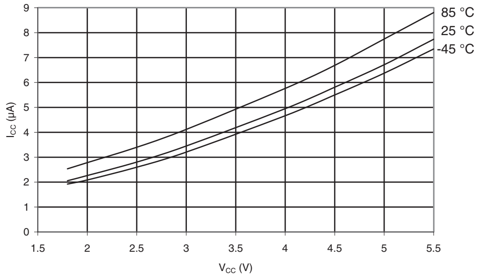
Figure 29-10. ATmega165A: Idle Supply Current vs. V_{CC} (32kHz Watch Crystal)
