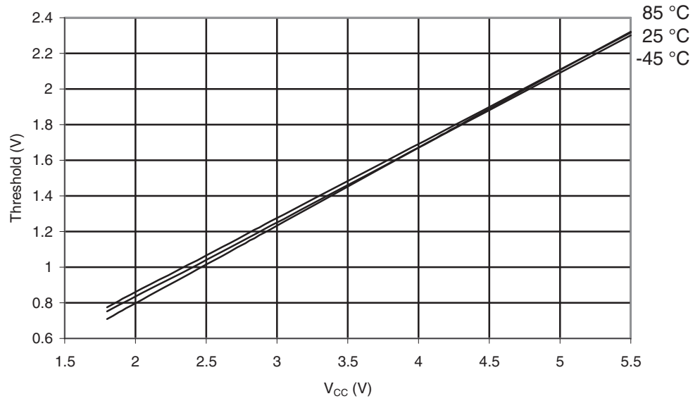
Figure 29-464. ATmega645P: Reset Input Threshold Voltage vs. V_{CC} ( V_{IL,Reset} Pin Read as "0")
