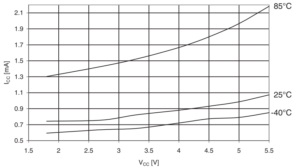
Figure 29-318. ATmega3250PA: Standby Supply Current vs. V_{CC} (32kHz Watch Crystal, Watchdog Timer Disabled)
