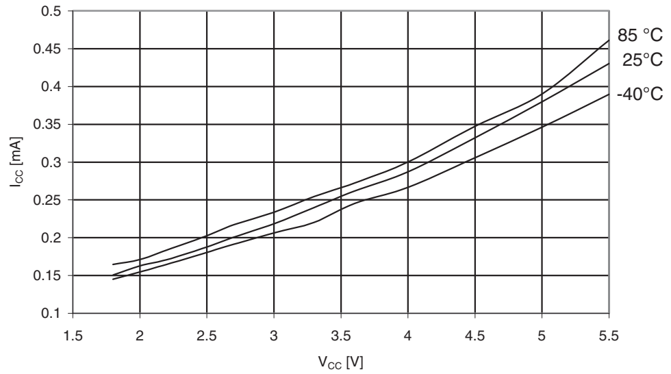
Figure 29-253. ATmega3250A: Idle Supply Current vs. V_{CC} (Internal RC Oscillator, 1 MHz)
