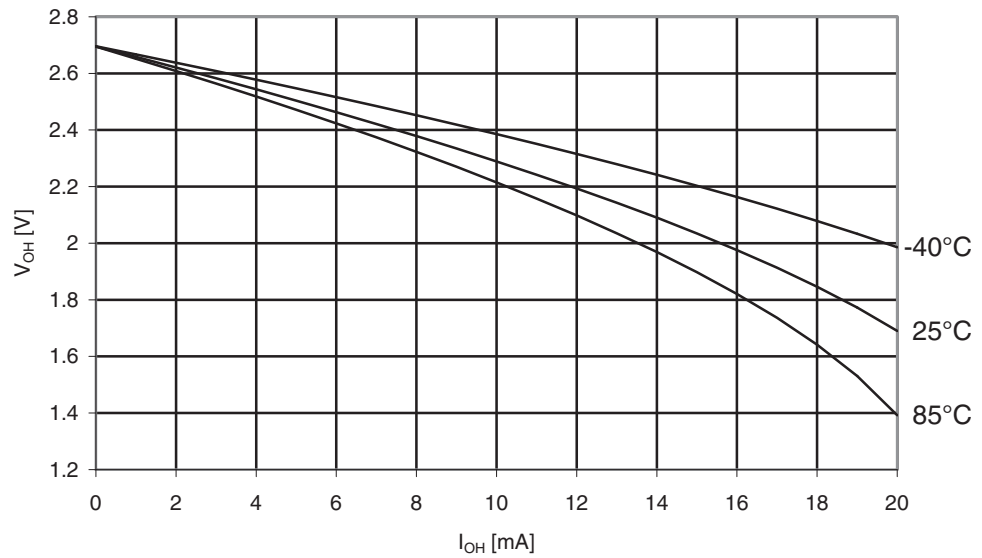
Figure 29-330. ATmega3250PA: I/O Pin Output Voltage vs. Source Current, Port B ( V_{CC} = 2.7V )
