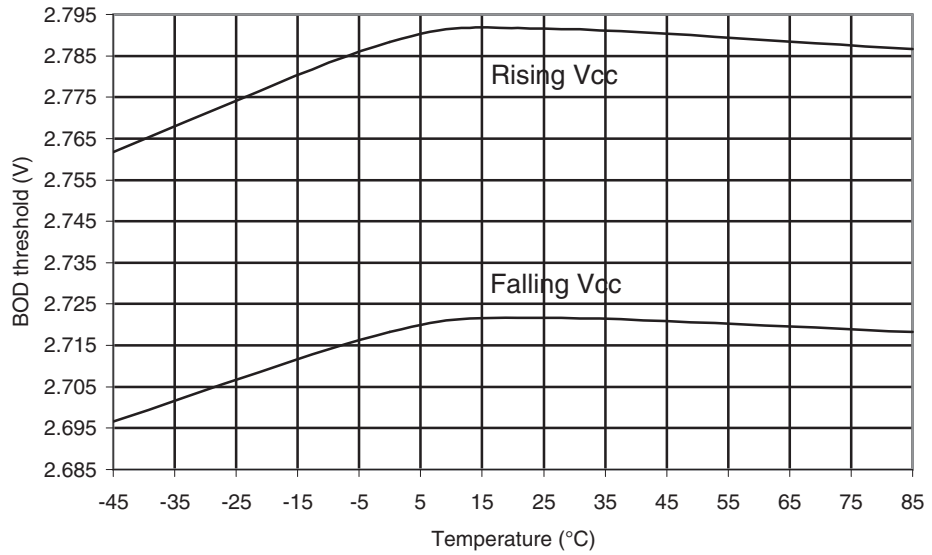
Figure 29-589. ATmega6450P: BOD Thresholds vs. Temperature (BOD Level is 2.7V)
