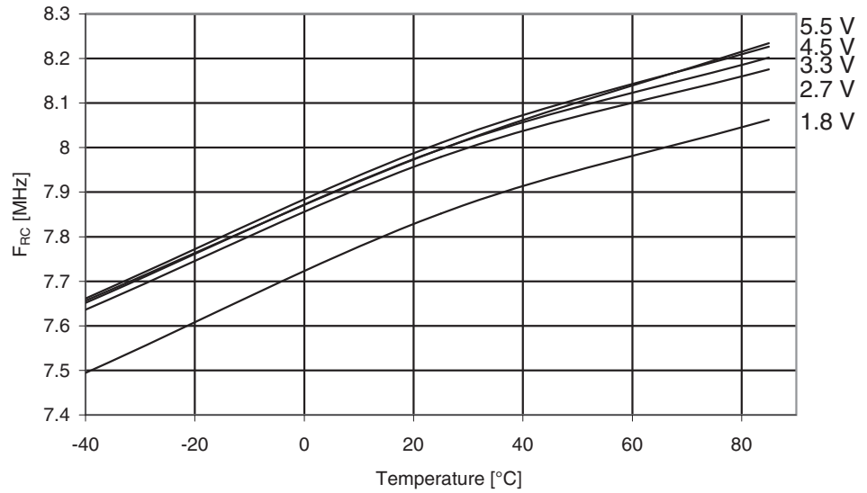
Figure 29-231. ATmega325PA: Calibrated 8MHz RC Oscillator Frequency vs. Temperature
