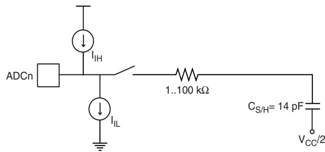
Figure 23-8. Analog Input Circuitry
