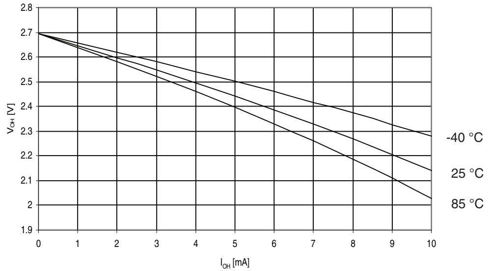
Figure 29-147. ATmega325A: I/O Pin Output Voltage vs. Source Current, Ports A, C, D, E, F, G ( V_{CC} = 2.7V )
