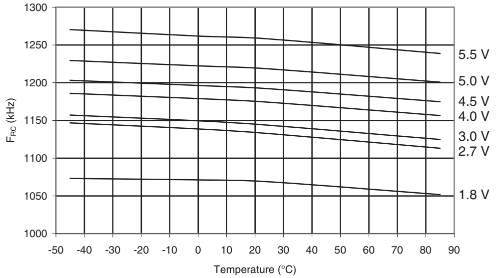
Figure 29-48. ATmega165A: Watchdog Oscillator Frequency vs. Temperature
