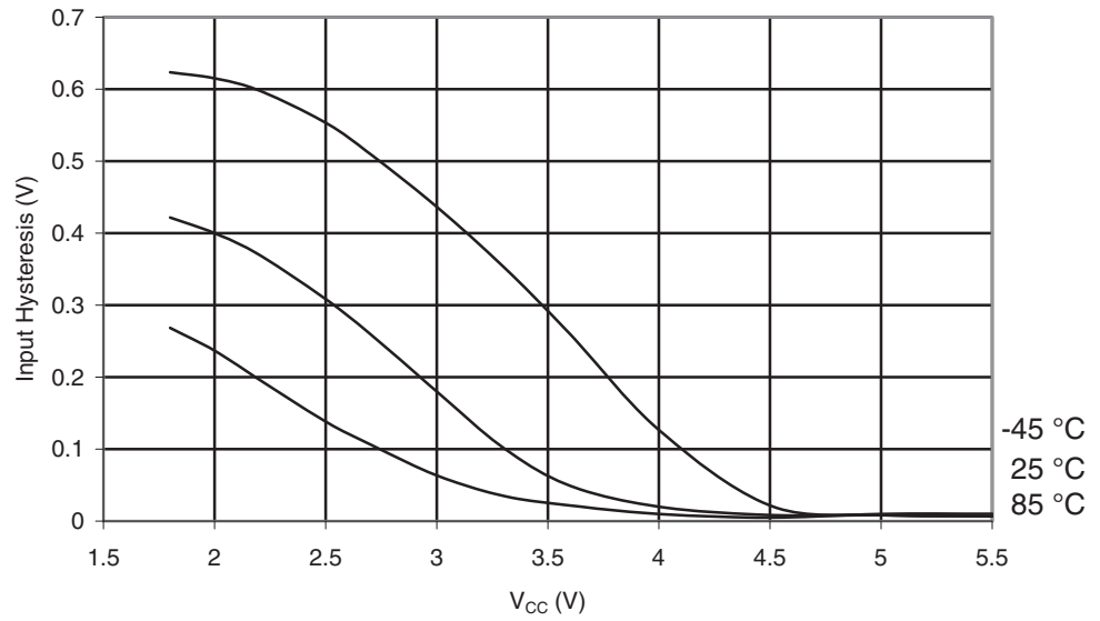
Figure 29-39. ATmega165A: Reset Input Pin Hysteresis vs. V_{CC}
