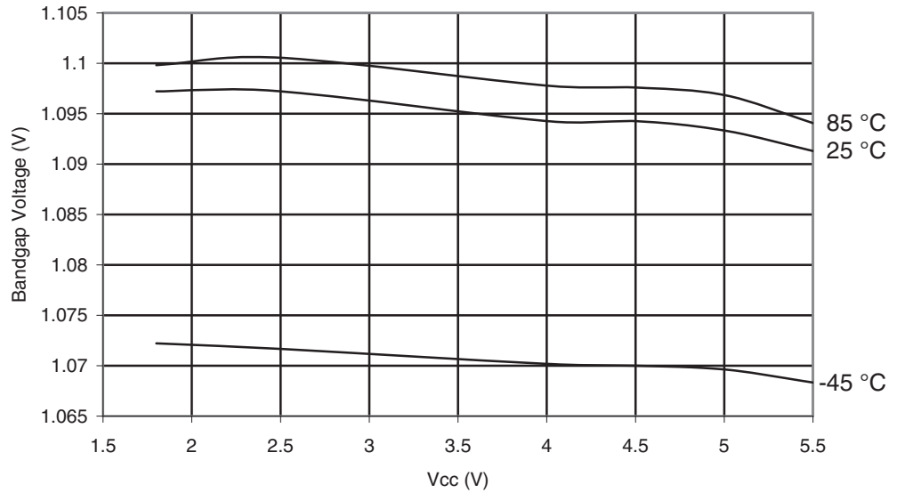
Figure 29-43. ATmega165A: Bandgap Voltage vs. V CC
