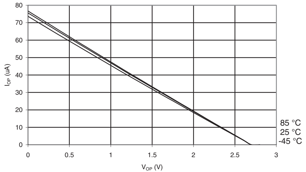
Figure 29-79. ATmega165PA: I/O Pin Pull-up Resistor Current vs. Input Voltage ( V_{CC} = 2.7V )
