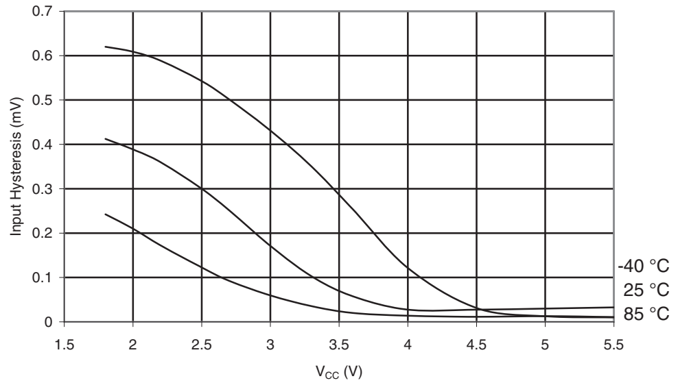
Figure 29-283. ATmega3250A: Reset Input Pin Hysteresis vs. V_{CC}
