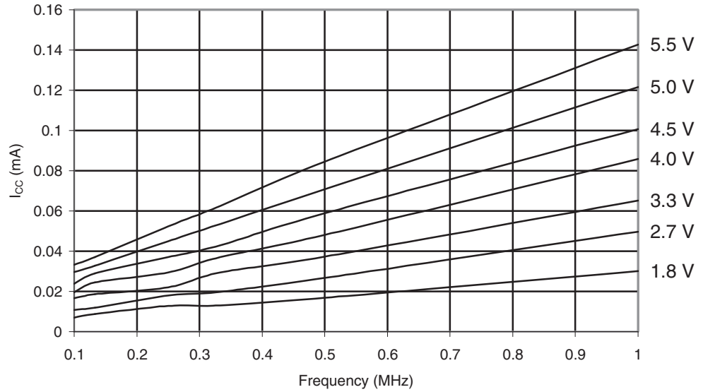
Figure 29-545. ATmega6450A: Reset Supply Current vs. V_{CC} (0.1 - 1.0MHz, Excluding Current Through The Reset Pull-up)
