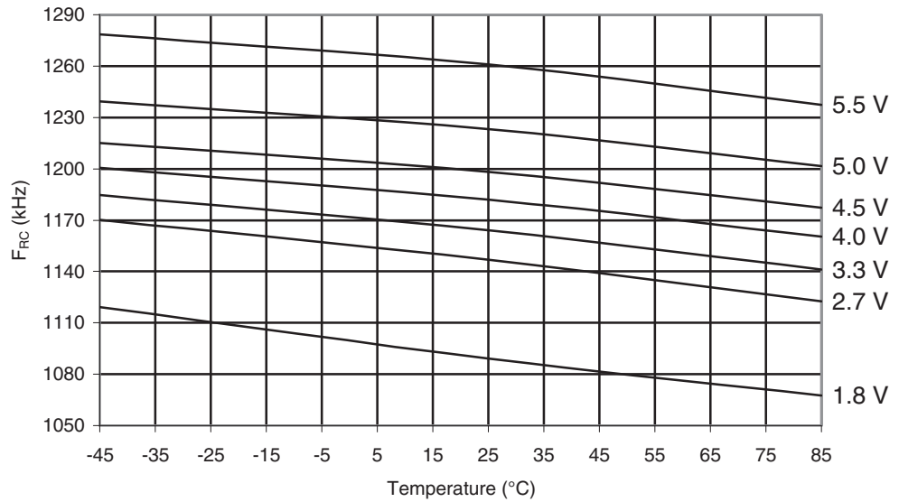
Figure 29-594. ATmega6450P: Watchdog Oscillator Frequency vs. Temperature
