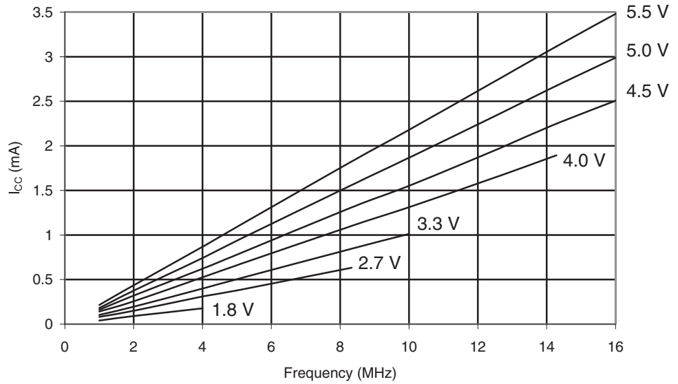
Figure 29-69. ATmega165PA: Idle Supply Current vs. Frequency (1 - 16MHz)
