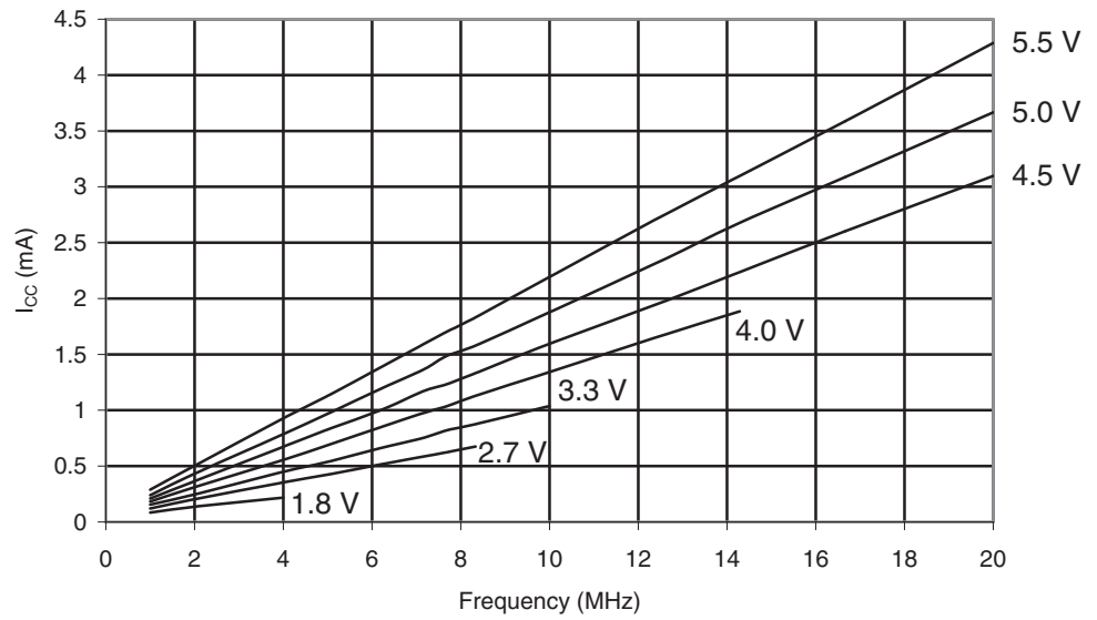
Figure 29-432. ATmega645P: Idle Supply Current vs. Frequency (1 - 20MHz)
