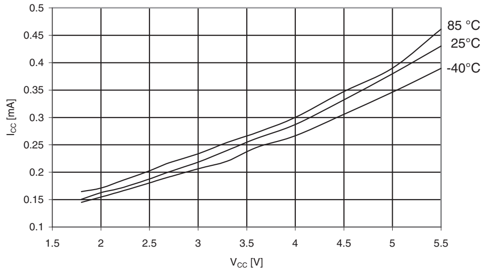
Figure 29-193. ATmega325PA: Idle Supply Current vs. V_{CC} (Internal RC Oscillator, 1 MHz)
