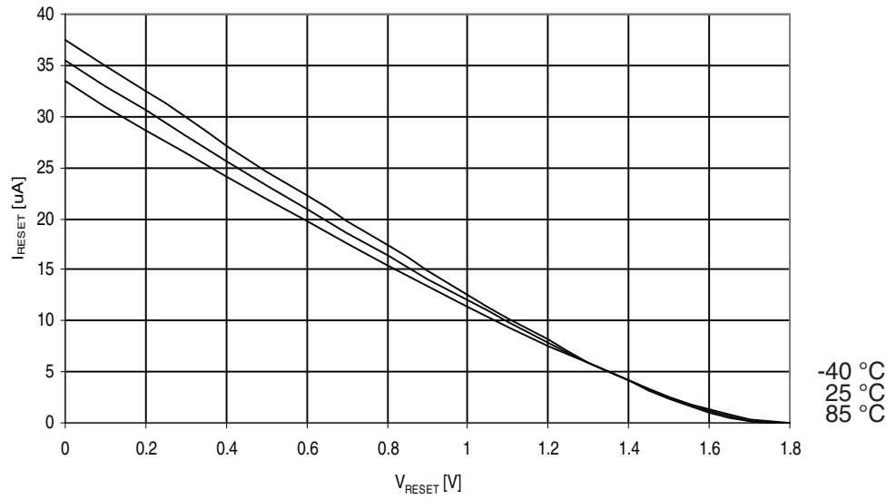
Figure 29-145. ATmega325A: Reset Pull-up Resistor Current vs. Reset Pin Voltage ( V_{CC} = 1.8V )
