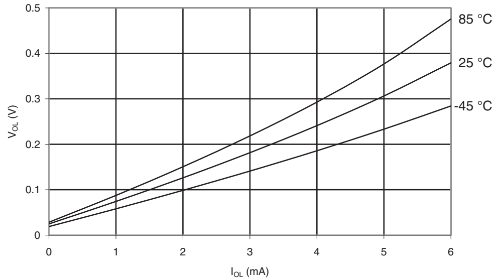
Figure 29-33. ATmega165A: I/O Pin Output Voltage vs. Sink Current, Port B ( V_{CC} = 1.8V )
