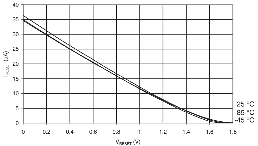
Figure 29-83. ATmega165PA: Reset Pull-up Resistor Current vs. Reset Pin Voltage ( V_{CC} = 1.8V )
