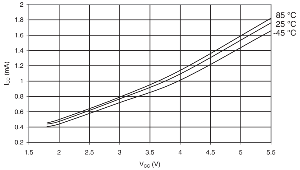
Figure 29-428. ATmega645P: Active Supply Current vs. V_{CC} (Internal RC Oscillator, 8MHz)
