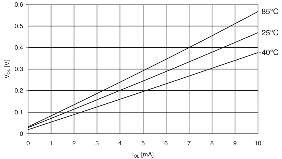
Figure 29-272. ATmega3250A: I/O Pin Output Voltage vs. Sink Current, Ports A, C, D, E, F, G ( V_{CC} = 5V )
