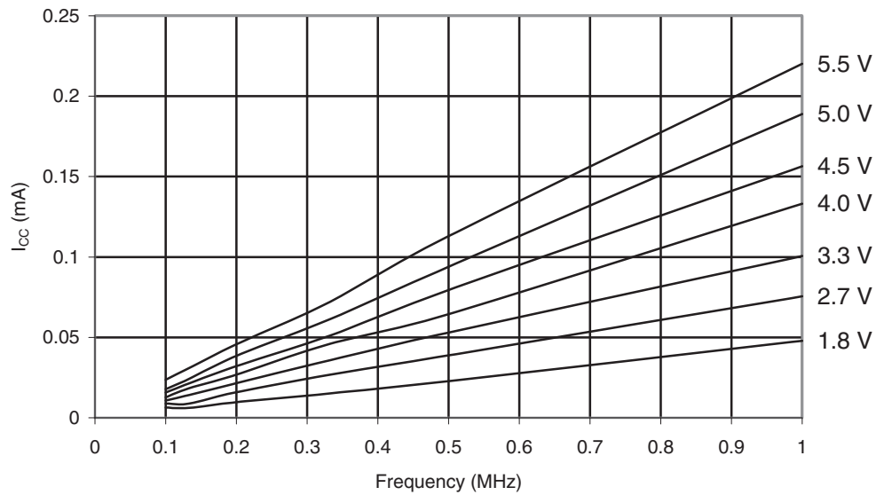
Figure 29-68. ATmega165PA: Idle Supply Current vs. Frequency (0.1 - 1.0MHz)
