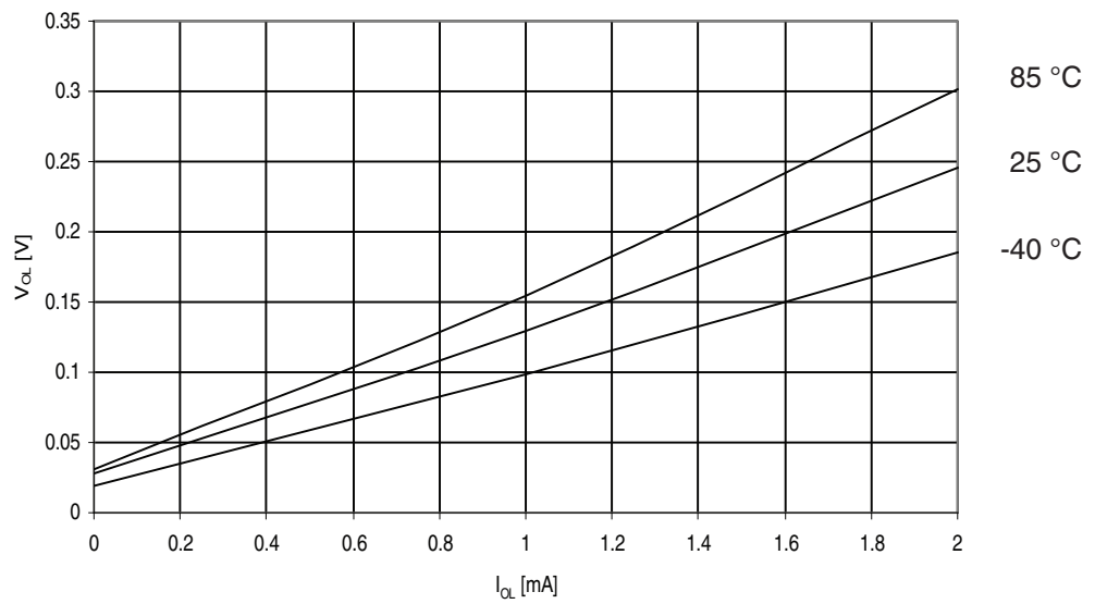
Figure 29-274. ATmega3250A: I/O Pin Output Voltage vs. Sink Current, Ports A, C, D, E, F, G ( V_{CC} = 1.8V )
