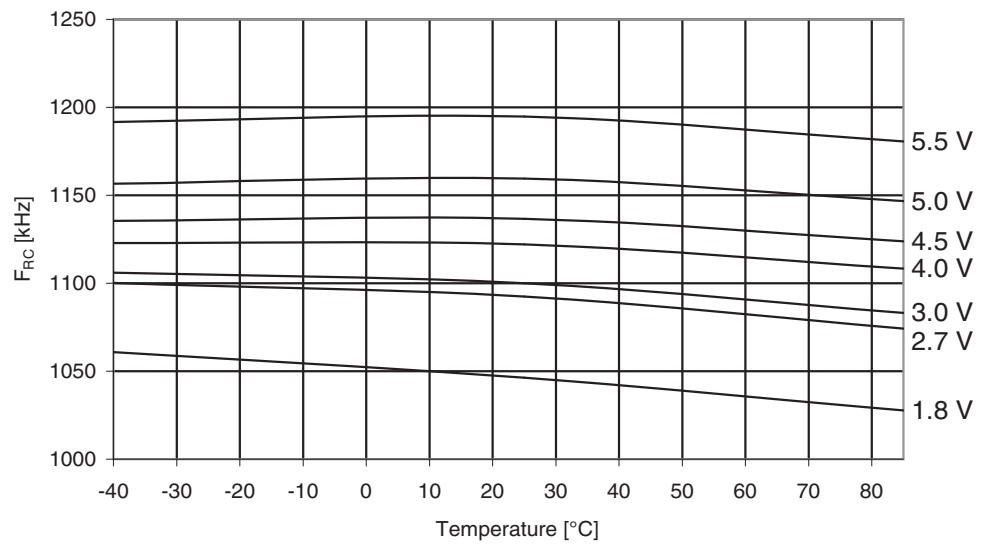
Figure 29-230. ATmega325PA: Watchdog Oscillator Frequency vs. Temperature
