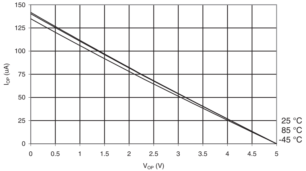
Figure 29-78. ATmega165PA: I/O Pin Pull-up Resistor Current vs. Input Voltage ( V_{CC} = 5V )
