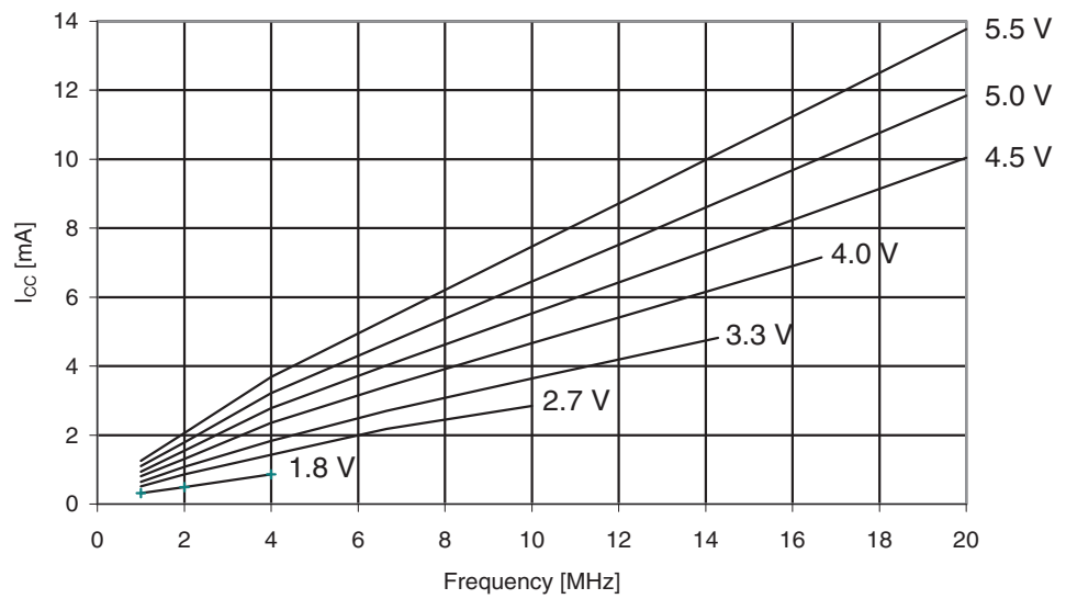
Figure 29-186. ATmega325PA: Active Supply Current vs. Frequency (1 - 20MHz)
