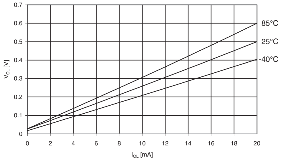
Figure 29-335. ATmega3250PA: I/O Pin Output Voltage vs. Sink Current, Port B ( V_{CC} = 5V )
