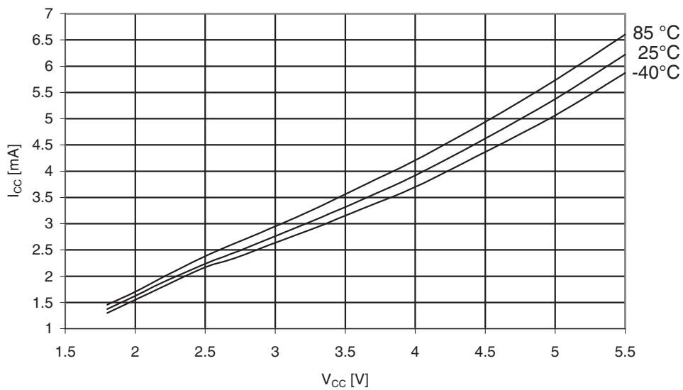
Figure 29-187. ATmega325PA: Active Supply Current vs. V_{CC} (Internal RC Oscillator, 8MHz)
