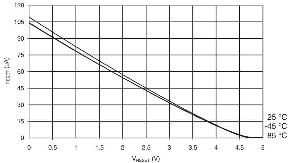
Figure 29-567. ATmega6450A: Reset Pull-up Resistor Current vs. Reset Pin Voltage ( V_{CC} = 5V )
