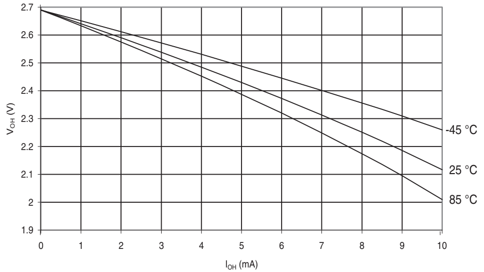
Figure 29-388. ATmega645A: I/O Pin Output Voltage vs. Source Current, Ports A, C, D, E, F, G ( V_{CC} = 2.7V )
