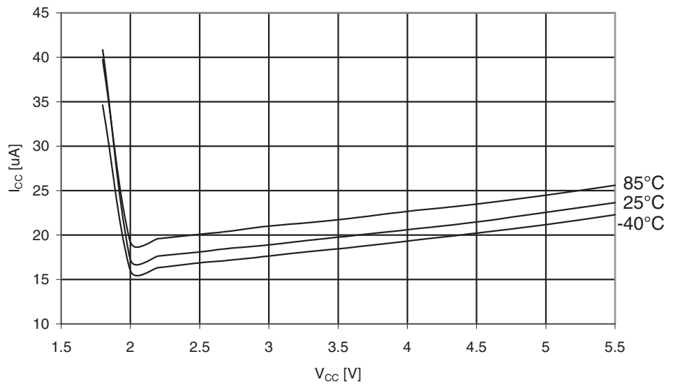
Figure 29-174. ATmega325A: Brownout Detector Current vs. V_{CC}
