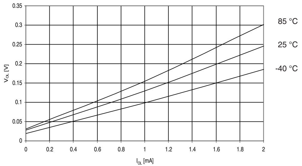
Figure 29-334. ATmega3250PA: I/O Pin Output Voltage vs. Sink Current, Ports A, C, D, E, F, G ( V_{CC} = 1.8V )
