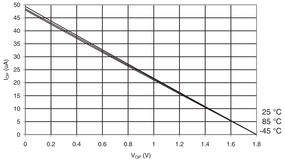
Figure 29-80. ATmega165PA: I/O Pin Pull-up Resistor Current vs. Input Voltage ( V_{CC} = 1.8V )
