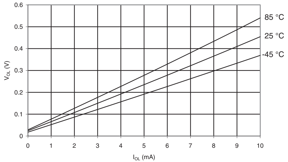
Figure 29-90. ATmega165PA: I/O Pin Output Voltage vs. Sink Current, Ports A, C, D, E, F, G ( V_{CC} = 5V )
