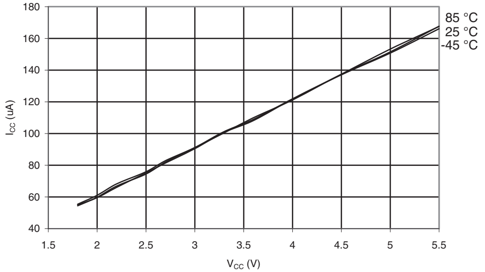
Figure 29-118. ATmega165PA: AREF External Reference Current vs. V_{CC}
