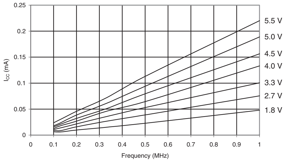
Figure 29-6. ATmega165A: Idle Supply Current vs. Frequency (0.1 - 1.0MHz)
