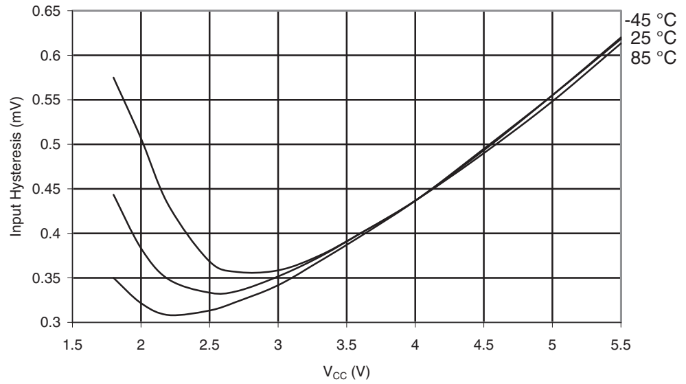
Figure 29-36. ATmega165A: I/O Pin Input Hysteresis vs. V_{CC}
