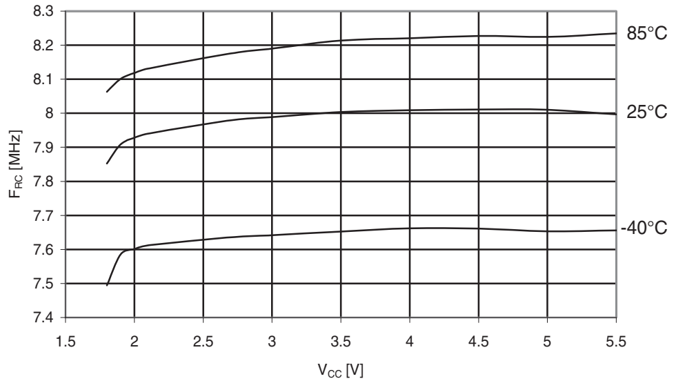
Figure 29-172. ATmega325A: Calibrated 8MHz RC Oscillator Frequency vs. V_{CC}
