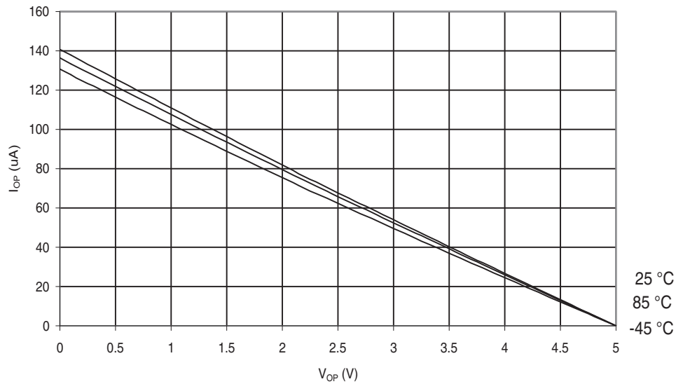
Figure 29-564. ATmega6450A: I/O Pin Pull-up Resistor Current vs. Input Voltage ( V_{CC} = 5V )
