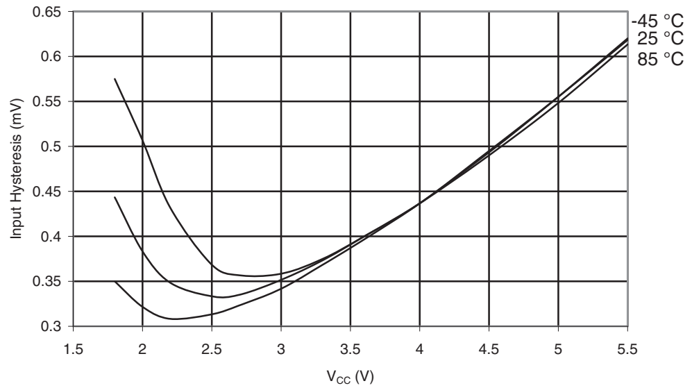
Figure 29-98. ATmega165PA: I/O Pin Input Hysteresis vs. V_{CC}
