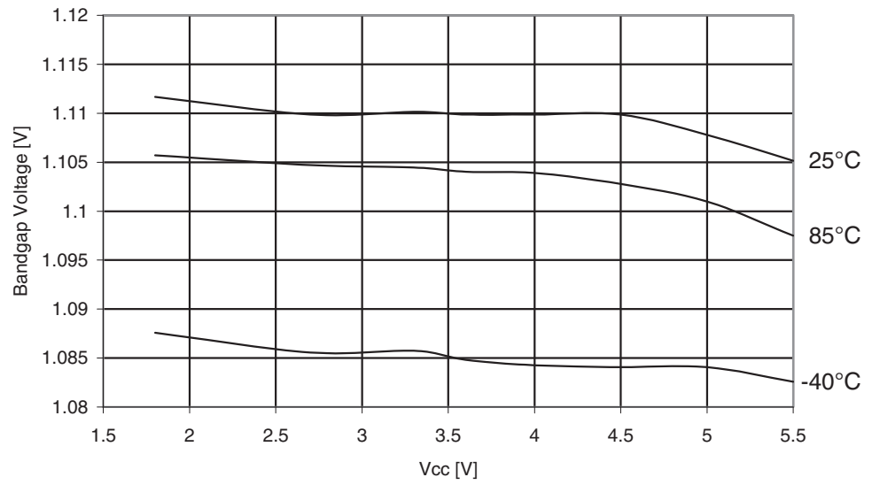
Figure 29-287. ATmega3250A: Bandgap Voltage vs. V_{CC}
