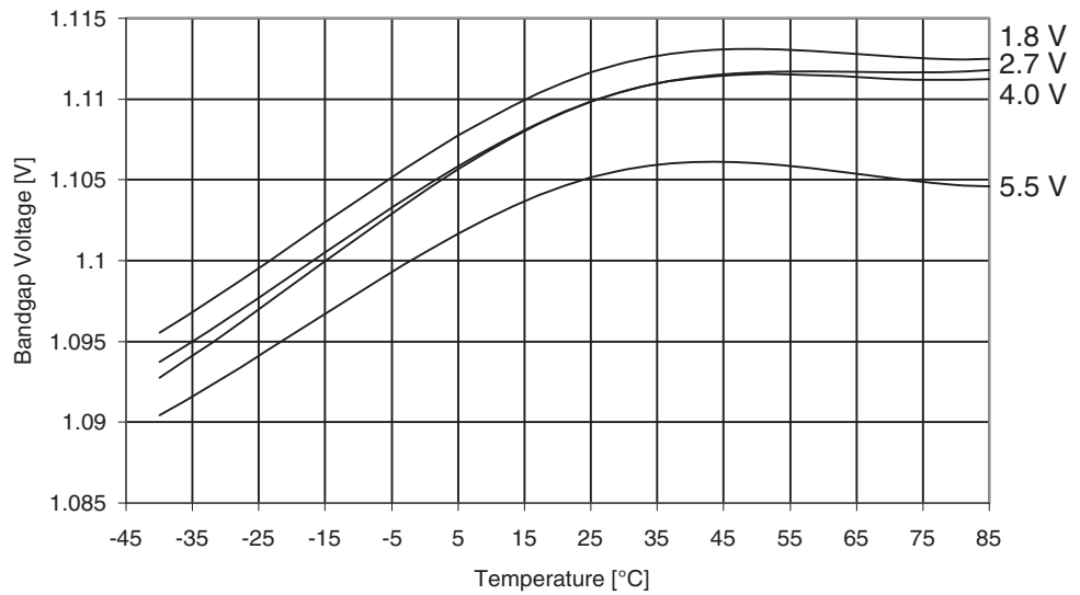
Figure 29-168. ATmega325A: Bandgap Voltage vs. Temperature
