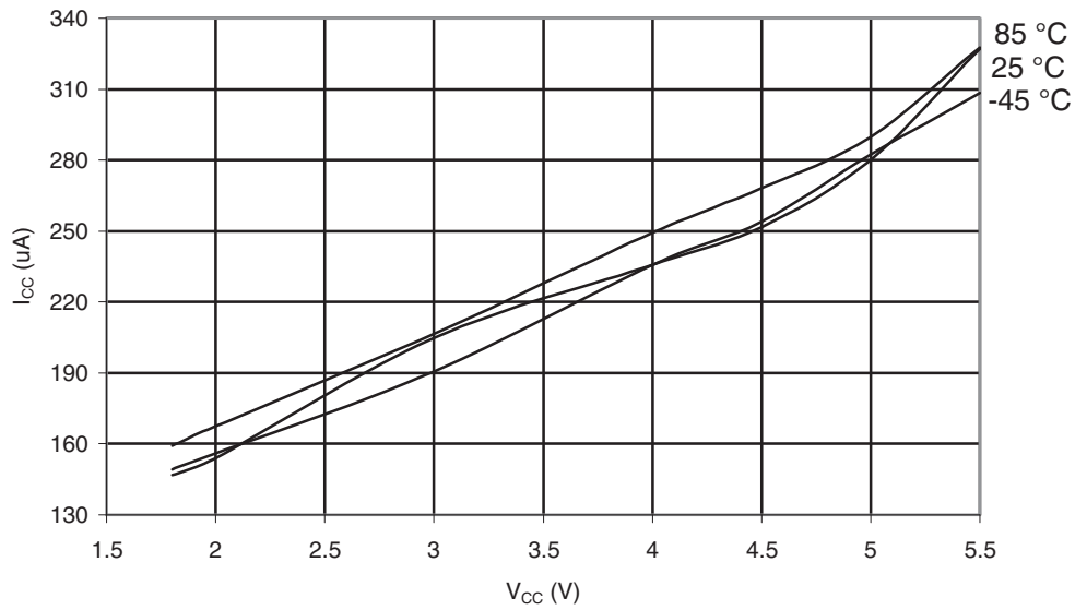
Figure 29-418. ATmega645A: Active Supply Current with ADC at 1MHz vs. V_{CC}
