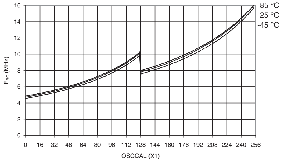
Figure 29-113. ATmega165PA: Calibrated 8MHz RC Oscillator Frequency vs. Oscscal Value
