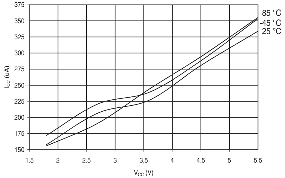
Figure 29-116. ATmega165PA: Active Supply Current with ADC at 200kHz vs. V_{CC}
