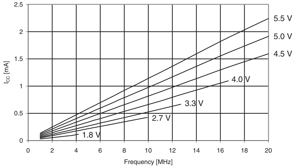
Figure 29-363. ATmega3250PA: Reset Supply Current vs. V_{CC} (1 - 20MHz, Excluding Current Through The Reset Pull-up)
