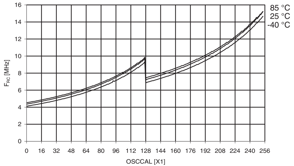
Figure 29-173. ATmega325A: Calibrated 8MHz RC Oscillator Frequency vs. Oscscal Value
