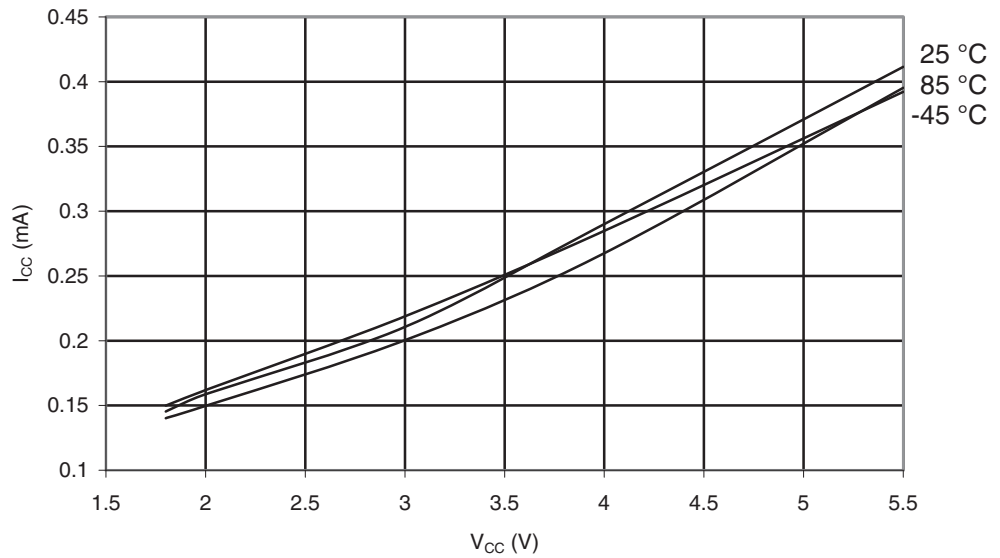
Figure 29-434. ATmega645P: Idle Supply Current vs. V_{CC} (Internal RC Oscillator, 1MHz)
