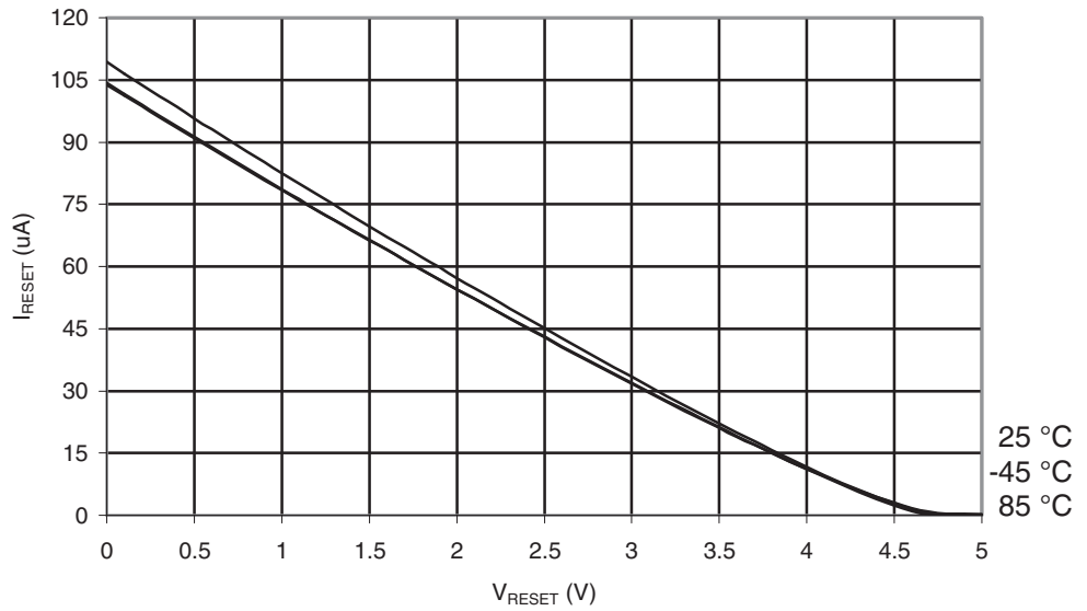
Figure 29-384. ATmega645A: Reset Pull-up Resistor Current vs. Reset Pin Voltage ( V_{CC} = 5V )
