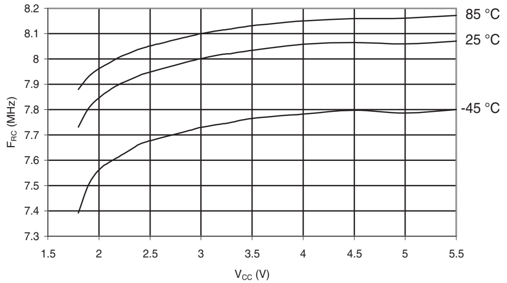
Figure 29-413. ATmega645A: Calibrated 8MHz RC Oscillator Frequency vs. V_{CC}
