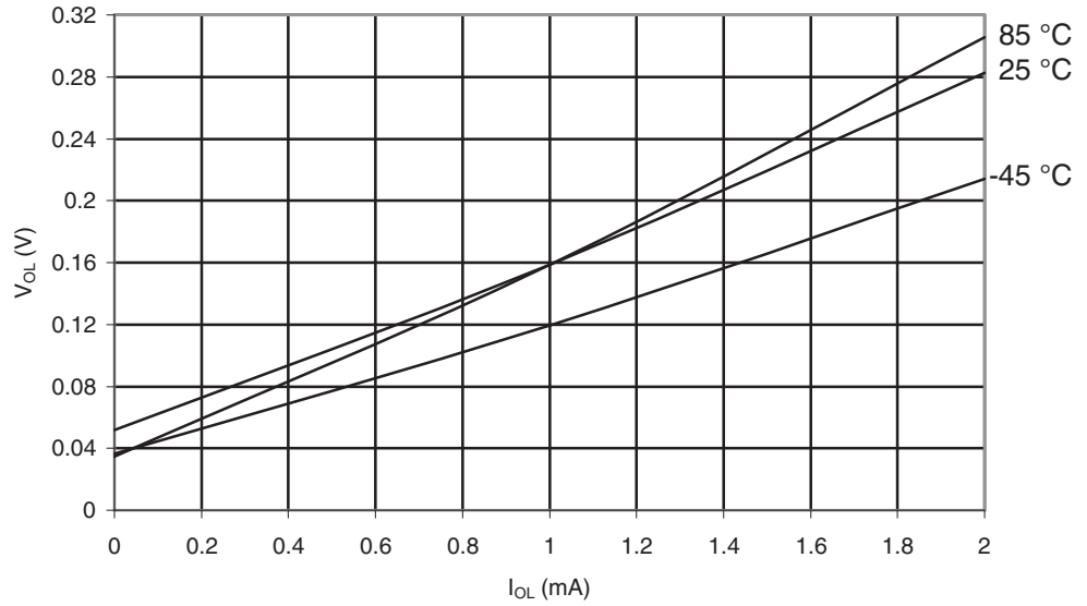
Figure 29-456. ATmega645P: I/O Pin Output Voltage vs. Sink Current, Ports A, C, D, E, F, G ( V_{CC} = 1.8V )
