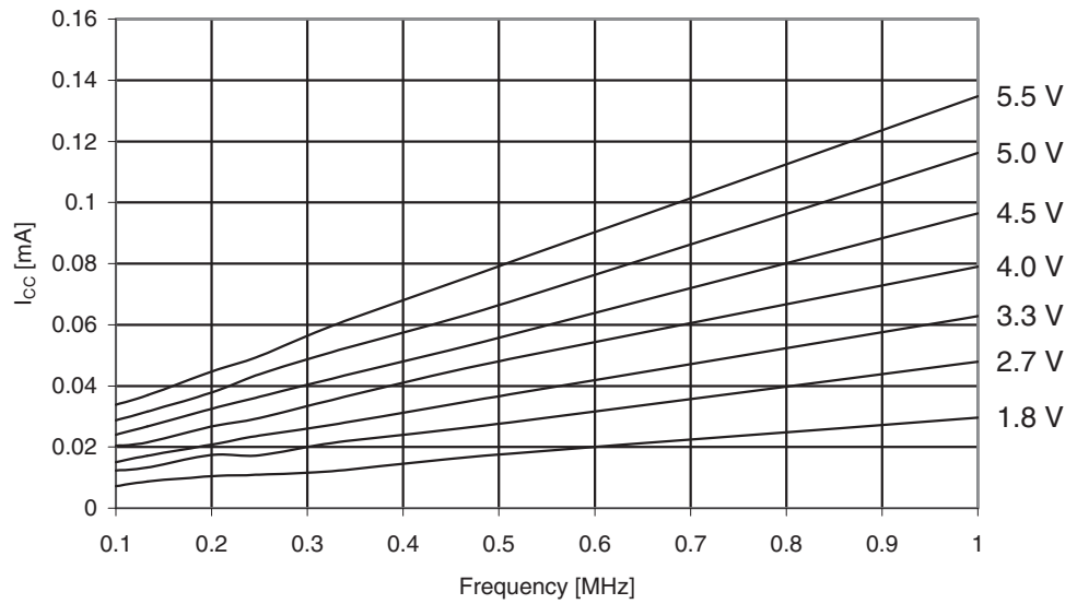
Figure 29-302. ATmega3250A: Reset Supply Current vs. V_{CC} (0.1 - 1.0MHz, Excluding Current Through The Reset Pull-up)
