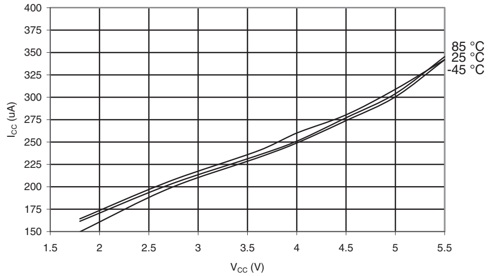
Figure 29-115. ATmega165PA: Active Supply Current with ADC at 50kHz vs. V_{CC}
