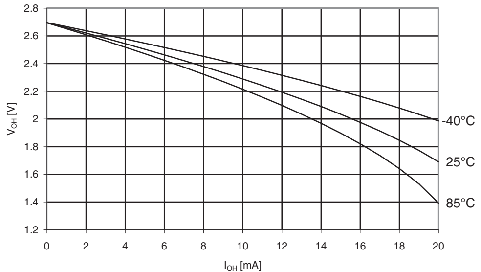
Figure 29-270. ATmega3250A: I/O Pin Output Voltage vs. Source Current, Port B ( V_{CC} = 2.7V )
