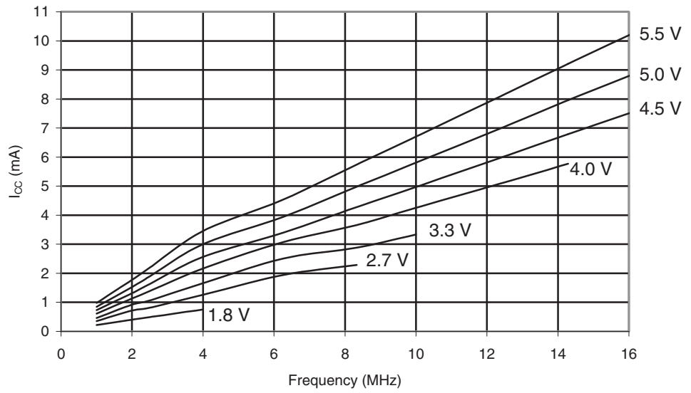
Figure 29-2. ATmega165A: Active Supply Current vs. Frequency (1 - 16MHz)
