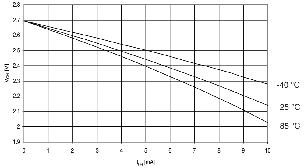
Figure 29-327. ATmega3250PA: I/O Pin Output Voltage vs. Source Current, Ports A, C, D, E, F, G ( V_{CC} = 2.7V )
