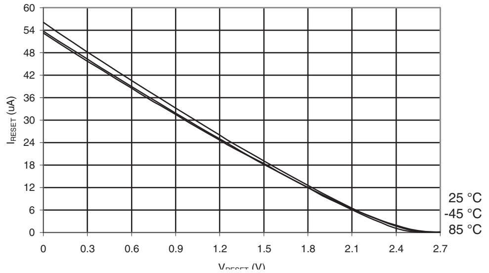
Figure 29-507. ATmega6450A: Reset Pull-up Resistor Current vs. Reset Pin Voltage ( V_{CC} = 2.7V )
