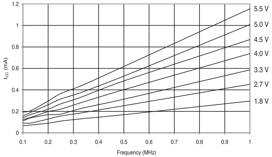
Figure 29-487. ATmega6450A: Active Supply Current vs. Low Frequency (0.1 - 1.0MHz)
