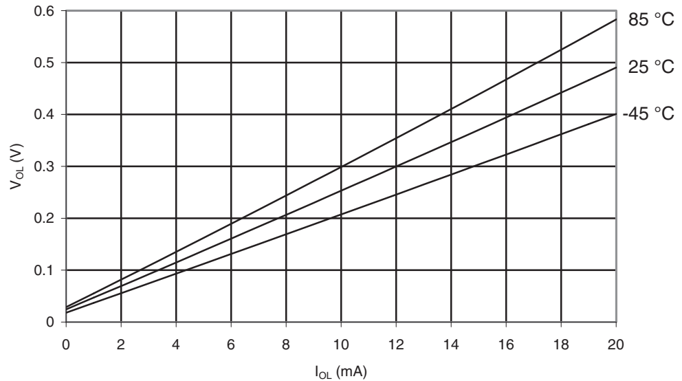
Figure 29-31. ATmega165A: I/O Pin Output Voltage vs. Sink Current, Port B ( V_{CC} = 5V )
