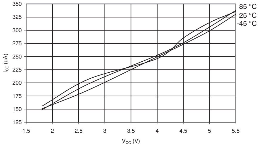
Figure 29-117. ATmega165A: Active Supply Current with ADC at 1MHz vs. V_{CC}
