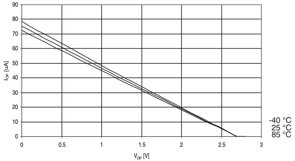
Figure 29-321. ATmega3250PA: I/O Pin Pull-up Resistor Current vs. Input Voltage ( V_{CC} = 2.7V )
