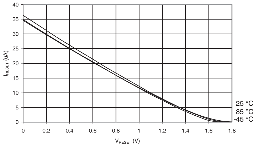
Figure 29-21. ATmega165A: Reset Pull-up Resistor Current vs. Reset Pin Voltage ( V_{CC} = 1.8V )
