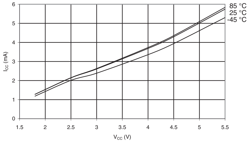
Figure 29-3. ATmega165A: Active Supply Current vs. V_{CC} (Internal RC Oscillator, 8MHz)
