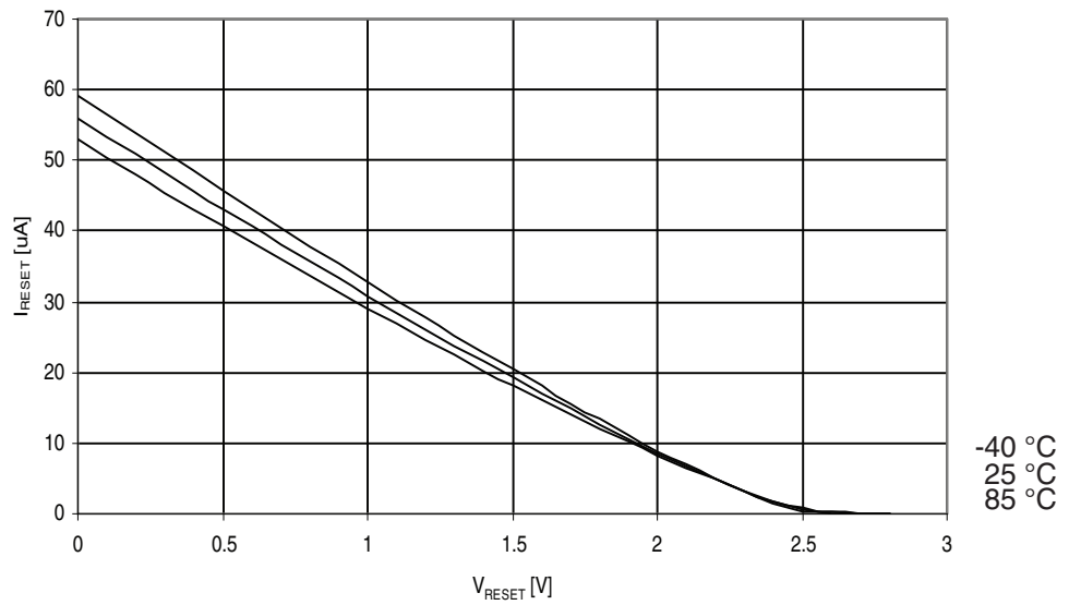
Figure 29-324. ATmega3250PA: Reset Pull-up Resistor Current vs. Reset Pin Voltage ( V_{CC} = 2.7V )
