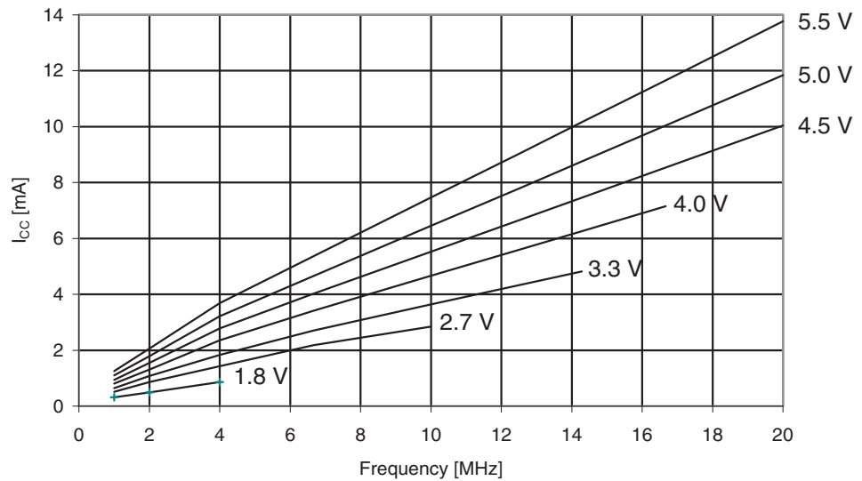
Figure 29-306. ATmega3250PA: Active Supply Current vs. Frequency (1 - 20MHz)
