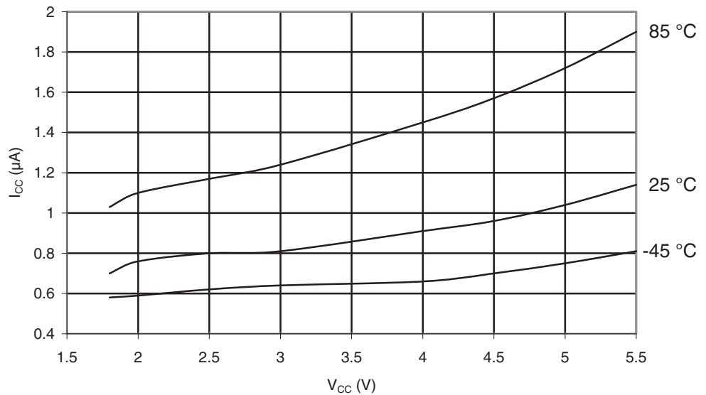
Figure 29-13. ATmega165A: Power-save Supply Current vs. V_{CC} (Watchdog Timer Disabled)
