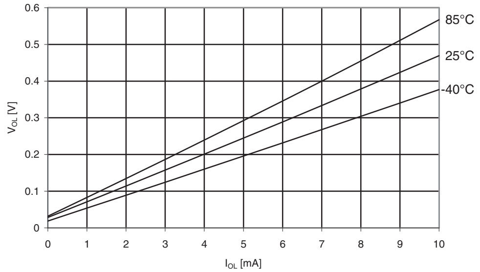
Figure 29-212. ATmega325PA: I/O Pin Output Voltage vs. Sink Current, Ports A, C, D, E, F, G ( V_{CC} = 5V )
