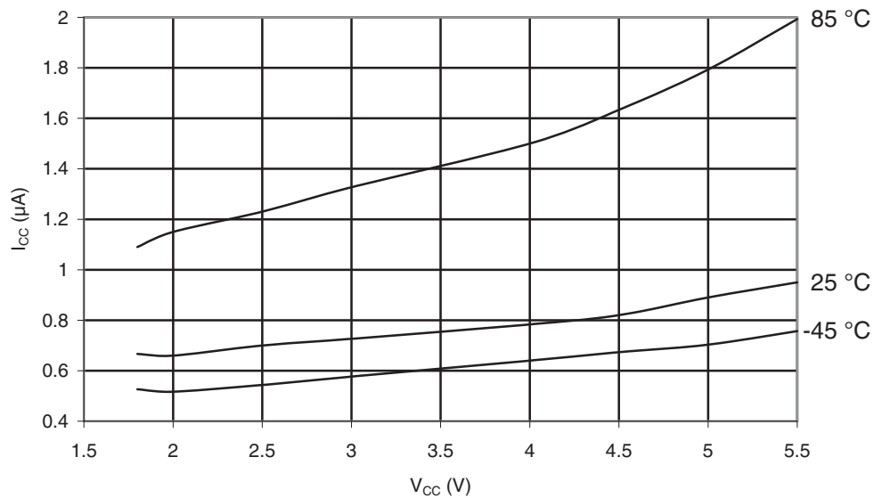
Figure 29-76. ATmega165PA: Standby Supply Current vs. V_{CC} (32kHz Watch Crystal, Watchdog Timer Disabled)
