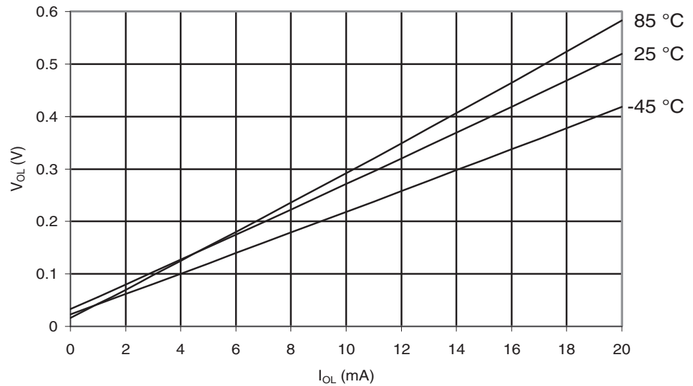
Figure 29-515. ATmega6450A: I/O Pin Output Voltage vs. Sink Current, Ports A, C, D, E, F, G ( V_{CC} = 5V )
