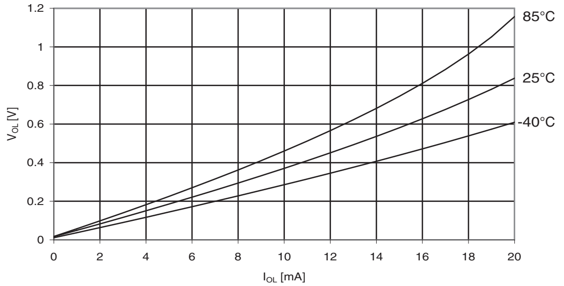
Figure 29-276. ATmega3250A: I/O Pin Output Voltage vs. Sink Current, Port B ( V_{CC} = 2.7V )
