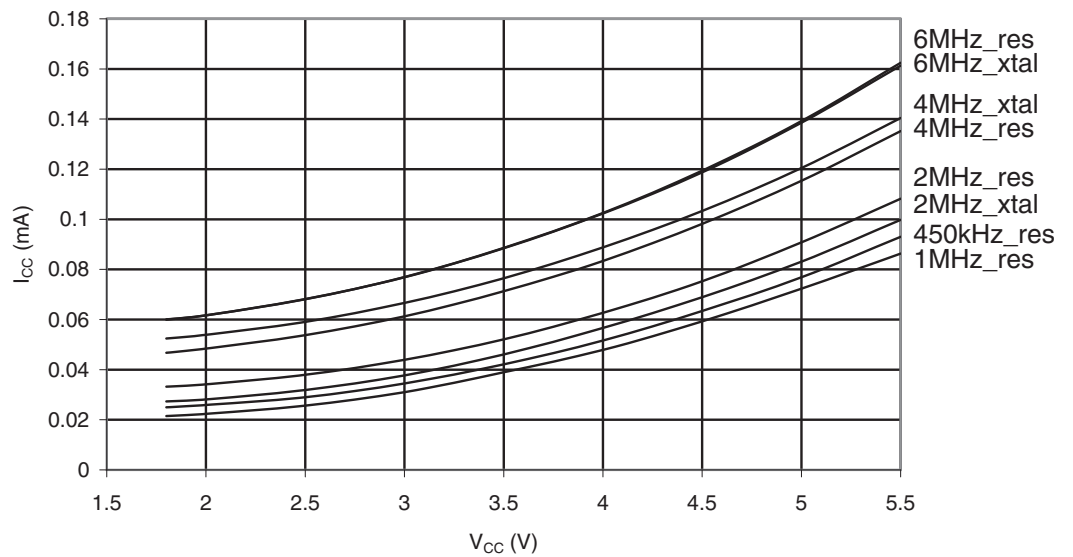
Figure 29-15. ATmega165A: Standby Supply Current vs. V_{CC} (Xtall and Resonator, Watchdog Timer Disabled)
