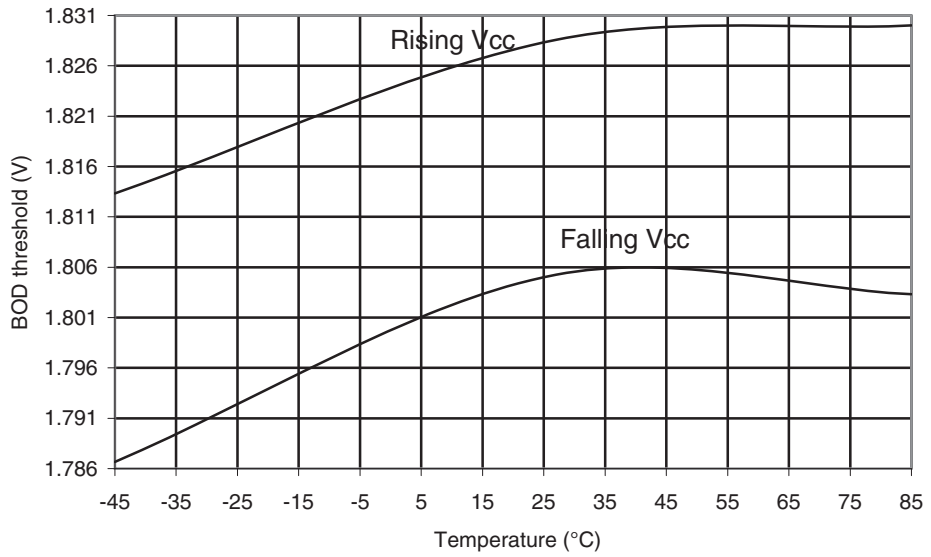
Figure 29-104. ATmega165PA: BOD Thresholds vs. Temperature (BOD Level is 1.8V)
