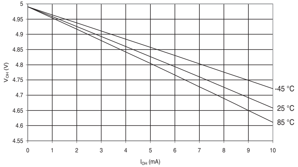
Figure 29-387. ATmega645A: I/O Pin Output Voltage vs. Source Current, Ports A, C, D, E, F, G ( V_{CC} = 5V )
