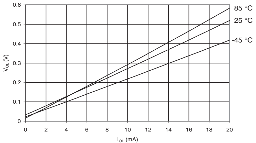
Figure 29-579. ATmega6450A: I/O Pin Output Voltage vs. Sink Current, Port B ( V_{CC} = 5V )
