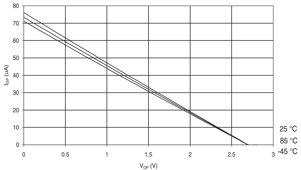
Figure 29-504. ATmega6450A: I/O Pin Pull-up Resistor Current vs. Input Voltage ( V_{CC} = 2.7V )
