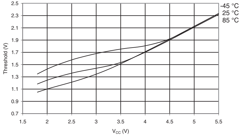
Figure 29-99. ATmega165PA: Reset Input Threshold Voltage vs. V_{CC} ( V_{IH} , Reset Pin Read as “1”)
