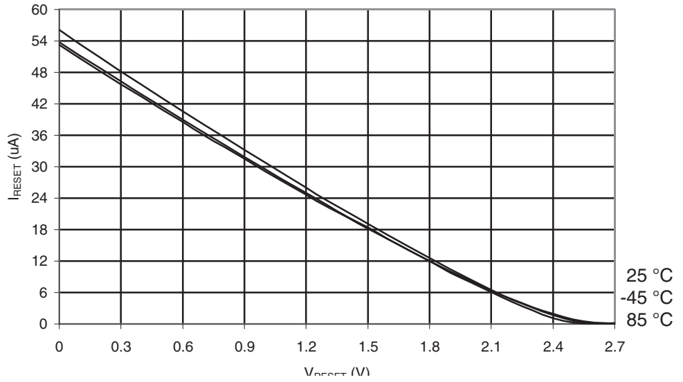
Figure 29-568. ATmega6450A: Reset Pull-up Resistor Current vs. Reset Pin Voltage ( V_{CC} = 2.7V )
