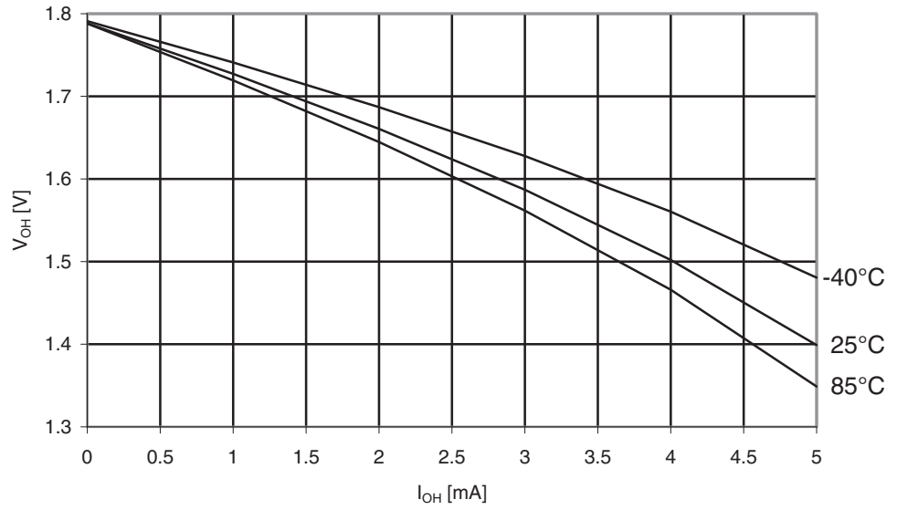
Figure 29-211. ATmega325PA: I/O Pin Output Voltage vs. Source Current, Port B ( V_{CC} = 1.8V )
