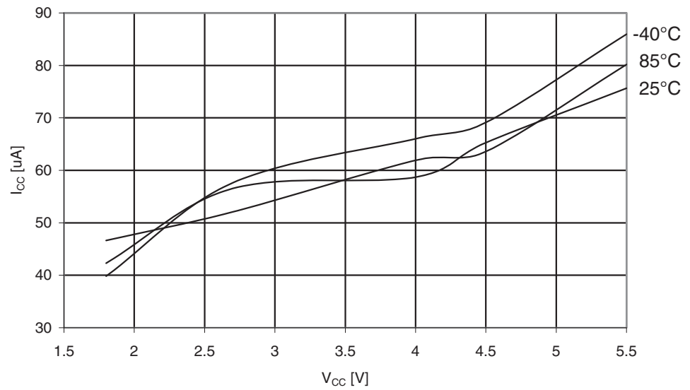
Figure 29-240. ATmega325PA: Analog Comparator Current vs. V_{CC}
