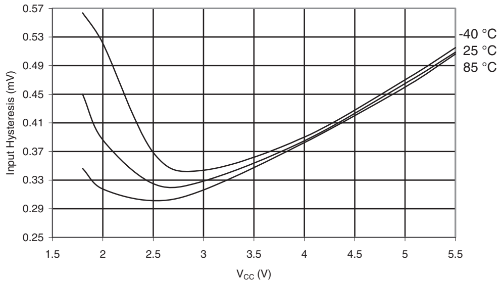
Figure 29-280. ATmega3250A: I/O Pin Input Hysteresis vs. V_{CC}
