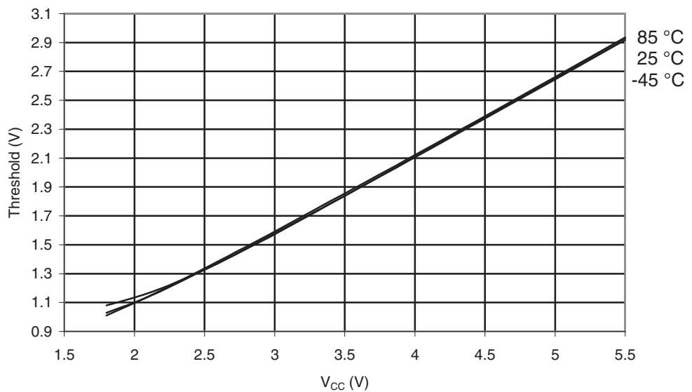
Figure 29-96. ATmega165PA: I/O Pin Input Threshold Voltage vs. V_{CC} ( V_{IH} , I/O Pin Read as “1”)
