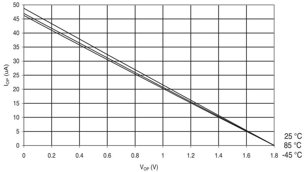
Figure 29-505. ATmega6450A: I/O Pin Pull-up Resistor Current vs. Input Voltage ( V_{CC} = 1.8V )
