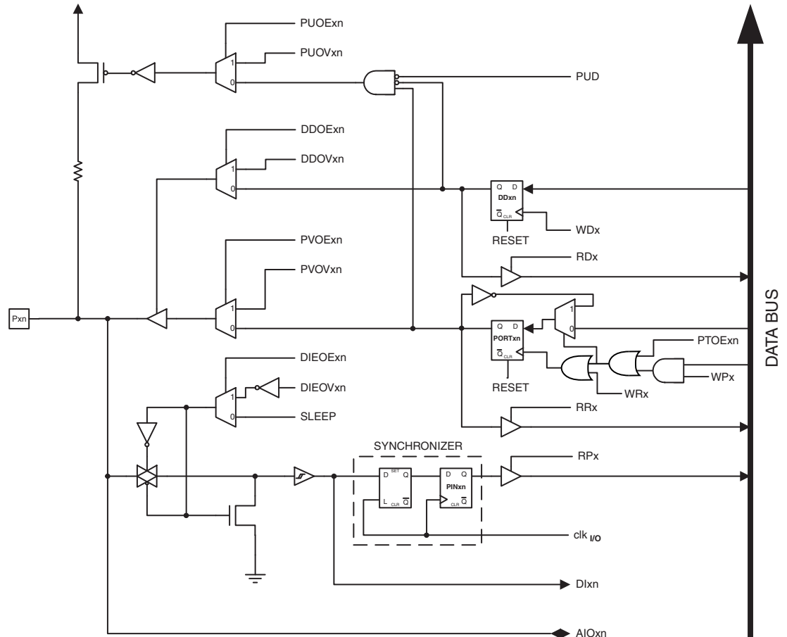
Figure 14-5. Alternate Port Functions (1)
