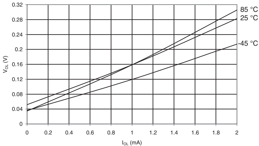
Figure 29-517. ATmega6450A: I/O Pin Output Voltage vs. Sink Current, Ports A, C, D, E, F, G ( V_{CC} = 1.8V )
