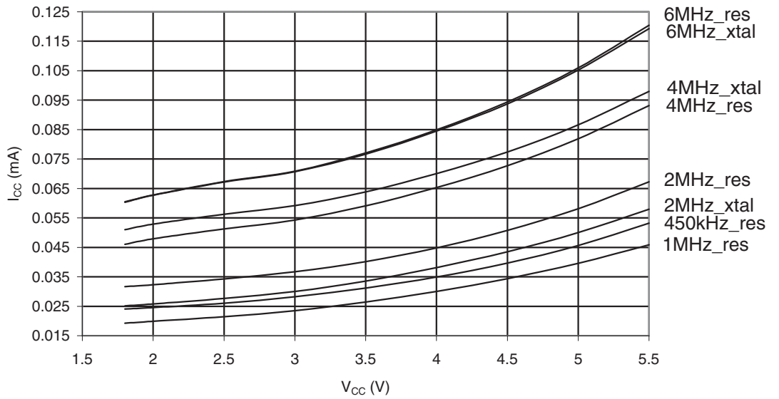
Figure 29-380. ATmega645A: Standby Supply Current vs. V_{CC} (Xtall and Resonator, Watchdog Timer Disabled)
