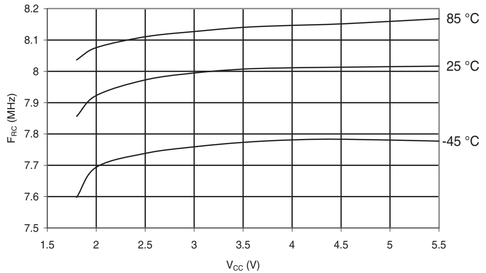
Figure 29-50. ATmega165A: Calibrated 8MHz RC Oscillator Frequency vs. V_{CC}
