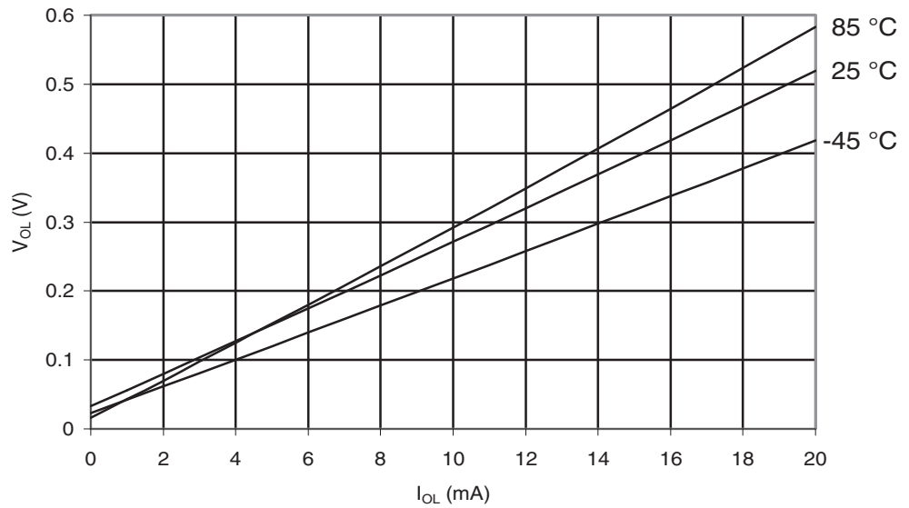
Figure 29-396. ATmega645A: I/O Pin Output Voltage vs. Sink Current, Port B ( V_{CC} = 5V )
