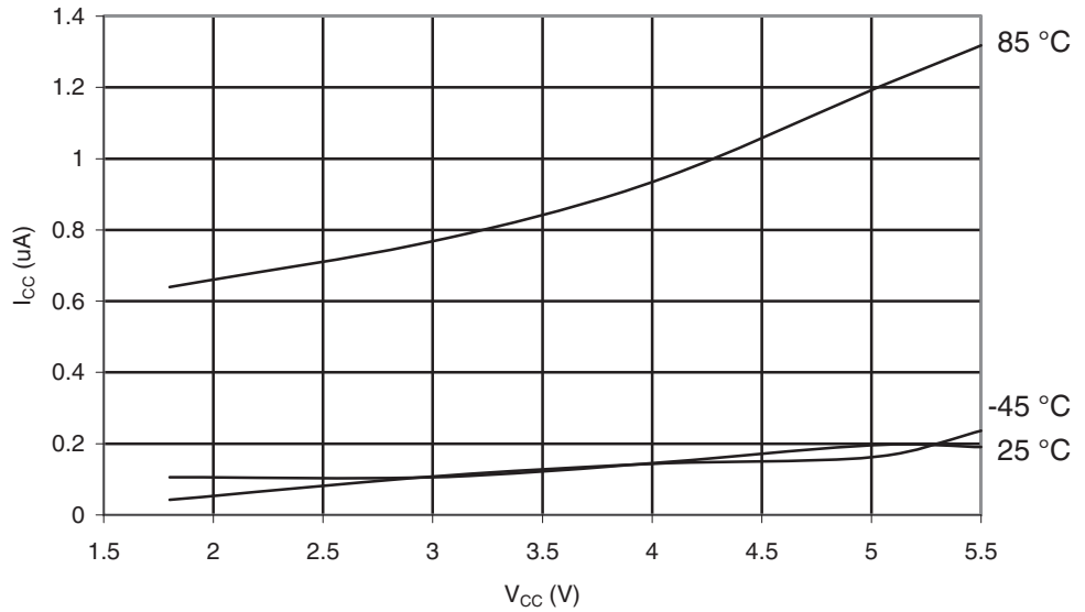
Figure 29-73. ATmega165PA: Power-down Supply Current vs. V_{CC} (Watchdog Timer Disabled)
