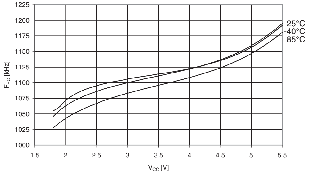
Figure 29-289. ATmega3250A: Watchdog Oscillator Frequency vs. V_{CC}
