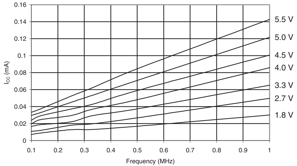
Figure 29-423. ATmega645A: Reset Supply Current vs. V_{CC} (0.1 - 1.0MHz, Excluding Current Through The Reset Pull-up)
