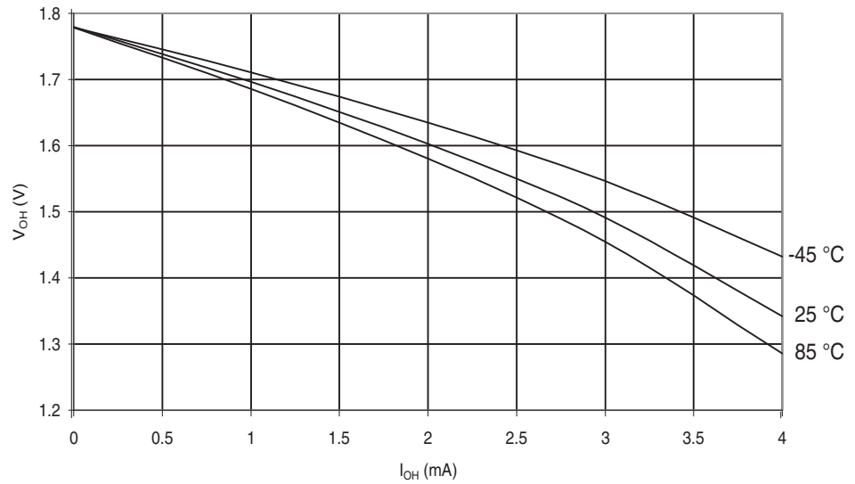
Figure 29-450. ATmega645P: I/O Pin Output Voltage vs. Source Current, Ports A, C, D, E, F, G ( V_{CC} = 1.8V )
