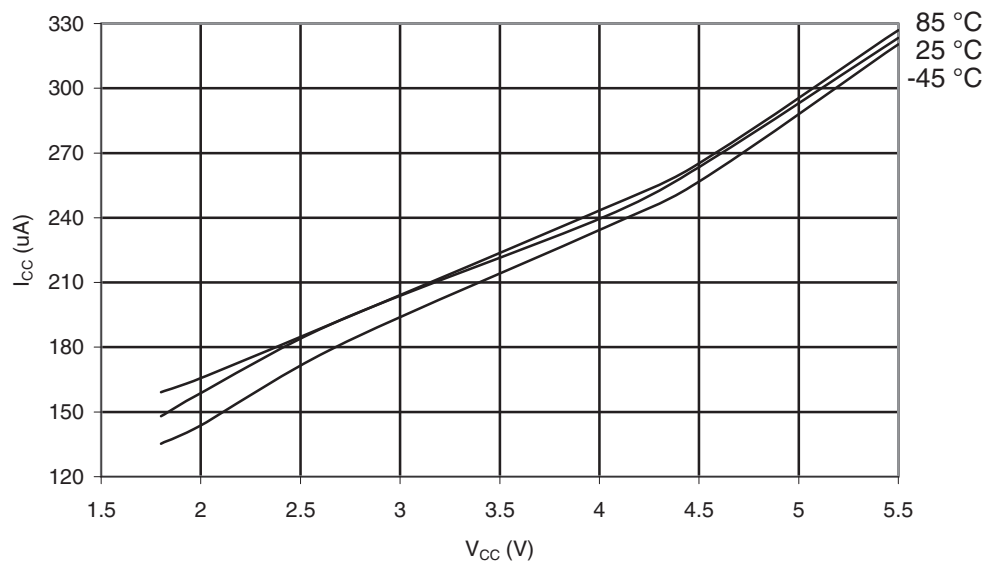
Figure 29-538. ATmega6450A: Active Supply Current with ADC at 50kHz vs. V_{CC}
