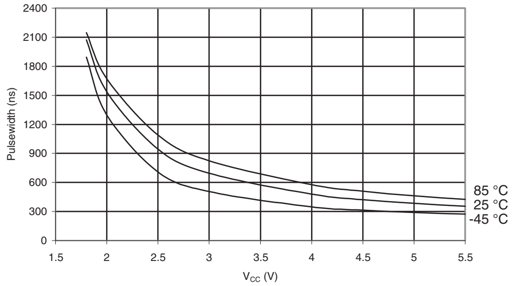
Figure 29-547. ATmega6450A: Minimum Reset Pulse Width vs. V_{CC}
