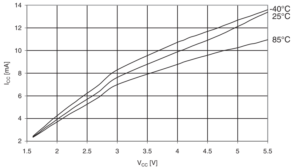
Figure 29-241. ATmega325PA: Programming Current vs. V_{CC}
