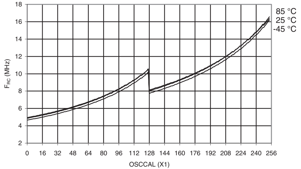
Figure 29-597. ATmega6450P: Calibrated 8MHz RC Oscillator Frequency vs. OSCAL Value
