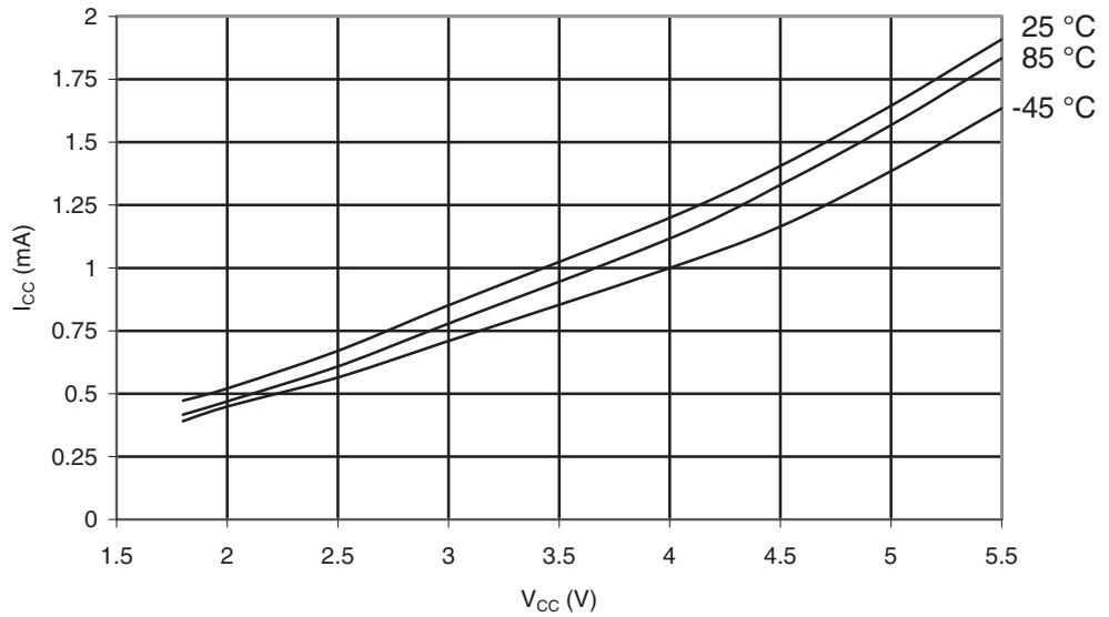
Figure 29-70. ATmega165PA: Idle Supply Current vs. V_{CC} (Internal RC Oscillator, 8MHz)
