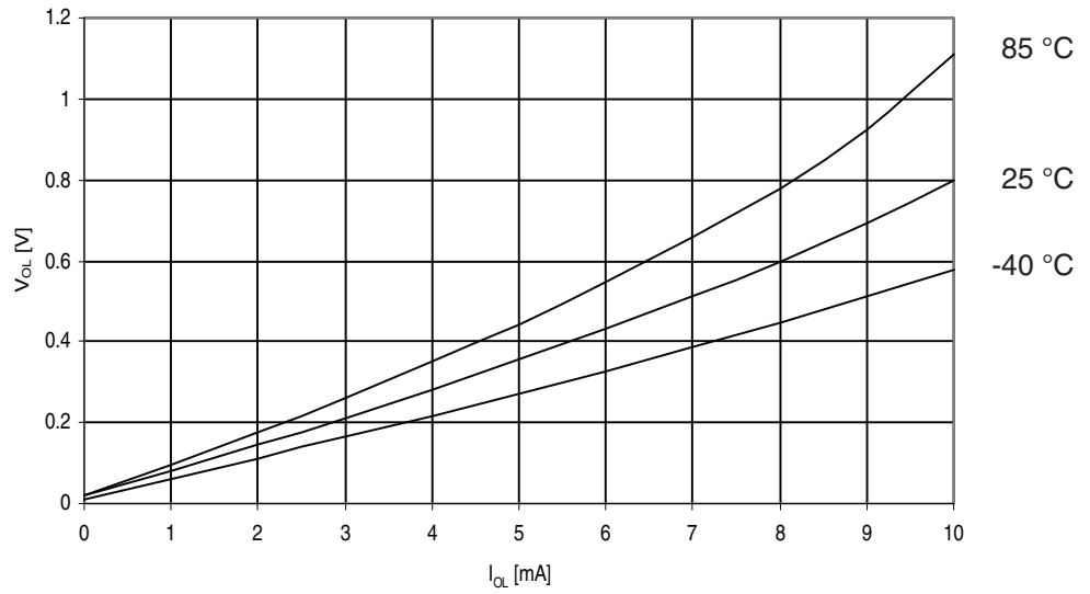
Figure 29-333. ATmega3250PA: I/O Pin Output Voltage vs. Sink Current, Ports A, C, D, E, F, G ( V_{CC} = 2.7V )
