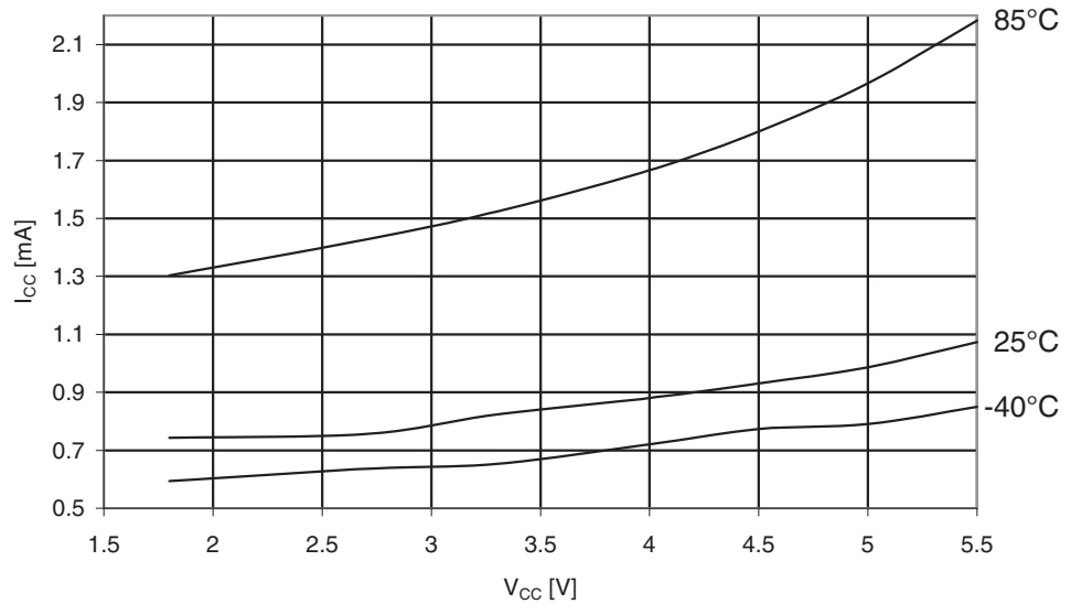
Figure 29-138. ATmega325A: Standby Supply Current vs. V_{CC} (32kHz Watch Crystal, Watchdog Timer Disabled)
