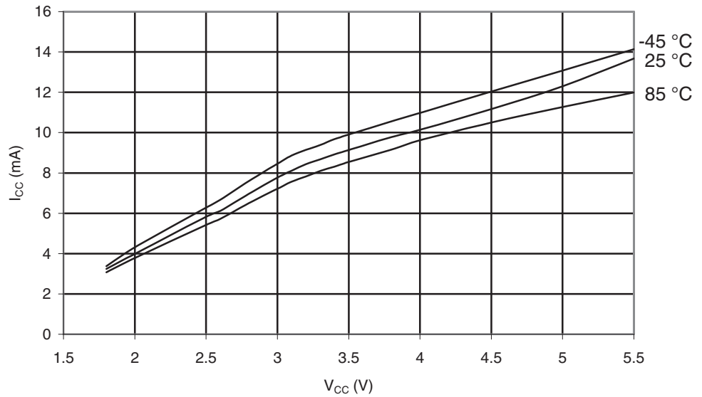
Figure 29-121. ATmega165PA: Programming Current vs. V_{CC}
