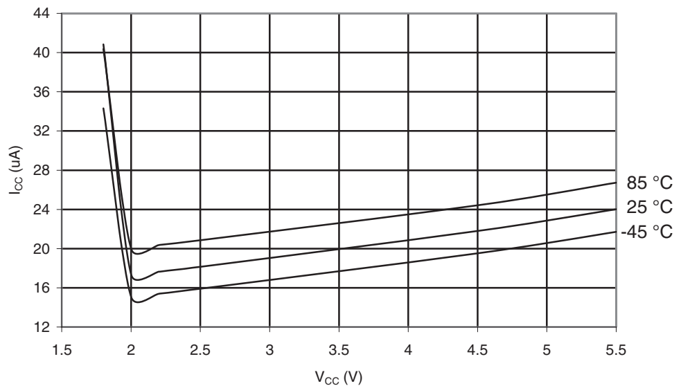
Figure 29-52. ATmega165A: Brownout Detector Current vs. V_{CC}
