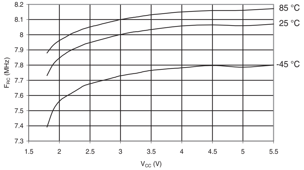
Figure 29-535. ATmega6450A: Calibrated 8MHz RC Oscillator Frequency vs. V_{CC}
