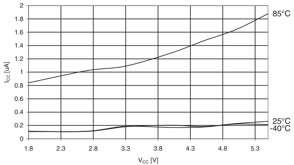
Figure 29-255. ATmega3250A: Power-down Supply Current vs. V_{CC} (Watchdog Timer Disabled)
