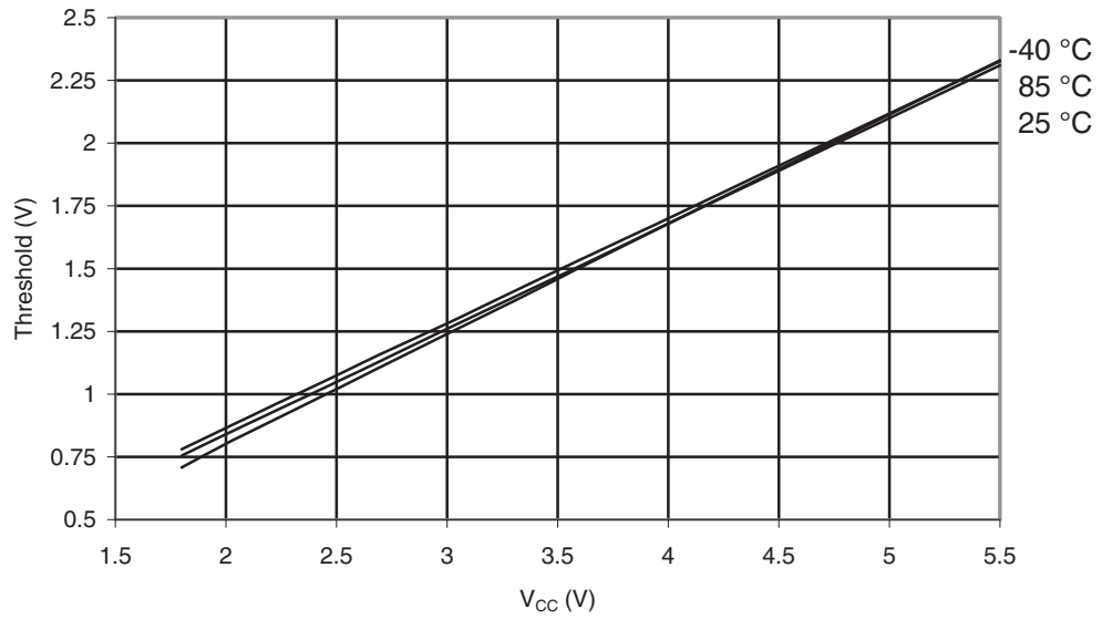
Figure 29-342. ATmega3250PA: Reset Input Threshold Voltage vs. V_{CC} ( V_{IL} , Reset Pin Read as "0")
