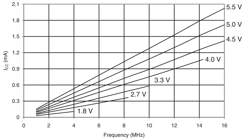
Figure 29-123. ATmega165PA: Reset Supply Current vs. V_{CC} (1 - 16MHz, Excluding Current Through The Reset Pull-up)
