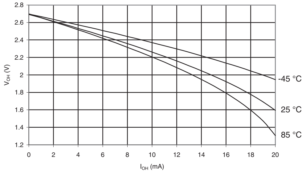
Figure 29-574. ATmega6450A: I/O Pin Output Voltage vs. Source Current, Port B ( V_{CC} = 2.7V )
