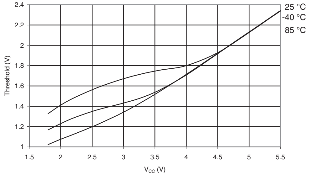
Figure 29-341. ATmega3250PA: Reset Input Threshold Voltage vs. V_{CC} ( V_{IH} , Reset Pin Read as "1")
