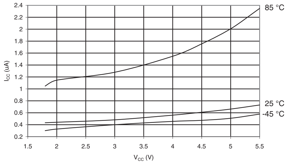
Figure 29-436. ATmega645P: Power-down Supply Current vs. V_{CC} (Watchdog Timer Disabled)
