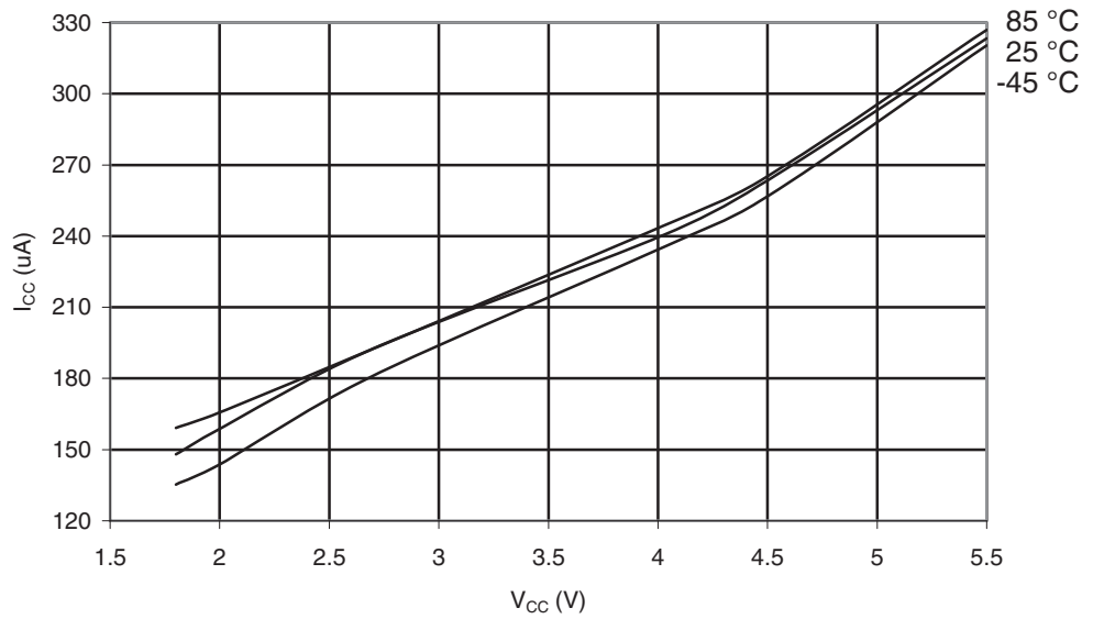
Figure 29-477. ATmega645P: Active Supply Current with ADC at 50kHz vs. V_{CC}
