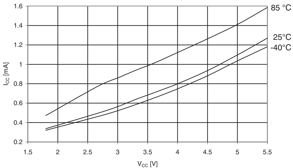
Figure 29-188. ATmega325PA: Active Supply Current vs. V_{CC} (Internal RC Oscillator, 1MHz)
