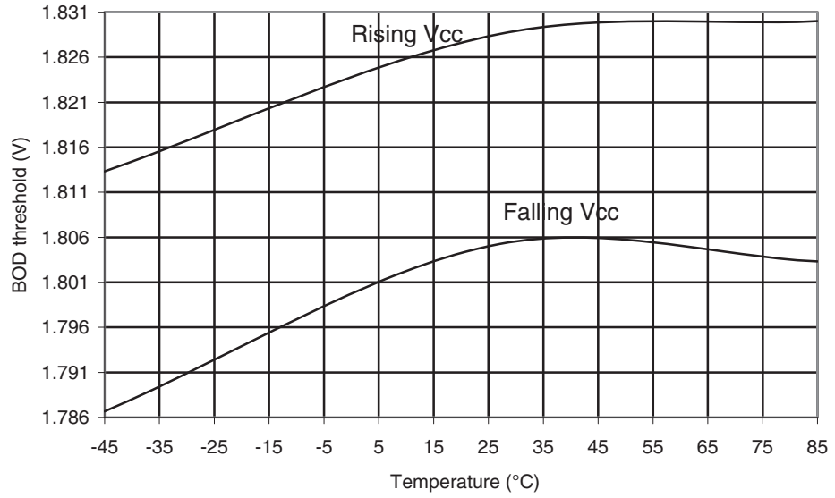
Figure 29-42. ATmega165A: BOD Thresholds vs. Temperature (BOD Level is 1.8V)
