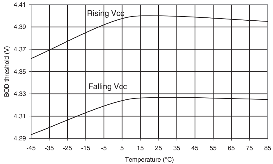
Figure 29-405. ATmega645A: BOD Thresholds vs. Temperature (BOD Level is 4.3V)
