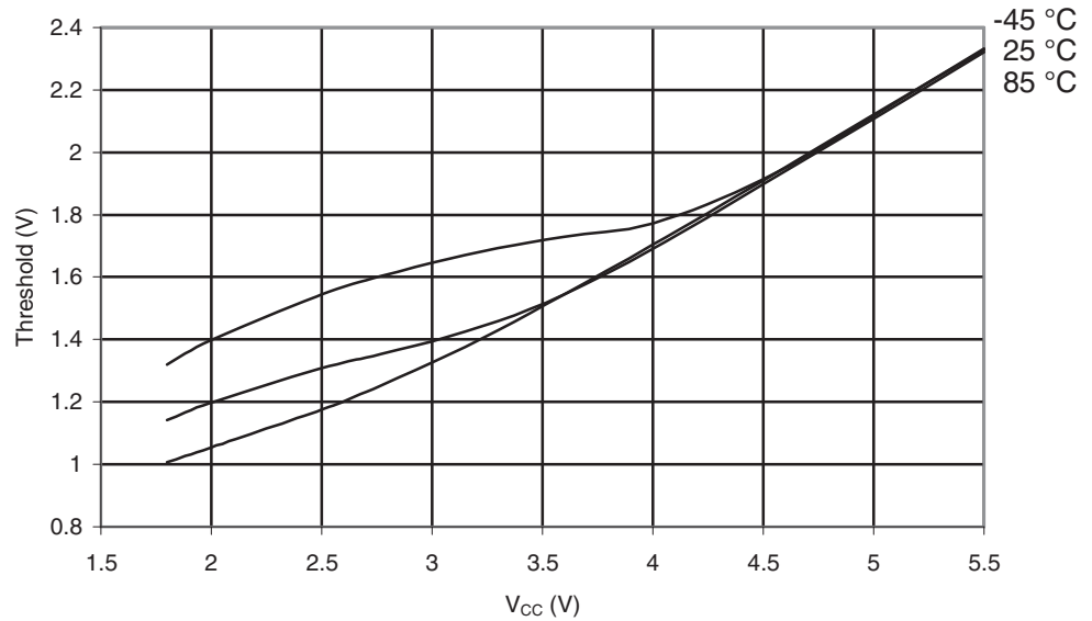
Figure 29-463. ATmega645P: Reset Input Threshold Voltage vs. V_{CC} ( V_{IH,Reset} , Reset Pin Read as "1")
