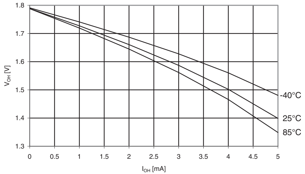
Figure 29-151. ATmega325A: I/O Pin Output Voltage vs. Source Current, Port B ( V_{CC} = 1.8V )
