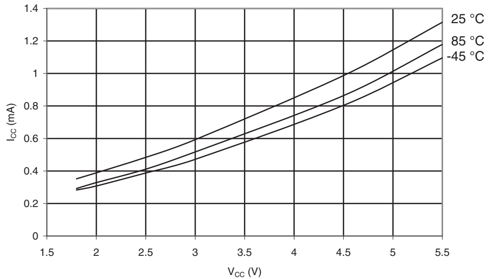
Figure 29-66. ATmega165PA: Active Supply Current vs. V_{CC} (Internal RC Oscillator, 1MHz)
