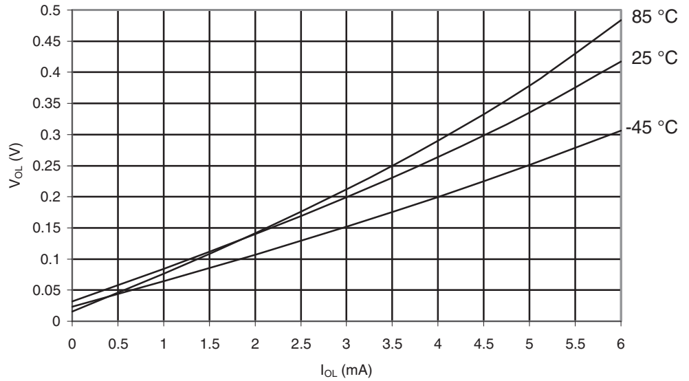
Figure 29-459. ATmega645P: I/O Pin Output Voltage vs. Sink Current, Port B ( V_{CC} = 1.8V )
