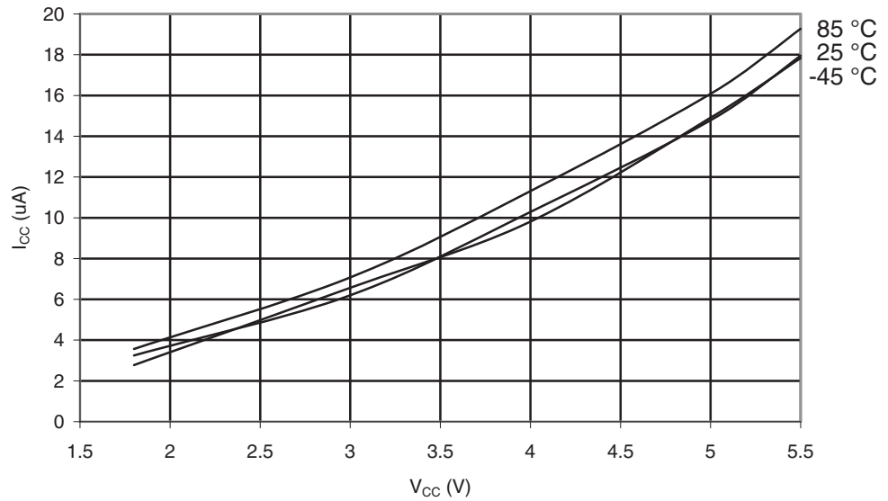
Figure 29-74. ATmega165PA: Power-down Supply Current vs. V_{CC} (Watchdog Timer Enabled)
