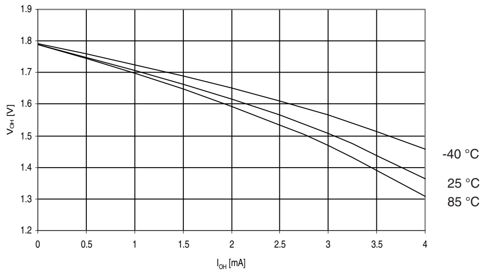
Figure 29-268. ATmega3250A: I/O Pin Output Voltage vs. Source Current, Ports A, C, D, E, F, G ( V_{CC} = 1.8V )
