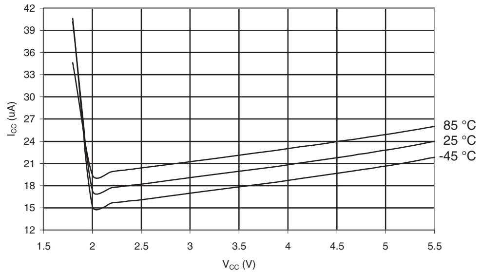
Figure 29-598. ATmega6450P: Brownout Detector Current vs. V_{CC}
