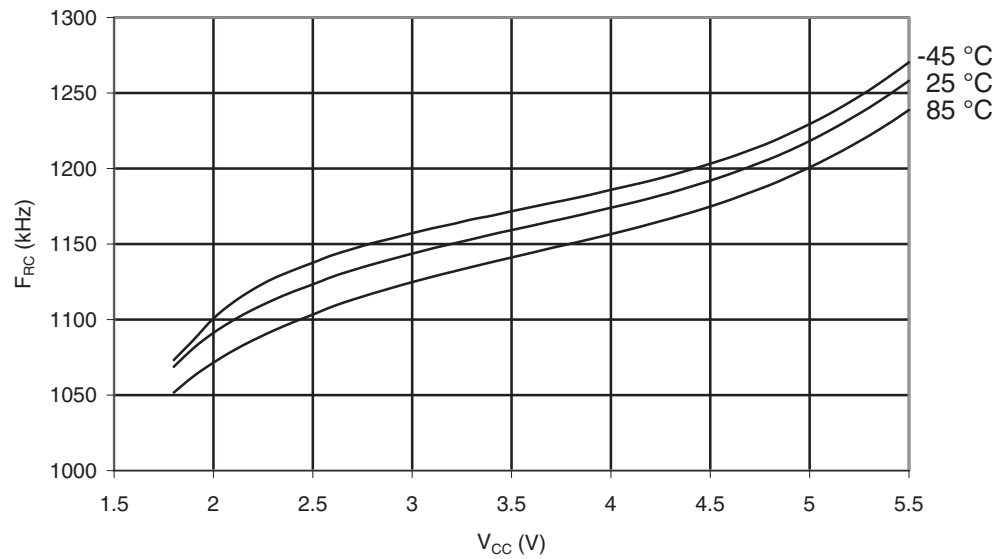
Figure 29-47. ATmega165A: Watchdog Oscillator Frequency vs. V_{CC}
