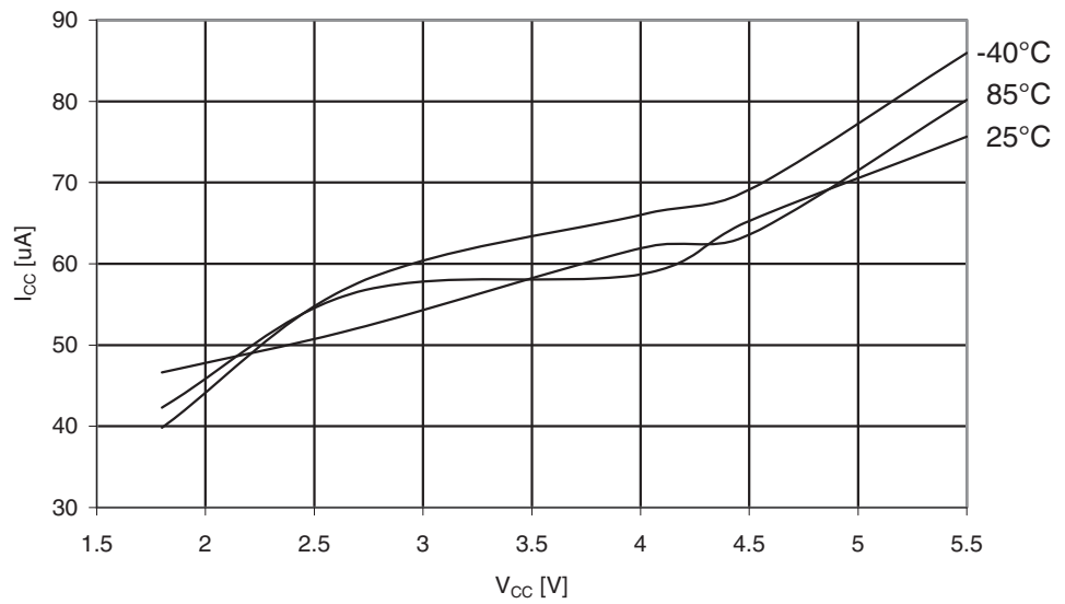
Figure 29-180. ATmega325A: Analog Comparator Current vs. V_{CC}
