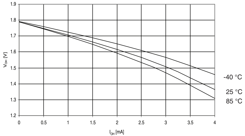
Figure 29-148. ATmega325A: I/O Pin Output Voltage vs. Source Current, Ports A, C, D, E, F, G ( V_{CC} = 1.8V )
