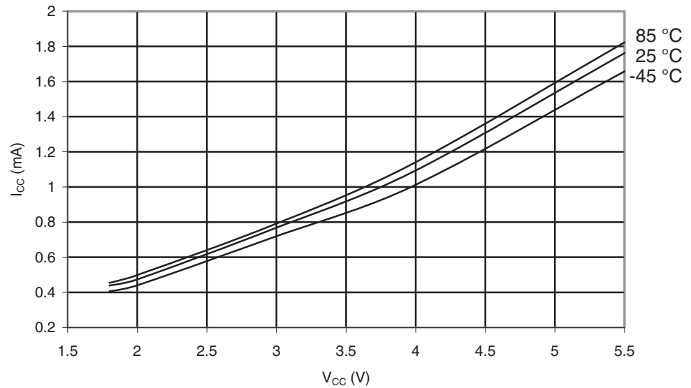
Figure 29-433. ATmega645P: Idle Supply Current vs. V_{CC} (Internal RC Oscillator, 8MHz)
