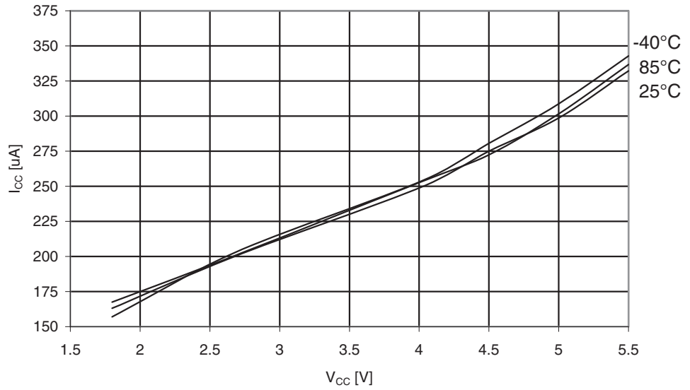
Figure 29-235. ATmega325PA: Active Supply Current with ADC at 50kHz vs. V_{CC}
