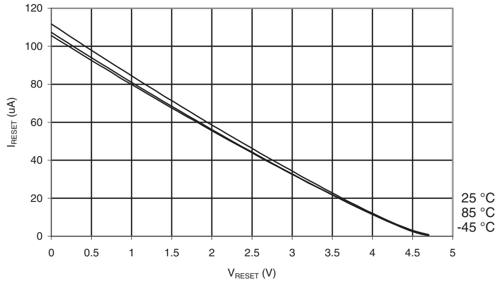
Figure 29-81. ATmega165PA: Reset Pull-up Resistor Current vs. Reset Pin Voltage ( V_{CC} = 5V )
