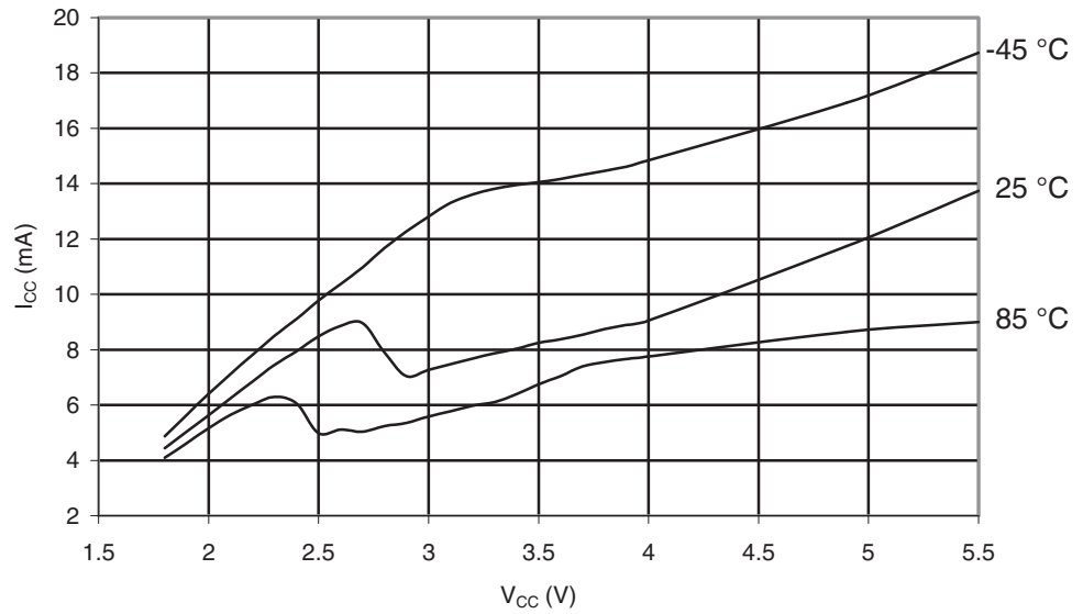
Figure 29-483. ATmega645P: Programming Current vs. V_{CC}
