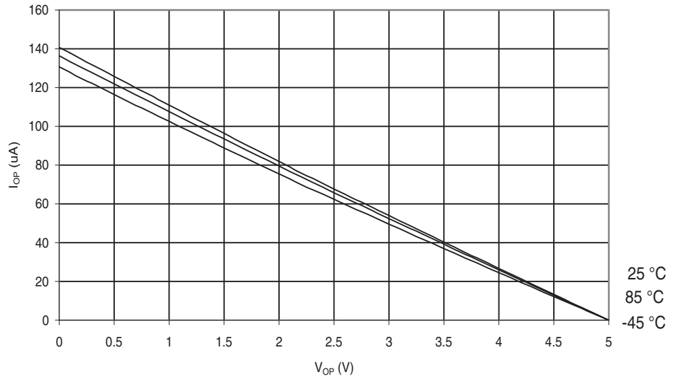
Figure 29-442. ATmega645P: I/O Pin Pull-up Resistor Current vs. Input Voltage ( V_{CC} = 5V )
