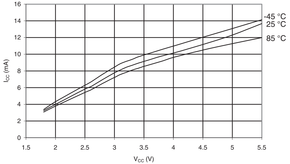
Figure 29-59. ATmega165A: Programming Current vs. V_{CC}
