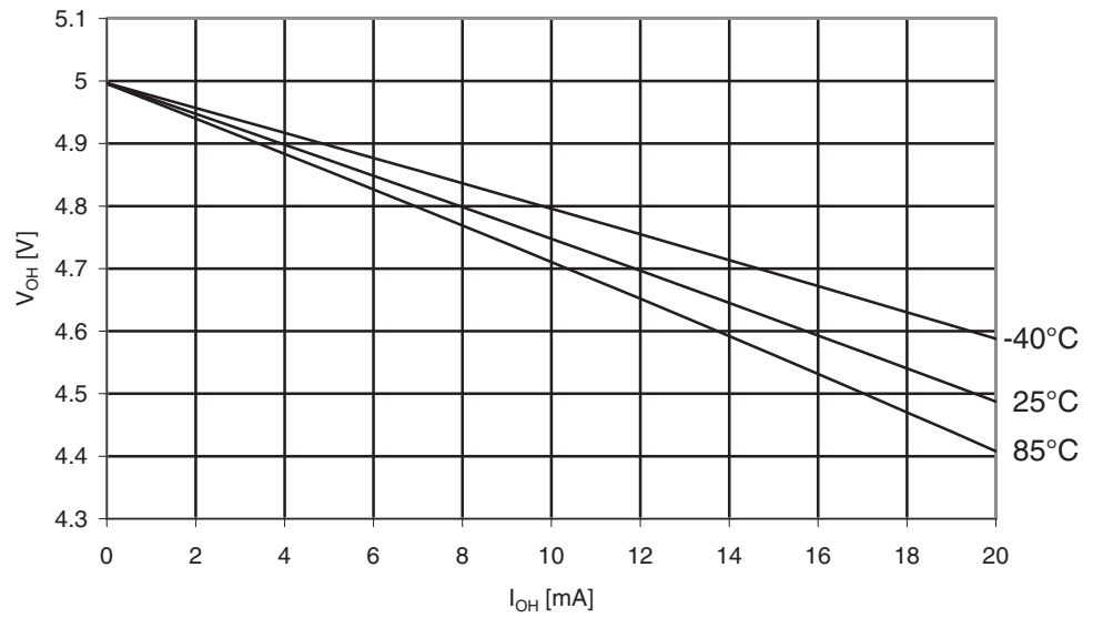
Figure 29-329. ATmega3250PA: I/O Pin Output Voltage vs. Source Current, Port B ( V_{CC} = 5V )
