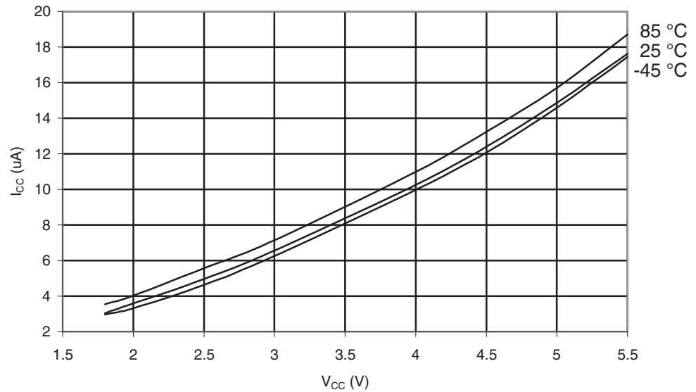
Figure 29-498. ATmega6450A: Power-down Supply Current vs. V_{CC} (Watchdog Timer Enabled)
