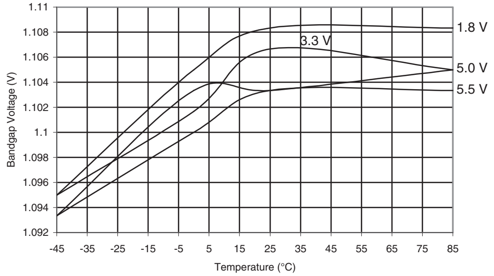
Figure 29-592. ATmega6450P: Bandgap Voltage vs. Temperature
