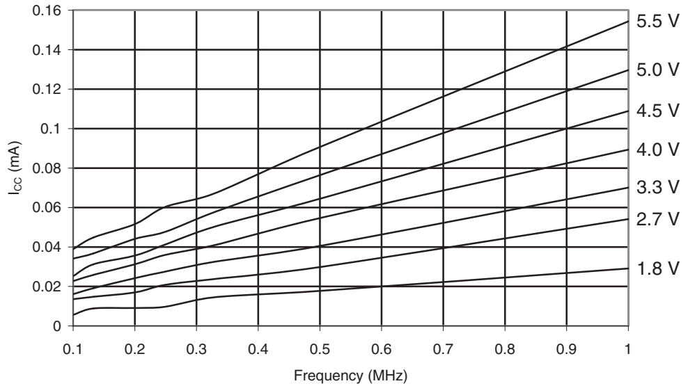
Figure 29-60. ATmega165A: Reset Supply Current vs. V_{CC} (0.1 - 1.0MHz, Excluding Current Through The Reset Pull-up)
