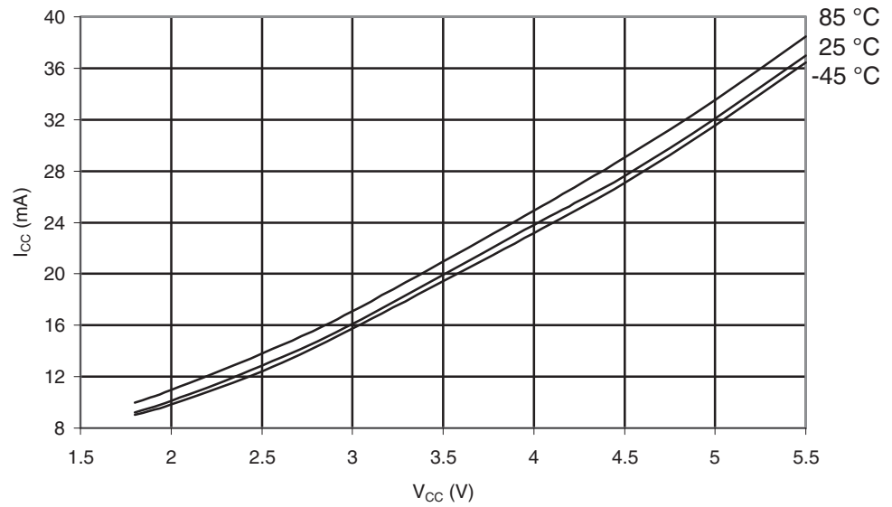
Figure 29-552. ATmega6450A: Active Supply Current vs. V_{CC} (32kHz Watch Crystal)
