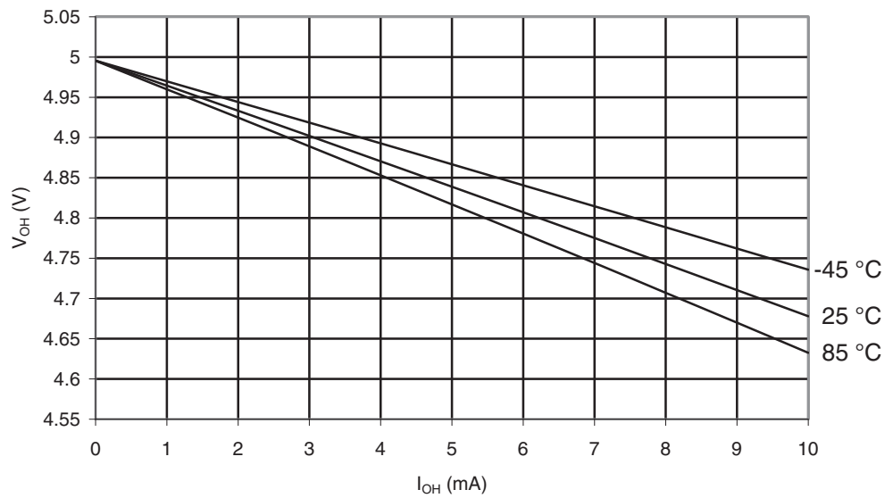
Figure 29-84. ATmega165PA: I/O Pin Output Voltage vs. Source Current, Ports A, C, D, E, F, G ( V_{CC} = 5V )
