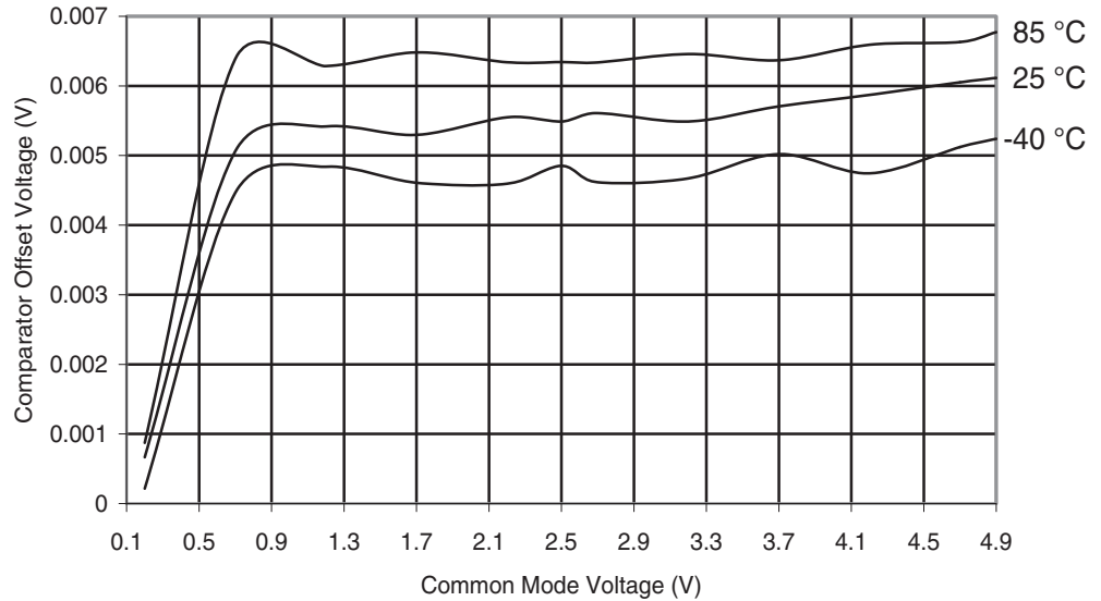
Figure 29-45. ATmega165A: Analog Comparator Offset Voltage vs. Common Mode Voltage ( V_{CC} = 5V )
