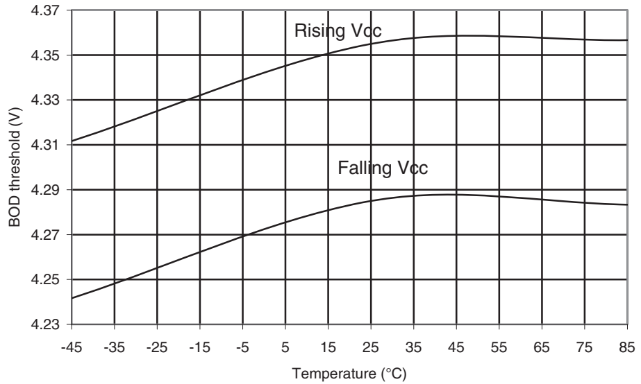
Figure 29-40. ATmega165A: BOD Thresholds vs. Temperature (BOD Level is 4.3V)
