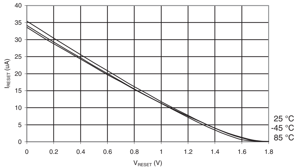
Figure 29-447. ATmega645P: Reset Pull-up Resistor Current vs. Reset Pin Voltage ( V_{CC} = 1.8V )
