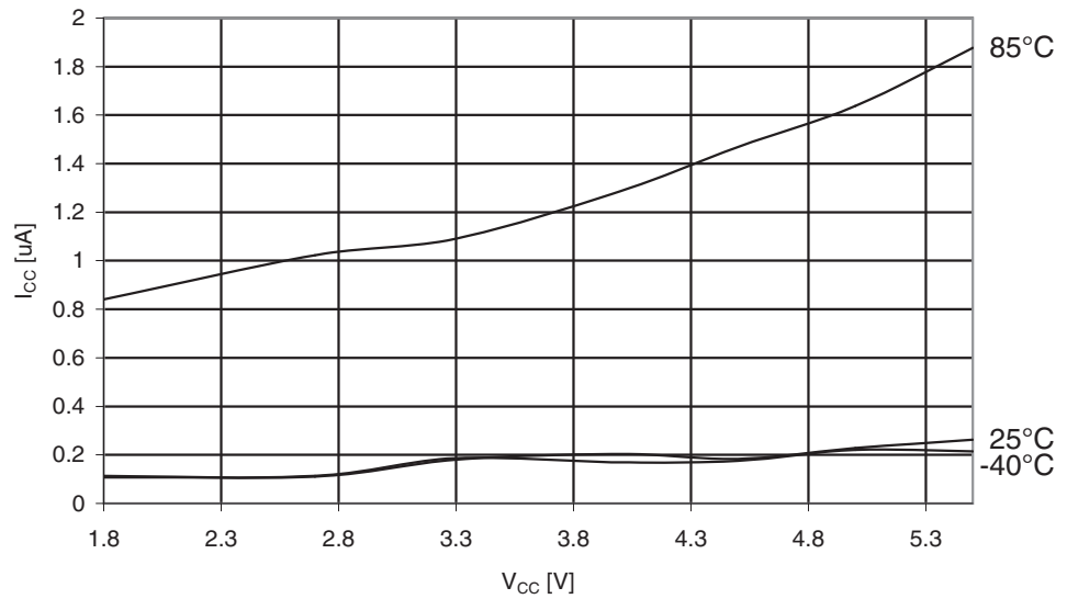
Figure 29-315. ATmega3250PA: Power-down Supply Current vs. V_{CC} (Watchdog Timer Disabled)
