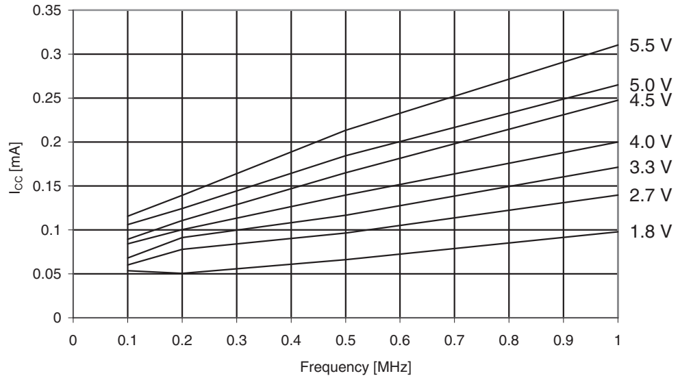
Figure 29-250. ATmega3250A: Idle Supply Current vs. Frequency (0.1 - 1.0MHz)
