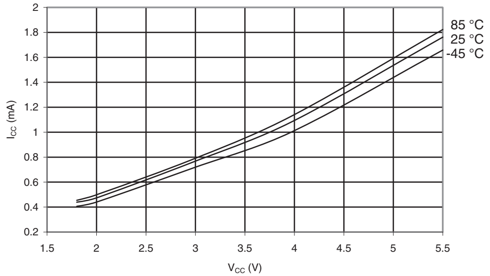
Figure 29-367. ATmega645A: Active Supply Current vs. V_{CC} (Internal RC Oscillator, 8MHz)
