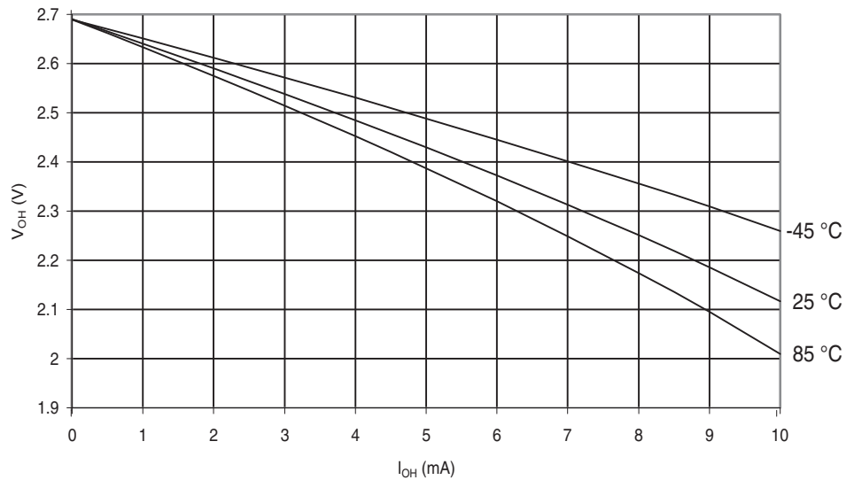
Figure 29-571. ATmega6450A: I/O Pin Output Voltage vs. Source Current, Ports A, C, D, E, F, G ( V_{CC} = 2.7V )
