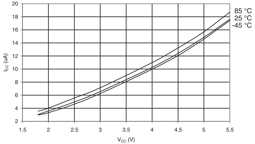
Figure 29-559. ATmega6450A: Power-down Supply Current vs. V_{CC} (Watchdog Timer Enabled)
