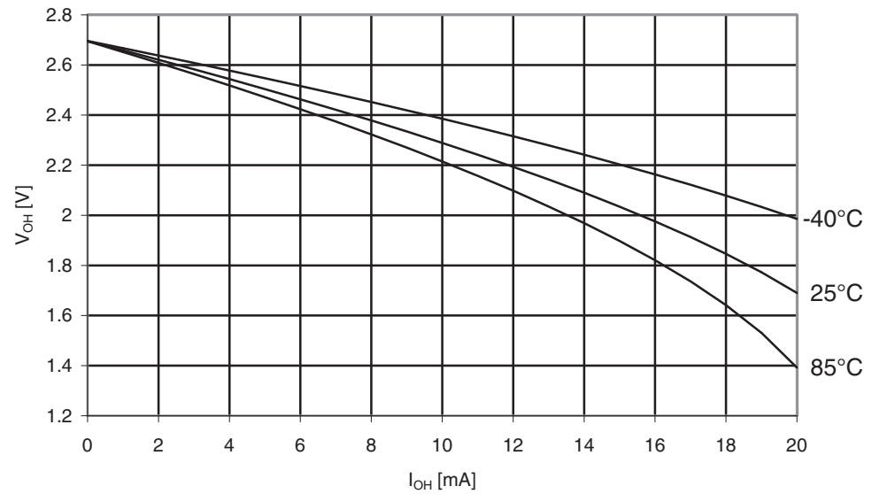
Figure 29-150. ATmega325A: I/O Pin Output Voltage vs. Source Current, Port B ( V_{CC} = 2.7V )
