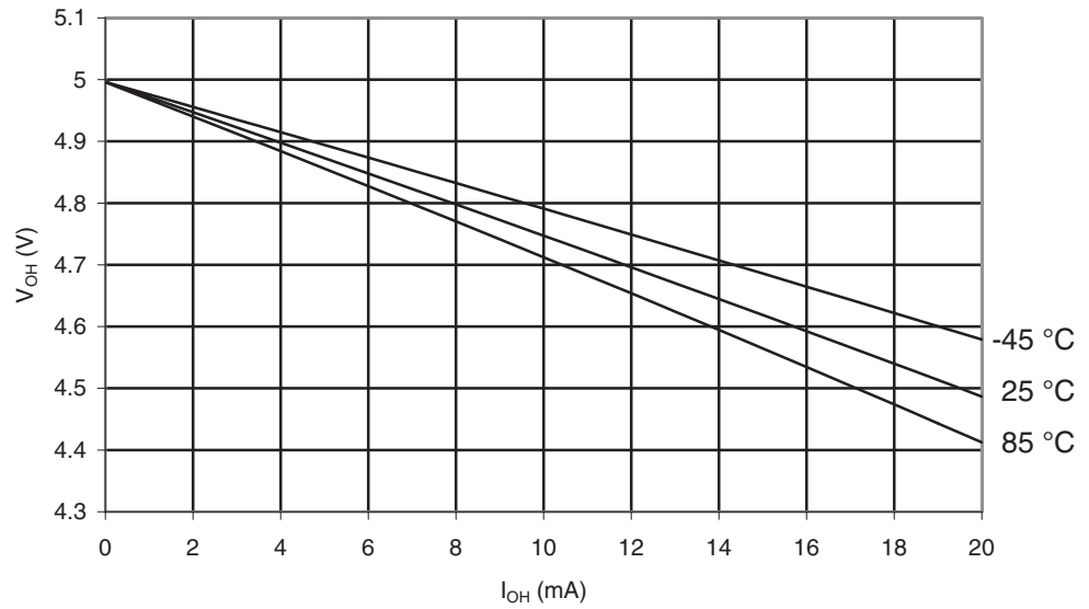
Figure 29-87. ATmega165PA: I/O Pin Output Voltage vs. Source Current, Port B ( V_{CC} = 5V )
