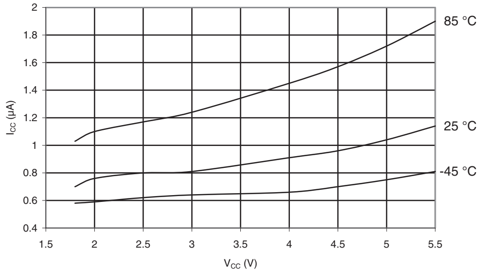
Figure 29-75. ATmega165PA: Power-save Supply Current vs. V_{CC} (Watchdog Timer Disabled)
