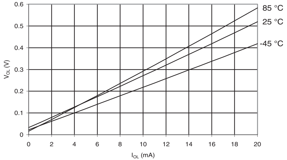
Figure 29-393. ATmega645A: I/O Pin Output Voltage vs. Sink Current, Ports A, C, D, E, F, G ( V_{CC} = 5V )
