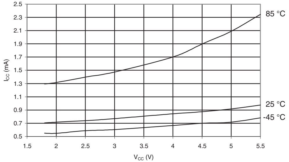
Figure 29-501. ATmega6450A: Standby Supply Current vs. V_{CC} (32kHz Watch Crystal, Watchdog Timer Disabled)
