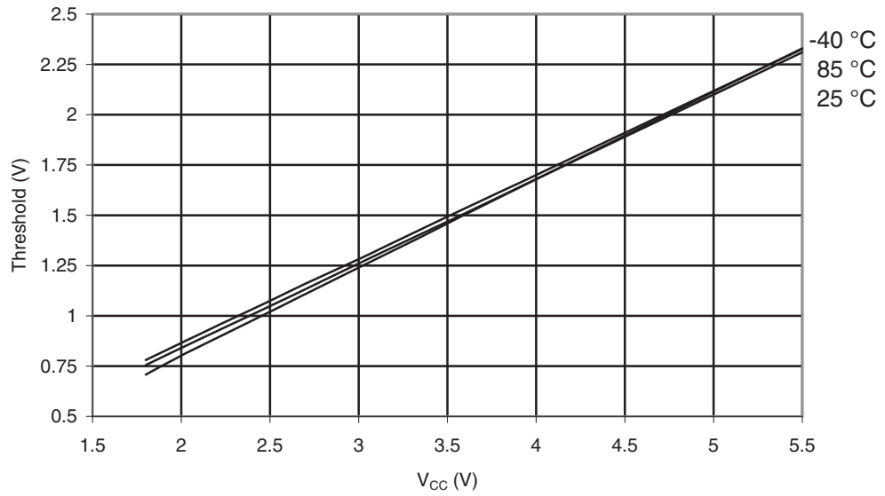
Figure 29-222. ATmega325PA: Reset Input Threshold Voltage vs. V_{CC} ( V_{IL} , Reset Pin Read as “0”)
