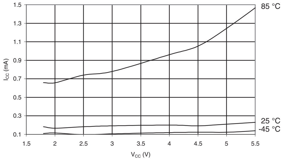
Figure 29-438. ATmega645P: Power-down Supply Current vs. V_{CC} (32kHz Watch Crystal)
