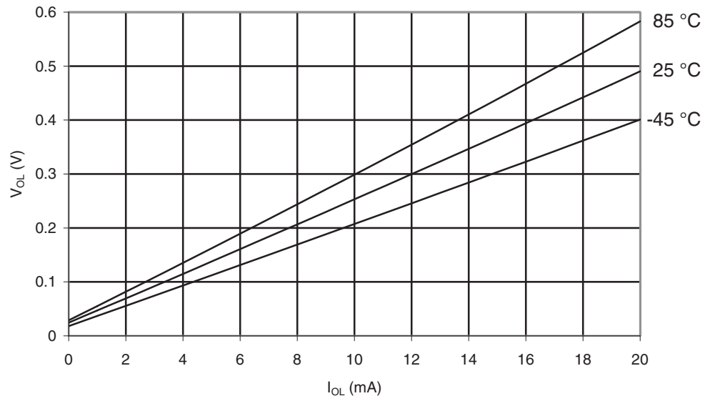
Figure 29-93. ATmega165PA: I/O Pin Output Voltage vs. Sink Current, Port B ( V_{CC} = 5V )
