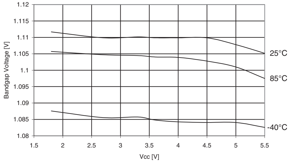
Figure 29-227. ATmega325PA: Bandgap Voltage vs. V_{CC}
