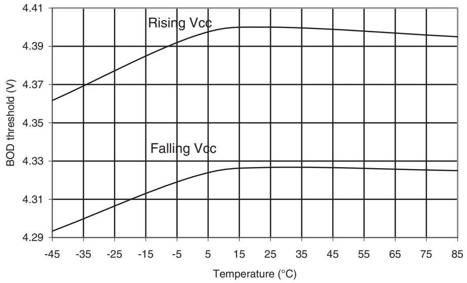
Figure 29-588. ATmega6450P: BOD Thresholds vs. Temperature (BOD Level is 4.3V)
