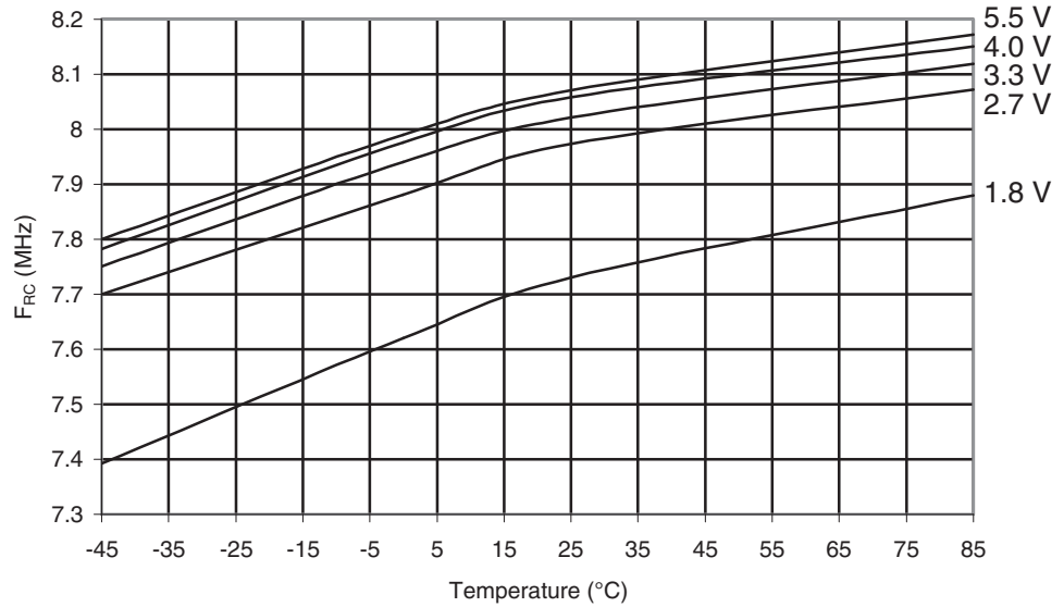
Figure 29-534. ATmega6450A: Calibrated 8MHz RC Oscillator Frequency vs. Temperature
