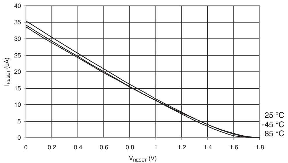
Figure 29-508. ATmega6450A: Reset Pull-up Resistor Current vs. Reset Pin Voltage ( V_{CC} = 1.8V )
