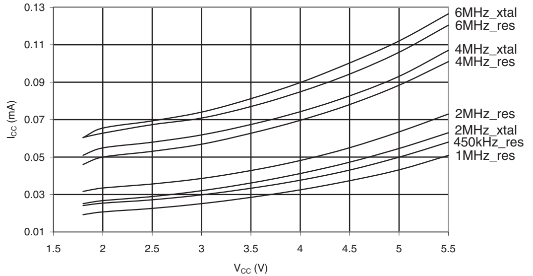
Figure 29-199. ATmega325PA: Standby Supply Current vs. V_{CC} (Xtall and Resonator, Watchdog Timer Disabled)
