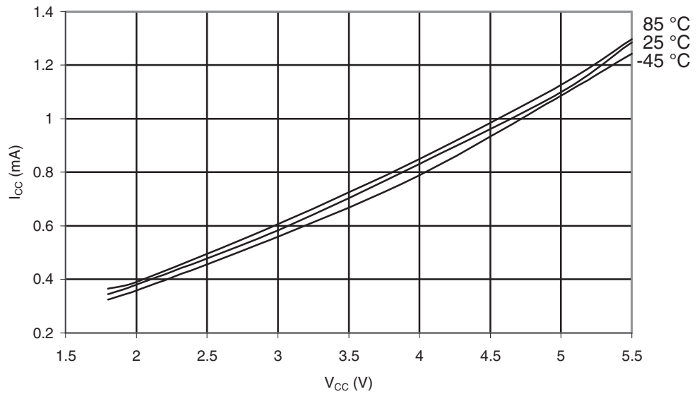
Figure 29-368. ATmega645A: Active Supply Current vs. V_{CC} (Internal RC Oscillator, 1MHz)
