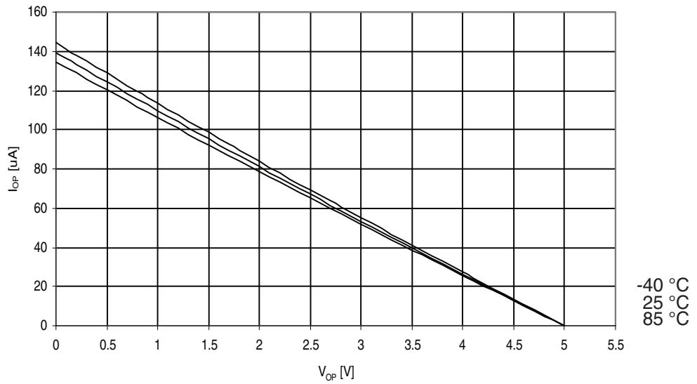
Figure 29-260. ATmega3250A: I/O Pin Pull-up Resistor Current vs. Input Voltage ( V_{CC} = 5V )
