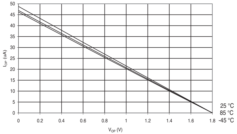
Figure 29-566. ATmega6450A: I/O Pin Pull-up Resistor Current vs. Input Voltage ( V_{CC} = 1.8V )
