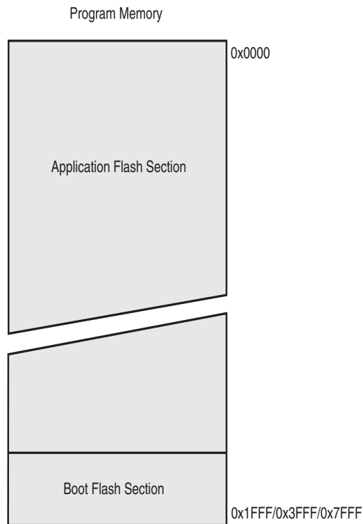
Figure 8-1. Program Memory Map
