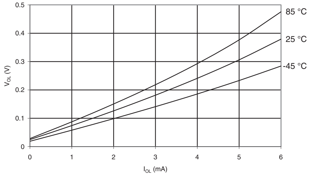
Figure 29-95. ATmega165PA: I/O Pin Output Voltage vs. Sink Current, Port B ( V_{CC} = 1.8V )
