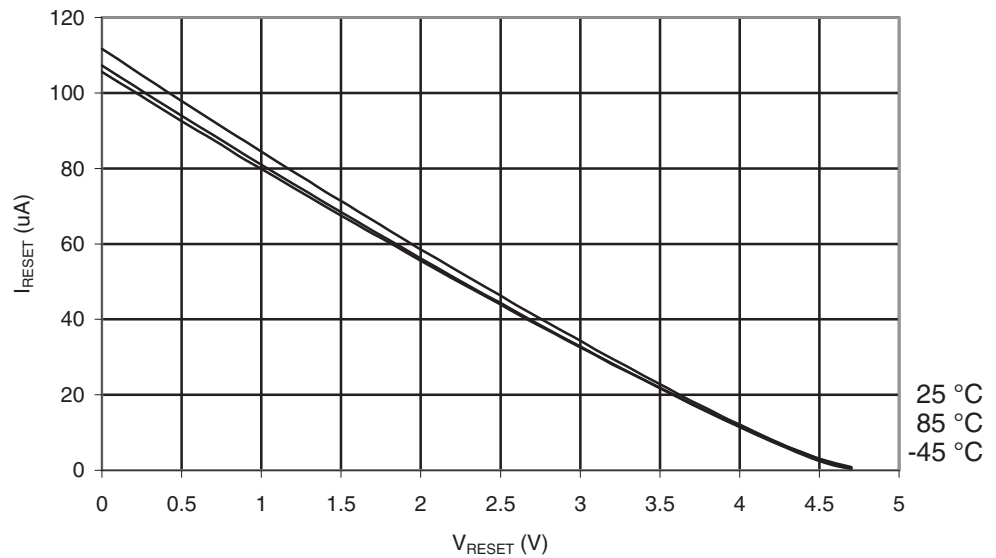
Figure 29-19. ATmega165A: Reset Pull-up Resistor Current vs. Reset Pin Voltage ( V_{CC} = 5V )
