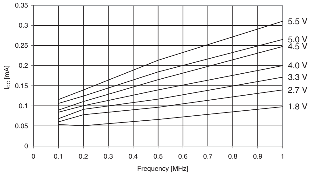
Figure 29-310. ATmega3250PA: Idle Supply Current vs. Frequency (0.1 - 1.0MHz)
