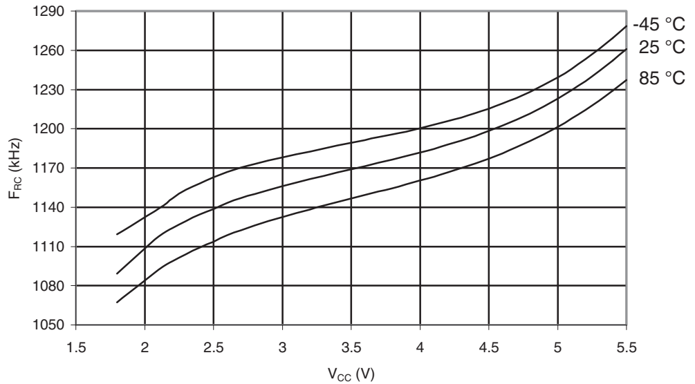
Figure 29-471. ATmega645P: Watchdog Oscillator Frequency vs. V_{CC}
