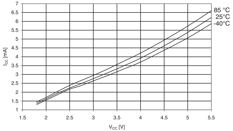
Figure 29-247. ATmega3250A: Active Supply Current vs. V_{CC} (Internal RC Oscillator, 8MHz)
