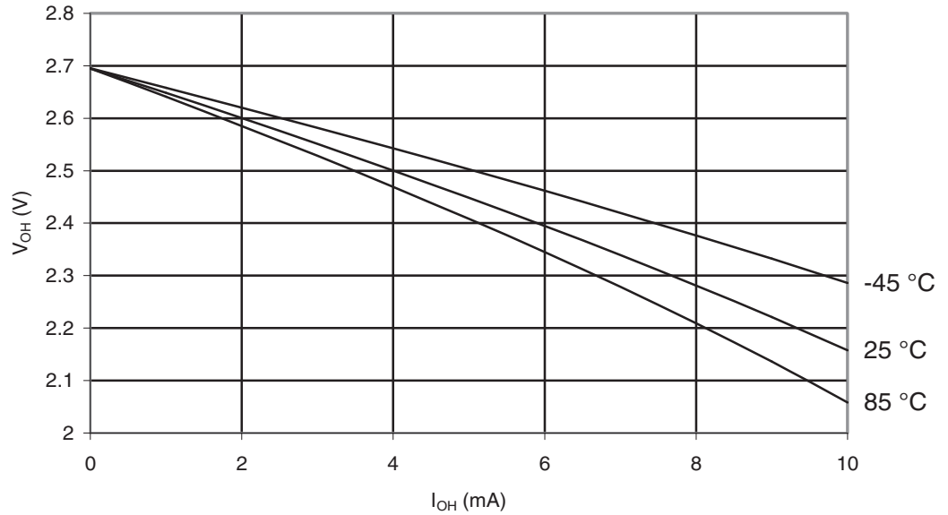
Figure 29-85. ATmega165PA: I/O Pin Output Voltage vs. Source Current, Ports A, C, D, E, F, G ( V_{CC} = 2.7V )
