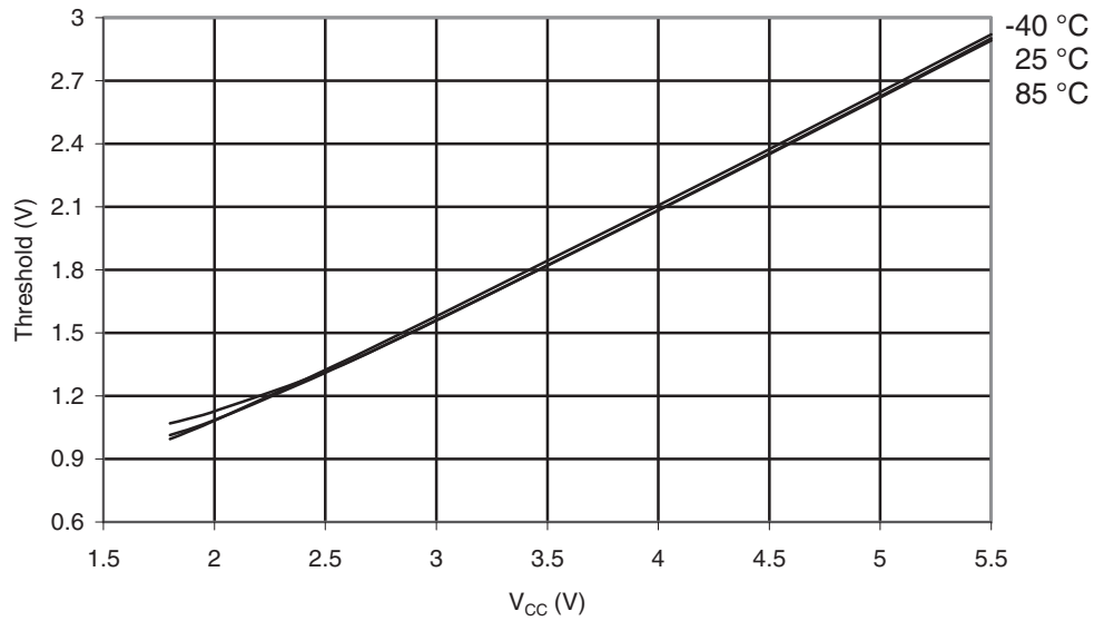
Figure 29-218. ATmega325PA: I/O Pin Input Threshold Voltage vs. V_{CC} ( V_{IH} , I/O Pin Read as "1")
