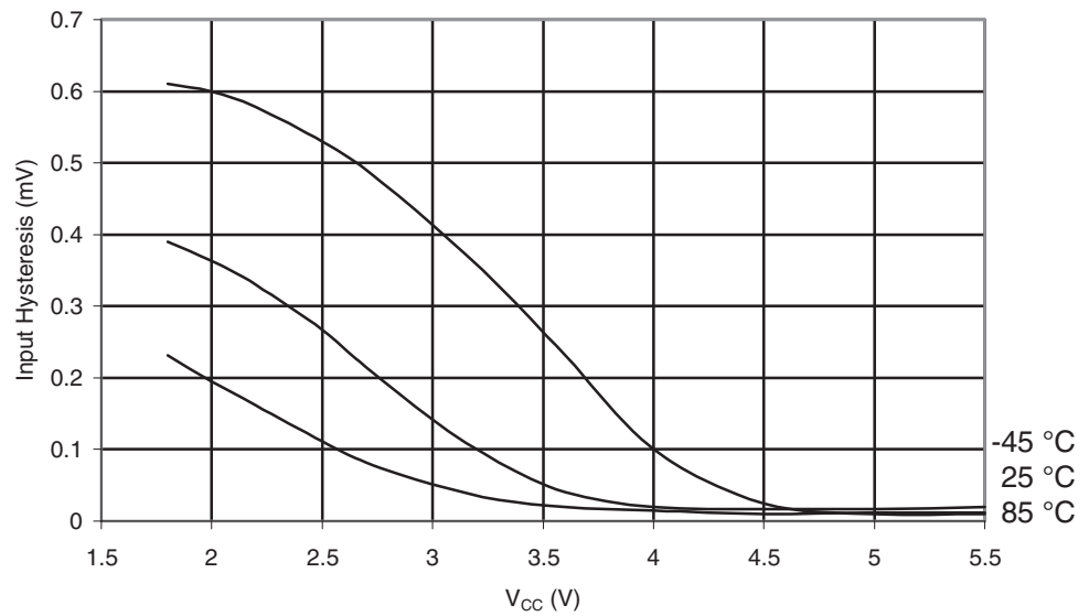
Figure 29-465. ATmega645P: Reset Input Pin Hysteresis vs. V_{CC}
