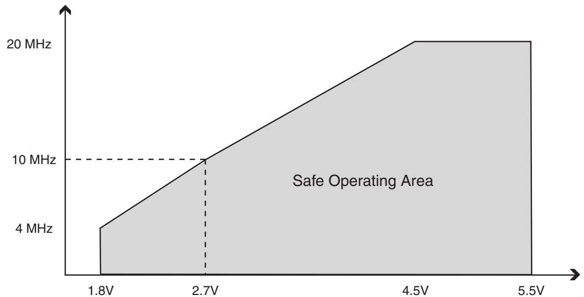
Figure 28-2. Maximum Frequency vs. V_{CC} (10 - 20MHz) ATmega325A/ATmega325PA/ATmega3250A/ATmega3250PA/ATmega6450A/ ATmega6450P
