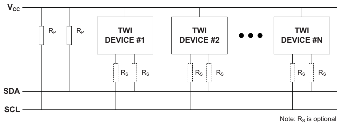
Figure 21-1. TWI bus topology.
