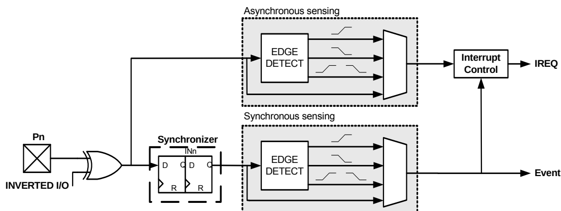
Figure 13-9. Input sensing.
