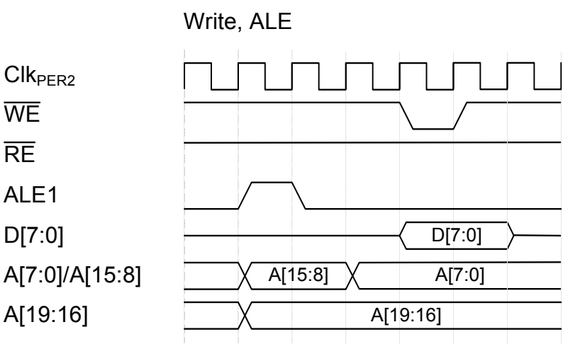
Figure 36-26. Write, ALE
