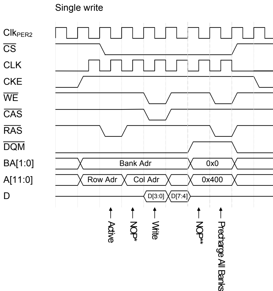
Figure 36-44. Single write
