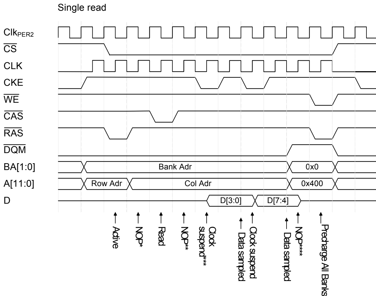
Figure 36-48. Single read
