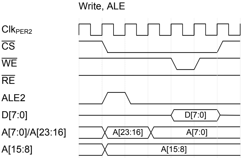
Figure 36-12. Write, ALE
