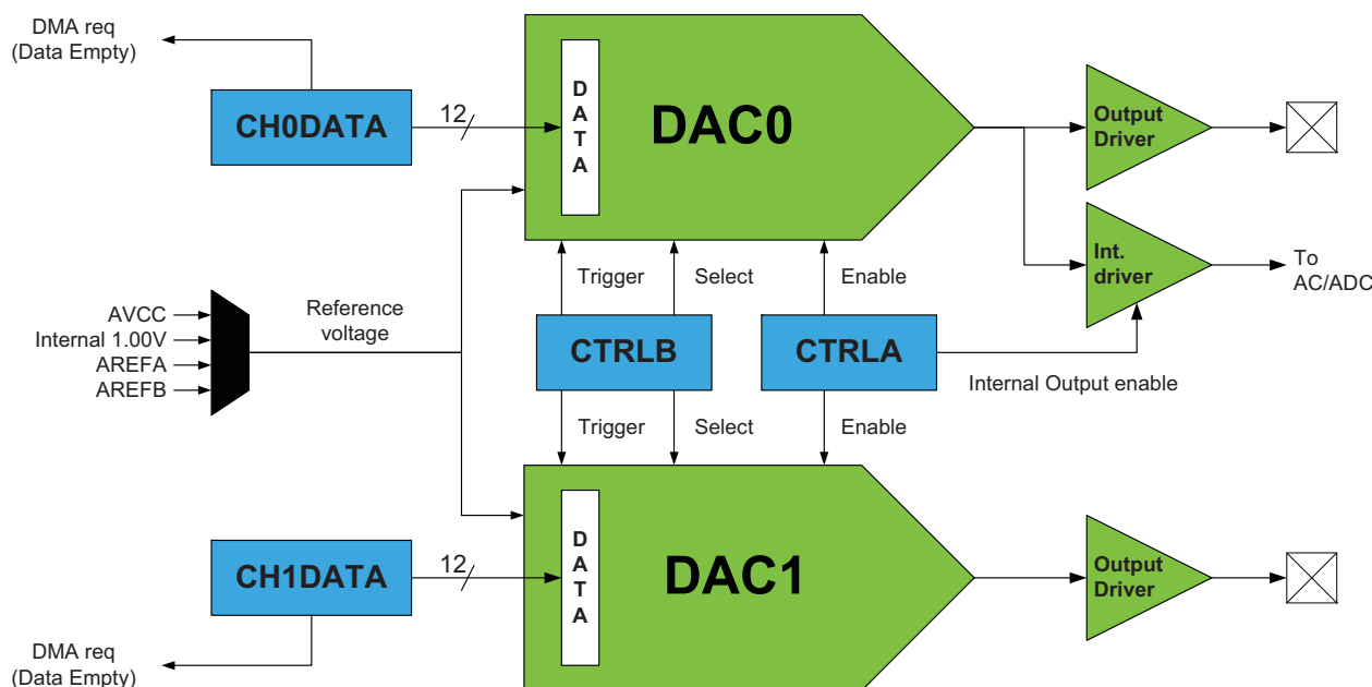
Figure 29-1. DAC overview.
