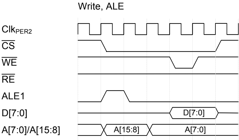
Figure 36-2. Write, ALE
