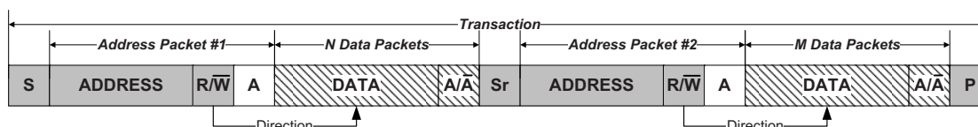
Figure 21-7. Combined Transaction.
