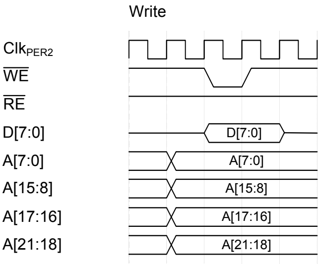
Figure 36-29.Write
