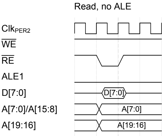
Figure 36-27.Read, no ALE
