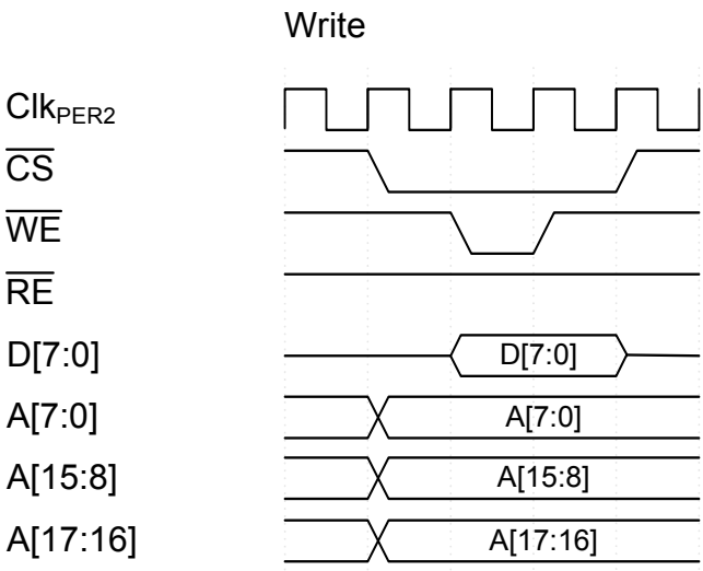
Figure 36-15. Write
