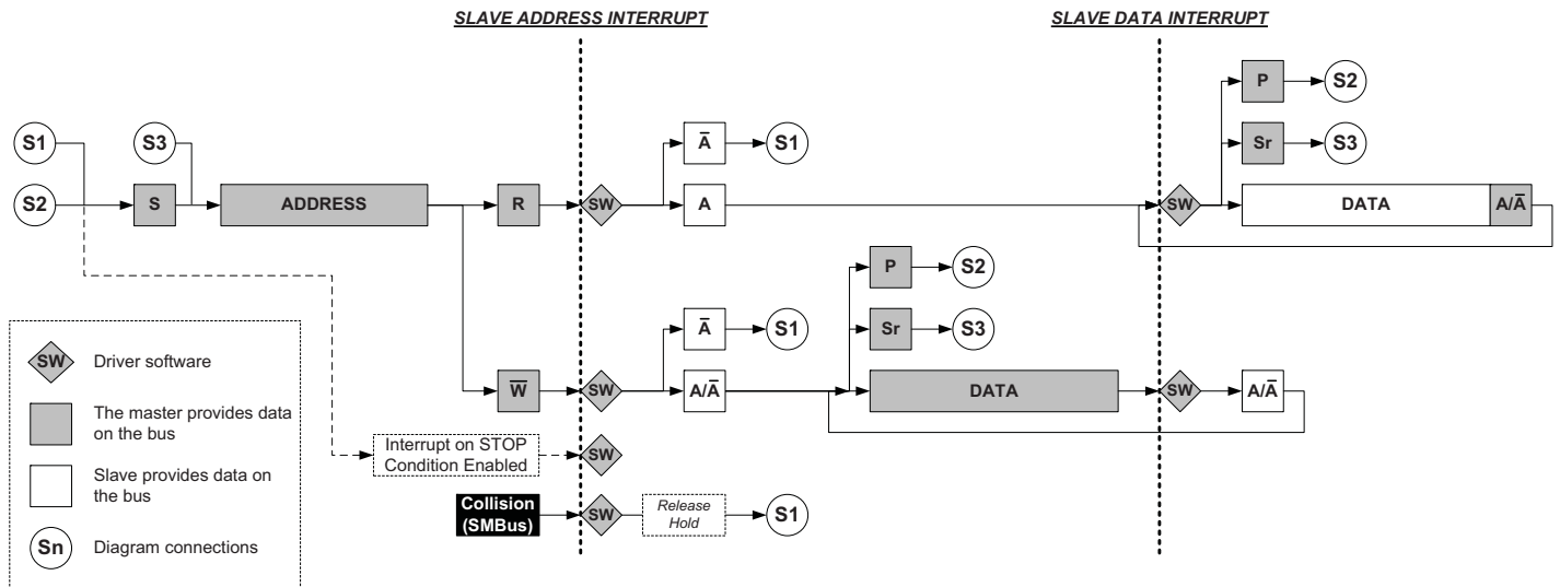
Figure 21-13.TWI slave operation.
