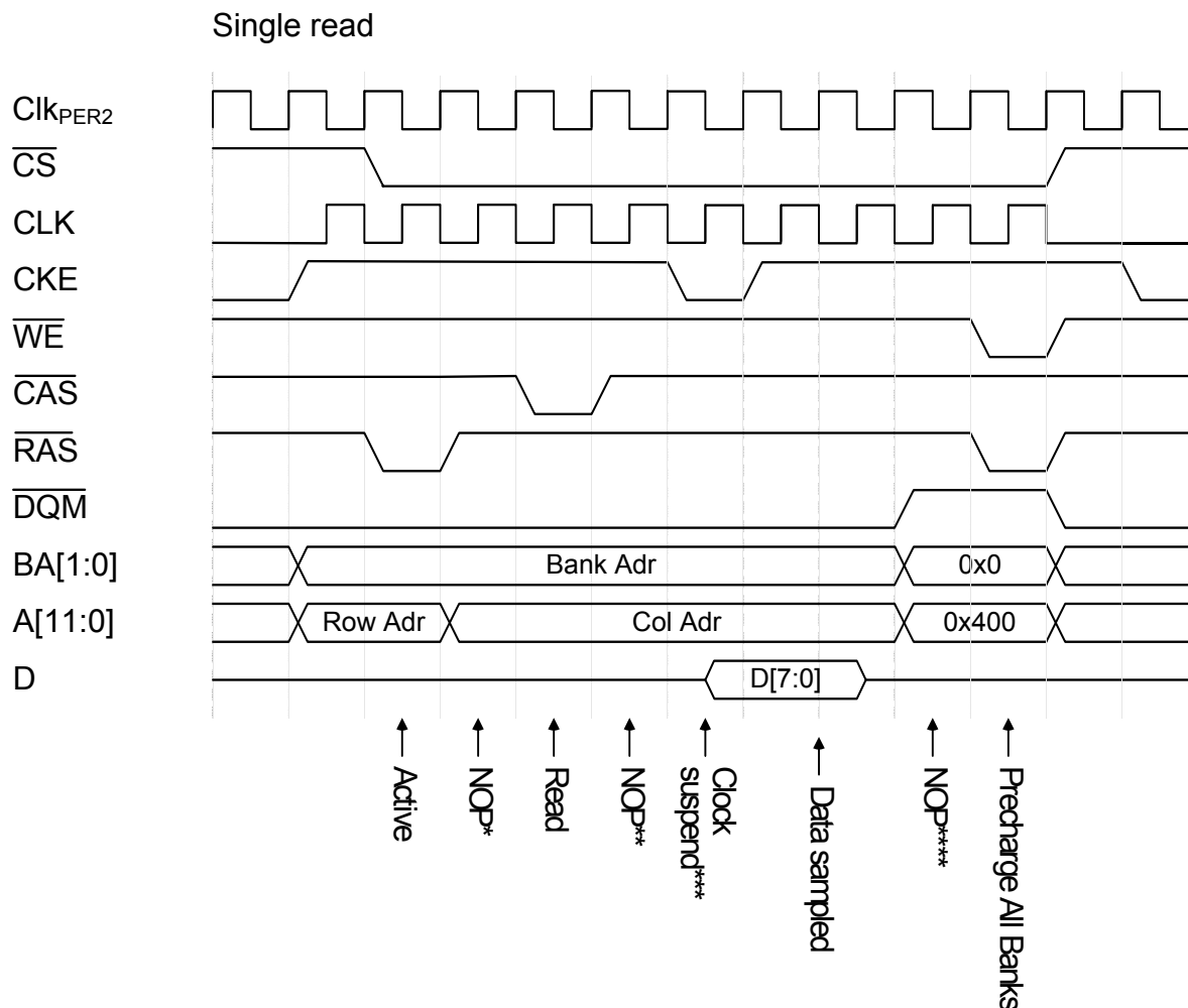
Figure 36-40. Single read
