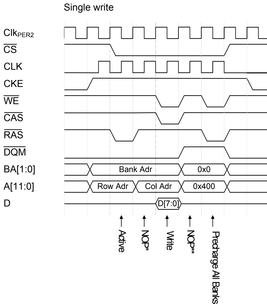
Figure 36-36. Single write
