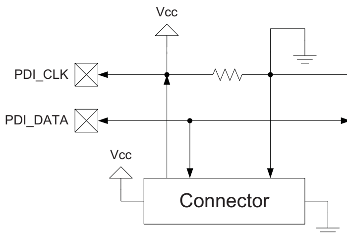
Figure 32-2. PDI connection.
