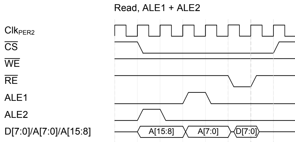
Figure 36-20.Read, ALE1 + ALE2
