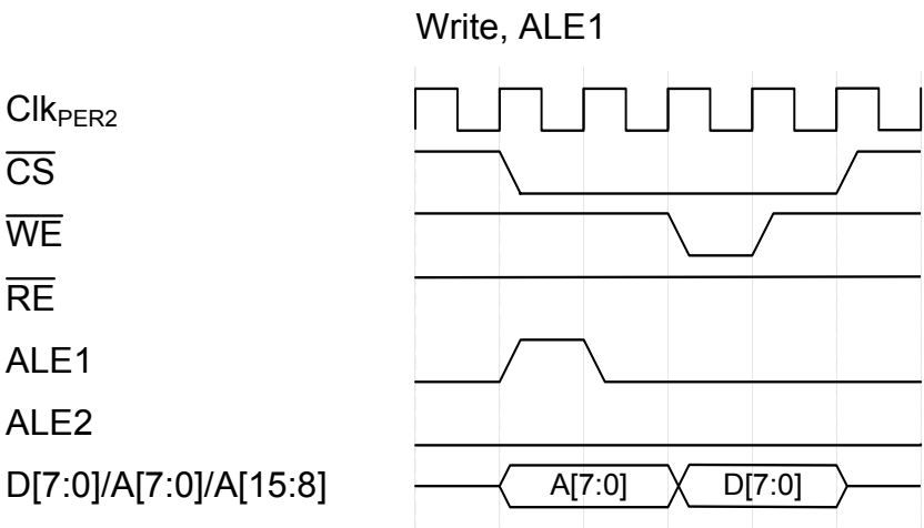
Figure 36-17. Write, ALE1
