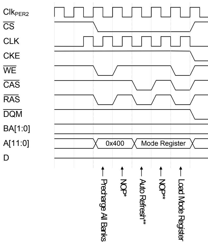
Figure 36-35.SDRAM init
