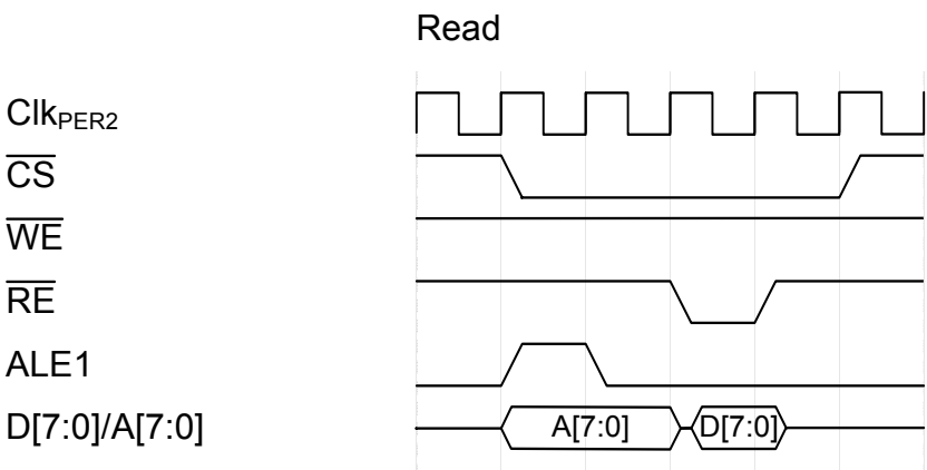
Figure 36-24. Read
