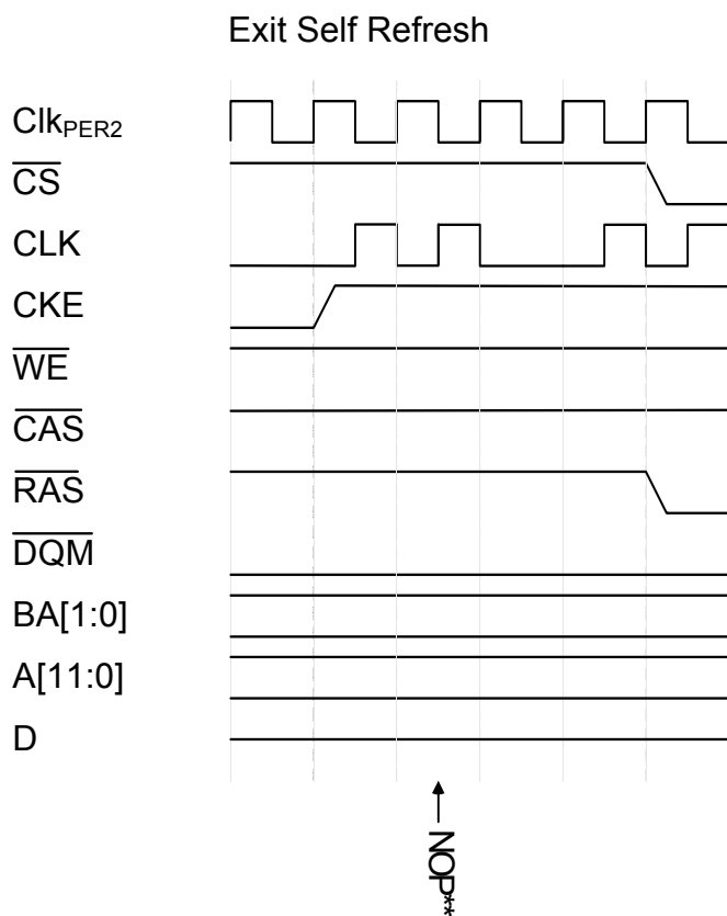
Figure 36-55.Exit Self Refresh
