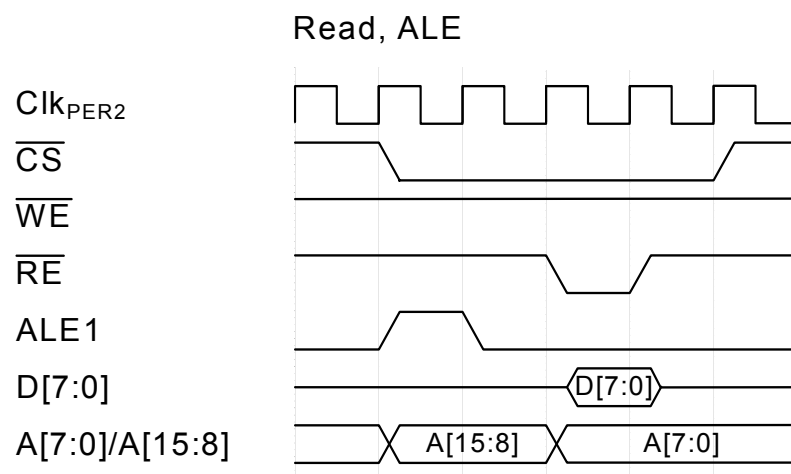
Figure 36-4. Read, ALE
