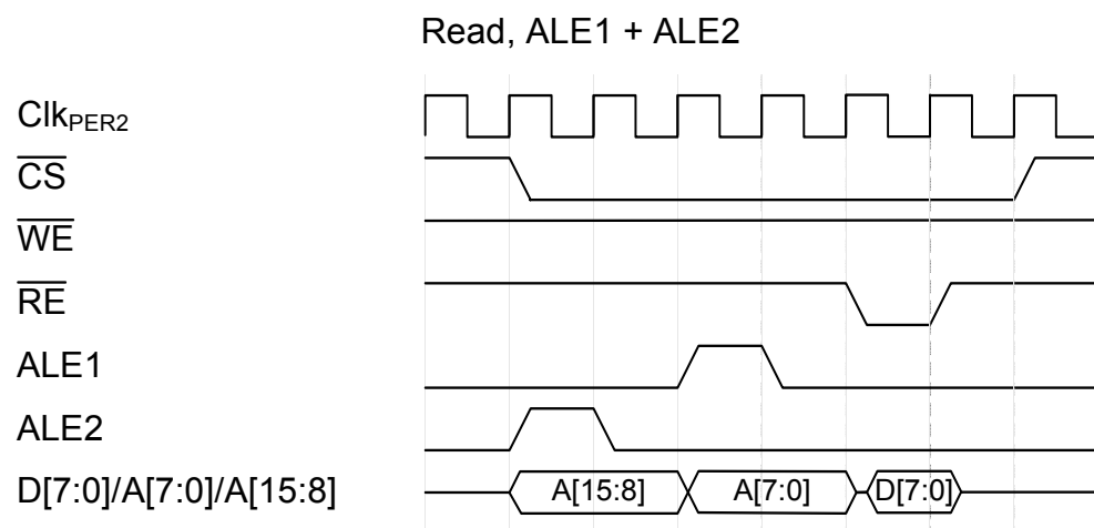
Figure 36-34.Read, ALE1 + ALE2
