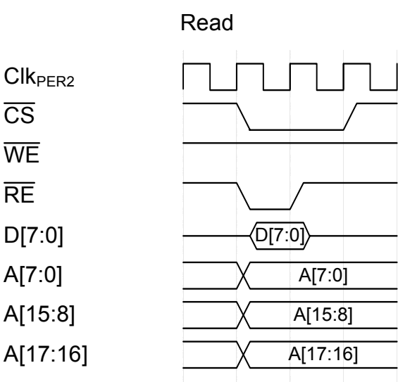
Figure 36-16. Read
