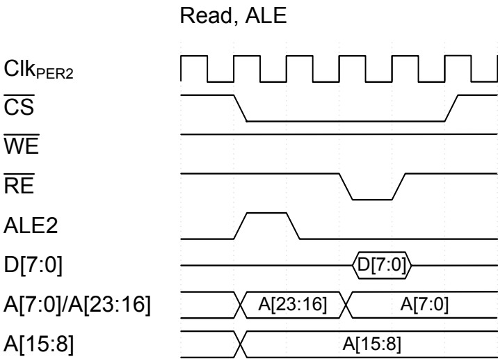
Figure 36-14.Read, ALE
