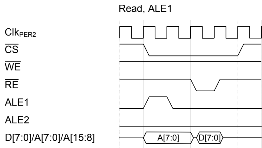
Figure 36-33.Read, ALE1
