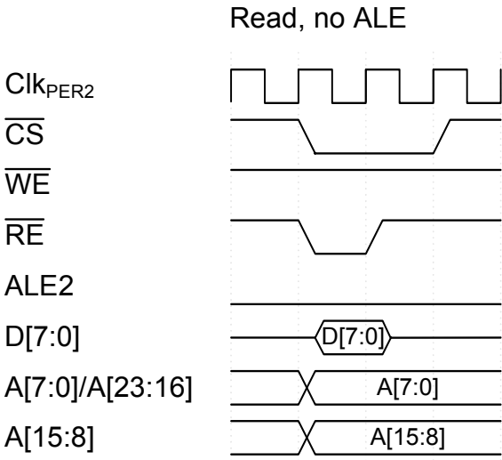
Figure 36-13.Read, no ALE
