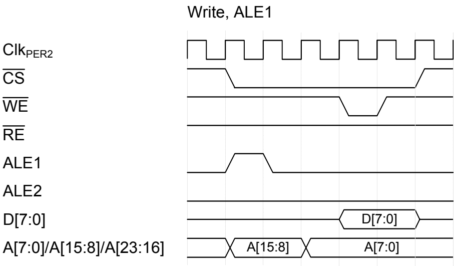
Figure 36-6. Write, ALE1
