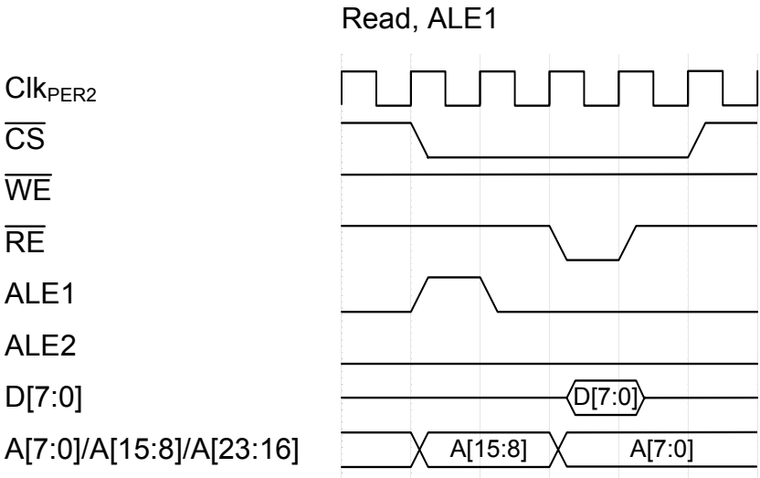
Figure 36-9. Read, ALE1
