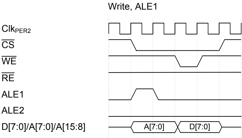
Figure 36-31. Write, ALE1
