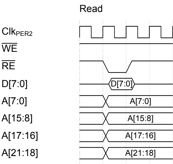
Figure 36-30.Read
