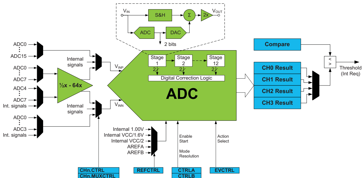
Figure 28-1. ADC overview.
