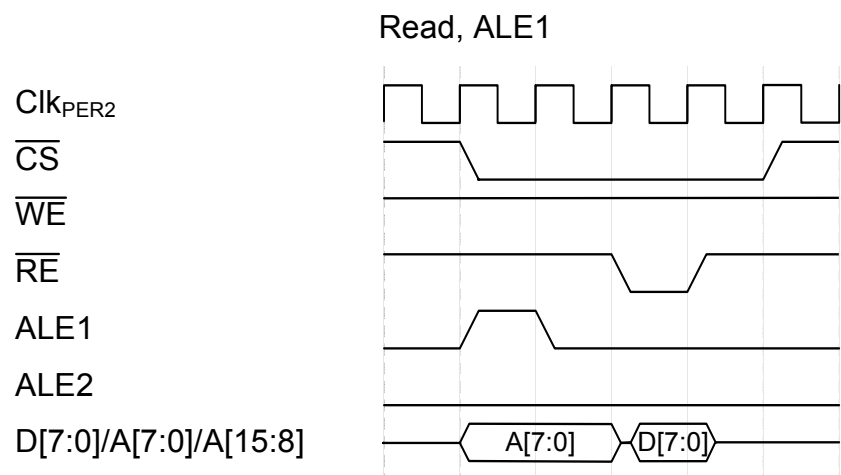
Figure 36-19.Read, ALE1
