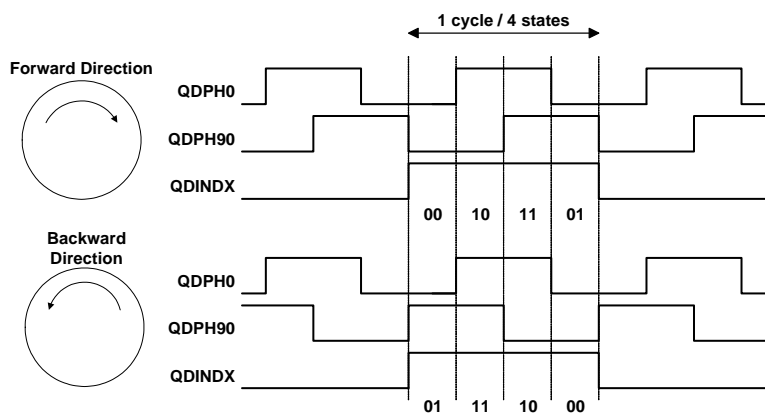
Figure 5-4. Quadrature signals from a rotary encoder
