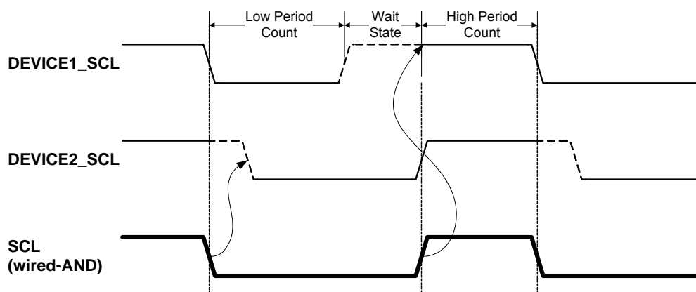
Figure 16-10. Clock Synchronization
