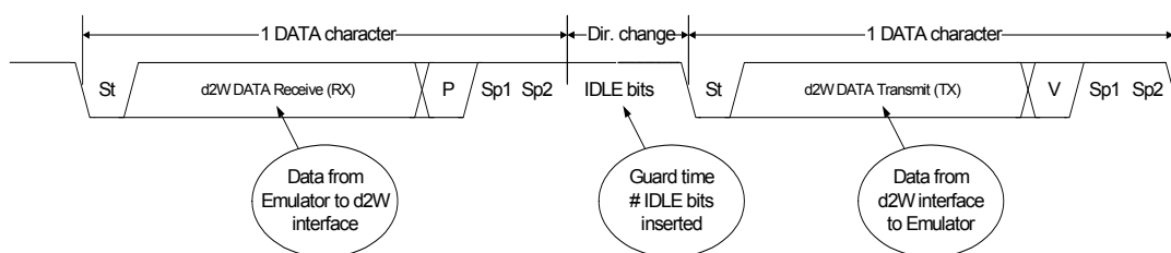
Figure 22-9. PDI direction change by inserting IDLE bits
