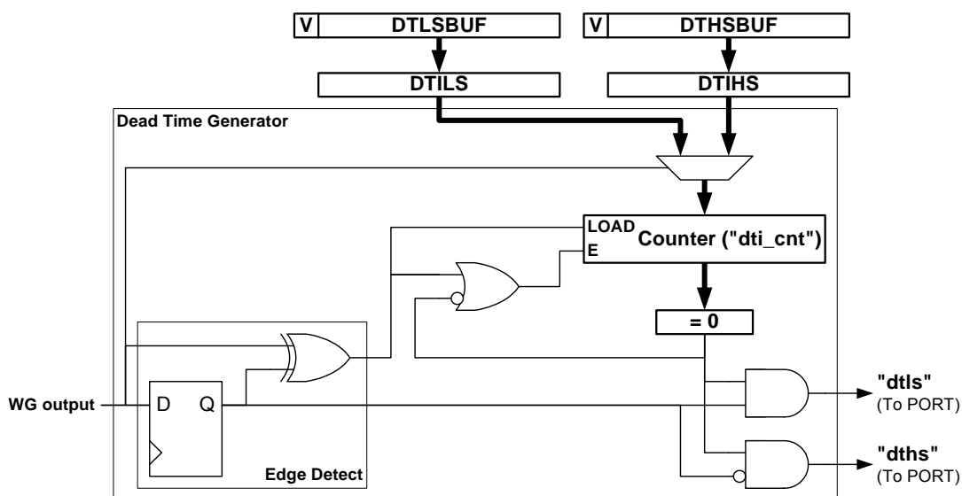
Figure 14-3. Dead Time Generator block diagram
