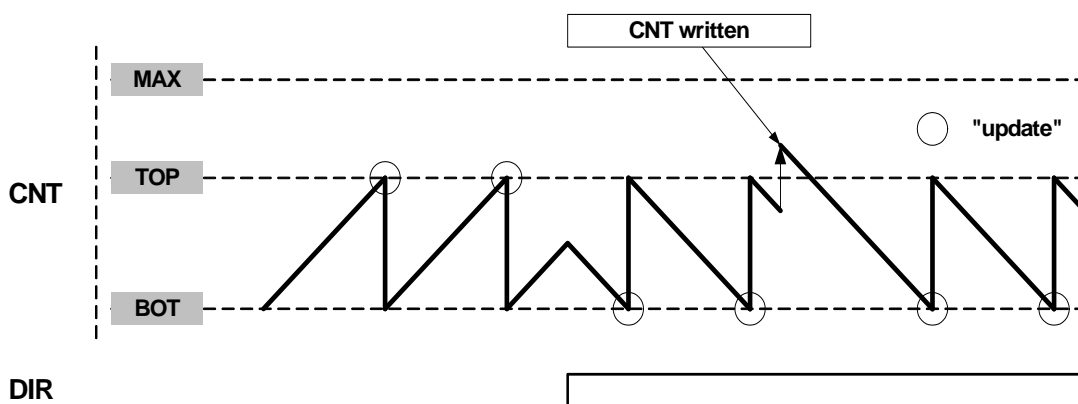
Figure 12-6. Normal Mode of Operation
