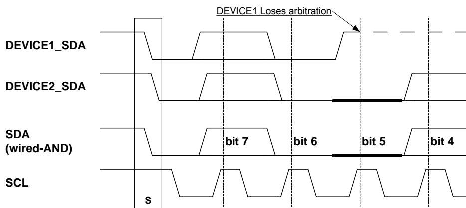
Figure 16-9. TWI Arbitration
