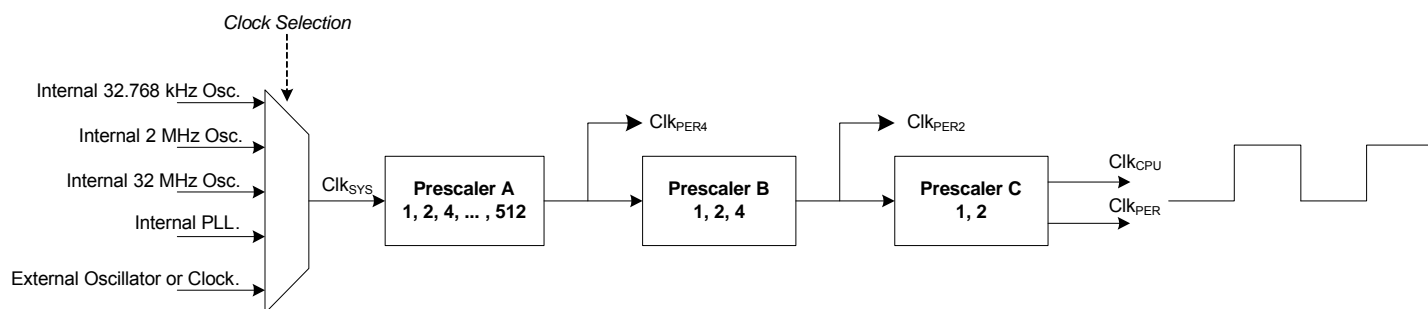
Figure 6-5. System Clock Selection and Prescalers
