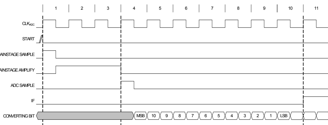
Figure 20-16. ADC timing for one single conversion with 32x or 64x gain
