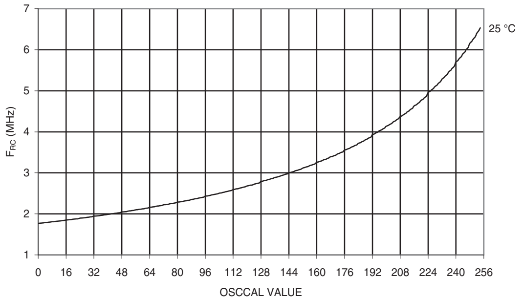
Figure 26-57. Calibrated 4MHz RC Oscillator Frequency vs. OSCCAL Value
