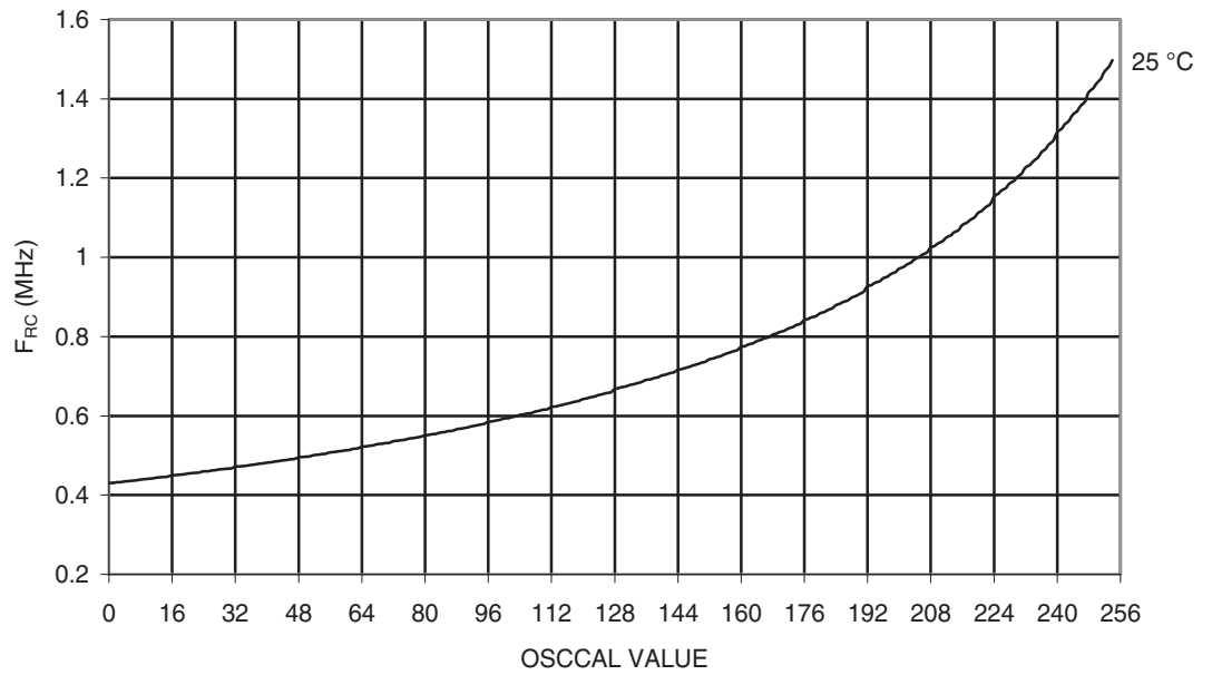
Figure 26-63. Calibrated 1MHz RC Oscillator Frequency vs. OSCCAL Value
