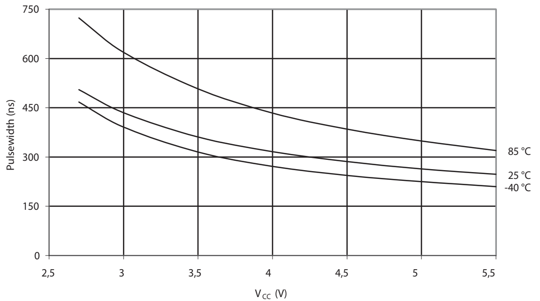
Figure 26-73. Reset Pulse Width vs. V_{CC}
