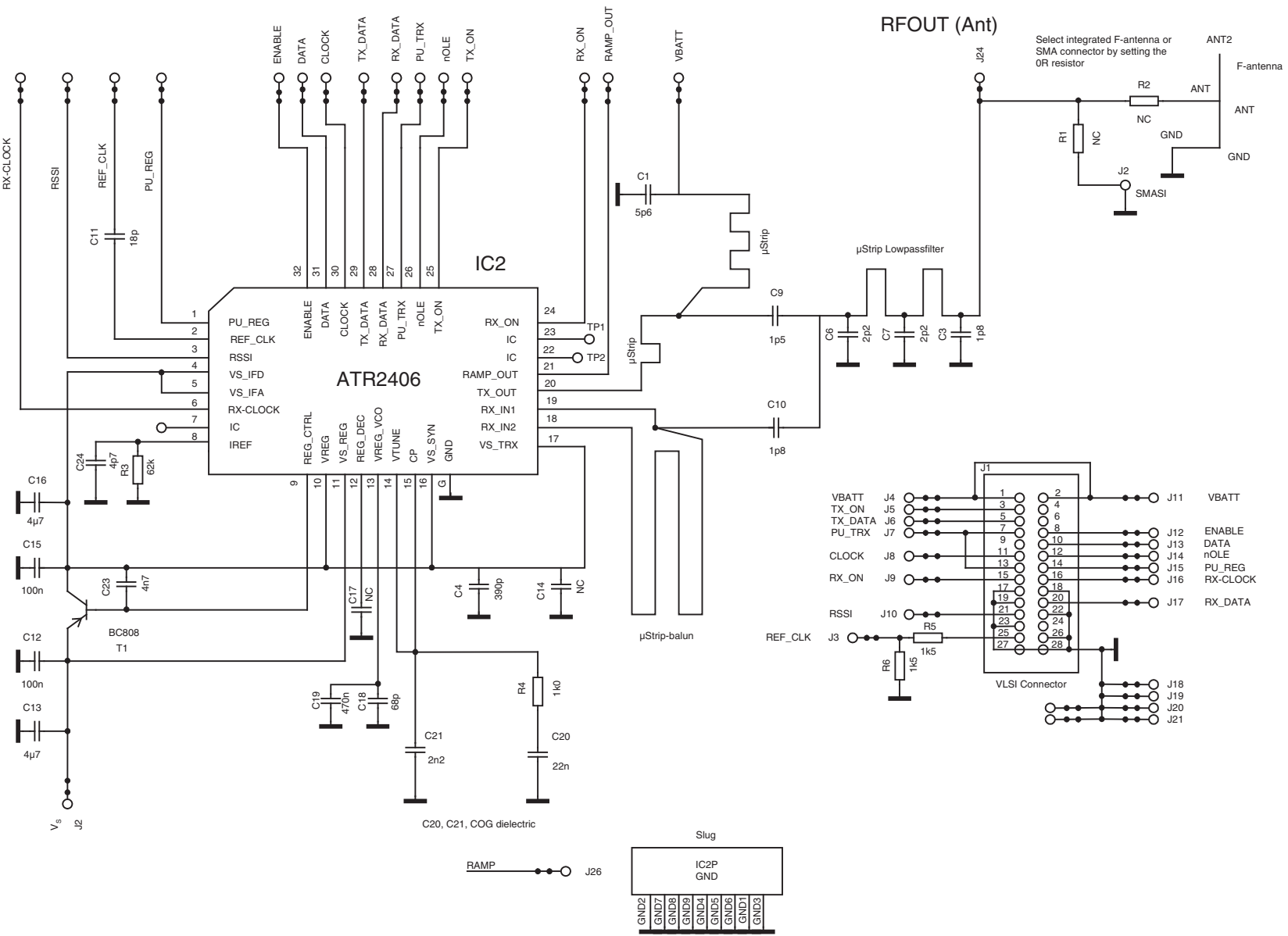
Figure 8-3. Application Circuit for ATR2406-DEV-BOARD
