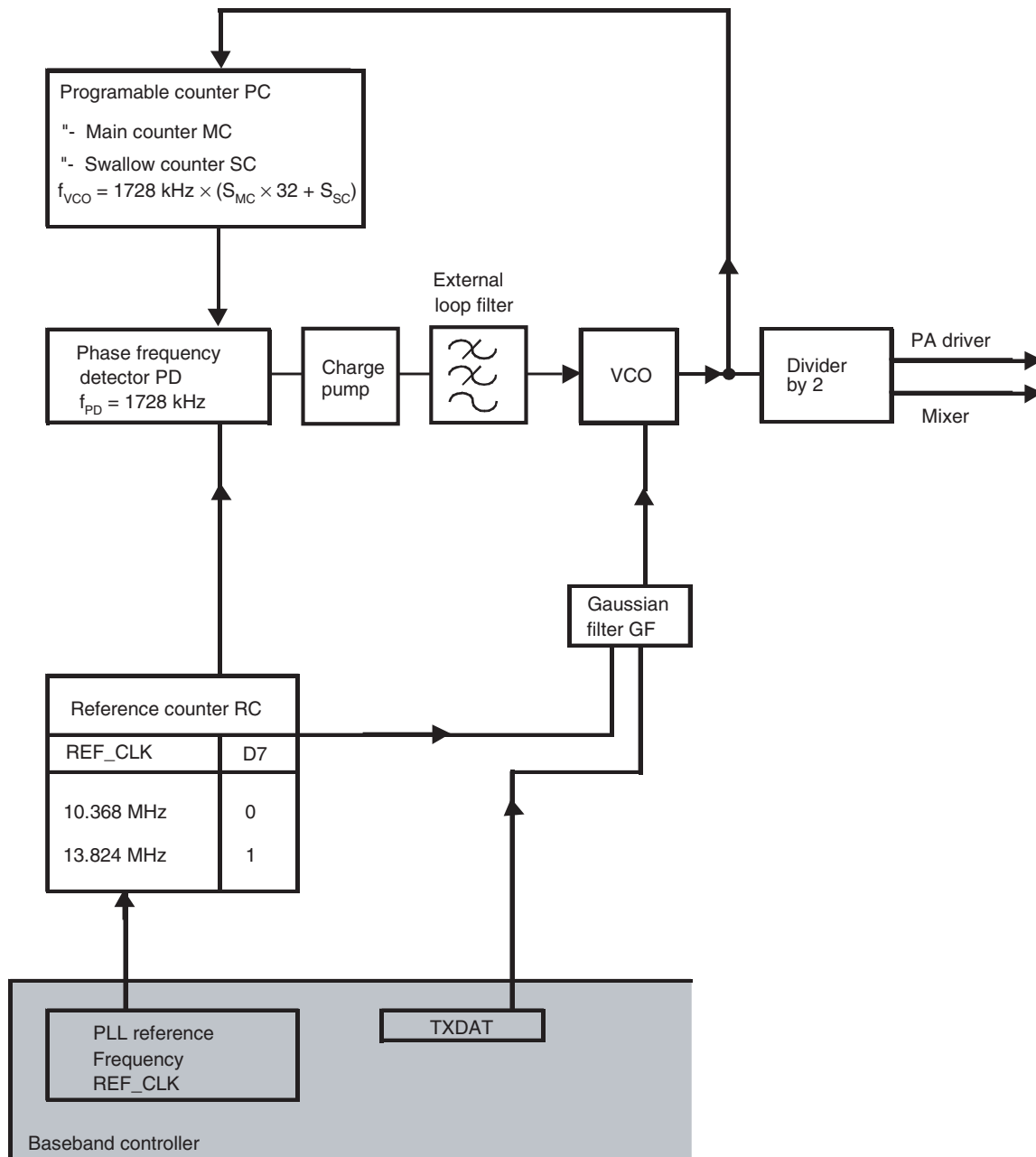
Figure 7-1. PLL Principle
