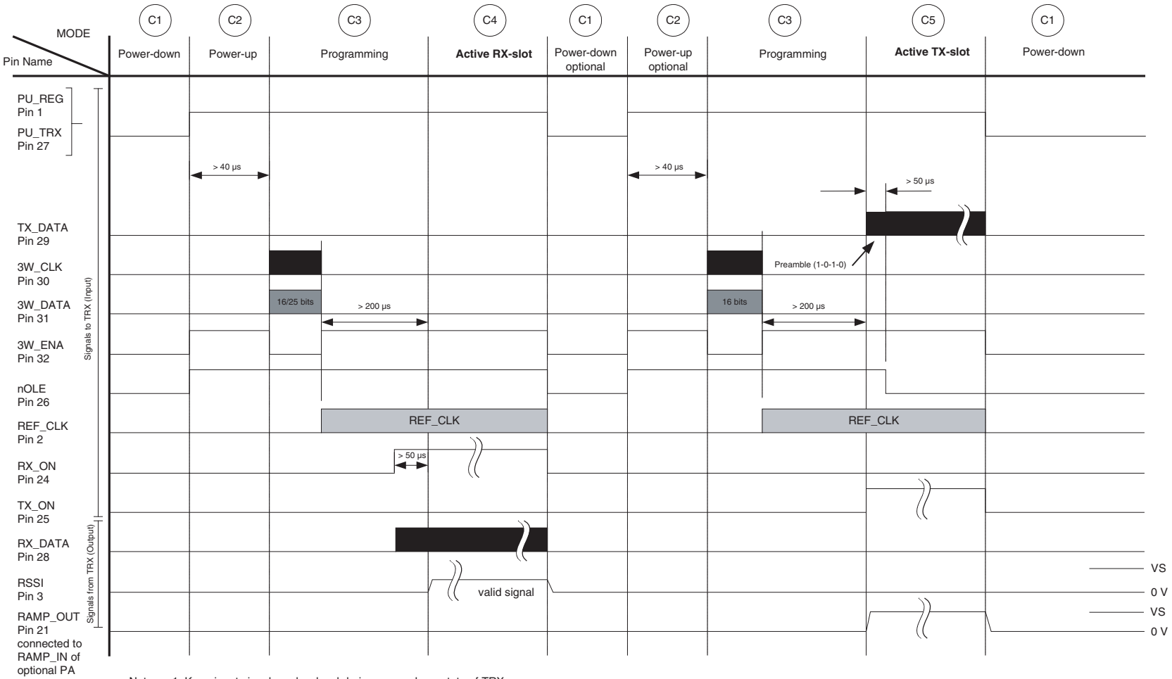
Figure 7-3. Example TX and RX Timing Diagram
