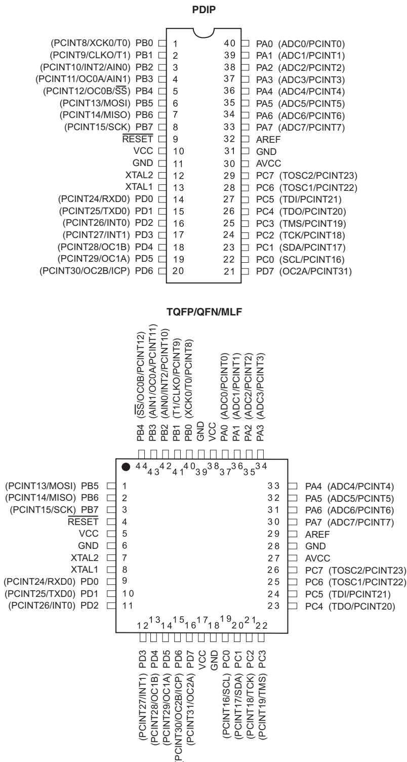
Figure 1-1. Pinout ATmega644
