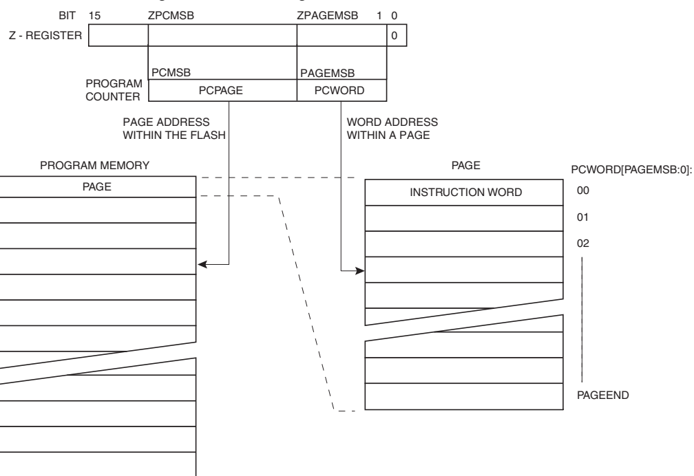
Figure 24-3. Addressing the Flash During SPM (1)
