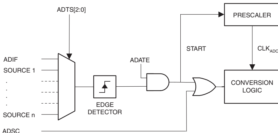
Figure 109. ADC Auto Trigger Logic
