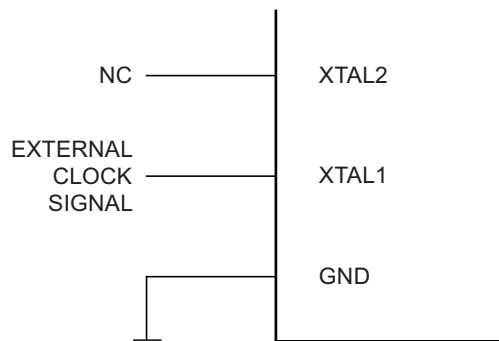
Figure 9-4. External Clock Drive Configuration
