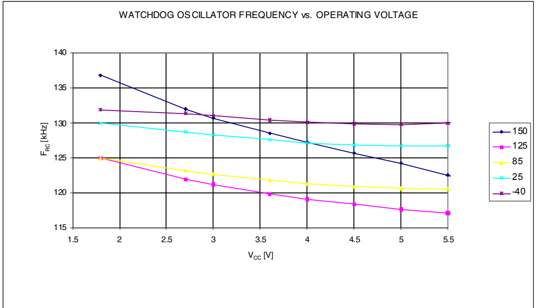
Figure 29-22. ATmega164P-B: Watchdog Oscillator Frequency vs. V_{CC}
