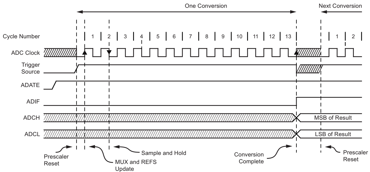
Figure 23-6. ADC Timing Diagram, Auto Triggerred Conversion
