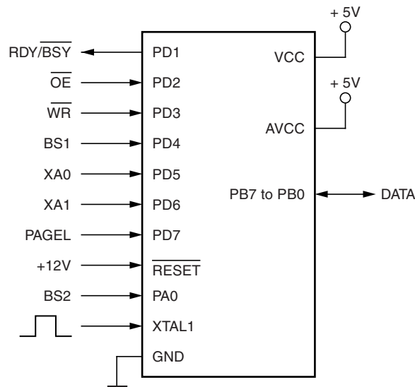
Figure 27-1. Parallel Programming (1)
