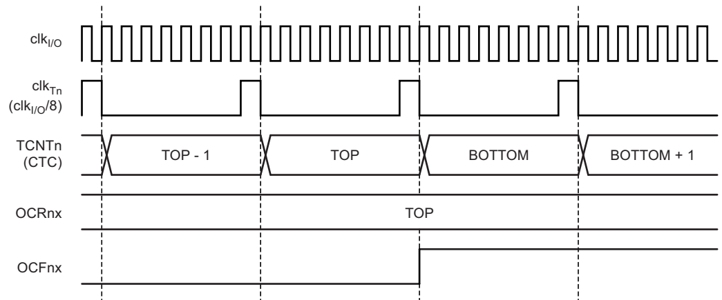
Figure 17-11. Timer/Counter Timing Diagram, Clear Timer on Compare Match mode, with Prescaler ( f_{clk_{I/O}}/8 )
