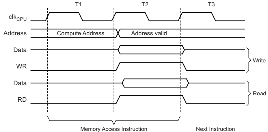
Figure 8-3. On-chip Data SRAM Access Cycles
