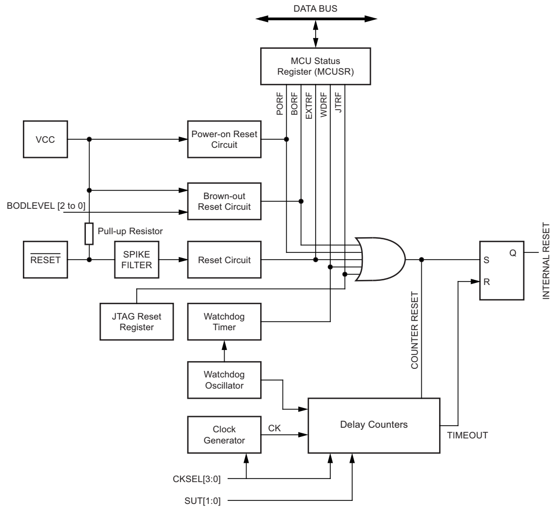
Figure 11-1. Reset Logic
