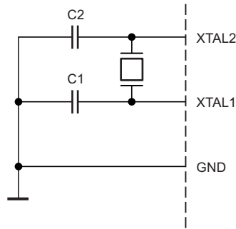
Figure 9-2. Crystal Oscillator Connections
