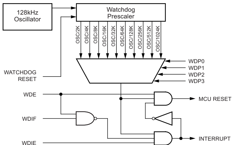
Figure 11-7. Watchdog Timer
