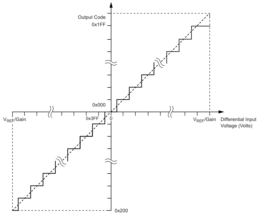
Figure 23-14. Differential Measurement Range
