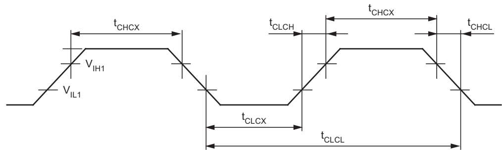
Figure 28-2. External Clock Drive Waveforms
