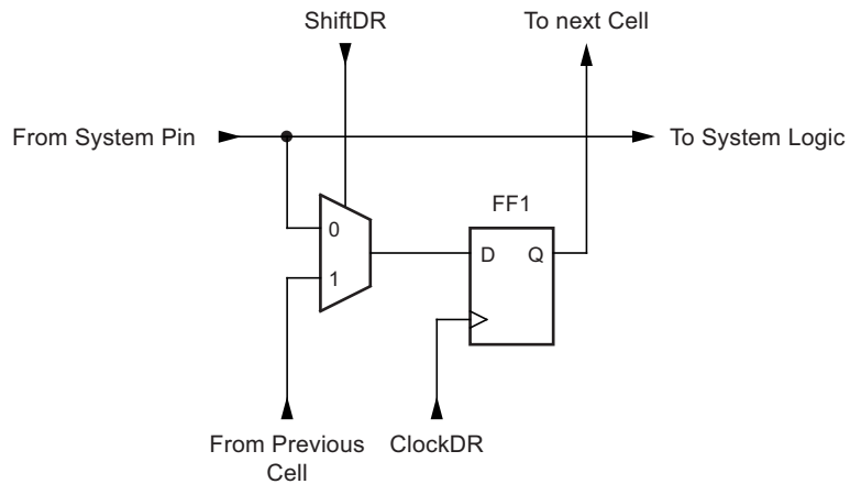
Figure 25-5. Observe-only Cell
