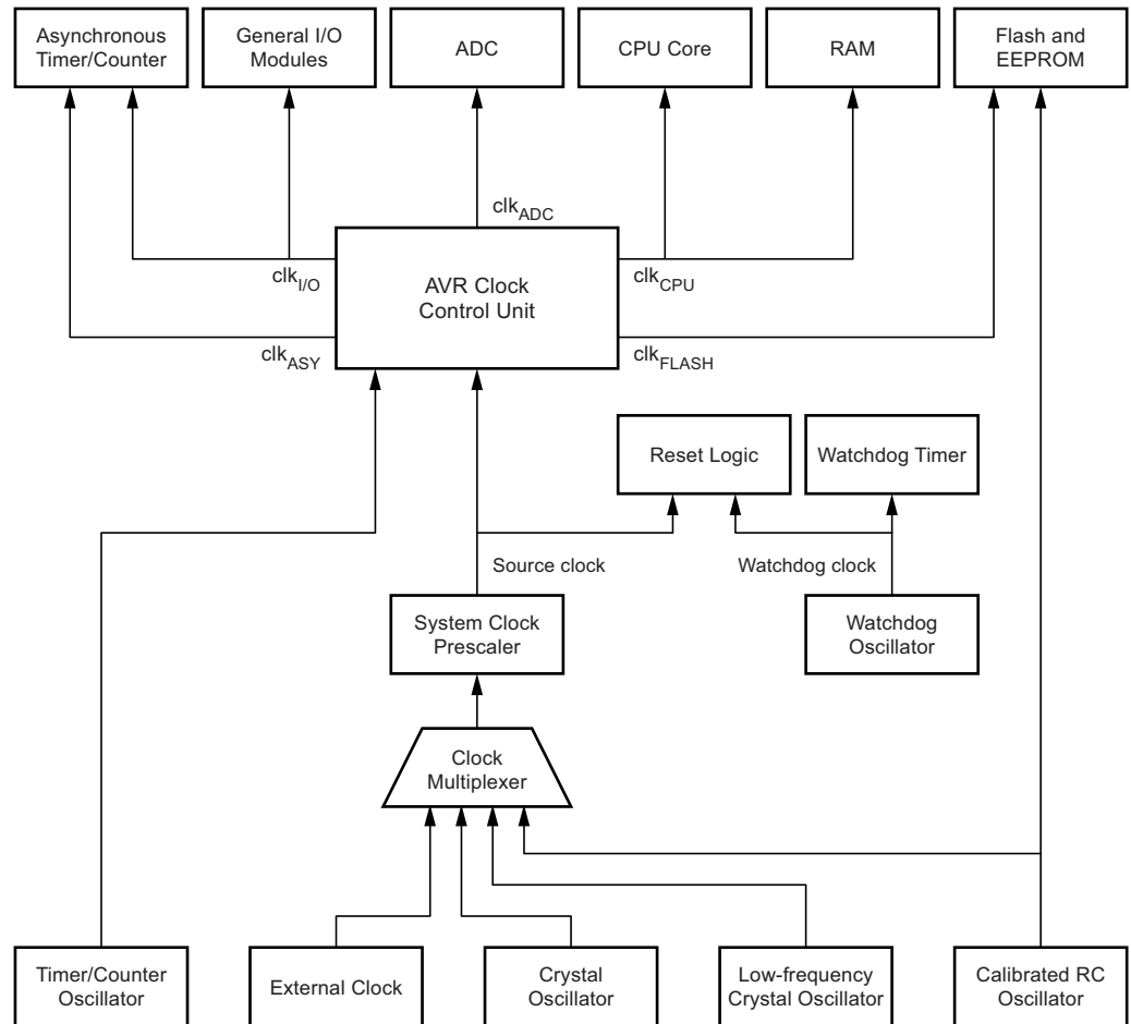
Figure 9-1. Clock Distribution
