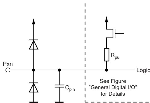
Figure 14-1. I/O Pin Equivalent Schematic
