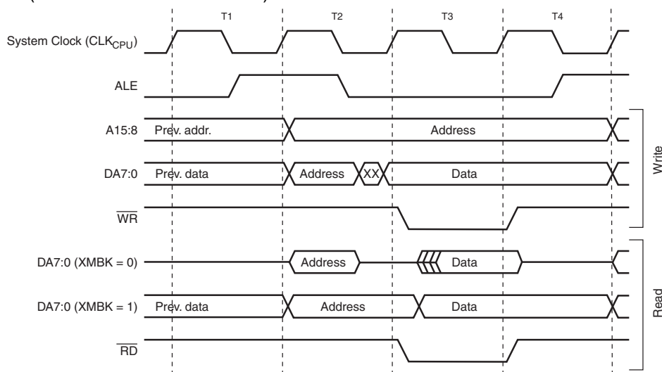
Figure 13. External Data Memory Cycles without Wait-state (SRWn1 = 0 and SRWn0 = 0) (1)
