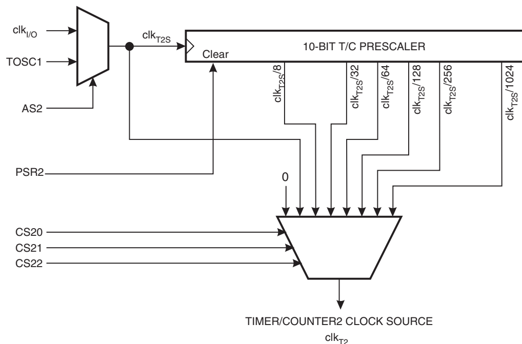
Figure 70. Prescaler for Timer/Counter2
