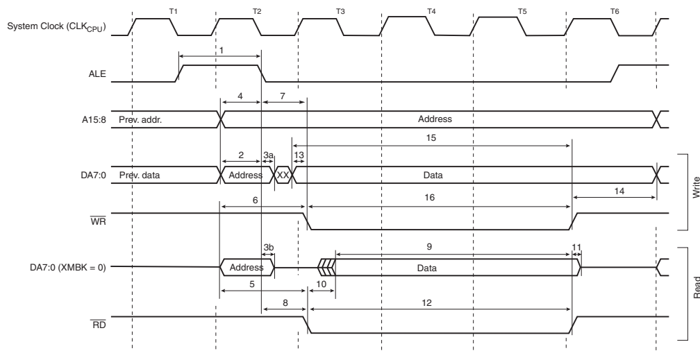
Figure 120. External Memory Timing (SRWn1 = 1, SRWn0 = 0)
