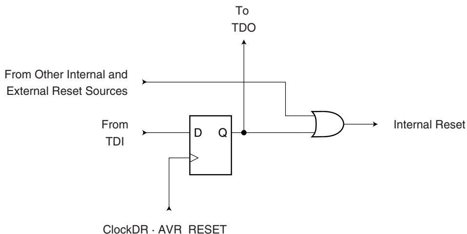
Figure 86. Reset Register
