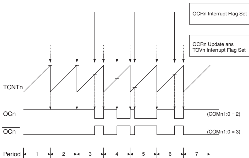
Figure 38. Fast PWM Mode, Timing Diagram
