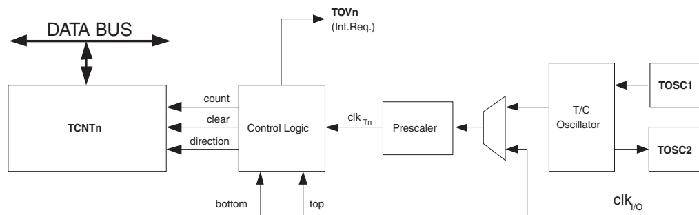
Figure 60. Counter Unit Block Diagram
