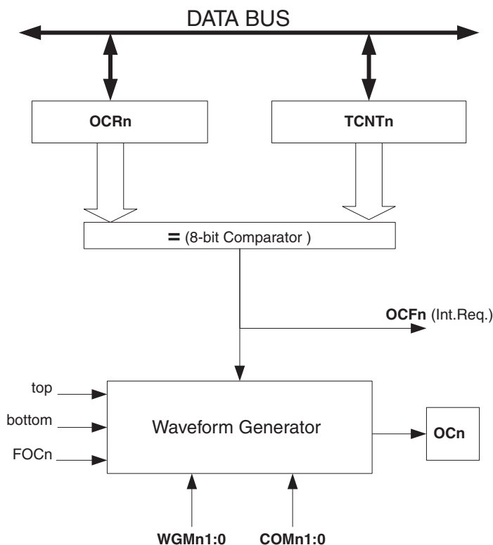
Figure 35. Output Compare Unit, Block Diagram
