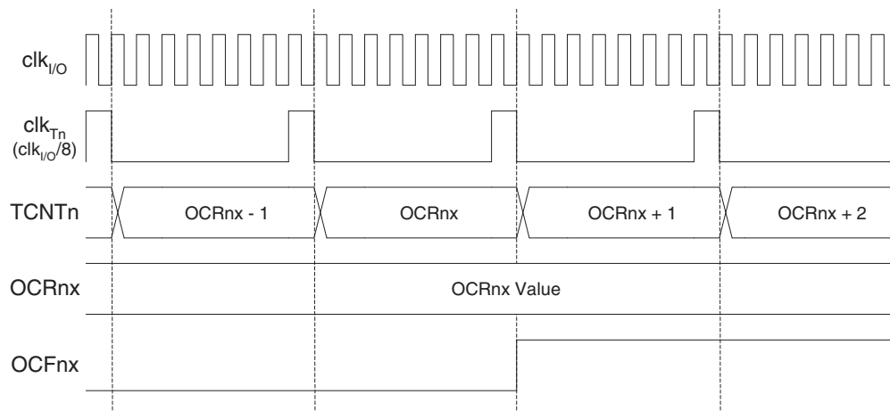
Figure 56. Timer/Counter Timing Diagram, Setting of \text{OCF}_{nx} , with Prescaler ( f_{\text{clk}_{I/O}}/8 )
