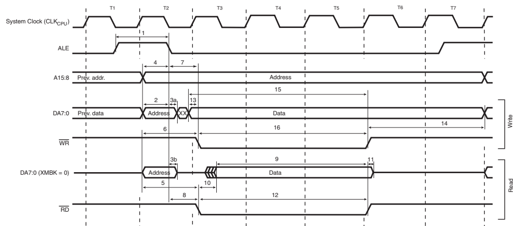
Figure 121. External Memory Timing (SRWn1 = 1, SRWn0 = 1) (1)
