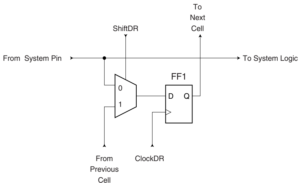
Figure 89. Observe-only Cell
