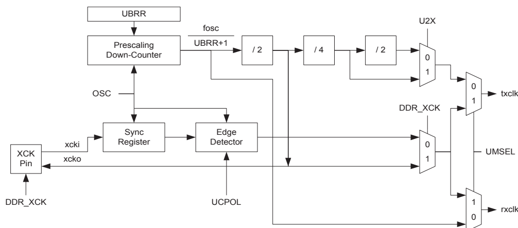
Figure 76. Clock Generation Logic, Block Diagram
