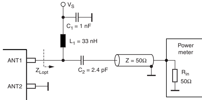
Figure 8-4. Output Power Measurement ATA8742
