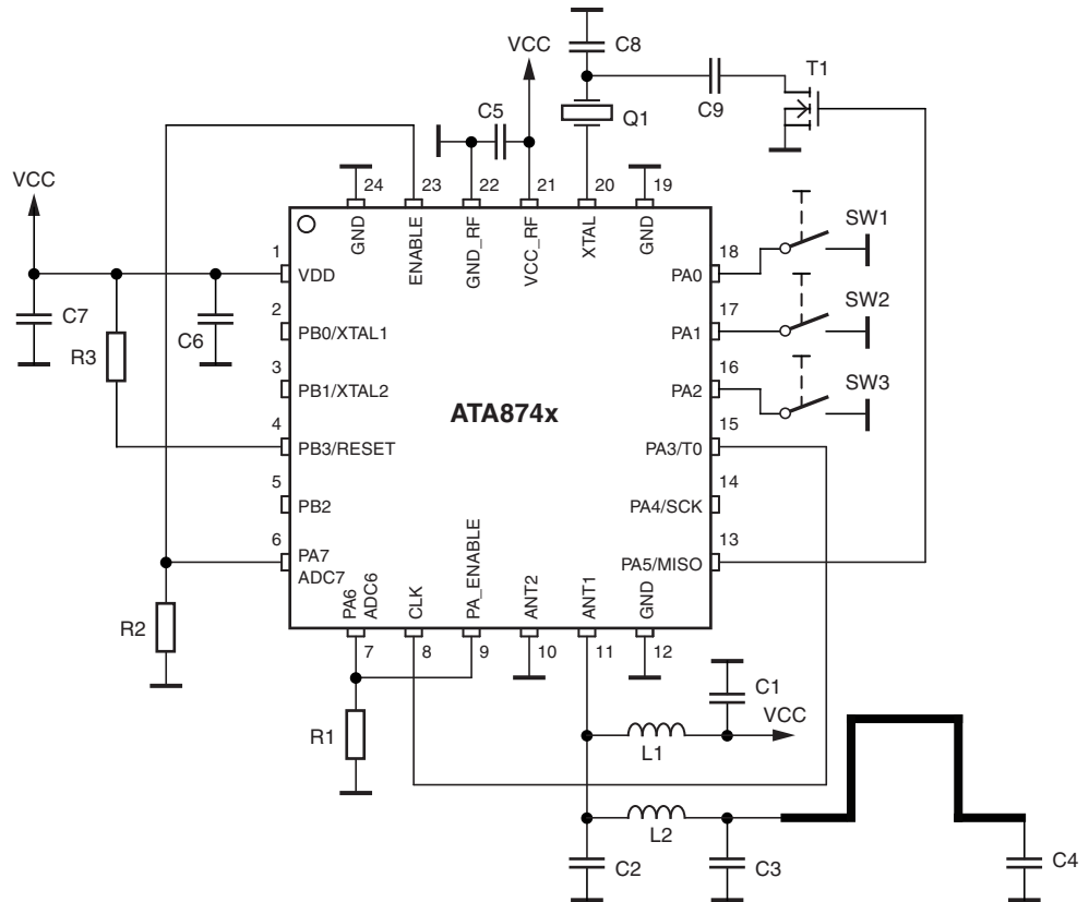
Figure 8-3. Typical FSK Application ATA8742
