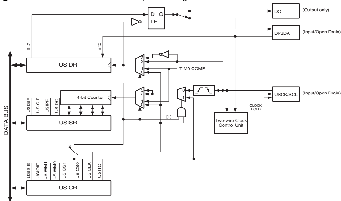
Figure 23-1. Universal Serial Interface, Block Diagram
